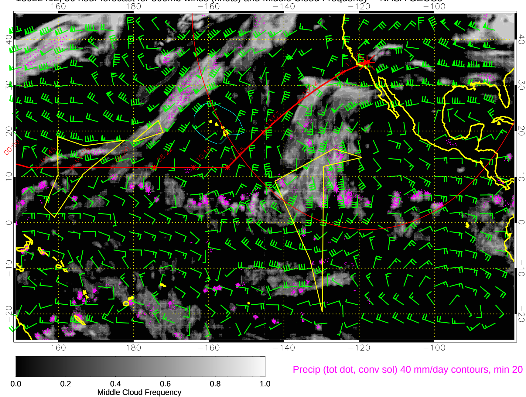
15022412, 36 hour forecast for 500mb winds (knots) and Middle Cloud Frequency -- NASA GEOS5
