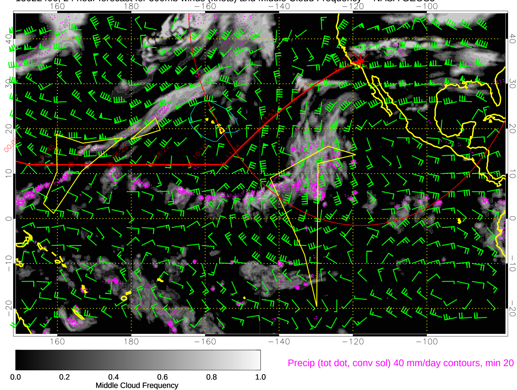
15022400, 24 hour forecast for 500mb winds (knots) and Middle Cloud Frequency -- NASA GEOS5
