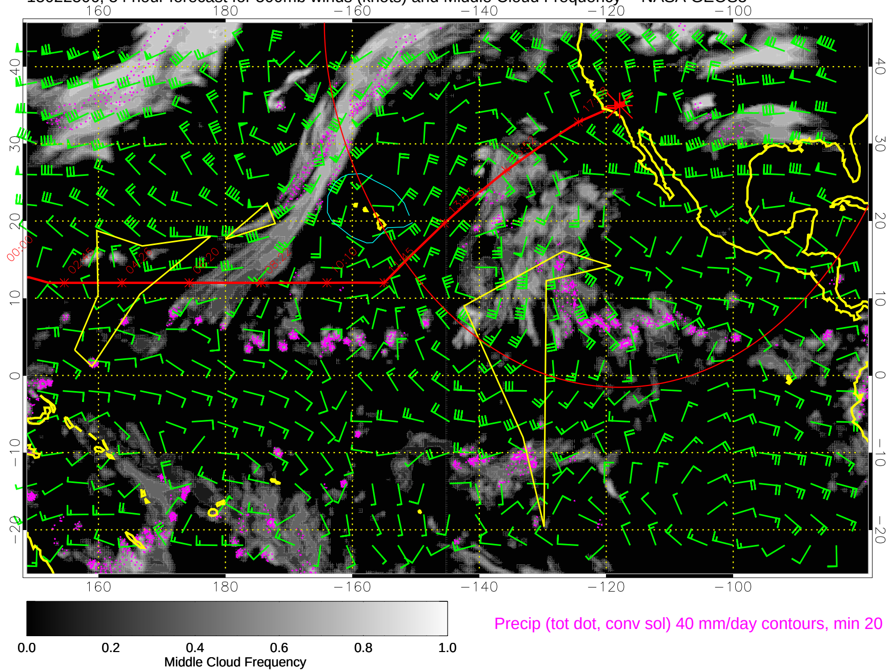
15022506, 54 hour forecast for 500mb winds (knots) and Middle Cloud Frequency -- NASA GEOS5
