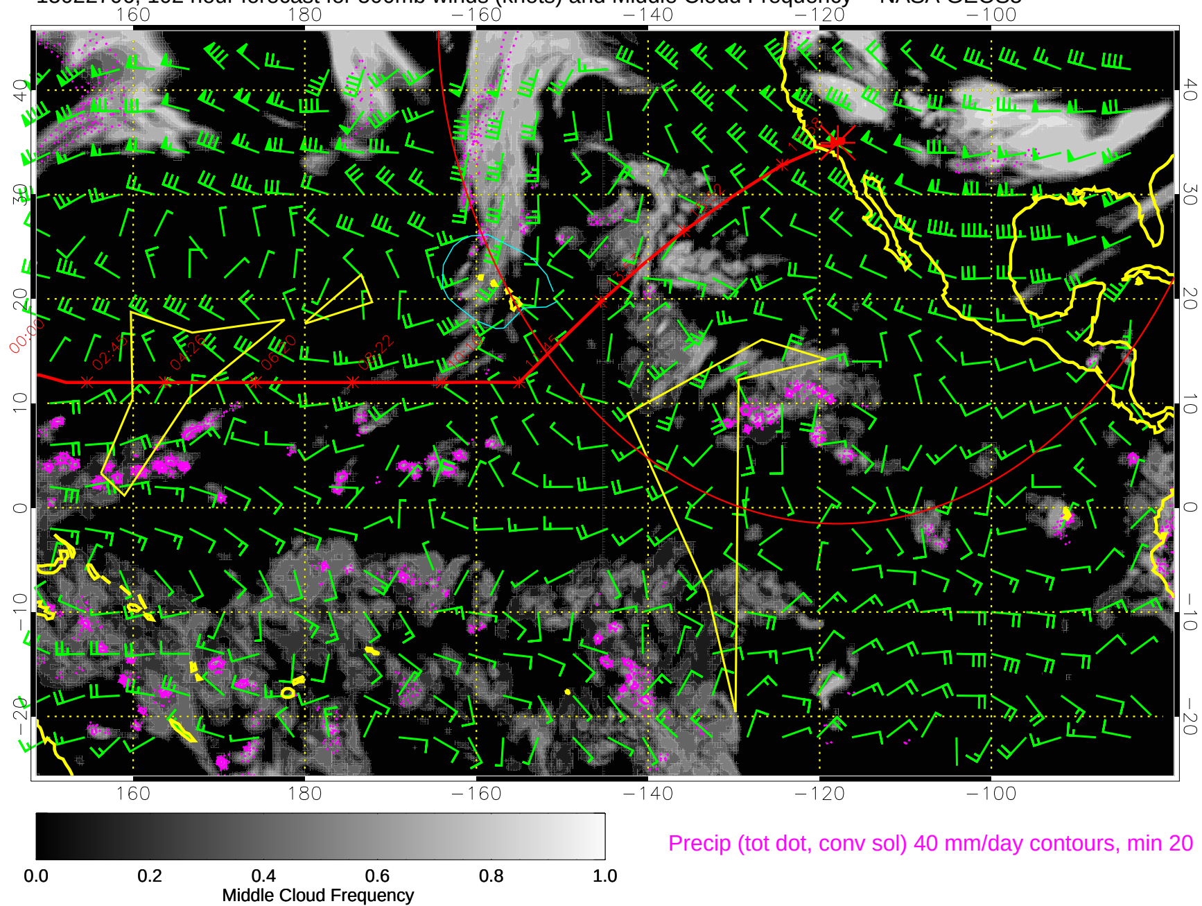
15022706, 102 hour forecast for 500mb winds (knots) and Middle Cloud Frequency -- NASA GEOS5
