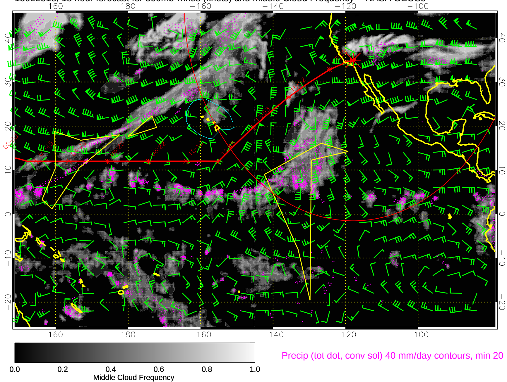
15022318, 18 hour forecast for 500mb winds (knots) and Middle Cloud Frequency -- NASA GEOS5
