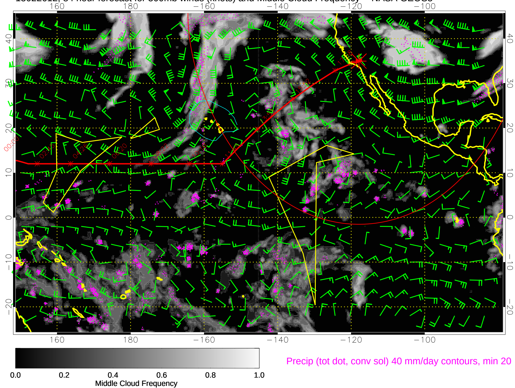
15022612, 84 hour forecast for 500mb winds (knots) and Middle Cloud Frequency -- NASA GEOS5
