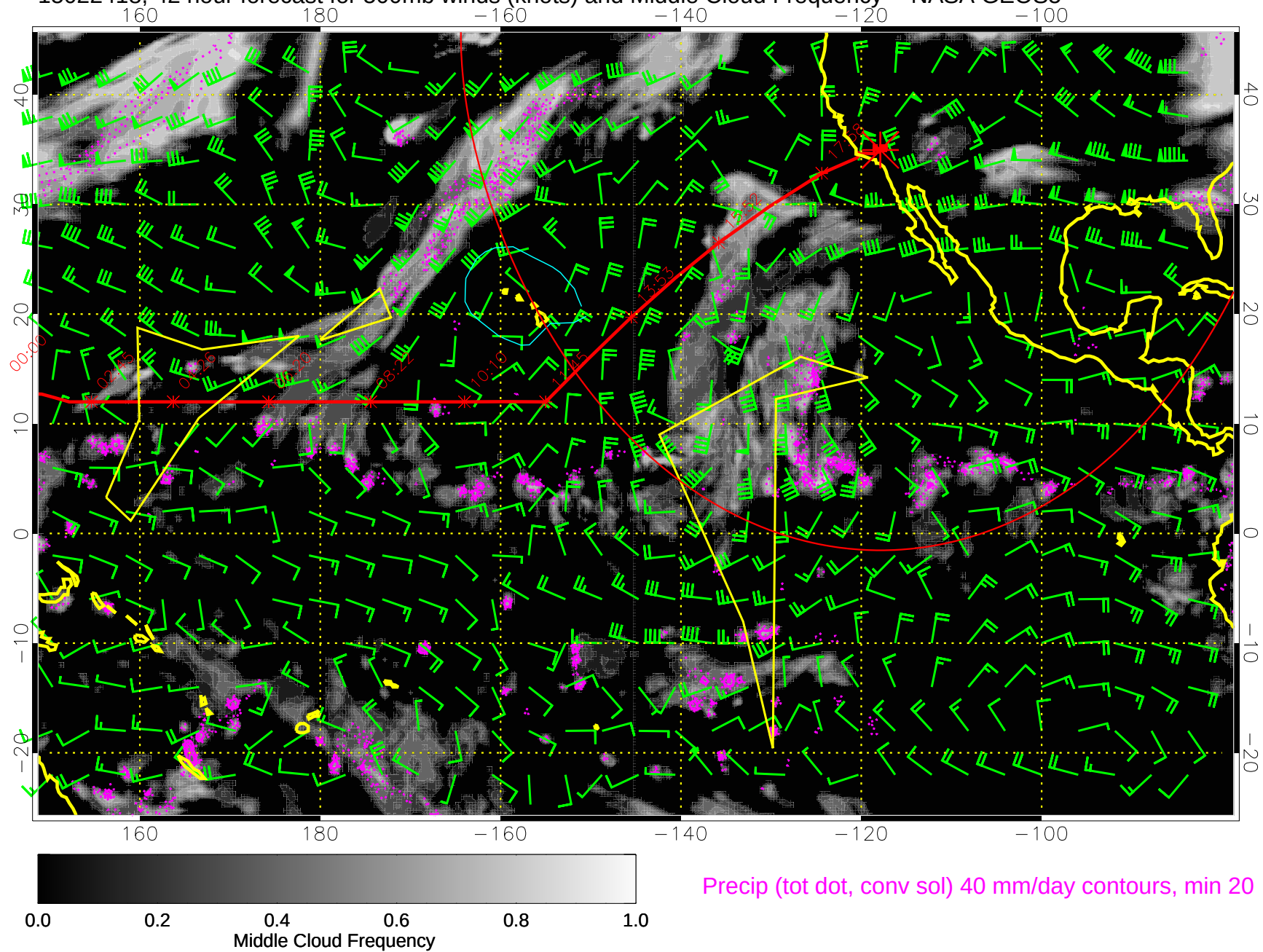
15022418, 42 hour forecast for 500mb winds (knots) and Middle Cloud Frequency -- NASA GEOS5
