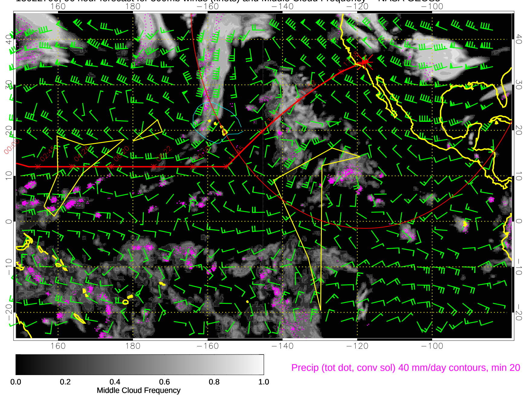
15022700, 96 hour forecast for 500mb winds (knots) and Middle Cloud Frequency -- NASA GEOS5
