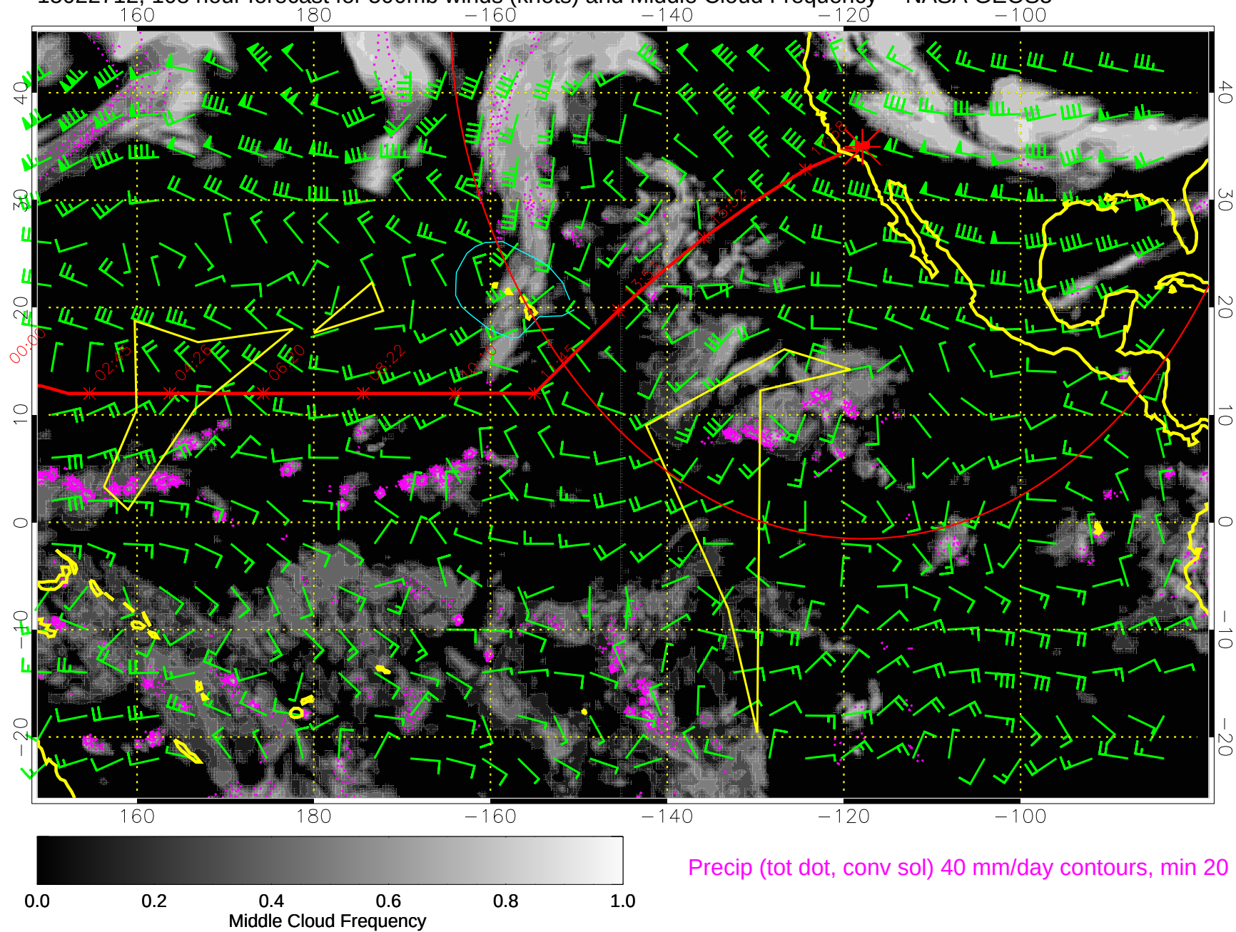
15022712, 108 hour forecast for 500mb winds (knots) and Middle Cloud Frequency -- NASA GEOS5
