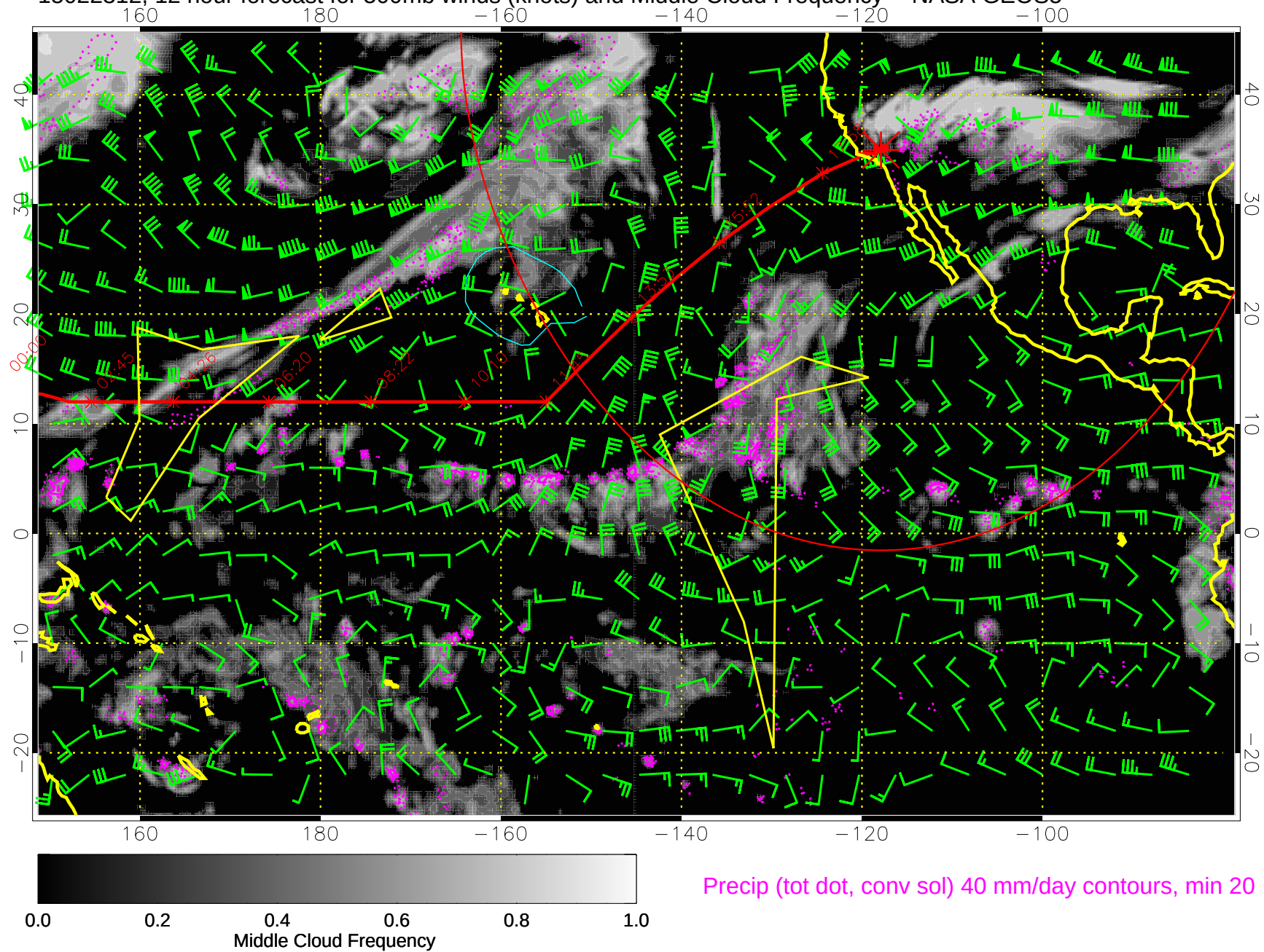
15022312, 12 hour forecast for 500mb winds (knots) and Middle Cloud Frequency -- NASA GEOS5
