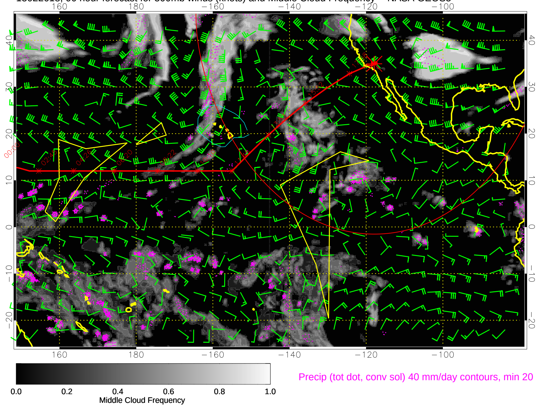
15022618, 90 hour forecast for 500mb winds (knots) and Middle Cloud Frequency -- NASA GEOS5
