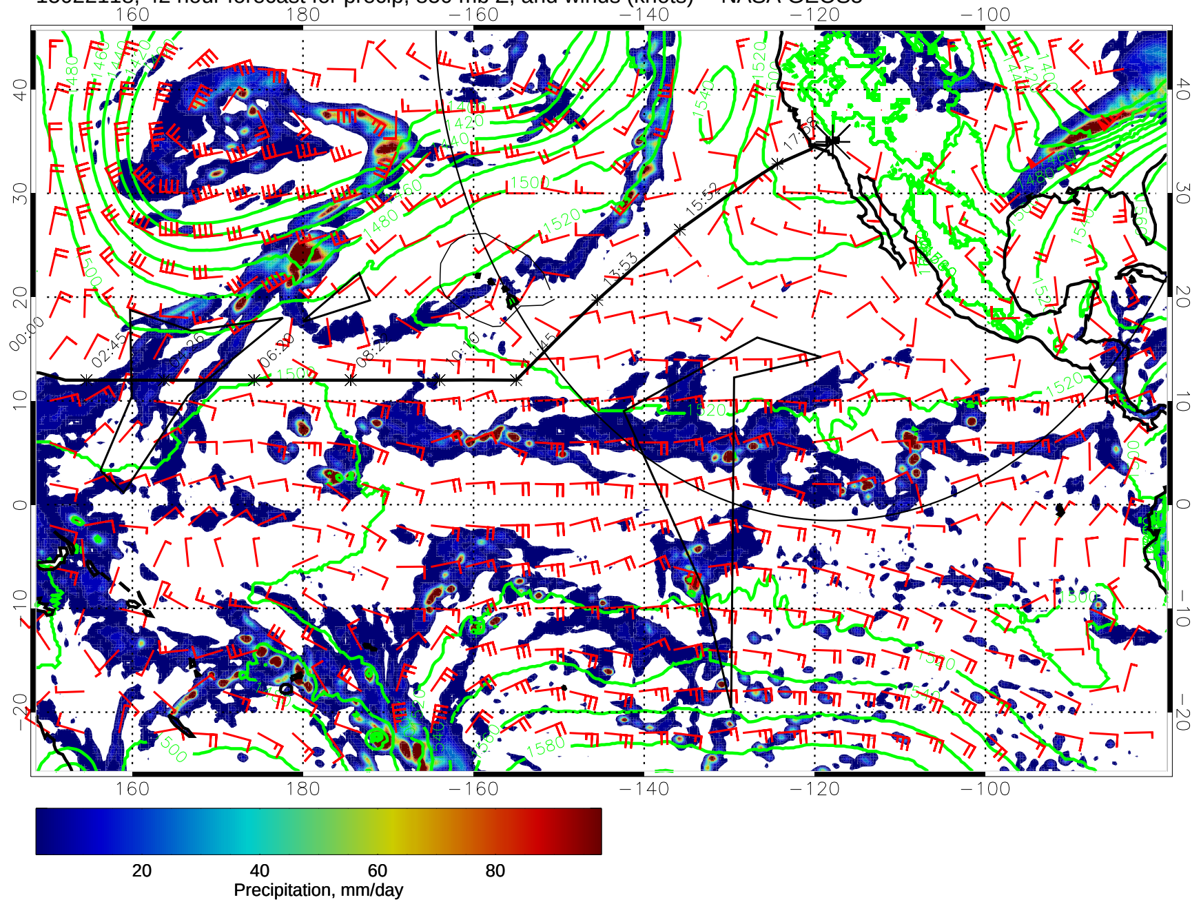
15022118, 42 hour forecast for precip, 850 mb Z, and winds (knots) -- NASA GEOS5
