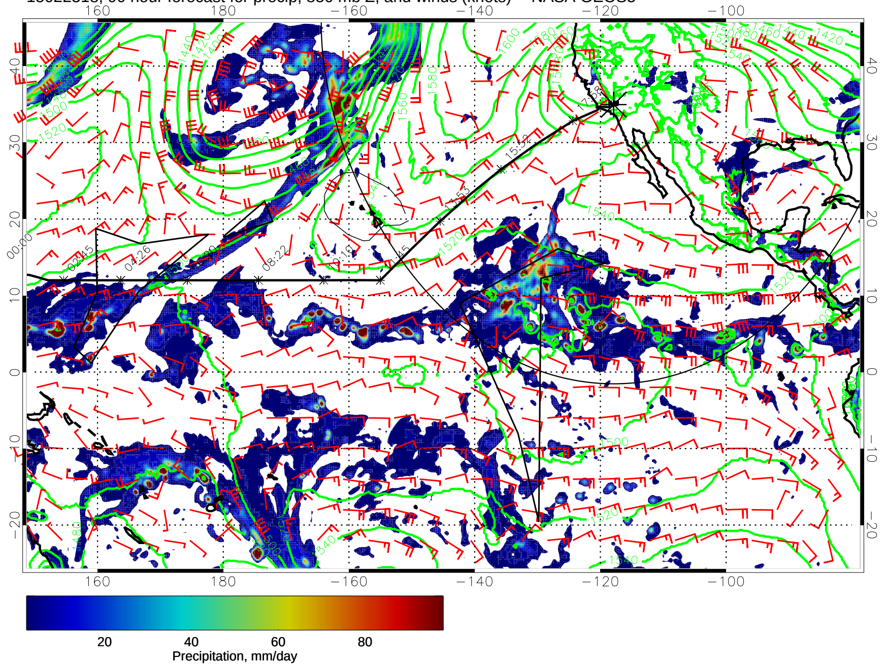
15022318, 90 hour forecast for precip, 850 mb Z, and winds (knots) -- NASA GEOS5
