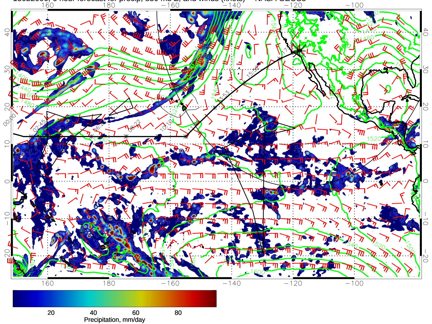
15022006, 6 hour forecast for precip, 850 mb Z, and winds (knots) -- NASA GEOS5
