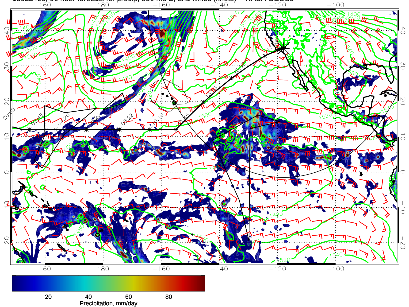
15022400, 96 hour forecast for precip, 850 mb Z, and winds (knots) -- NASA GEOS5
