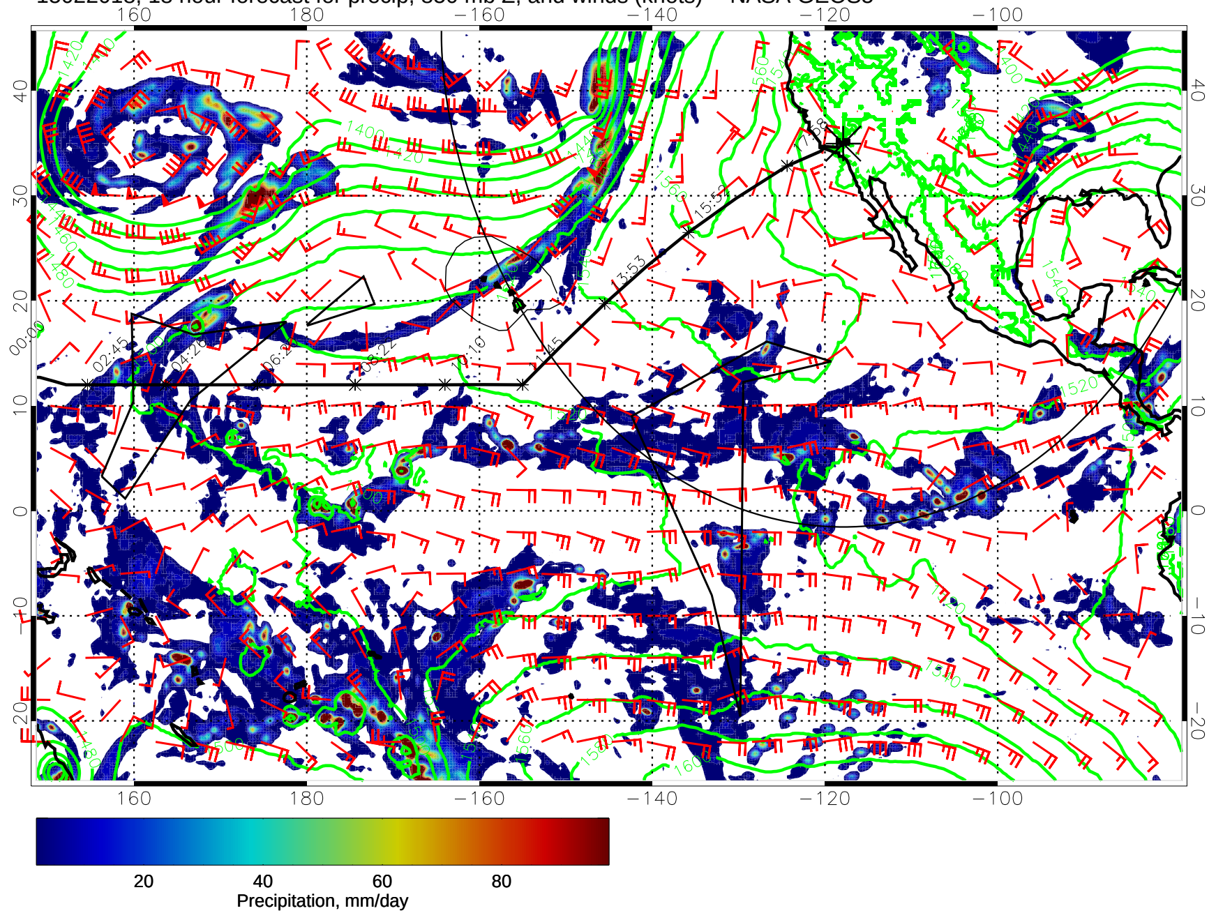
15022018, 18 hour forecast for precip, 850 mb Z, and winds (knots) -- NASA GEOS5
