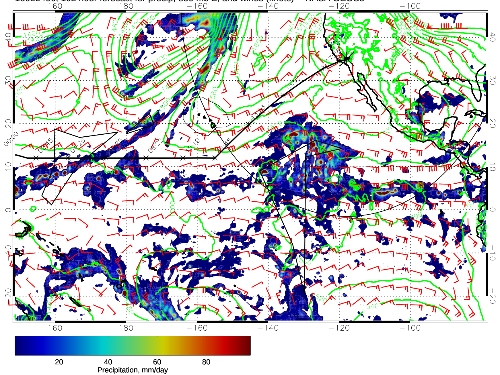
15022406, 102 hour forecast for precip, 850 mb Z, and winds (knots) -- NASA GEOS5
