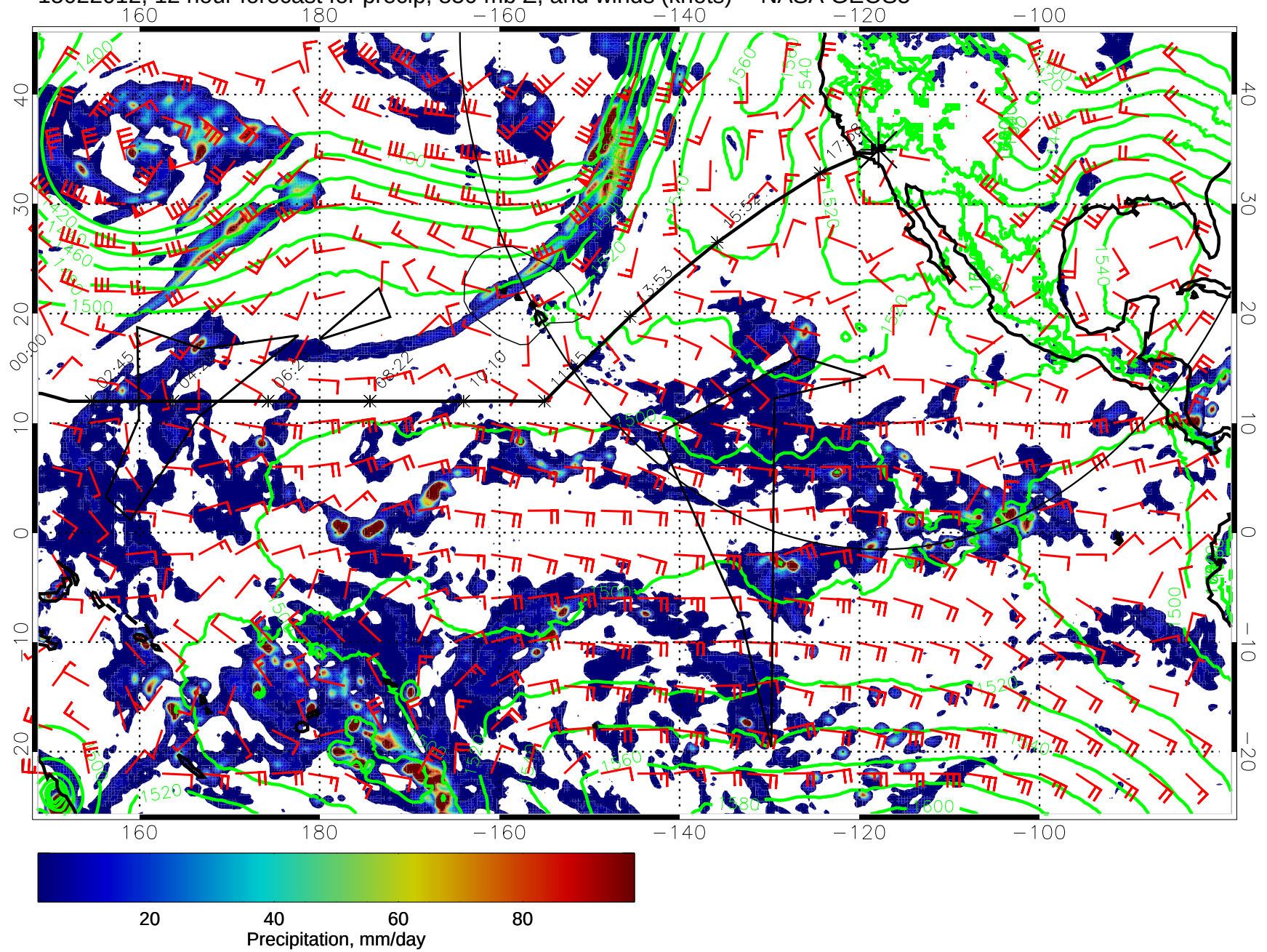
15022012, 12 hour forecast for precip, 850 mb Z, and winds (knots) -- NASA GEOS5
