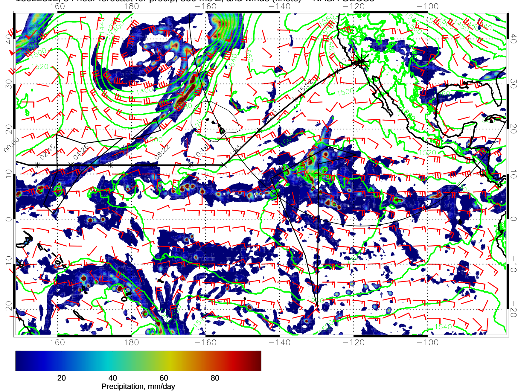
15022312, 84 hour forecast for precip, 850 mb Z, and winds (knots) -- NASA GEOS5
