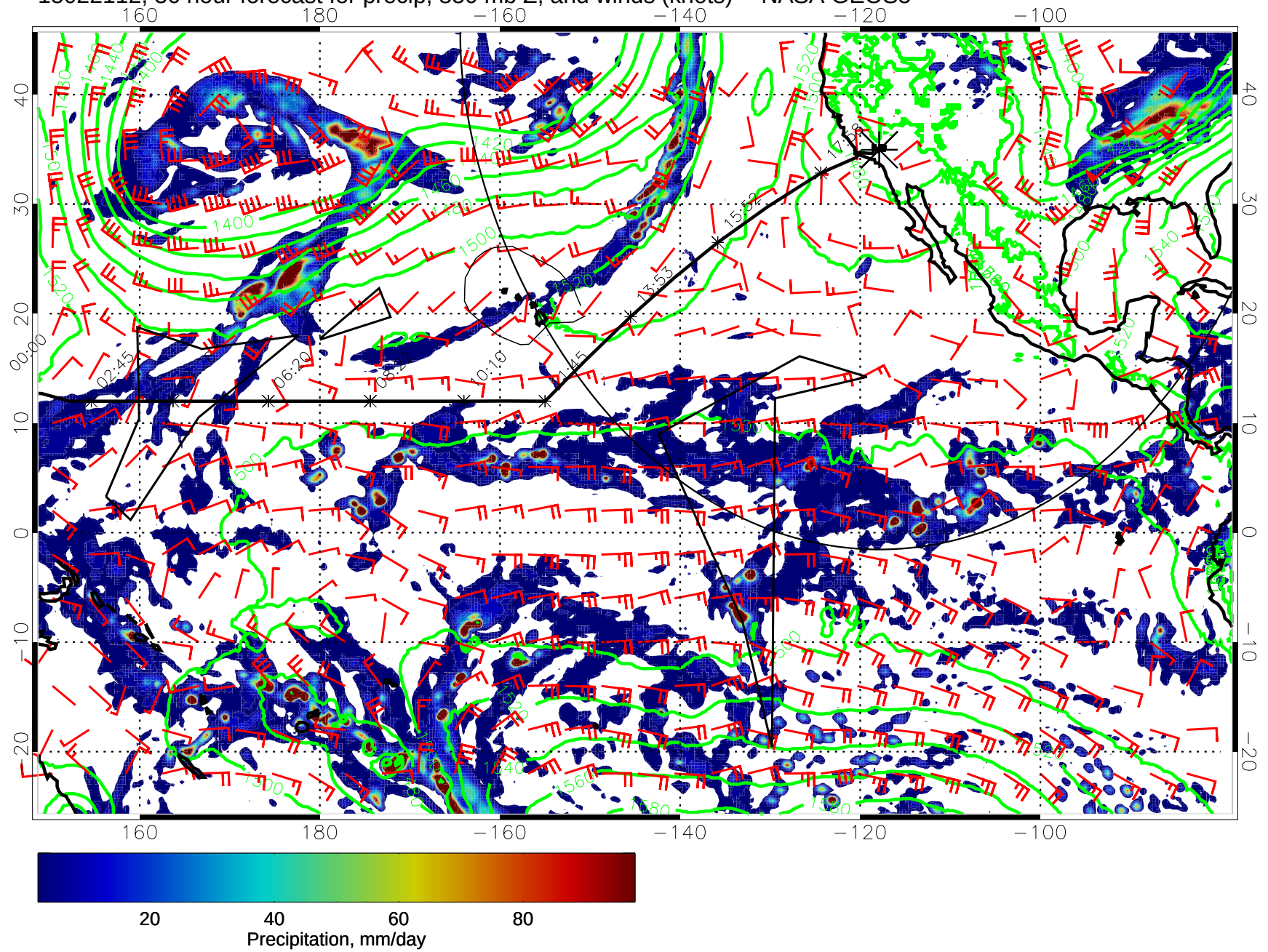
15022112, 36 hour forecast for precip, 850 mb Z, and winds (knots) -- NASA GEOS5
