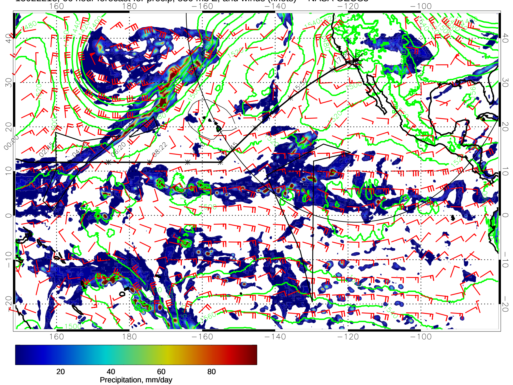
15022218, 66 hour forecast for precip, 850 mb Z, and winds (knots) -- NASA GEOS5
