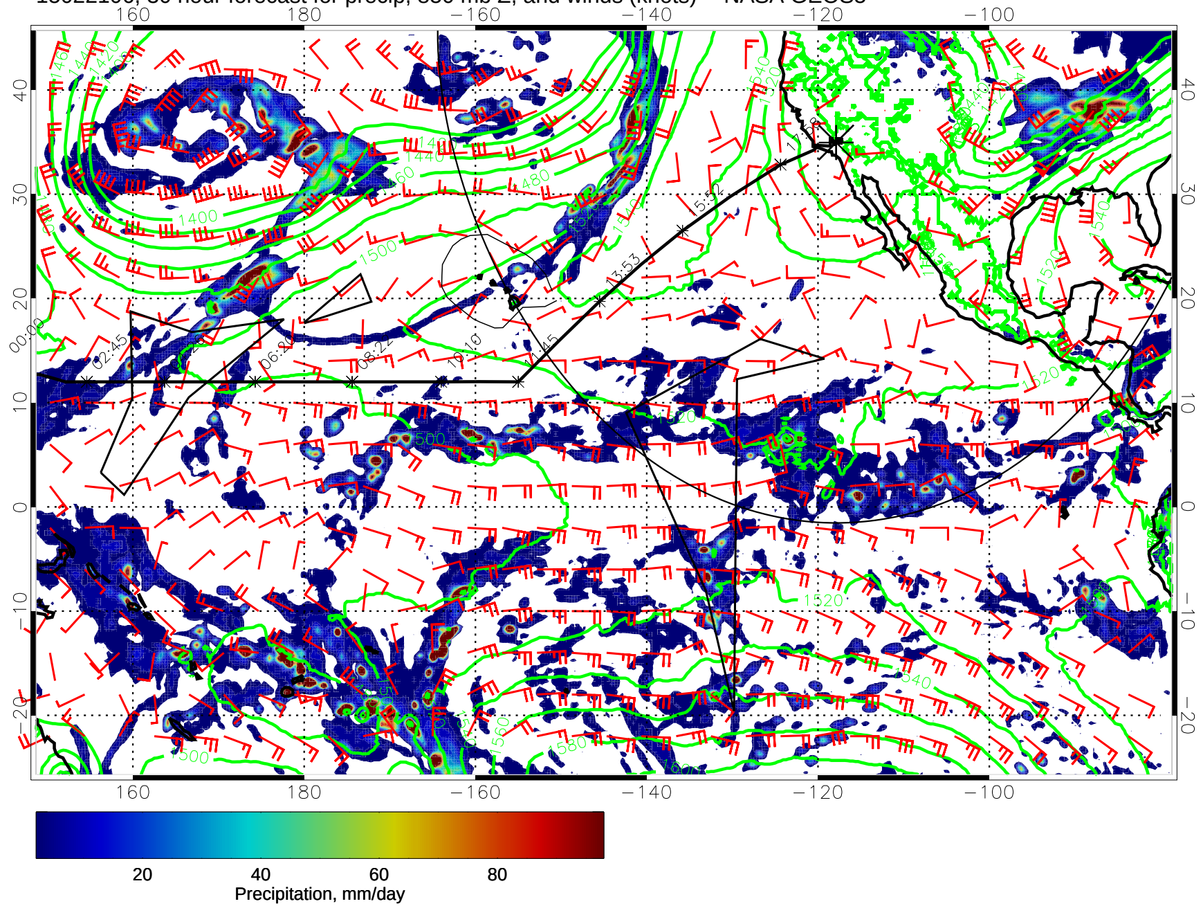
15022106, 30 hour forecast for precip, 850 mb Z, and winds (knots) -- NASA GEOS5
