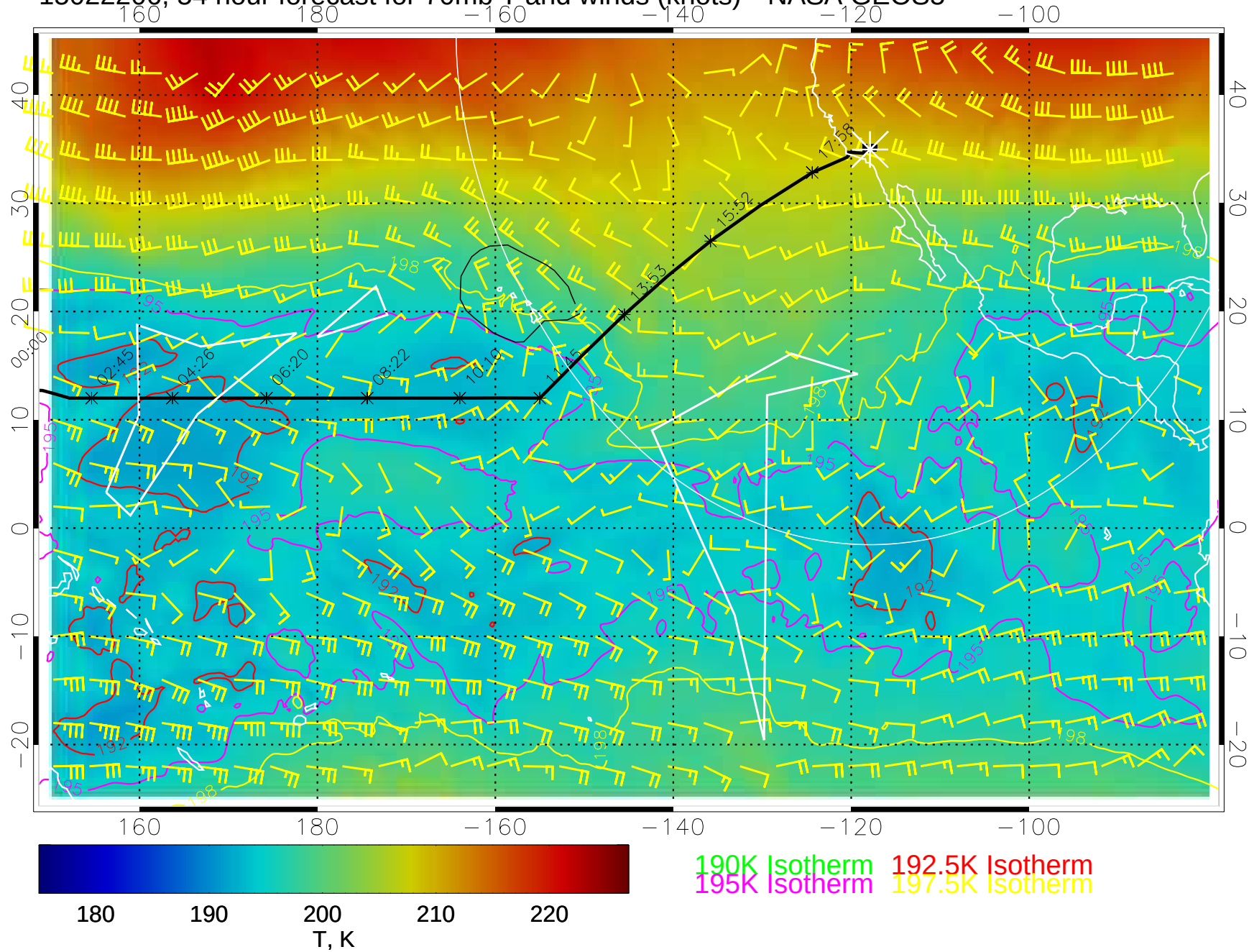
15022206, 54 hour forecast for 70mb T and winds (knots)-- NASA GEOS5
