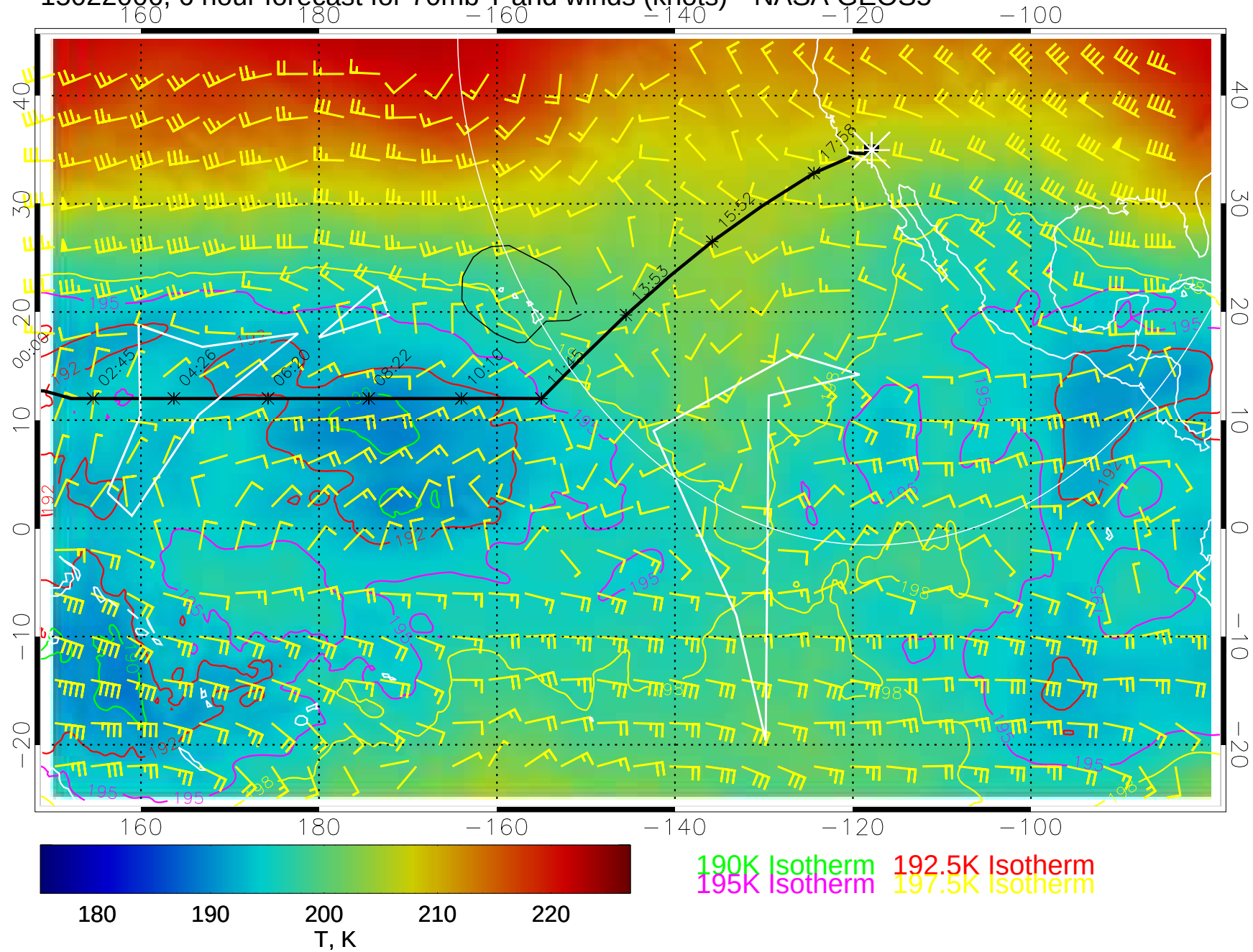
15022006, 6 hour forecast for 70mb T and winds (knots)-- NASA GEOS5
