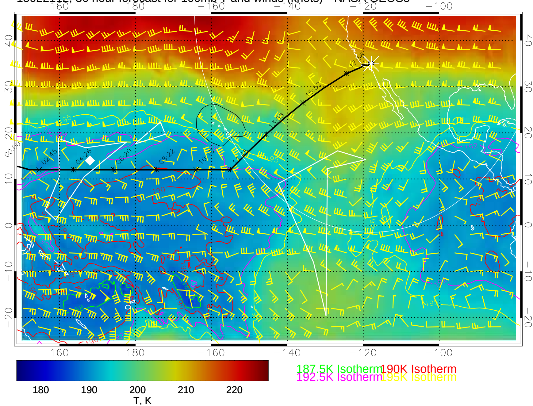
15022112, 36 hour forecast for 100mb T and winds (knots)-- NASA GEOS5
