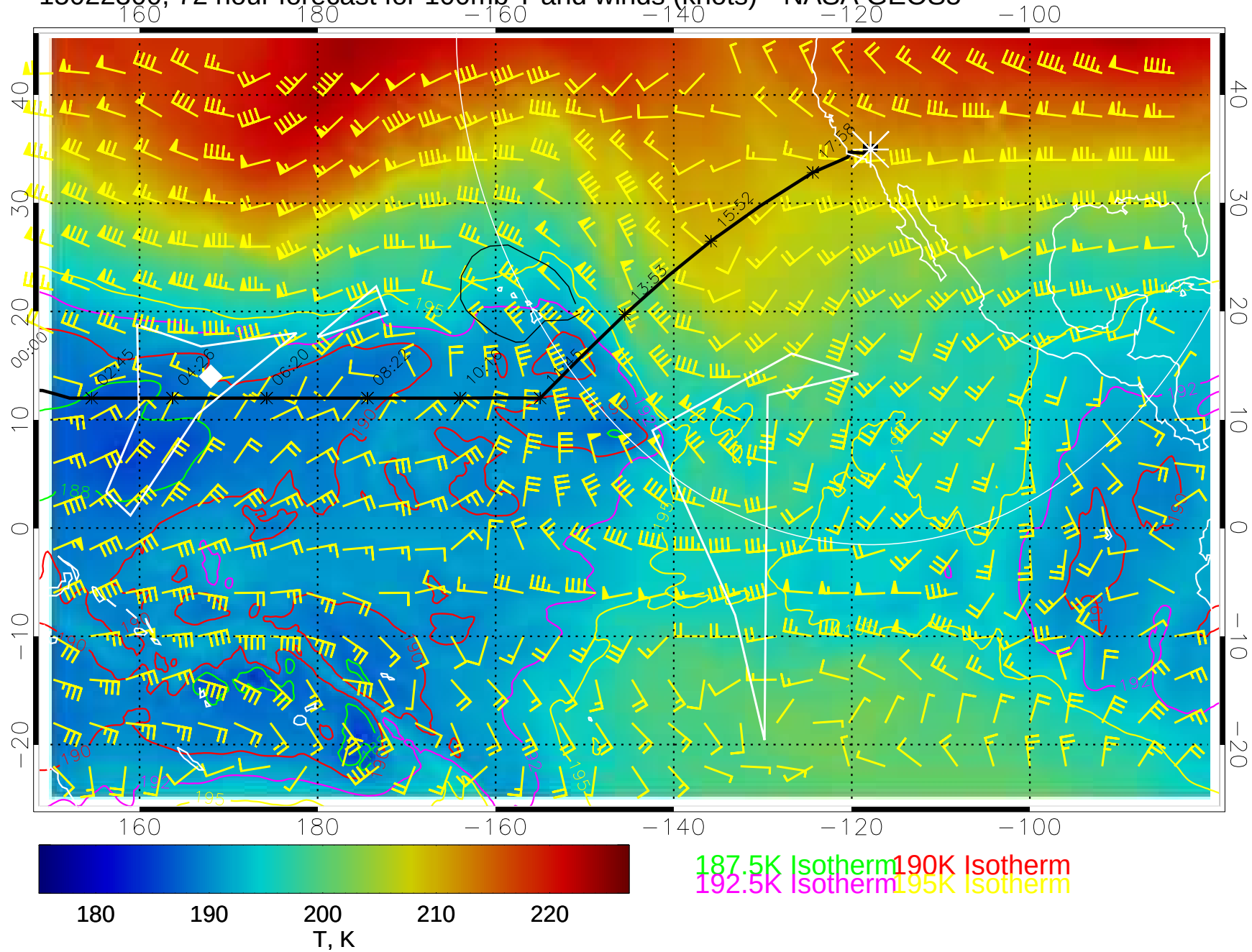
15022300, 72 hour forecast for 100mb T and winds (knots)-- NASA GEOS5
