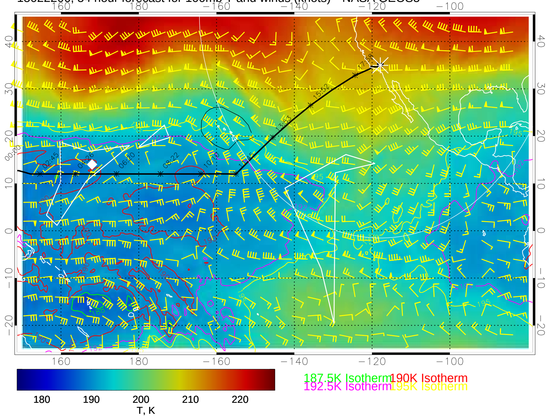
15022206, 54 hour forecast for 100mb T and winds (knots)-- NASA GEOS5
