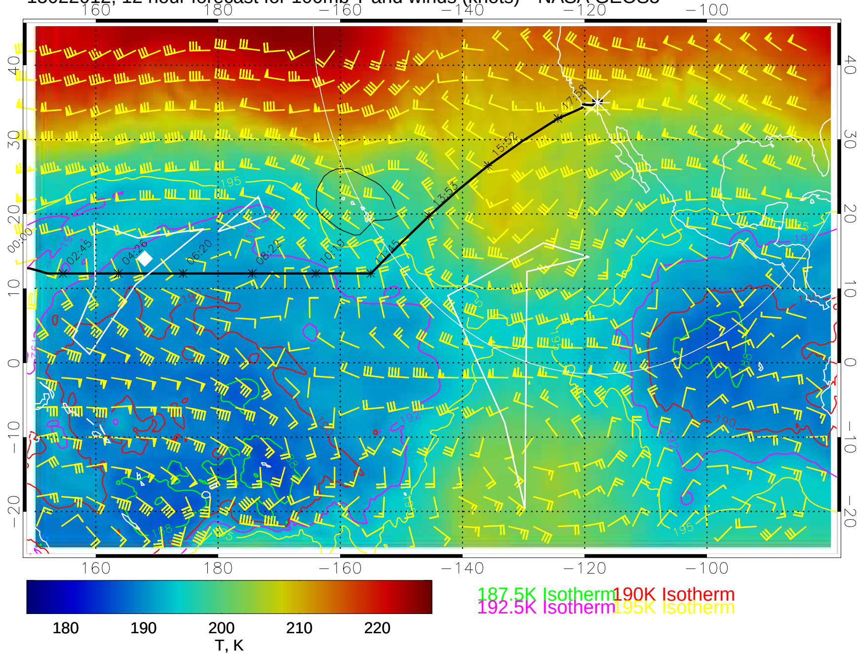
15022012, 12 hour forecast for 100mb T and winds (knots)-- NASA GEOS5
