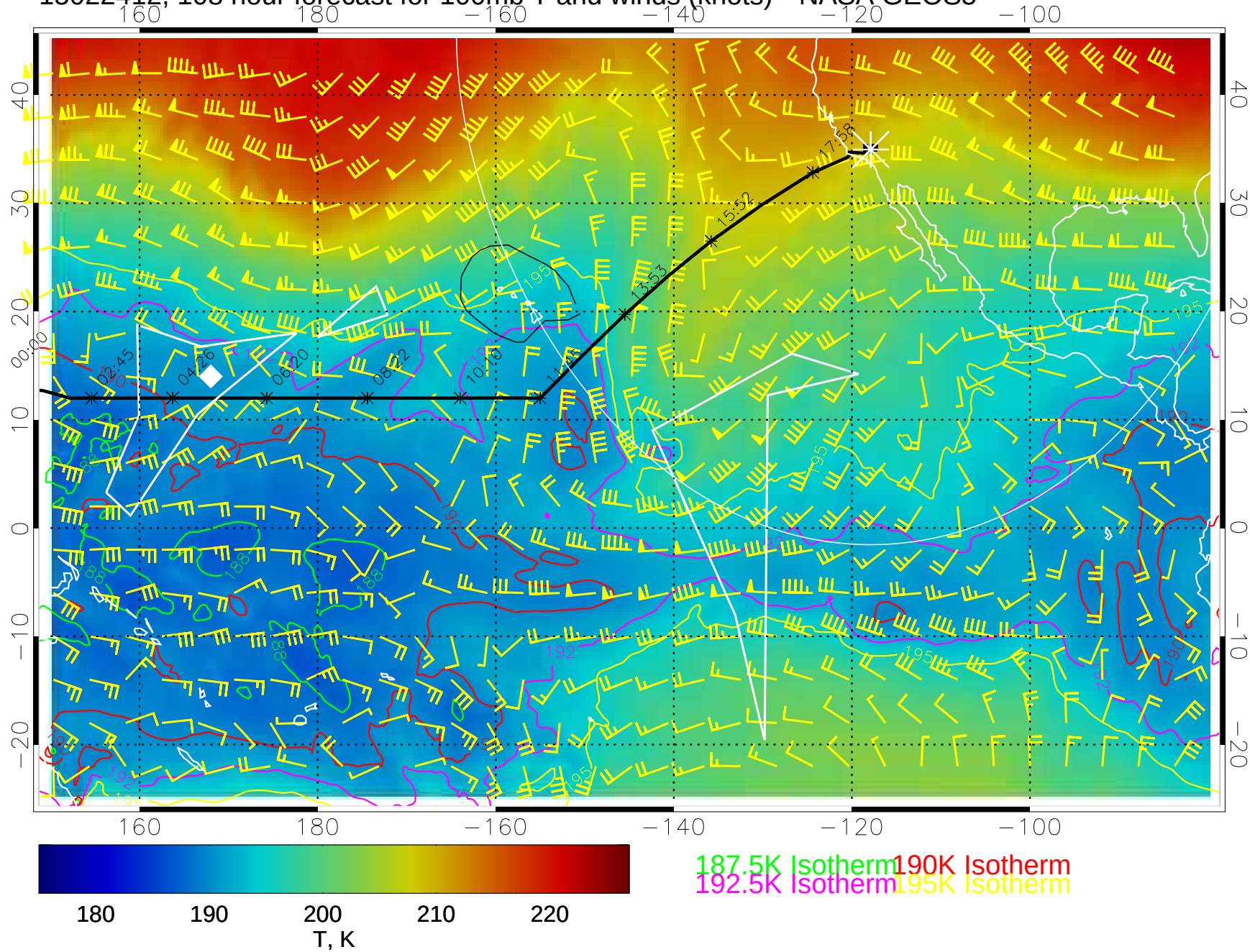
15022412, 108 hour forecast for 100mb T and winds (knots)-- NASA GEOS5
