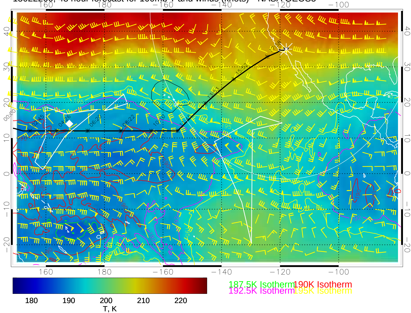
15022200, 48 hour forecast for 100mb T and winds (knots)-- NASA GEOS5
