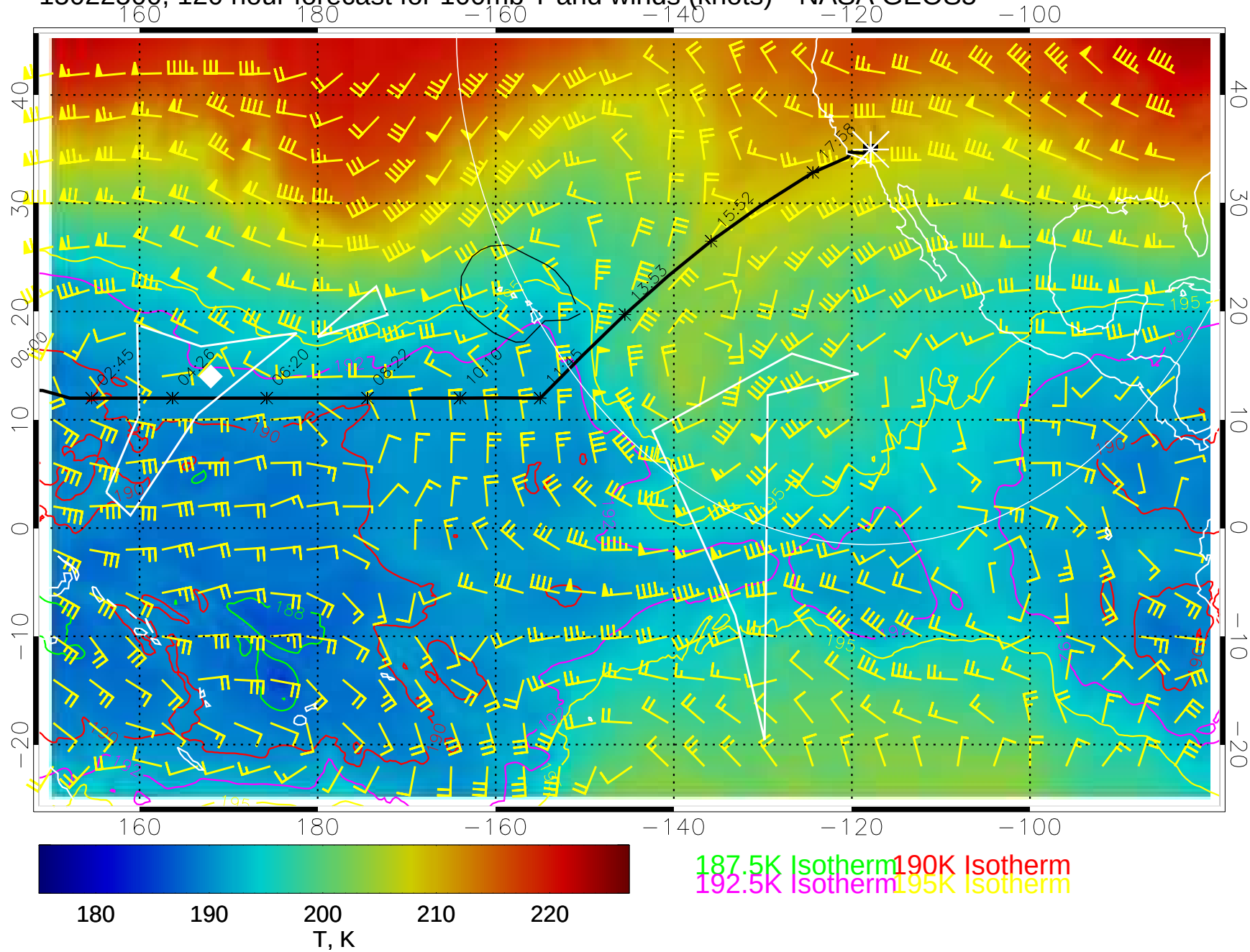
15022500, 120 hour forecast for 100mb T and winds (knots)-- NASA GEOS5
