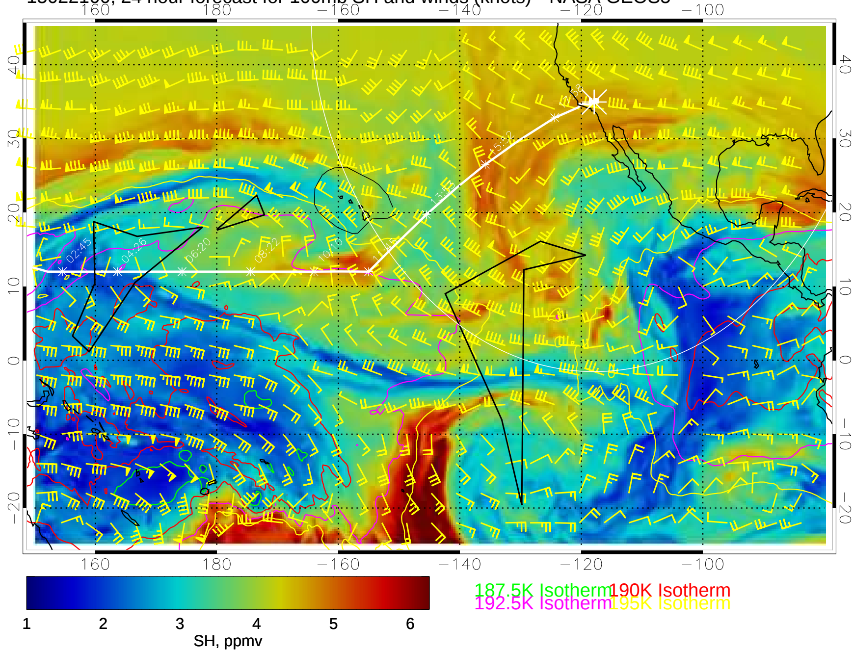
15022100, 24 hour forecast for 100mb SH and winds (knots)-- NASA GEOS5
