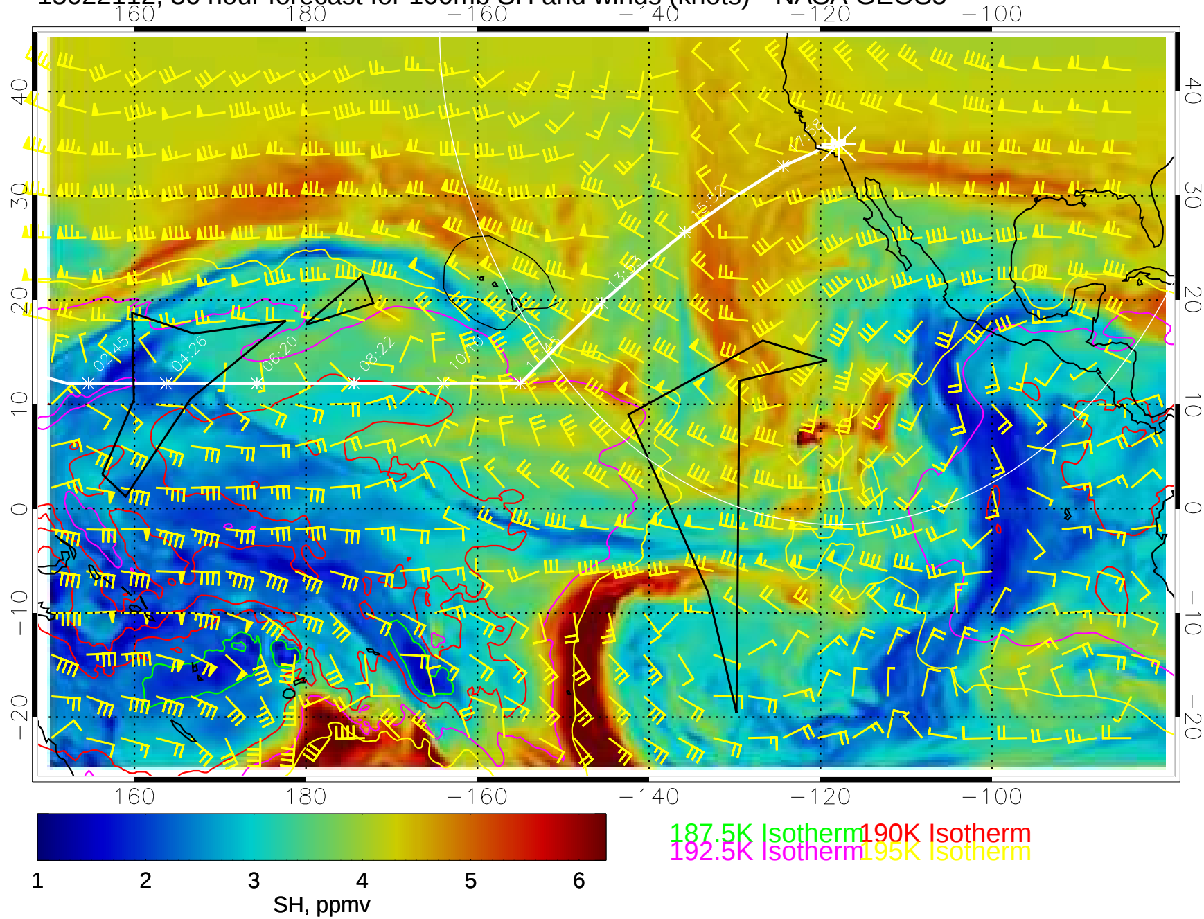
15022112, 36 hour forecast for 100mb SH and winds (knots)-- NASA GEOS5
