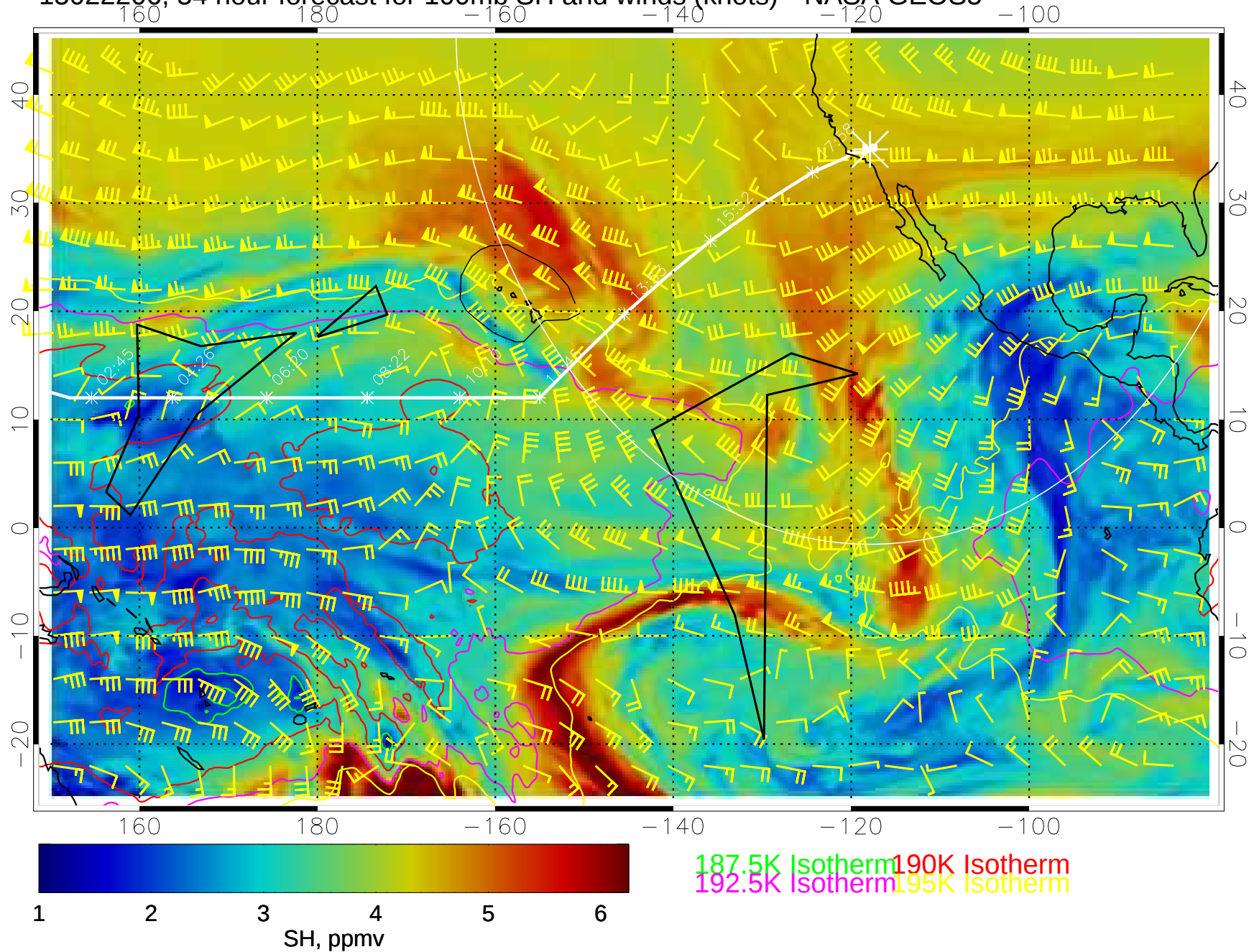
15022206, 54 hour forecast for 100mb SH and winds (knots)-- NASA GEOS5
