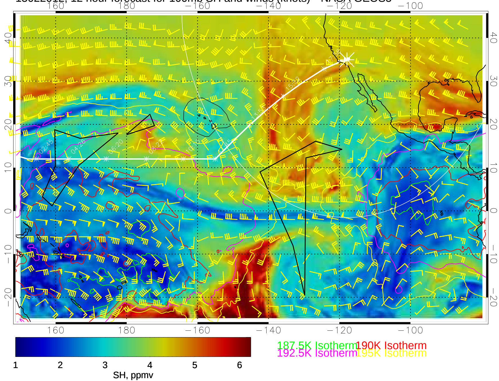
15022012, 12 hour forecast for 100mb SH and winds (knots)-- NASA GEOS5
