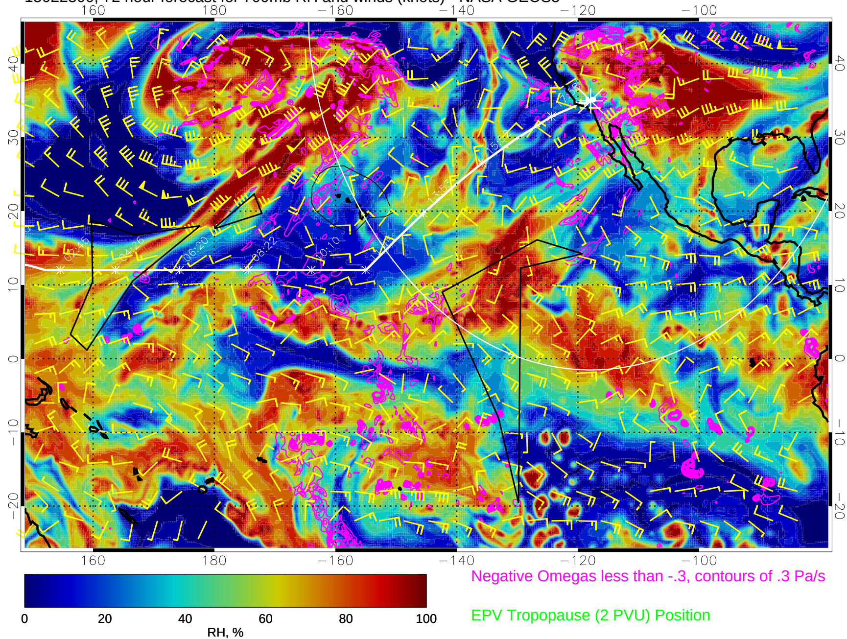
15022300, 72 hour forecast for 700mb RH and winds (knots) - NASA GEOS5
