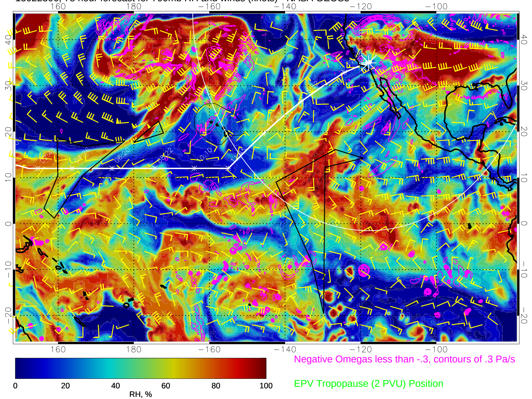
15022306, 78 hour forecast for 700mb RH and winds (knots) - NASA GEOS5
