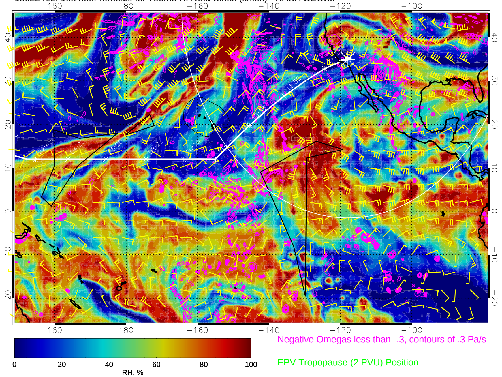
15022412, 108 hour forecast for 700mb RH and winds (knots) - NASA GEOS5
