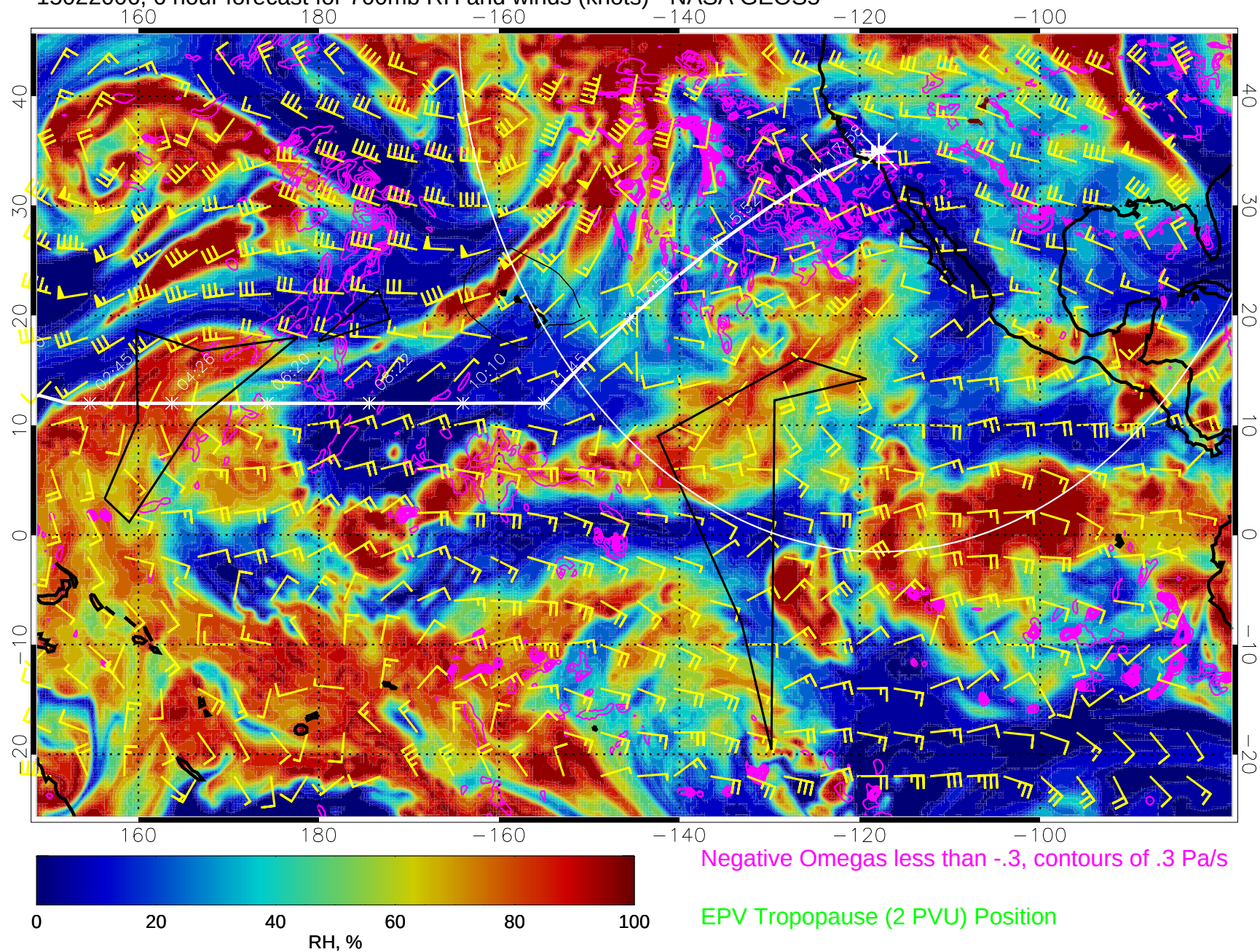
15022006, 6 hour forecast for 700mb RH and winds (knots) - NASA GEOS5
