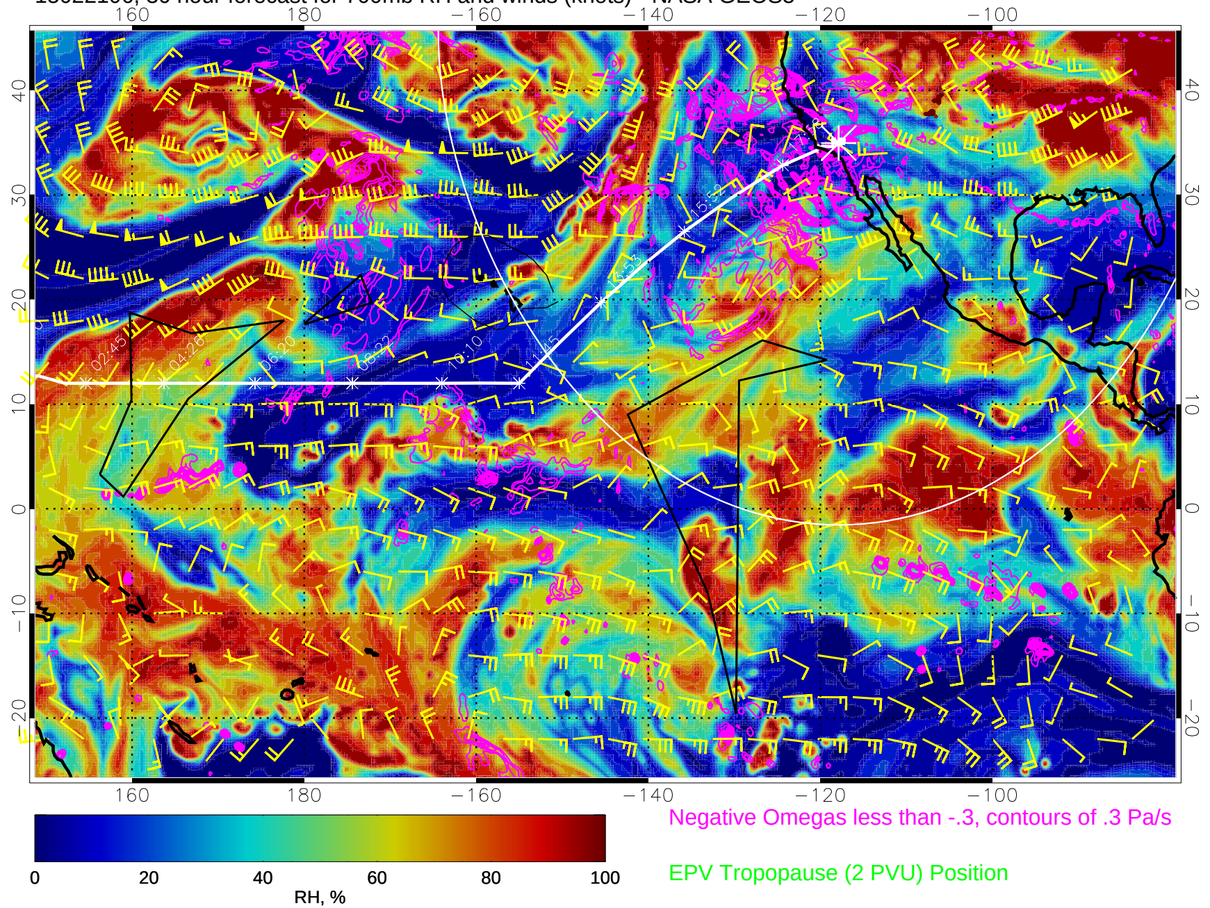
15022106, 30 hour forecast for 700mb RH and winds (knots) - NASA GEOS5
