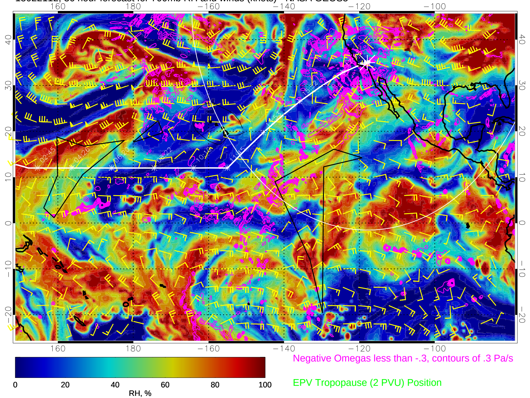
15022112, 36 hour forecast for 700mb RH and winds (knots) - NASA GEOS5
