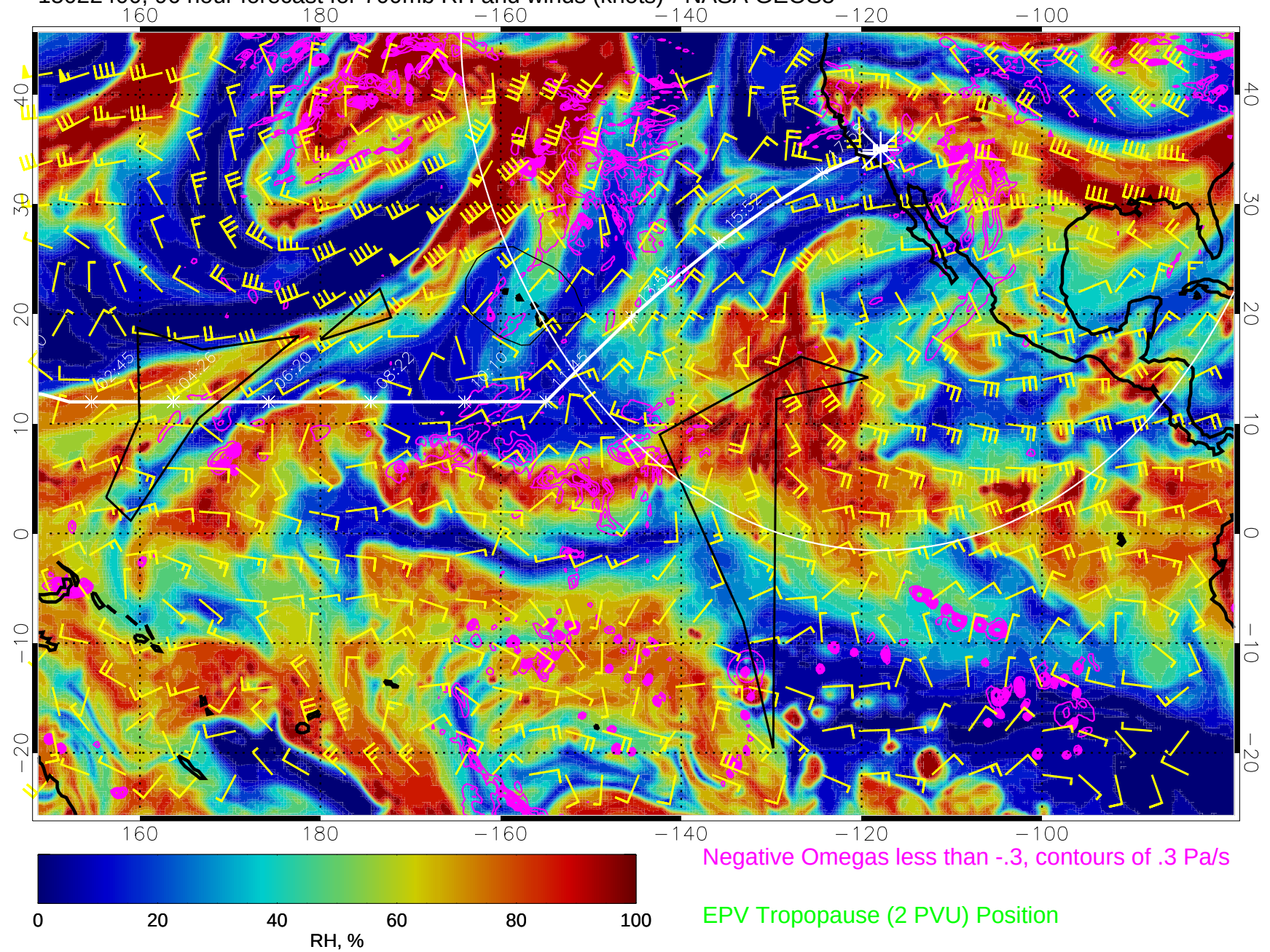
15022400, 96 hour forecast for 700mb RH and winds (knots) - NASA GEOS5
