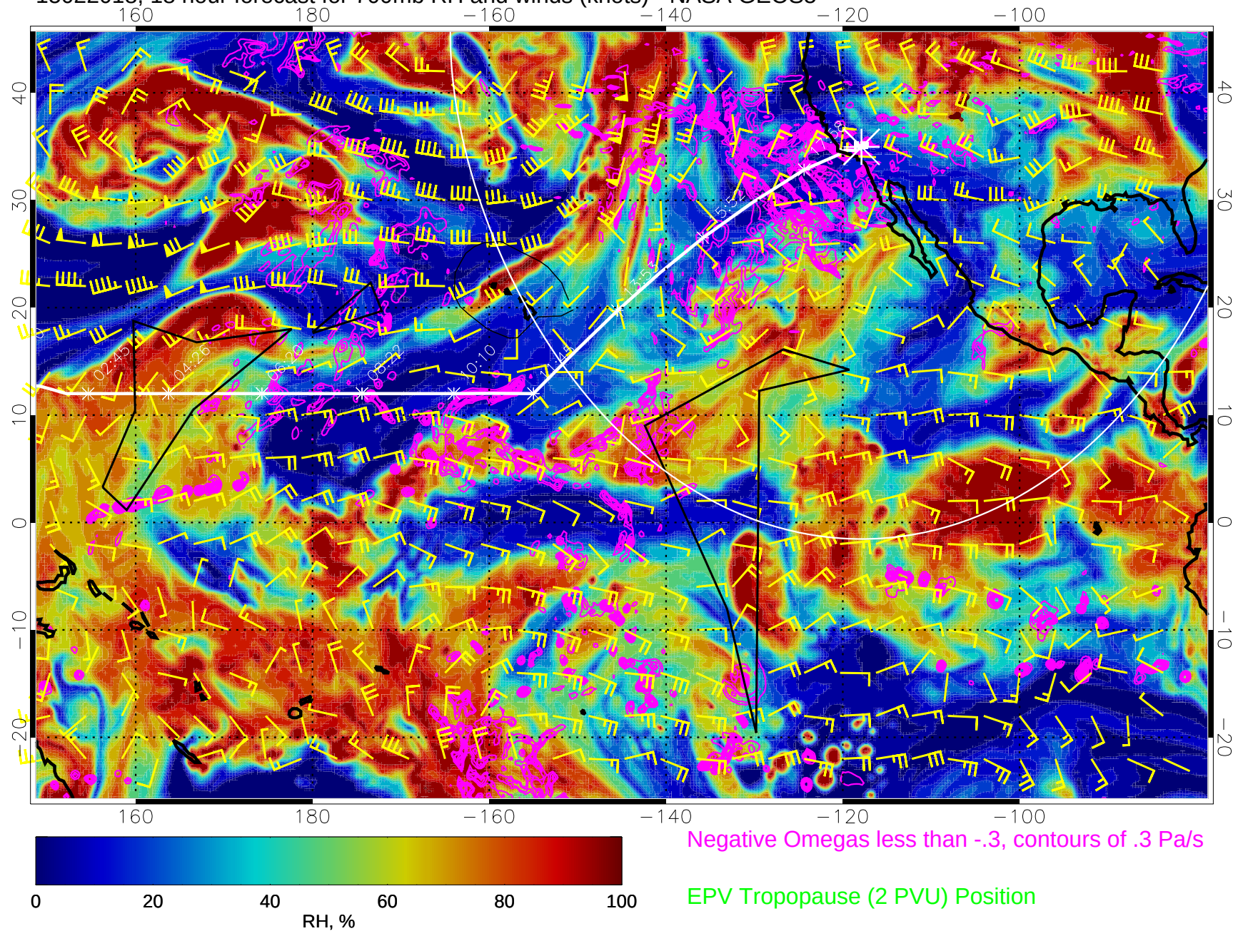
15022018, 18 hour forecast for 700mb RH and winds (knots) - NASA GEOS5
