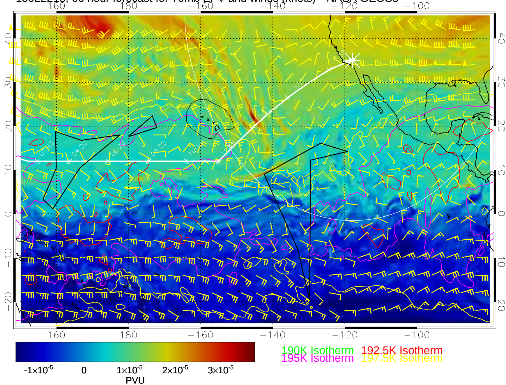
15022218, 66 hour forecast for 70mb EPV and winds (knots)-- NASA GEOS5
