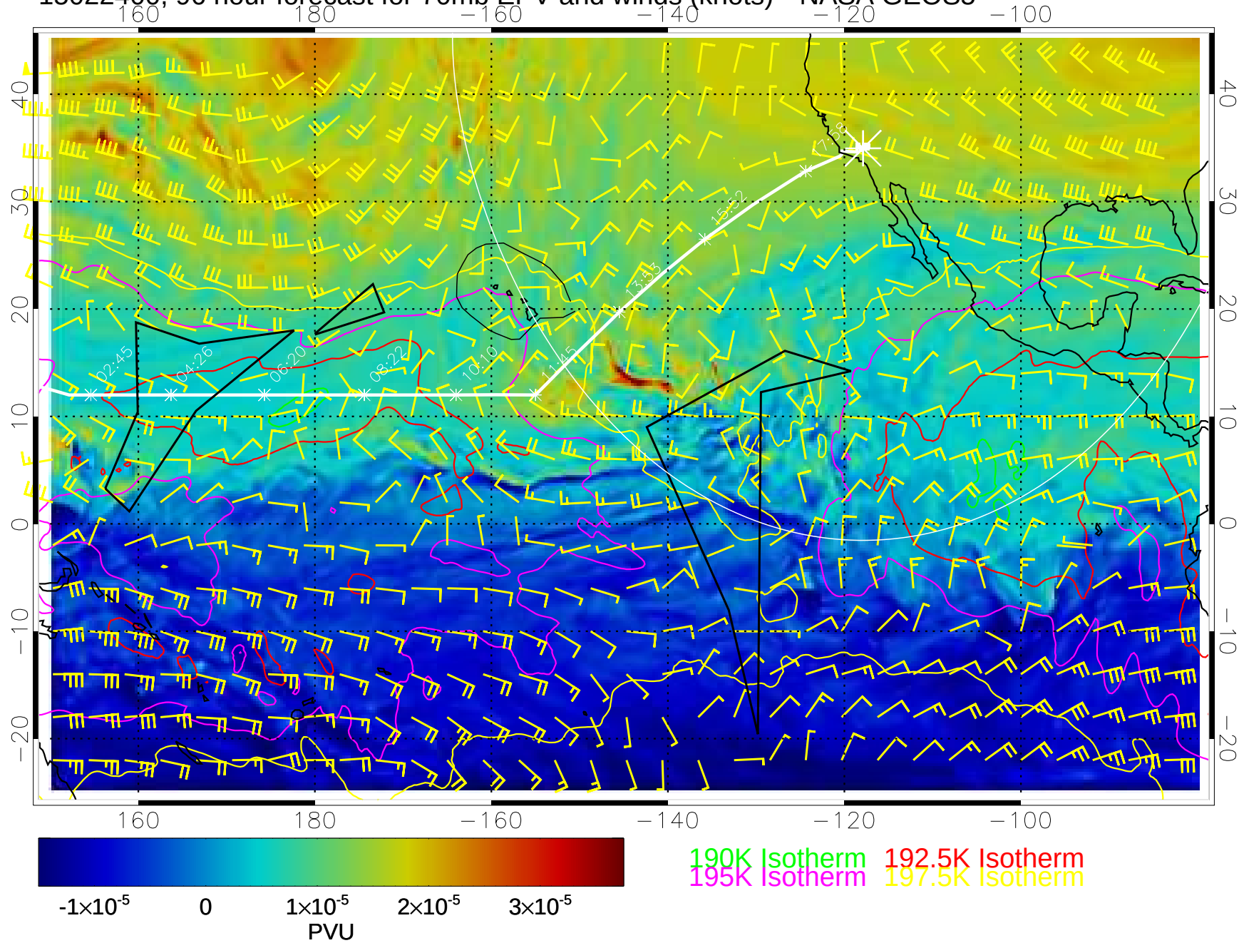
15022400, 96 hour forecast for 70mb EPV and winds (knots)-- NASA GEOS5
