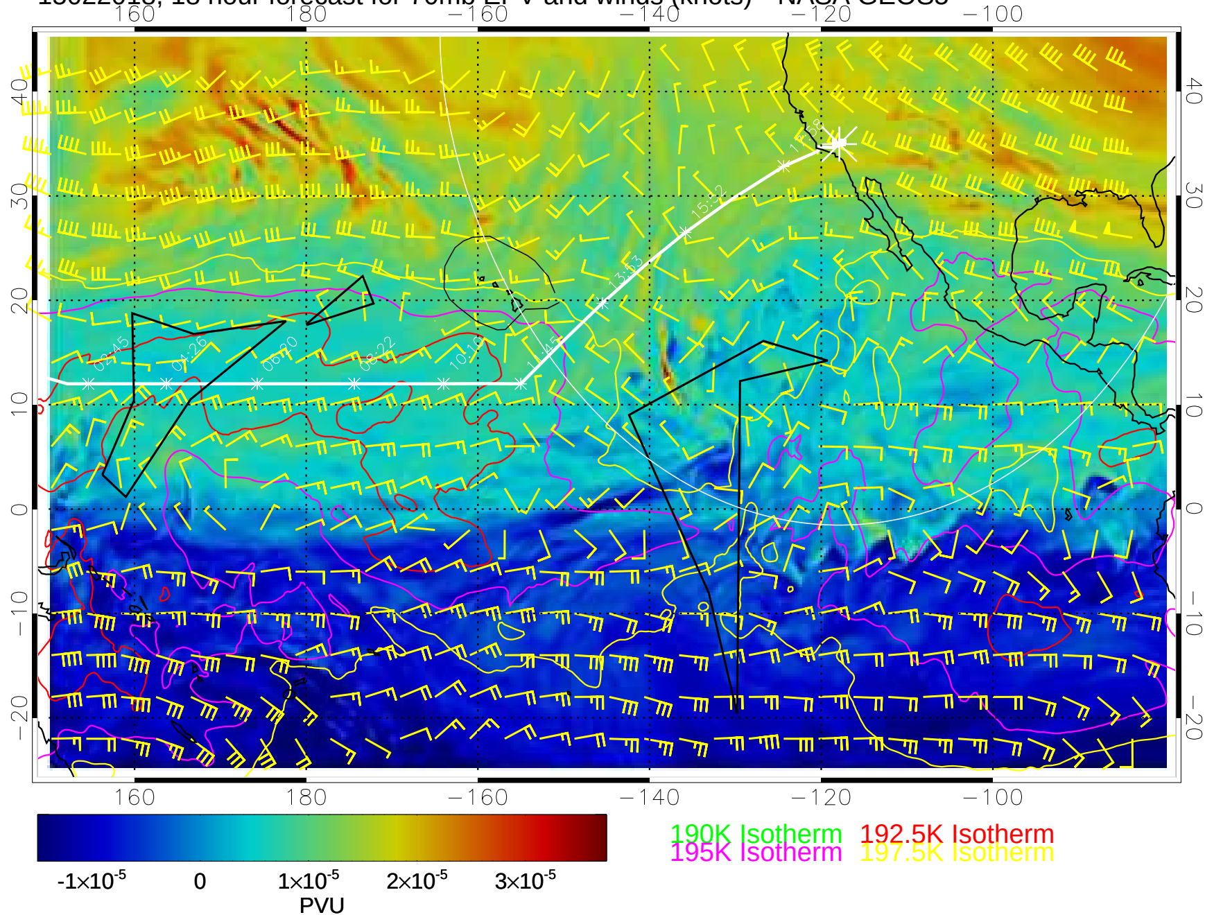
15022018, 18 hour forecast for 70mb EPV and winds (knots)-- NASA GEOS5
