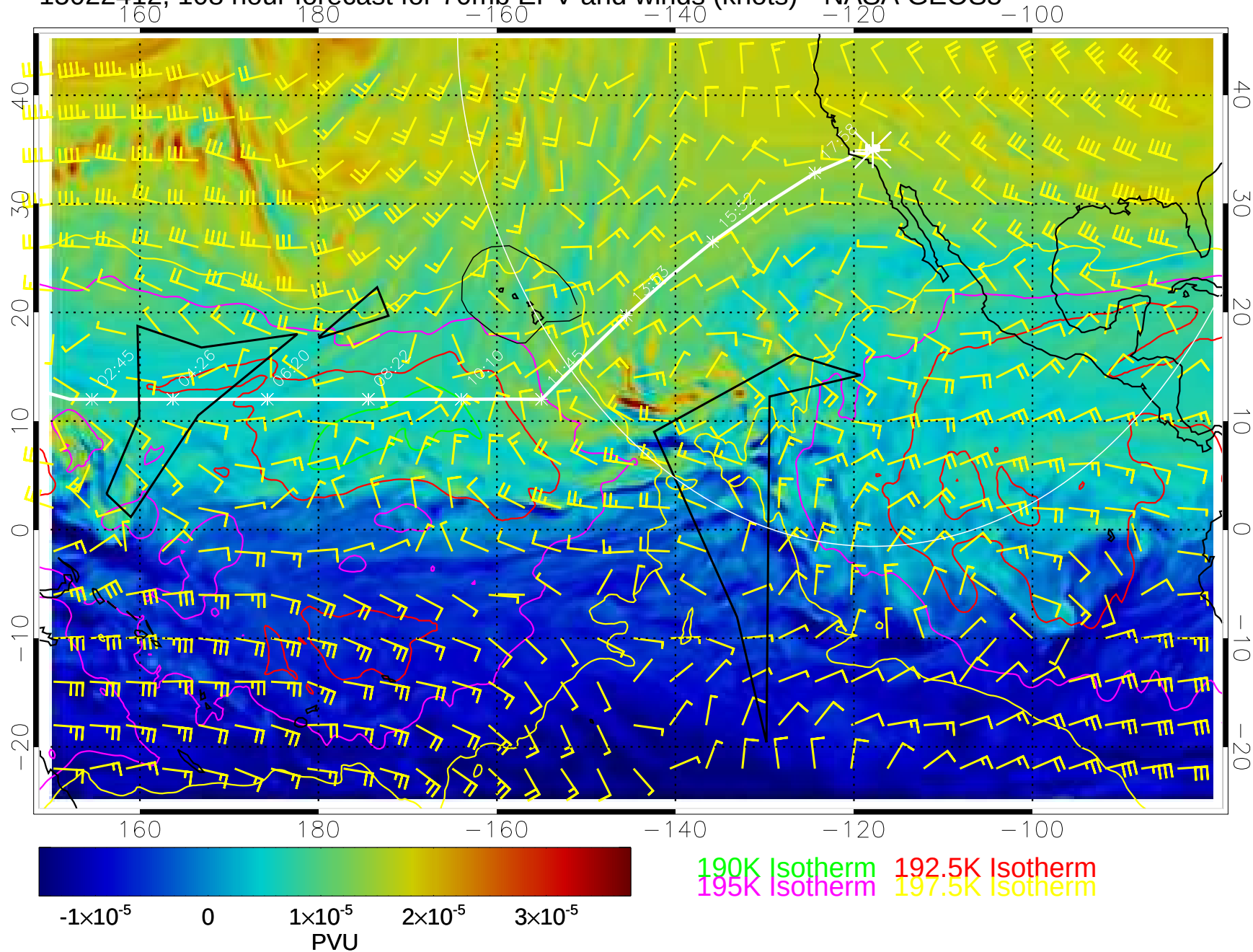
15022412, 108 hour forecast for 70mb EPV and winds (knots)-- NASA GEOS5
