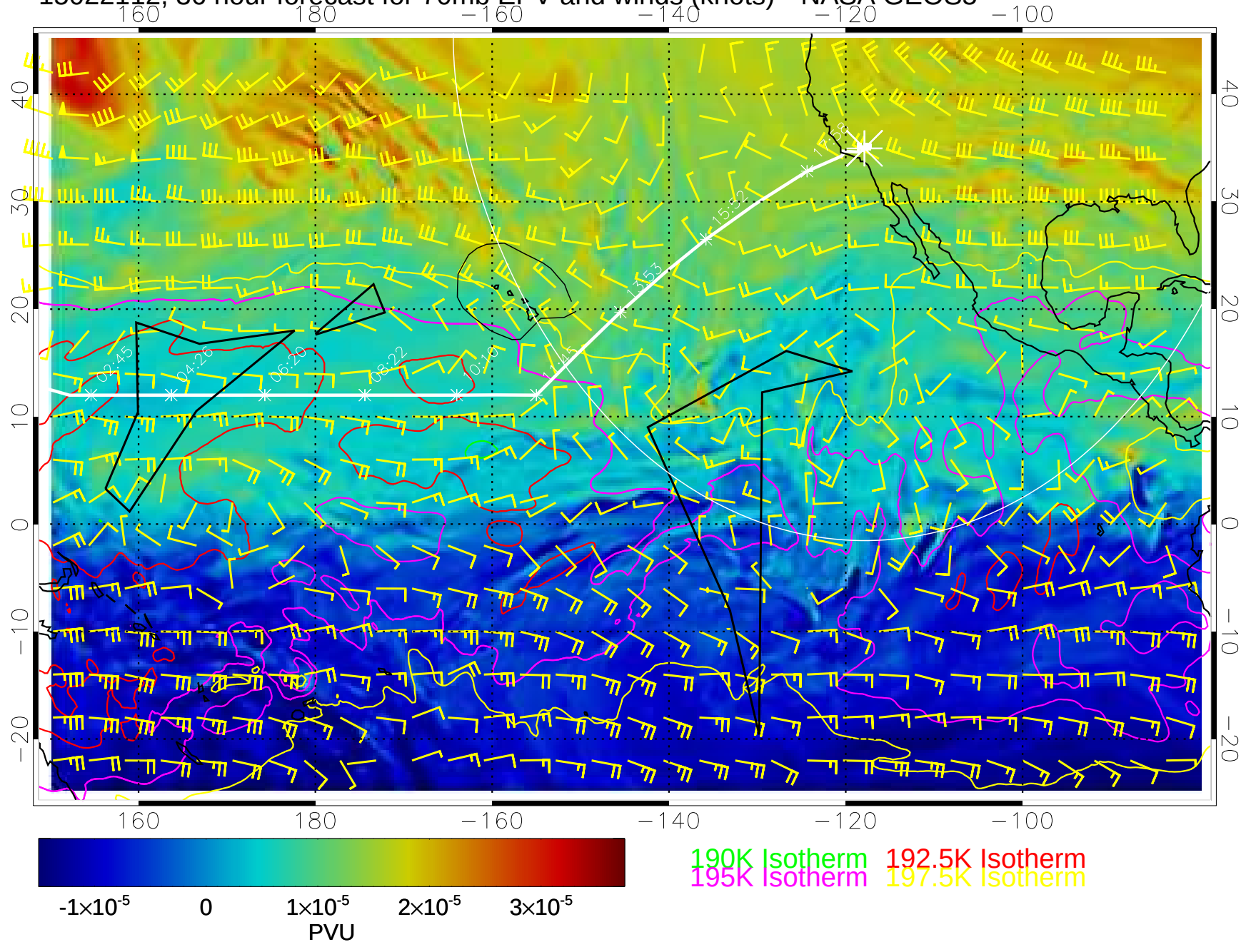
15022112, 36 hour forecast for 70mb EPV and winds (knots)-- NASA GEOS5
