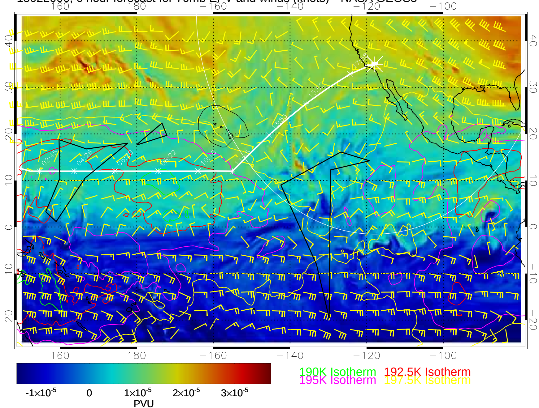
15022006, 6 hour forecast for 70mb EPV and winds (knots)-- NASA GEOS5
