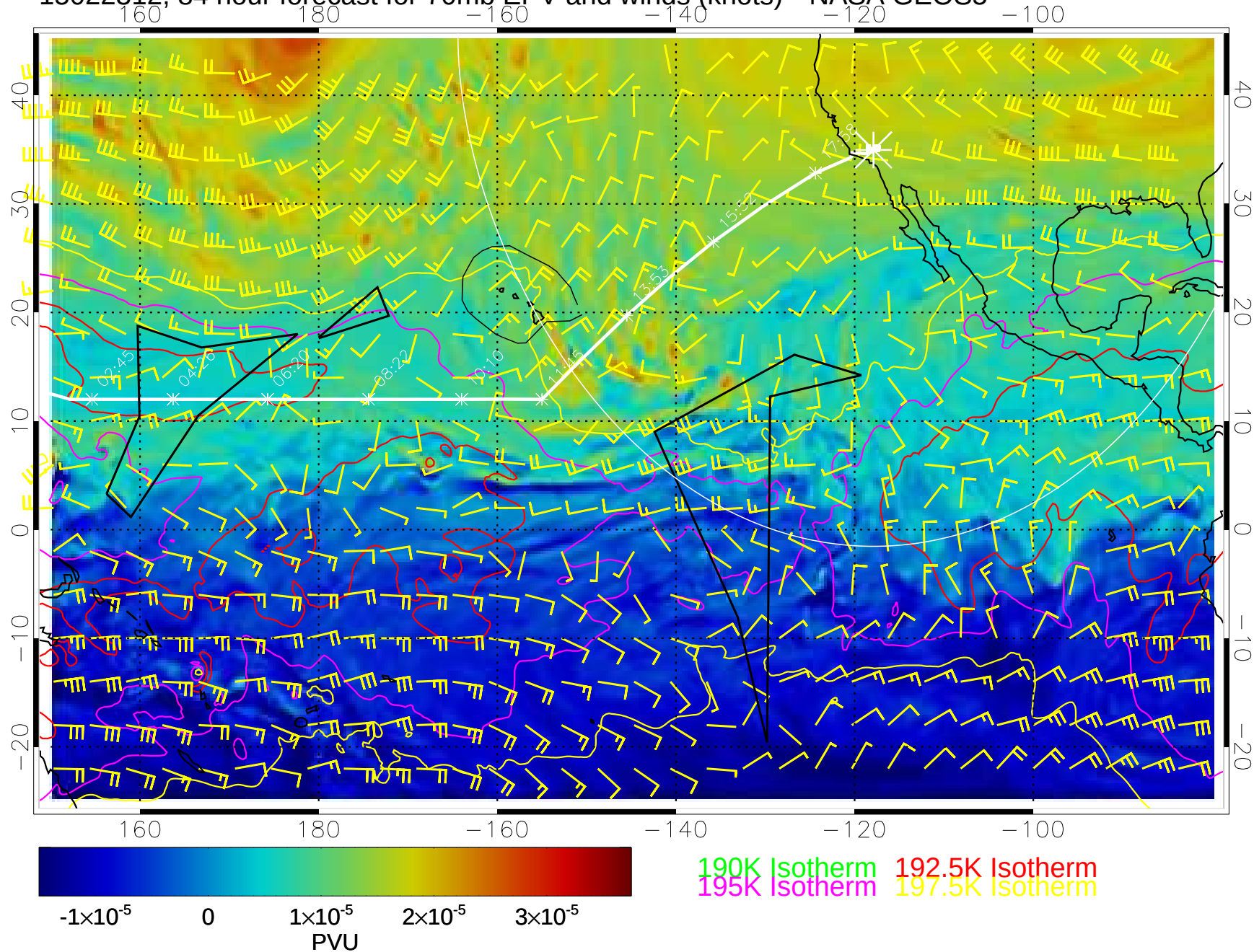
15022312, 84 hour forecast for 70mb EPV and winds (knots)-- NASA GEOS5
