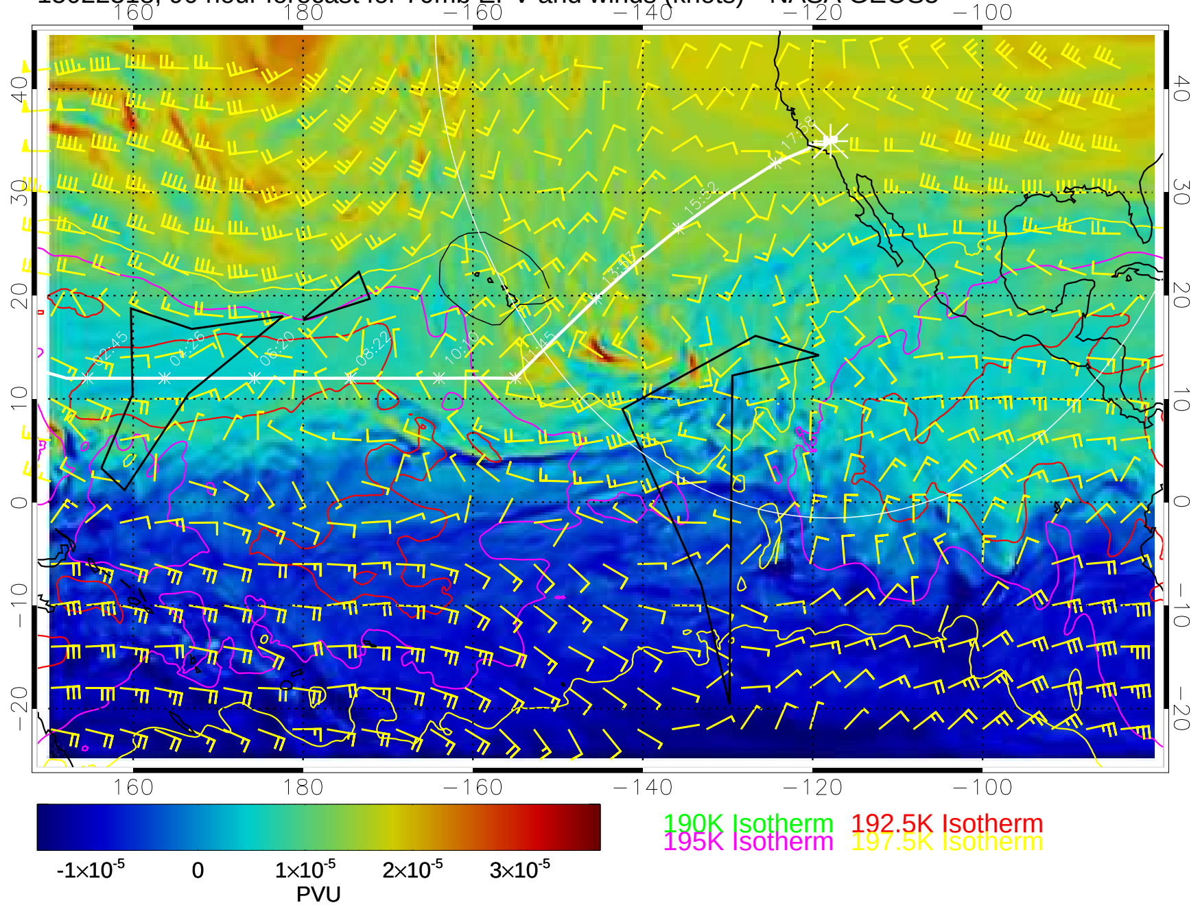
15022318, 90 hour forecast for 70mb EPV and winds (knots)-- NASA GEOS5
