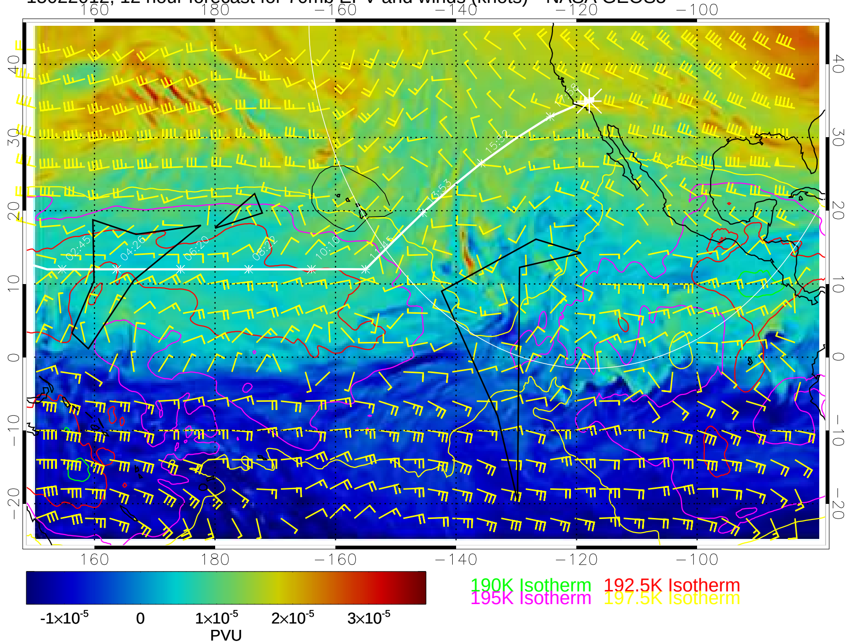
15022012, 12 hour forecast for 70mb EPV and winds (knots)-- NASA GEOS5
