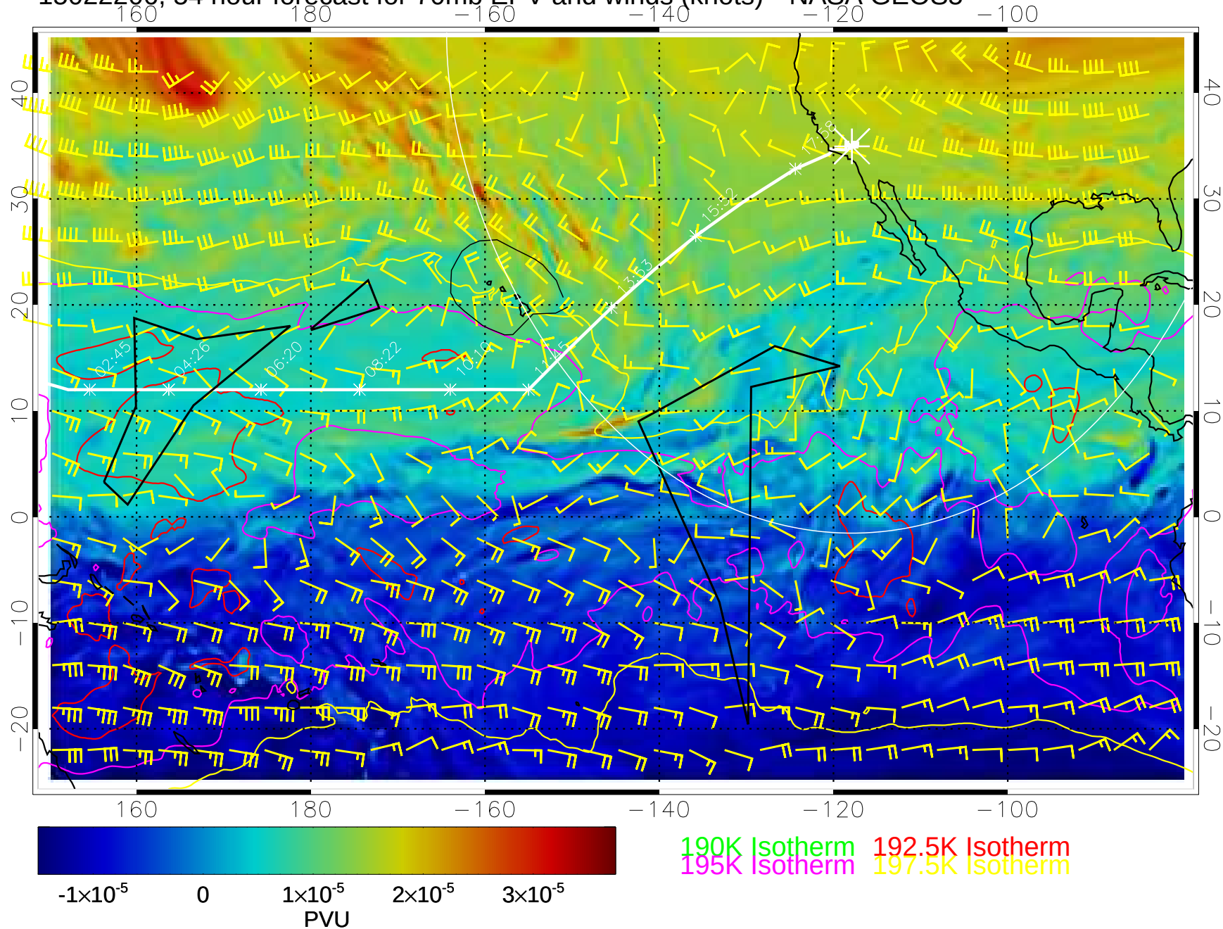
15022206, 54 hour forecast for 70mb EPV and winds (knots)-- NASA GEOS5
