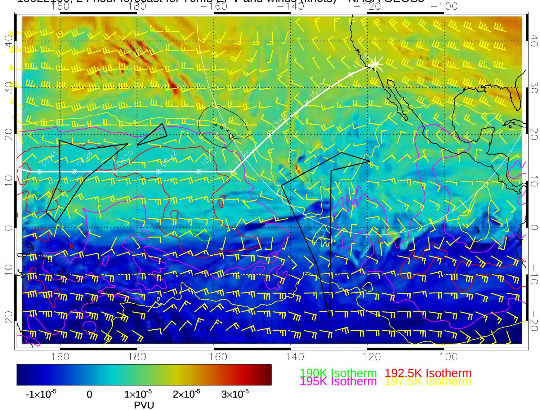
15022100, 24 hour forecast for 70mb EPV and winds (knots)-- NASA GEOS5
