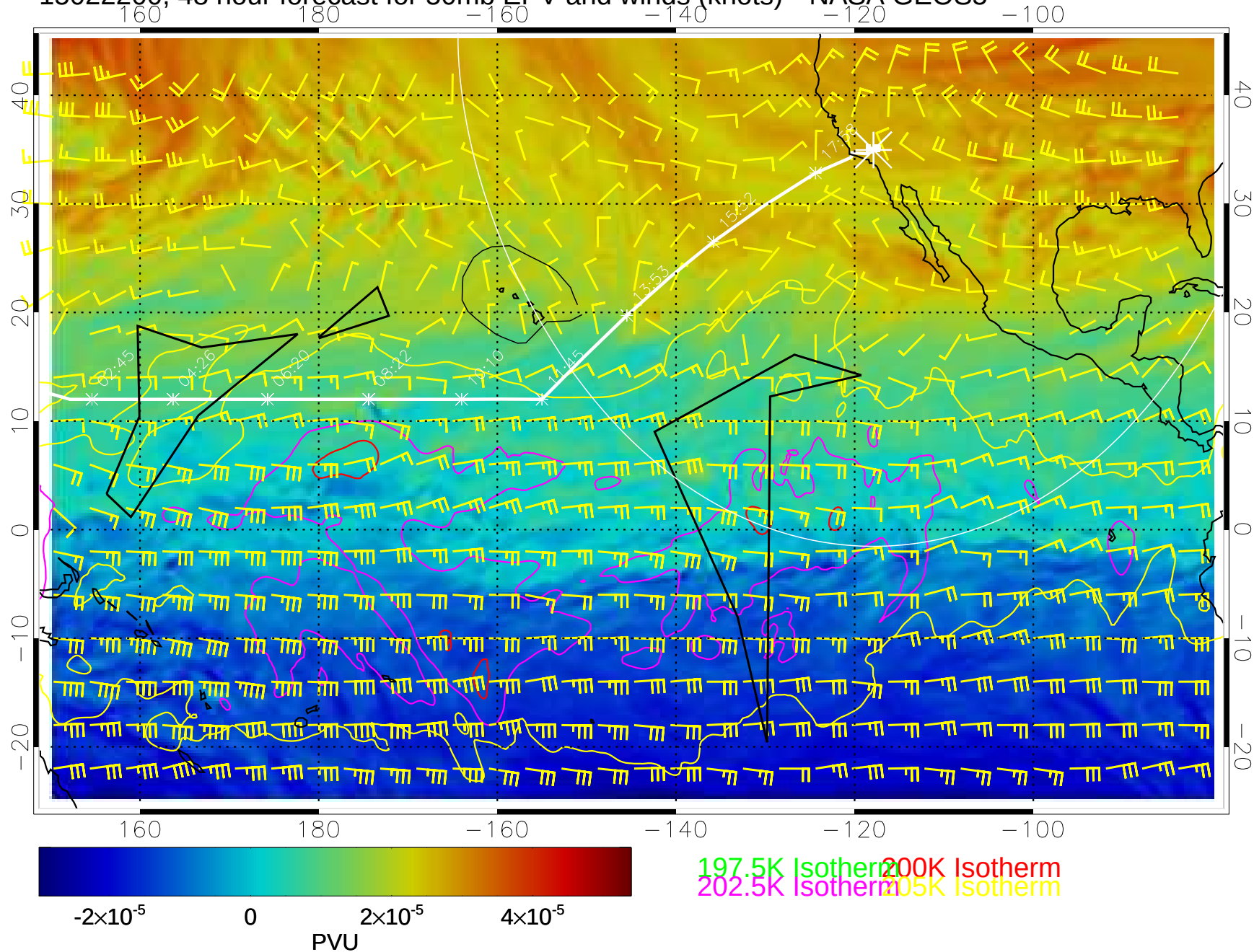
15022200, 48 hour forecast for 50mb EPV and winds (knots)-- NASA GEOS5
