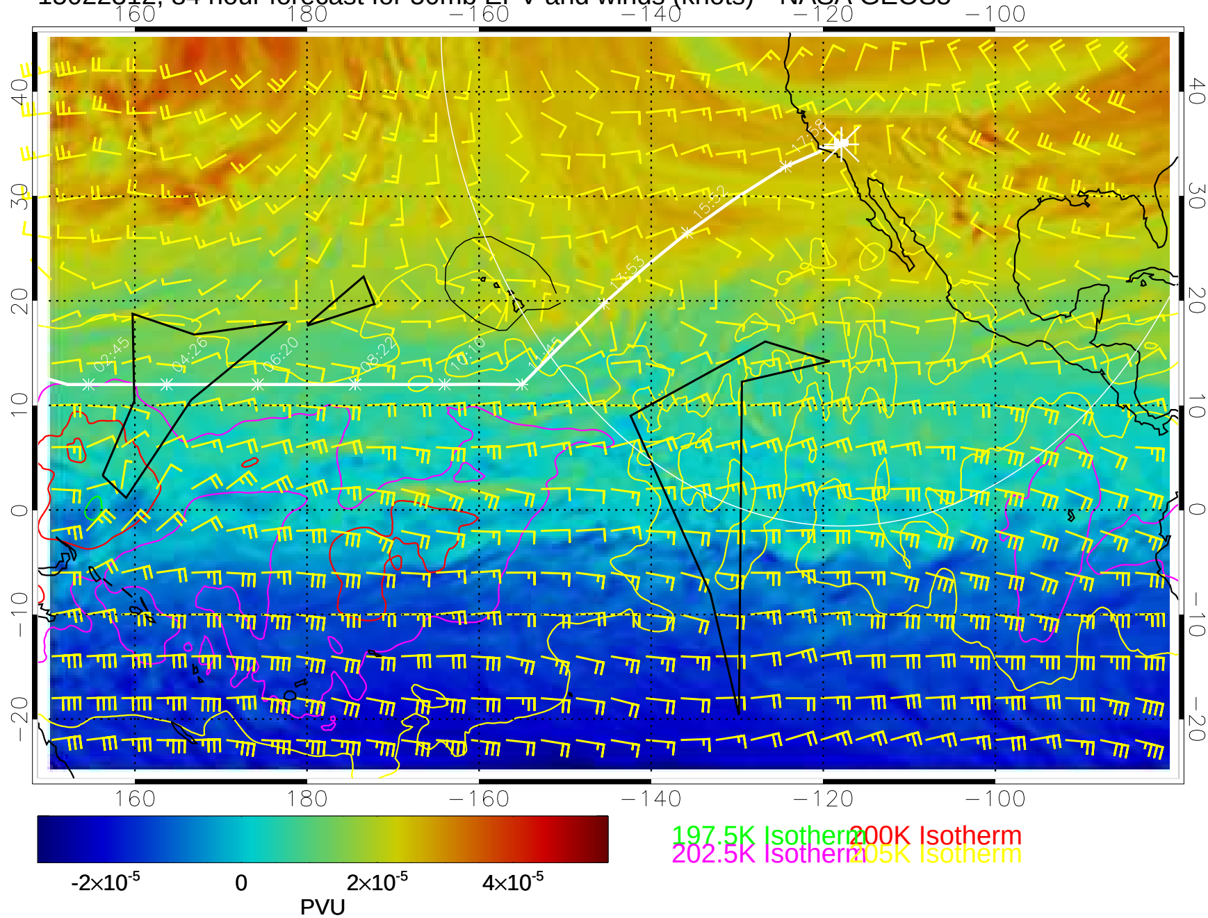
15022312, 84 hour forecast for 50mb EPV and winds (knots)-- NASA GEOS5
