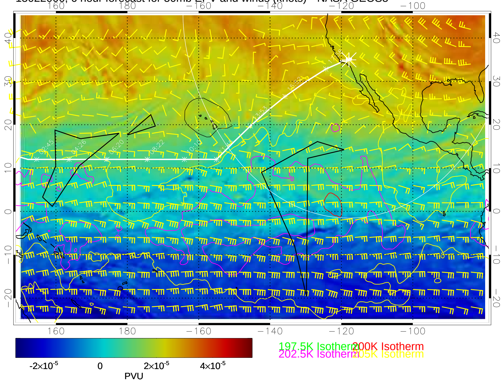
15022006, 6 hour forecast for 50mb EPV and winds (knots)-- NASA GEOS5
