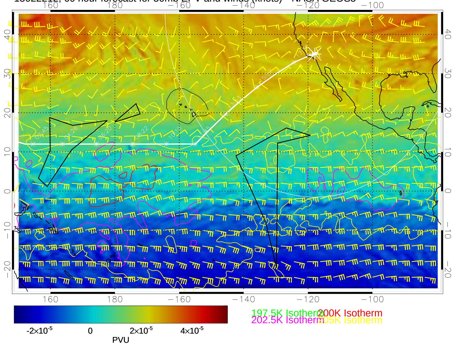
15022212, 60 hour forecast for 50mb EPV and winds (knots)-- NASA GEOS5
