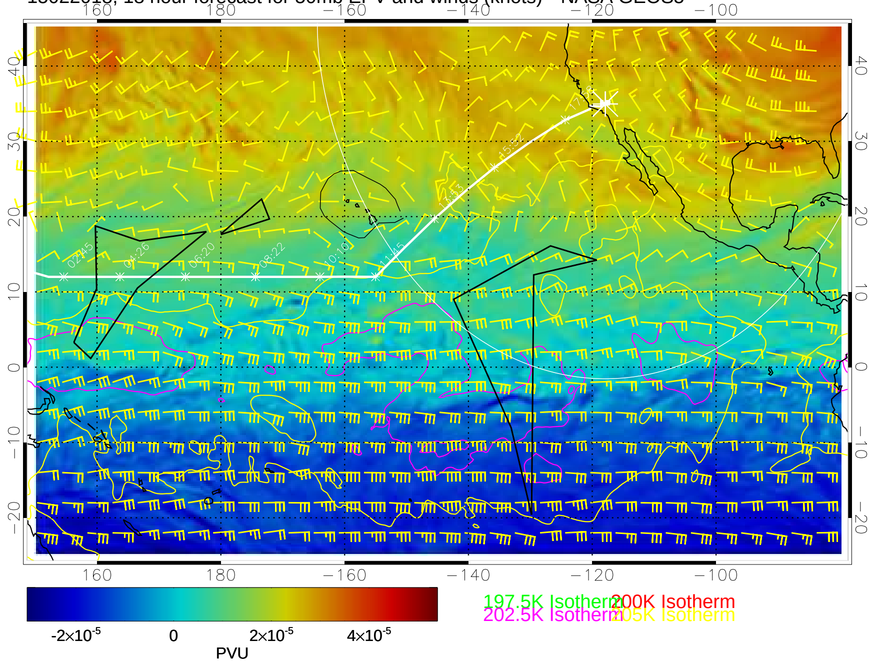
15022018, 18 hour forecast for 50mb EPV and winds (knots)-- NASA GEOS5
