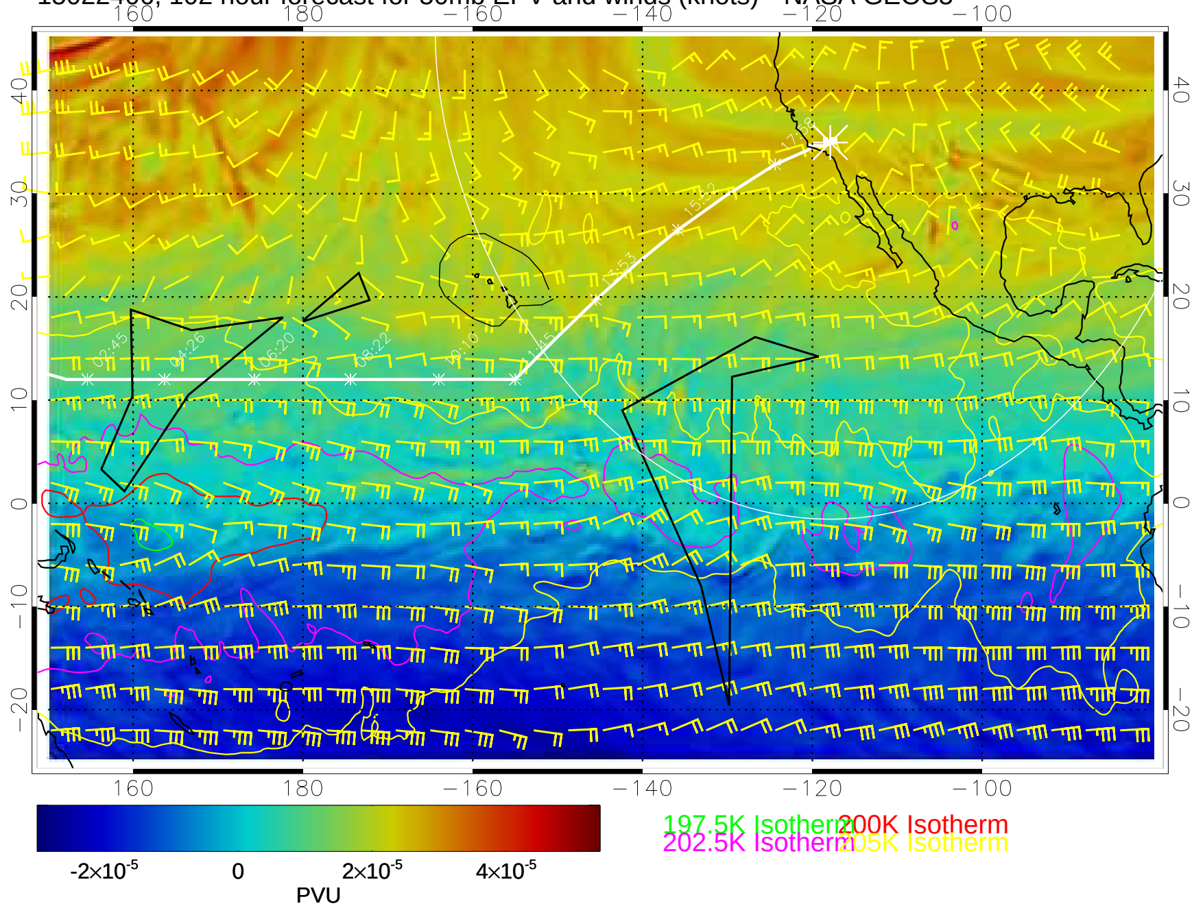
15022406, 102 hour forecast for 50mb EPV and winds (knots)-- NASA GEOS5
