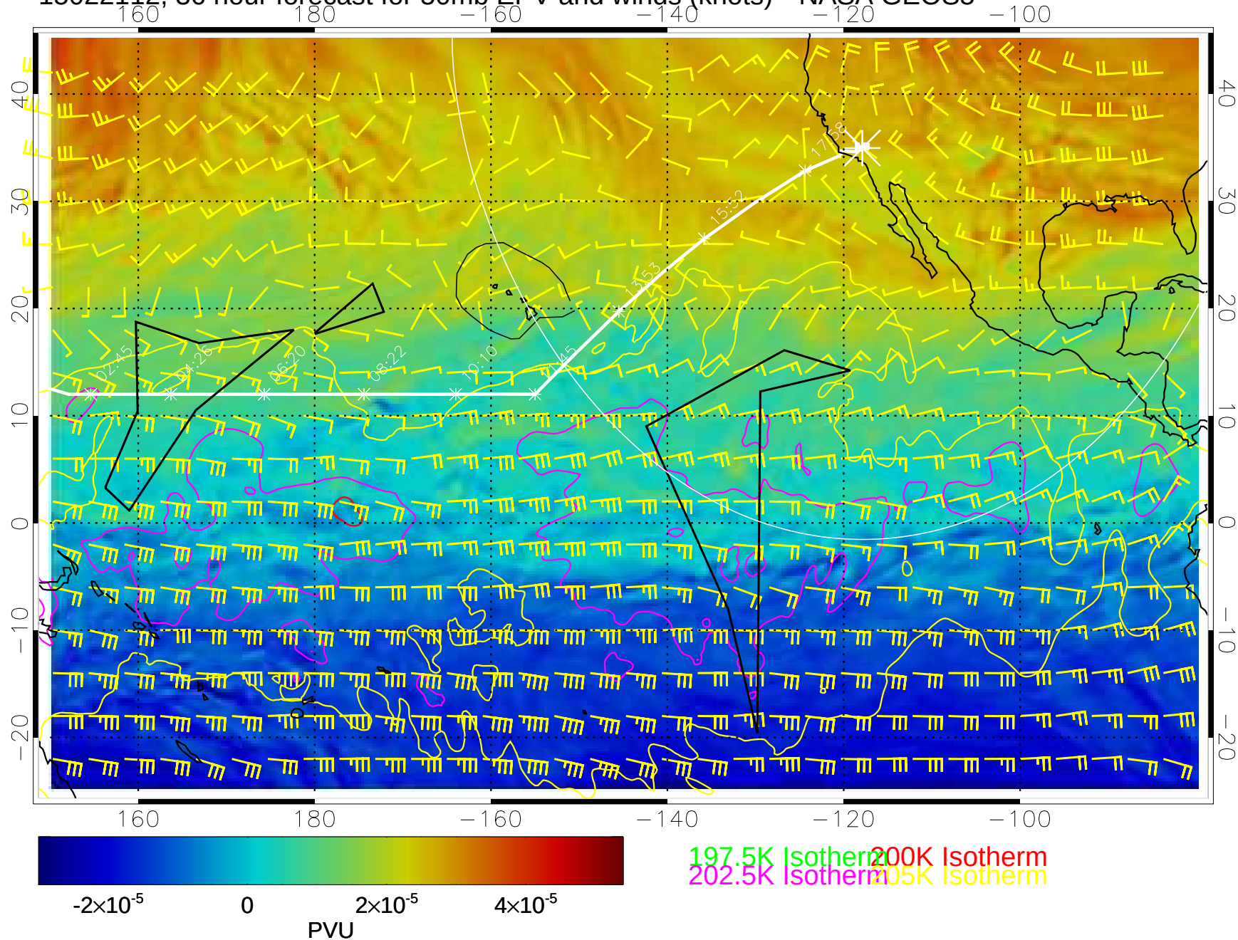
15022112, 36 hour forecast for 50mb EPV and winds (knots)-- NASA GEOS5
