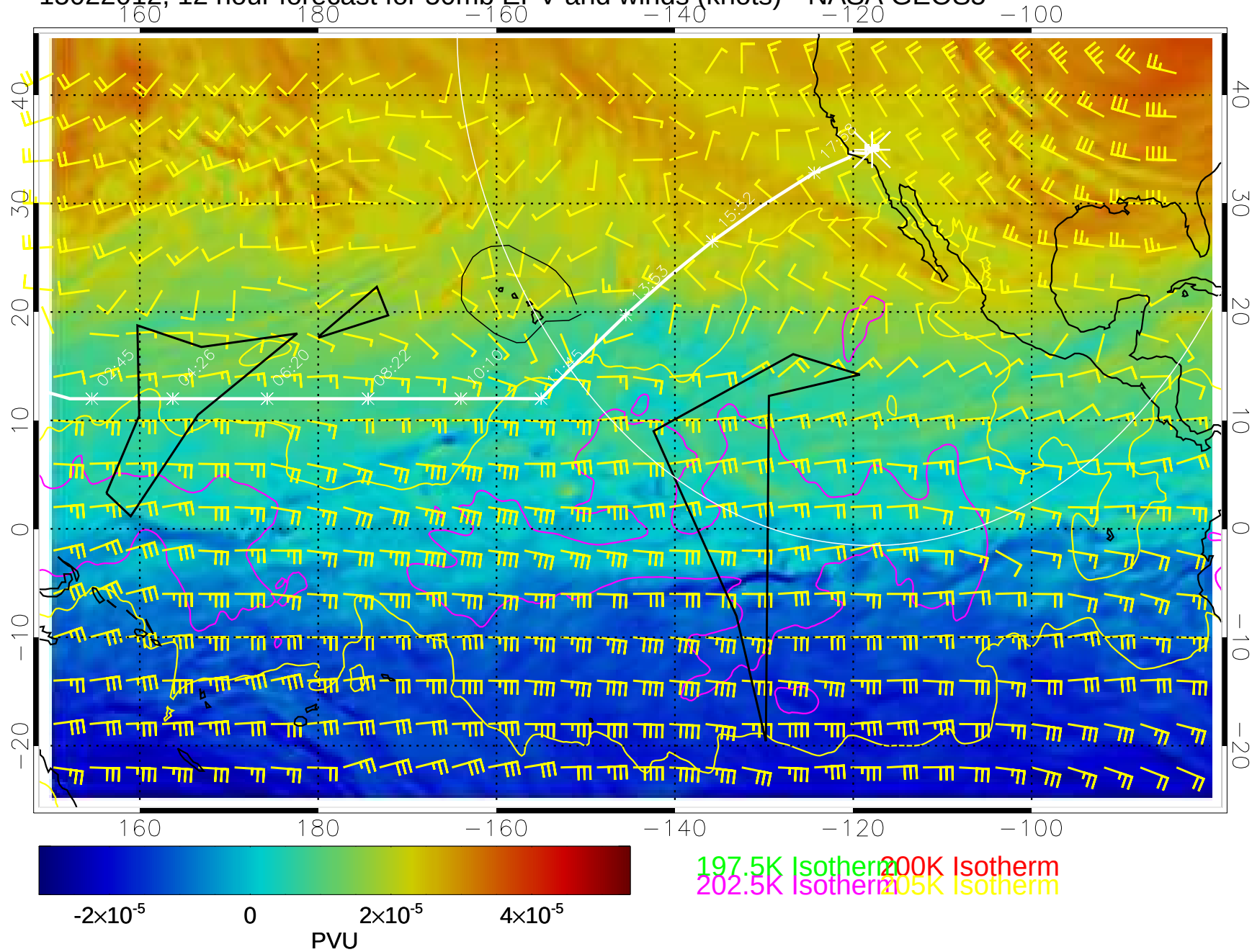
15022012, 12 hour forecast for 50mb EPV and winds (knots)-- NASA GEOS5
