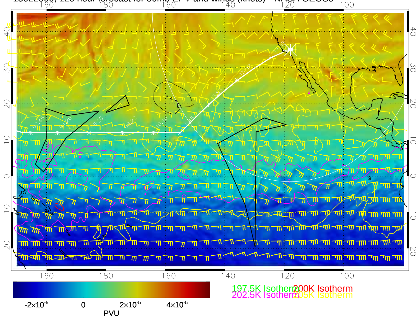
15022500, 120 hour forecast for 50mb EPV and winds (knots)-- NASA GEOS5
