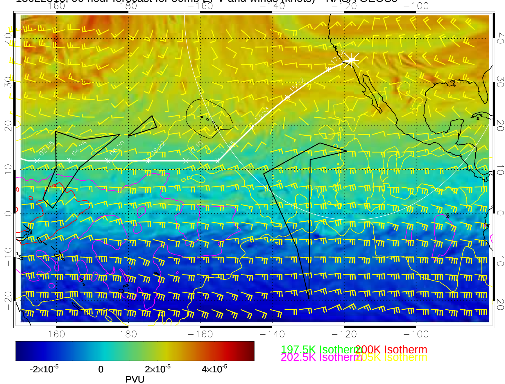
15022318, 90 hour forecast for 50mb EPV and winds (knots)-- NASA GEOS5
