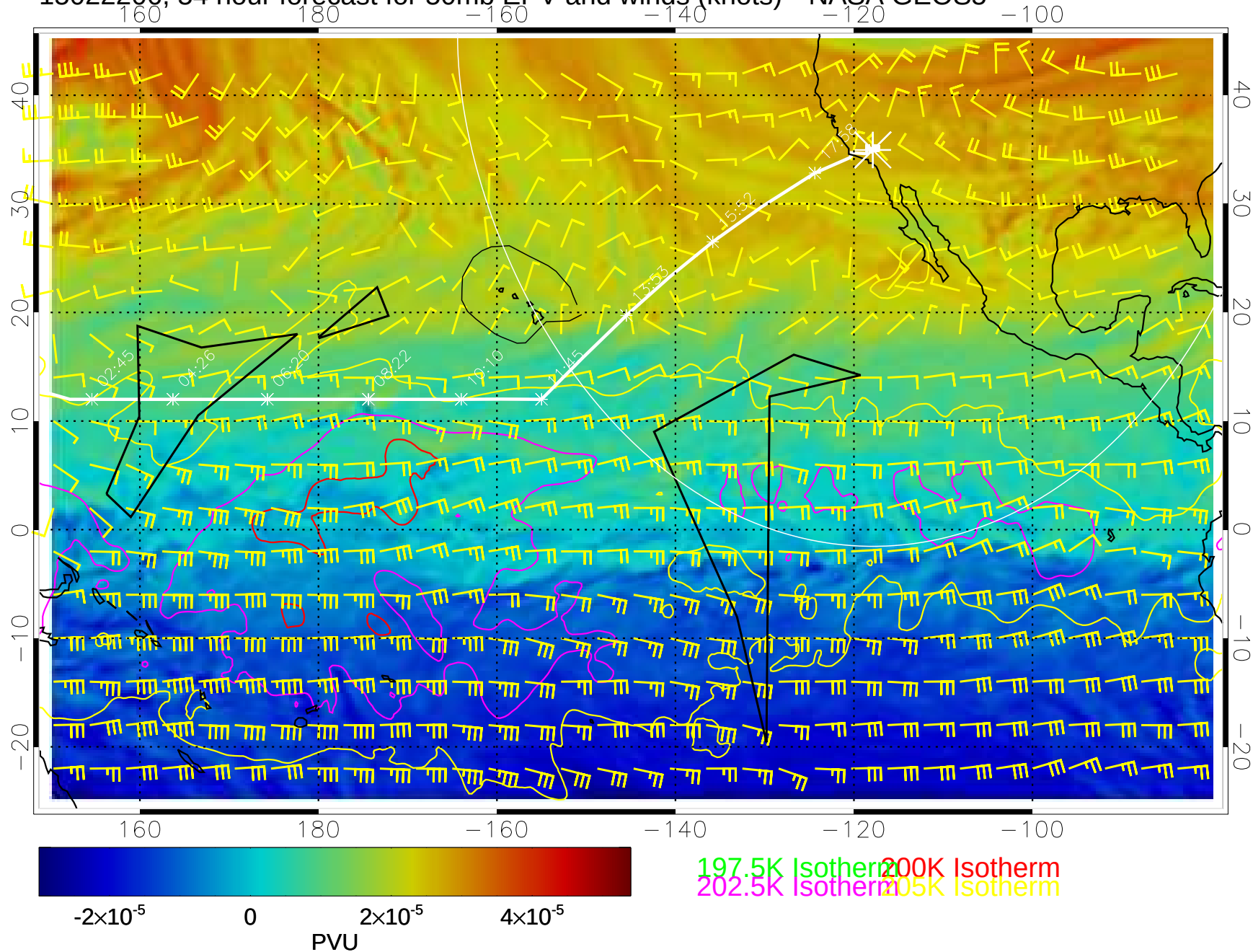
15022206, 54 hour forecast for 50mb EPV and winds (knots)-- NASA GEOS5
