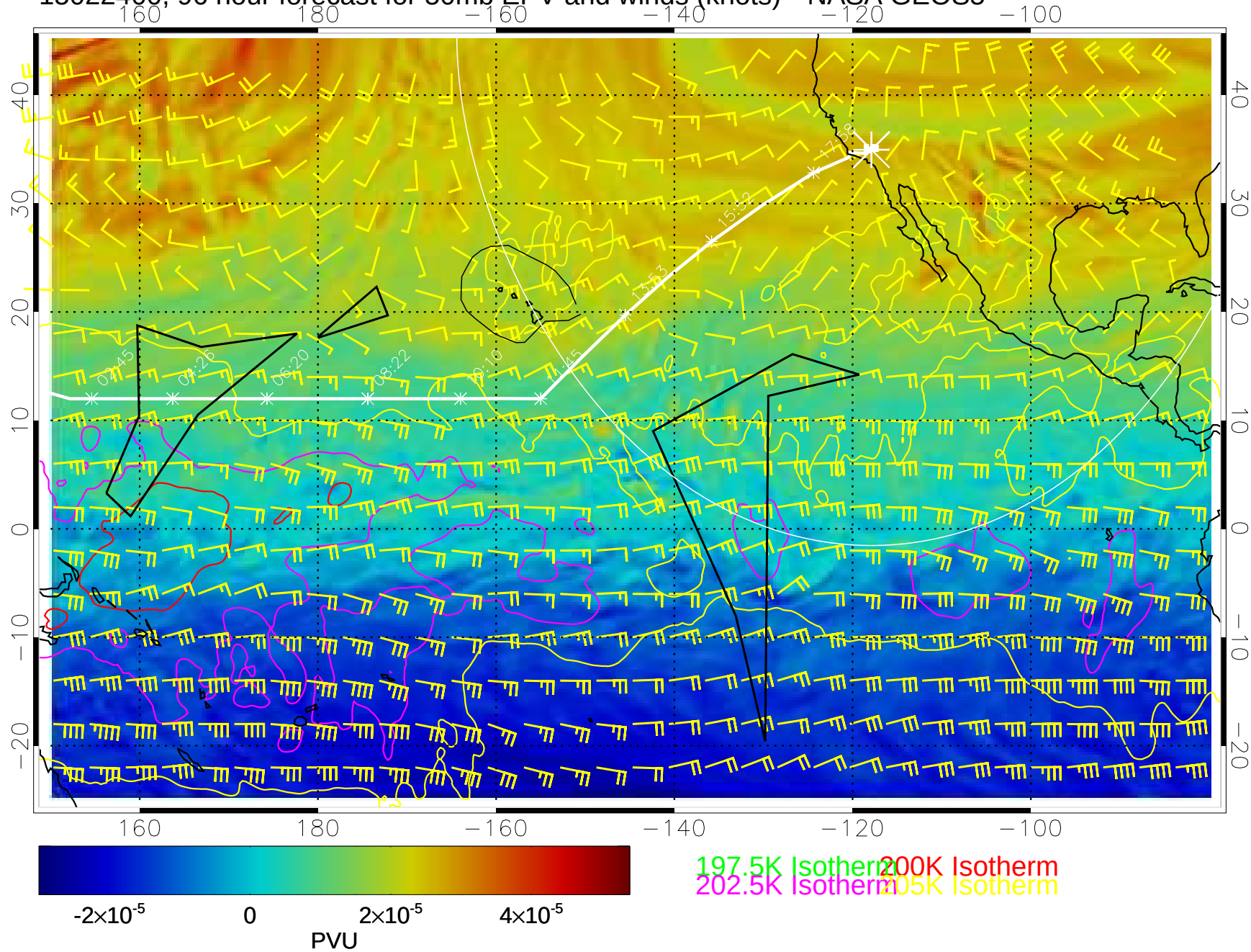
15022400, 96 hour forecast for 50mb EPV and winds (knots)-- NASA GEOS5
