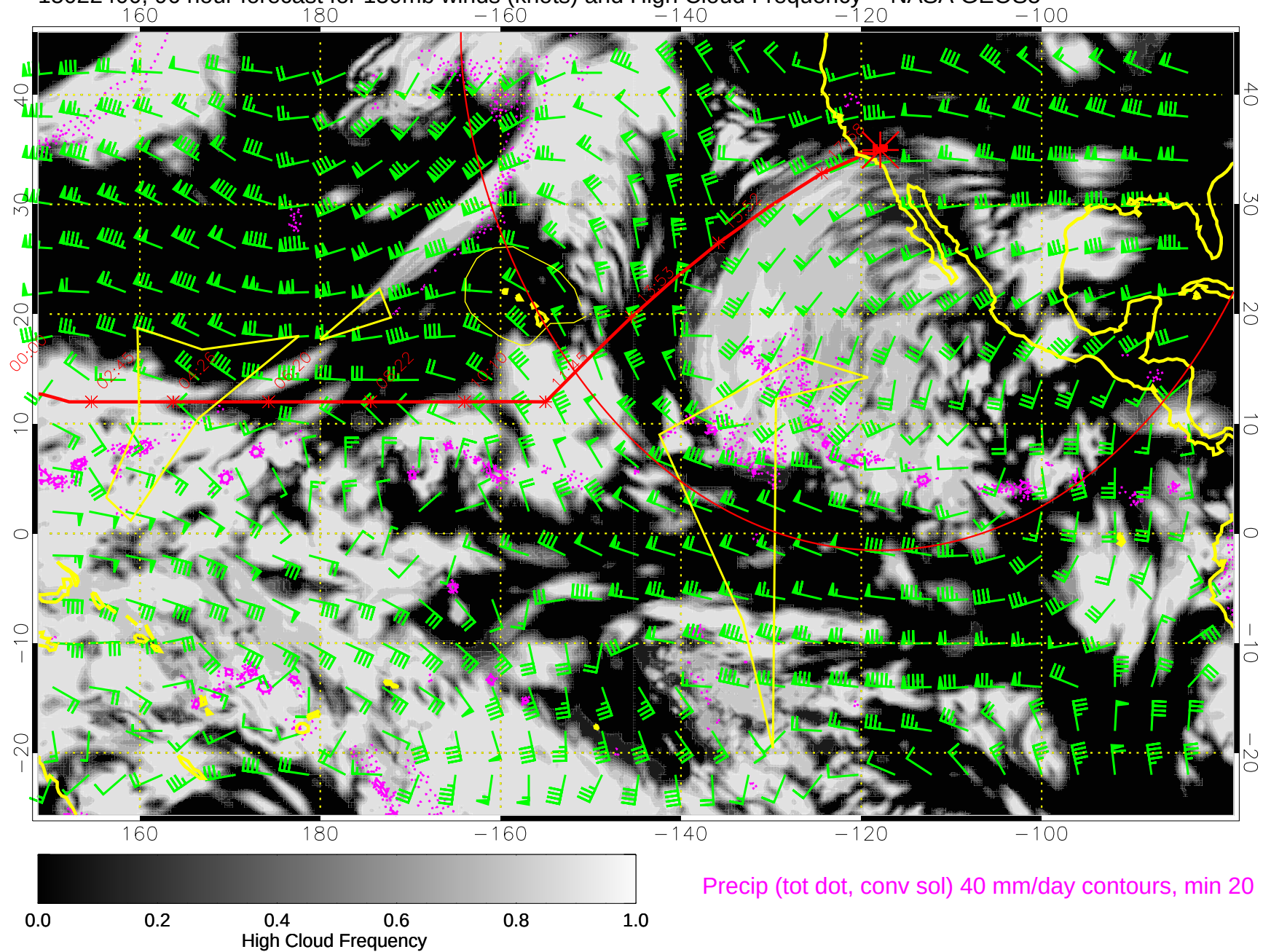
15022400, 96 hour forecast for 150mb winds (knots) and High Cloud Frequency -- NASA GEOS5
