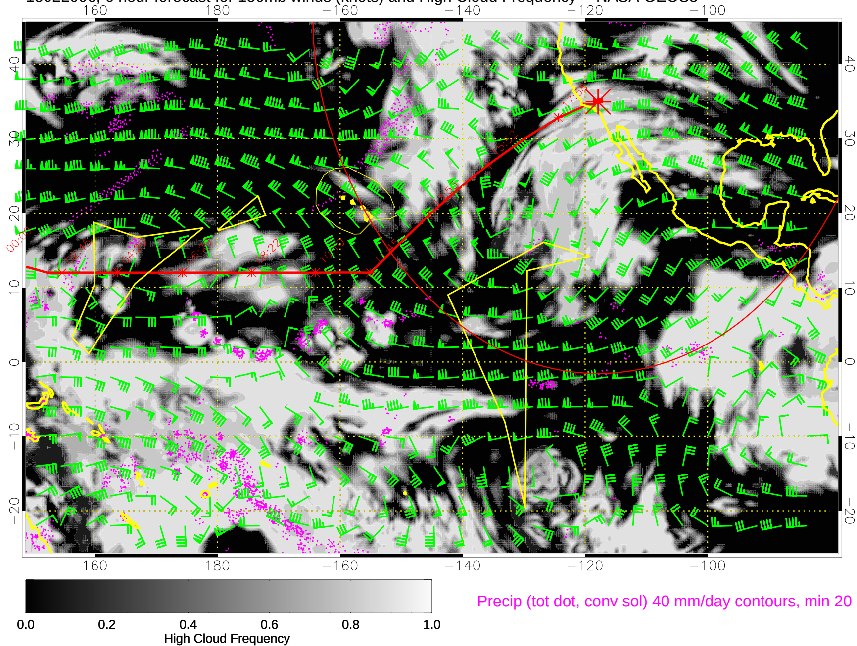
15022006, 6 hour forecast for 150mb winds (knots) and High Cloud Frequency -- NASA GEOS5
