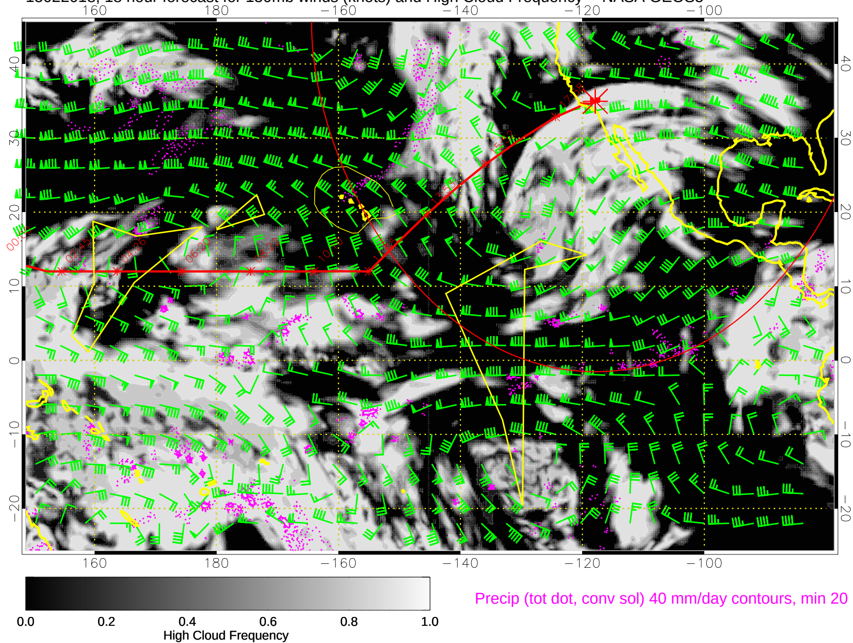
15022018, 18 hour forecast for 150mb winds (knots) and High Cloud Frequency -- NASA GEOS5
