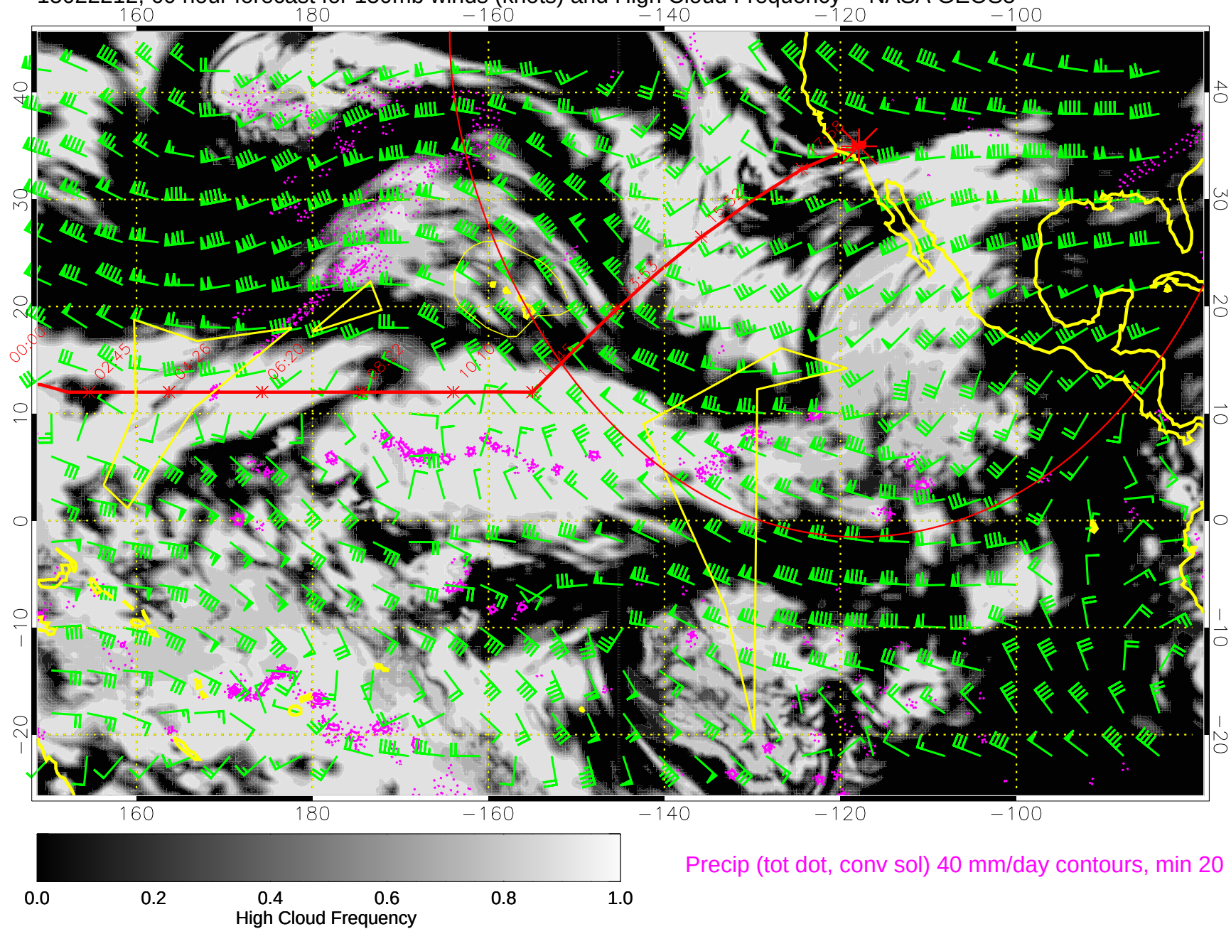
15022212, 60 hour forecast for 150mb winds (knots) and High Cloud Frequency -- NASA GEOS5
