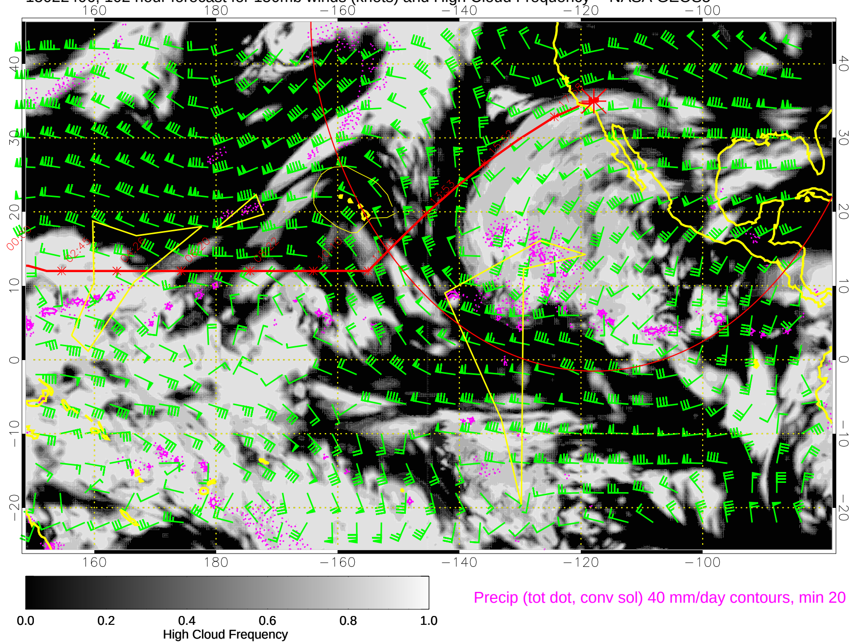
15022406, 102 hour forecast for 150mb winds (knots) and High Cloud Frequency -- NASA GEOS5
