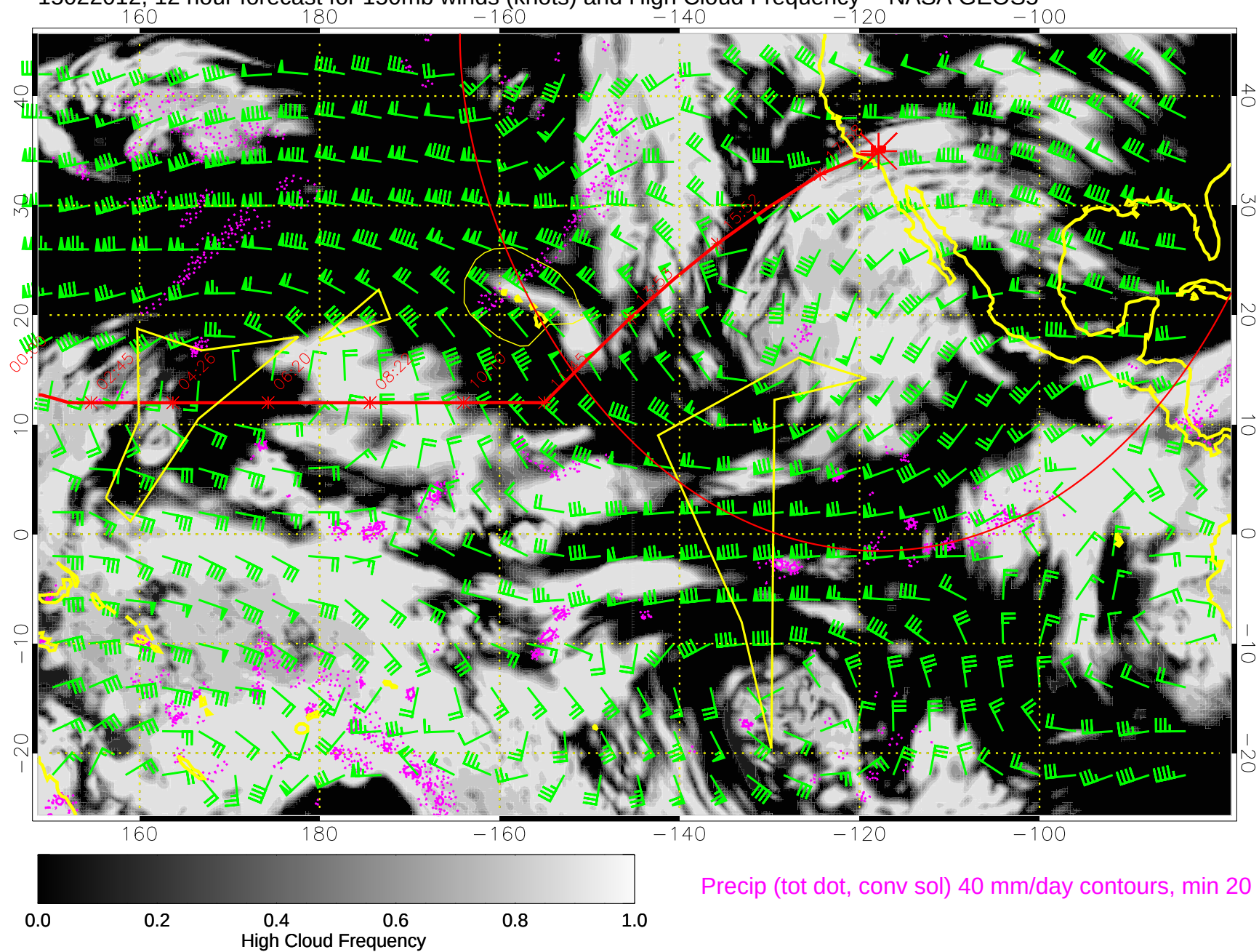
15022012, 12 hour forecast for 150mb winds (knots) and High Cloud Frequency -- NASA GEOS5
