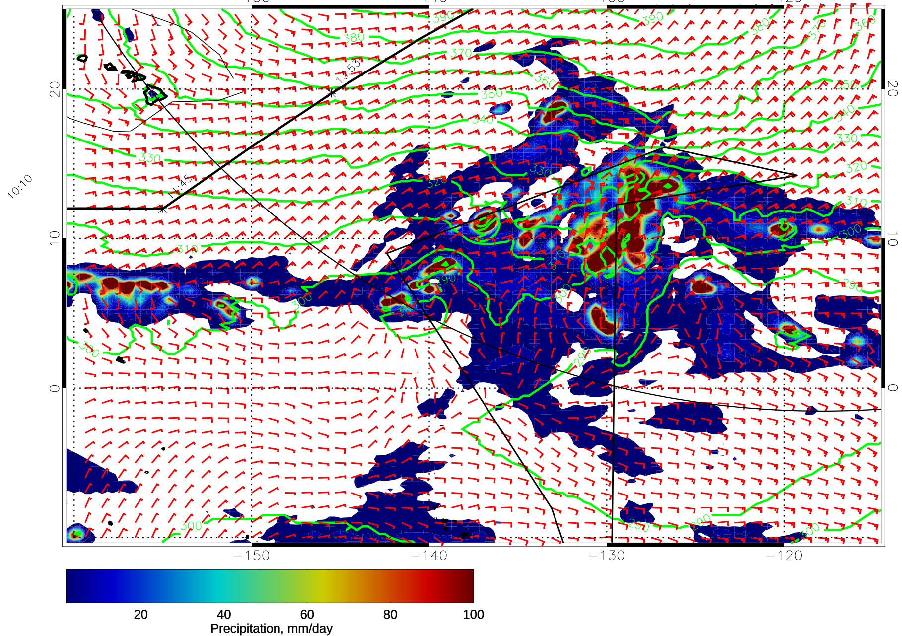
15022400, 120 hour forecast for 975mb Z, Precip., and Surface Winds (knots) -- NASA GEOS5
