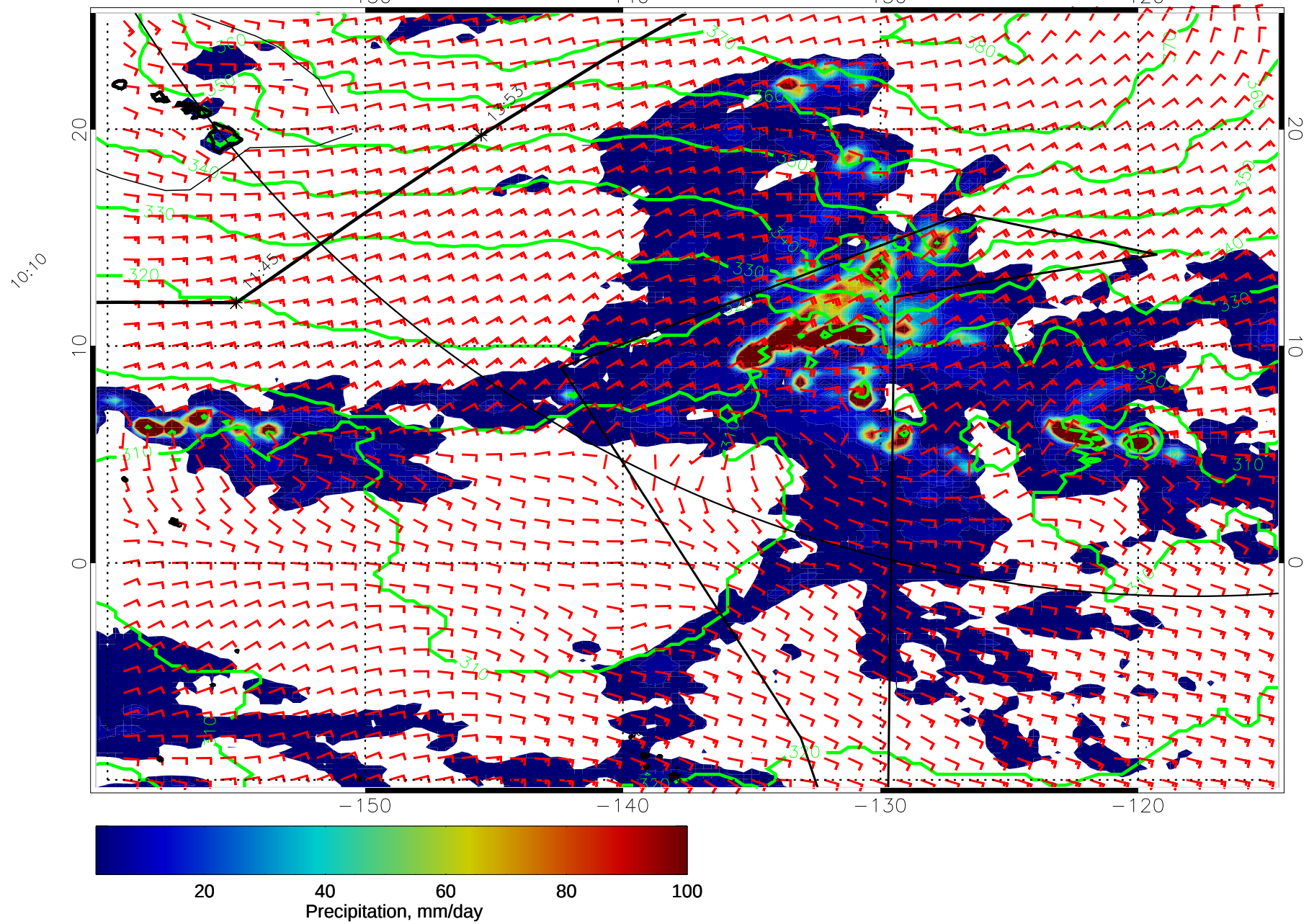
15022306, 102 hour forecast for 975mb Z, Precip., and Surface Winds (knots) -- NASA GEOS5
