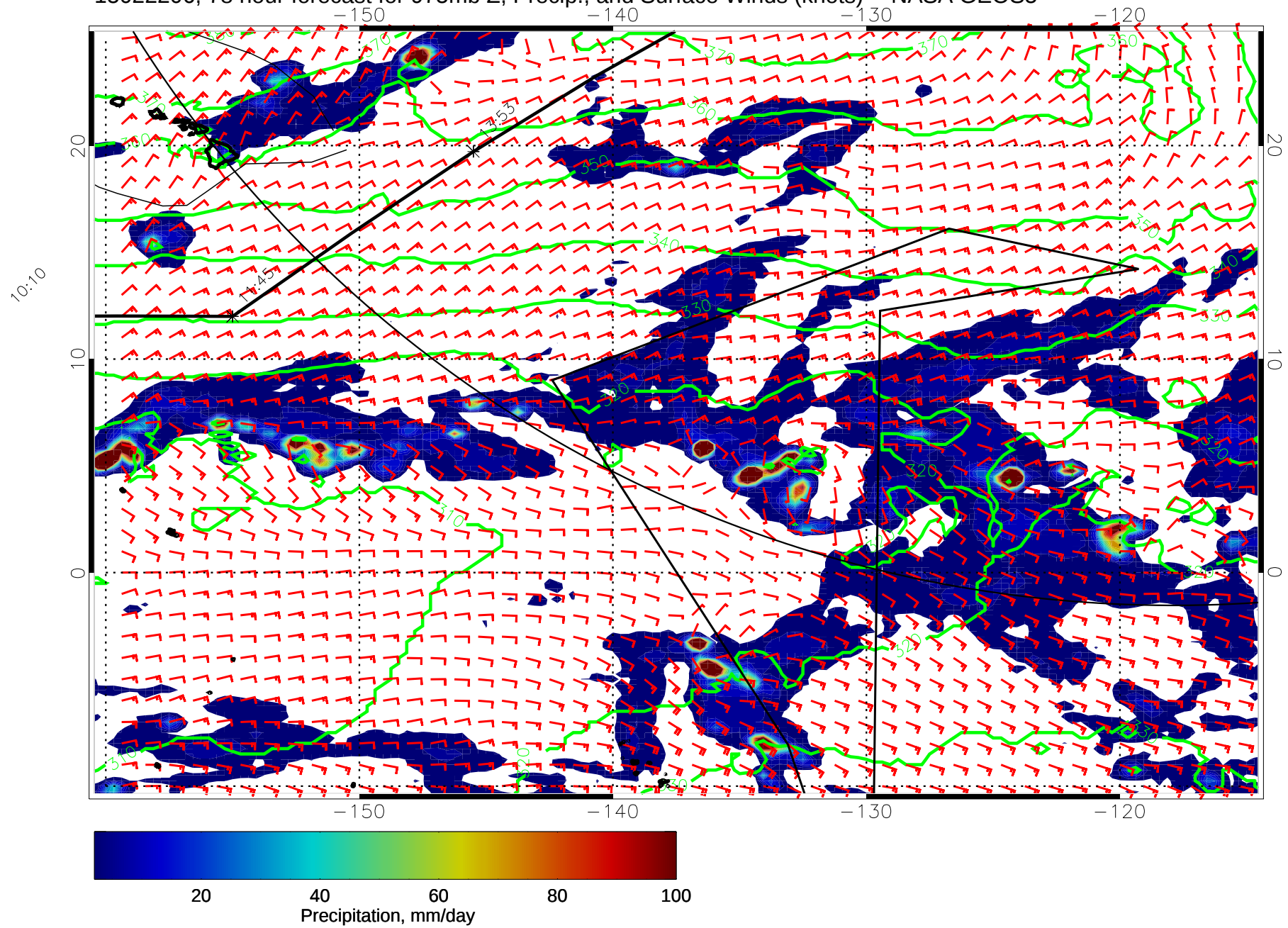
15022206, 78 hour forecast for 975mb Z, Precip., and Surface Winds (knots) -- NASA GEOS5
