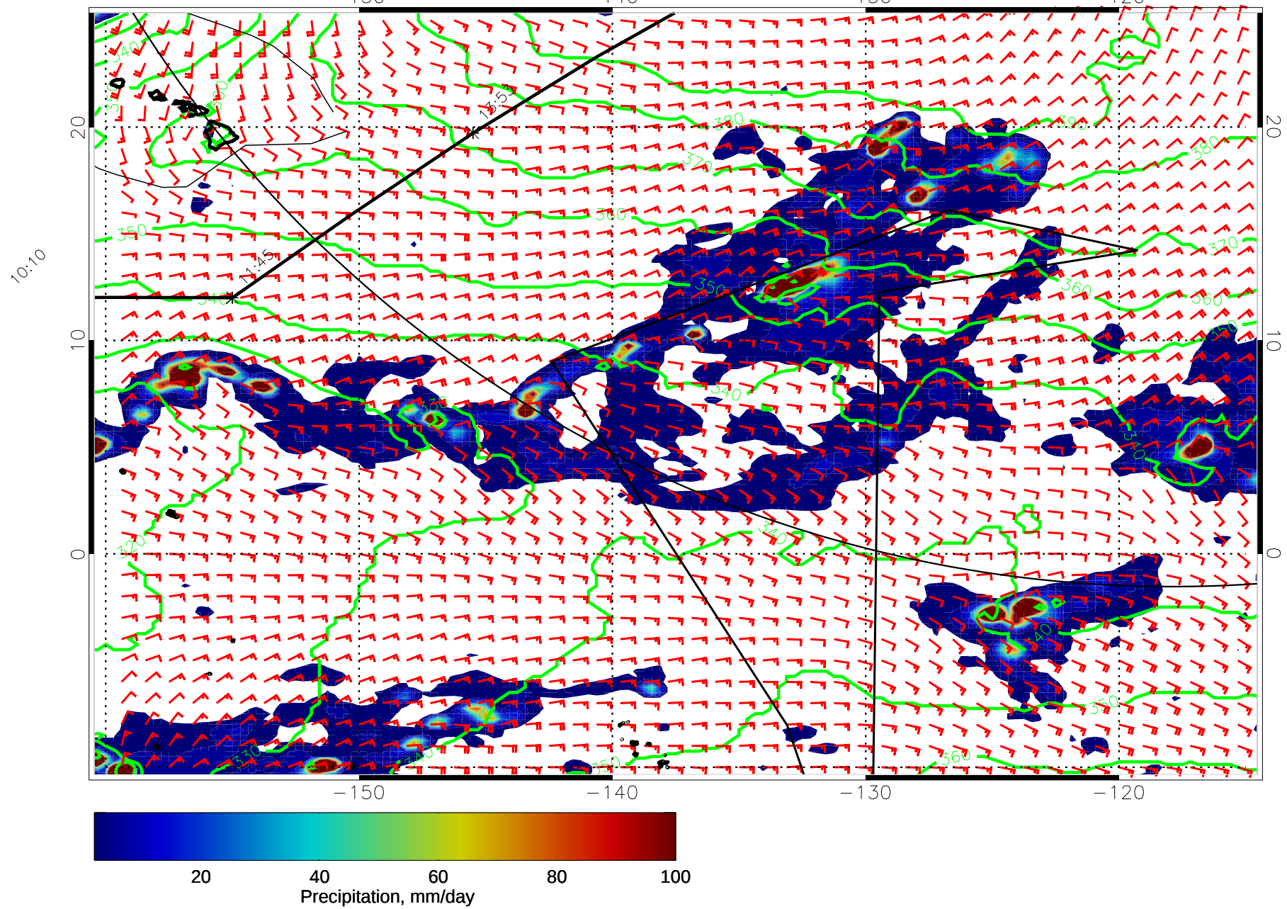
15021918, 18 hour forecast for 975mb Z, Precip., and Surface Winds (knots) -- NASA GEOS5
