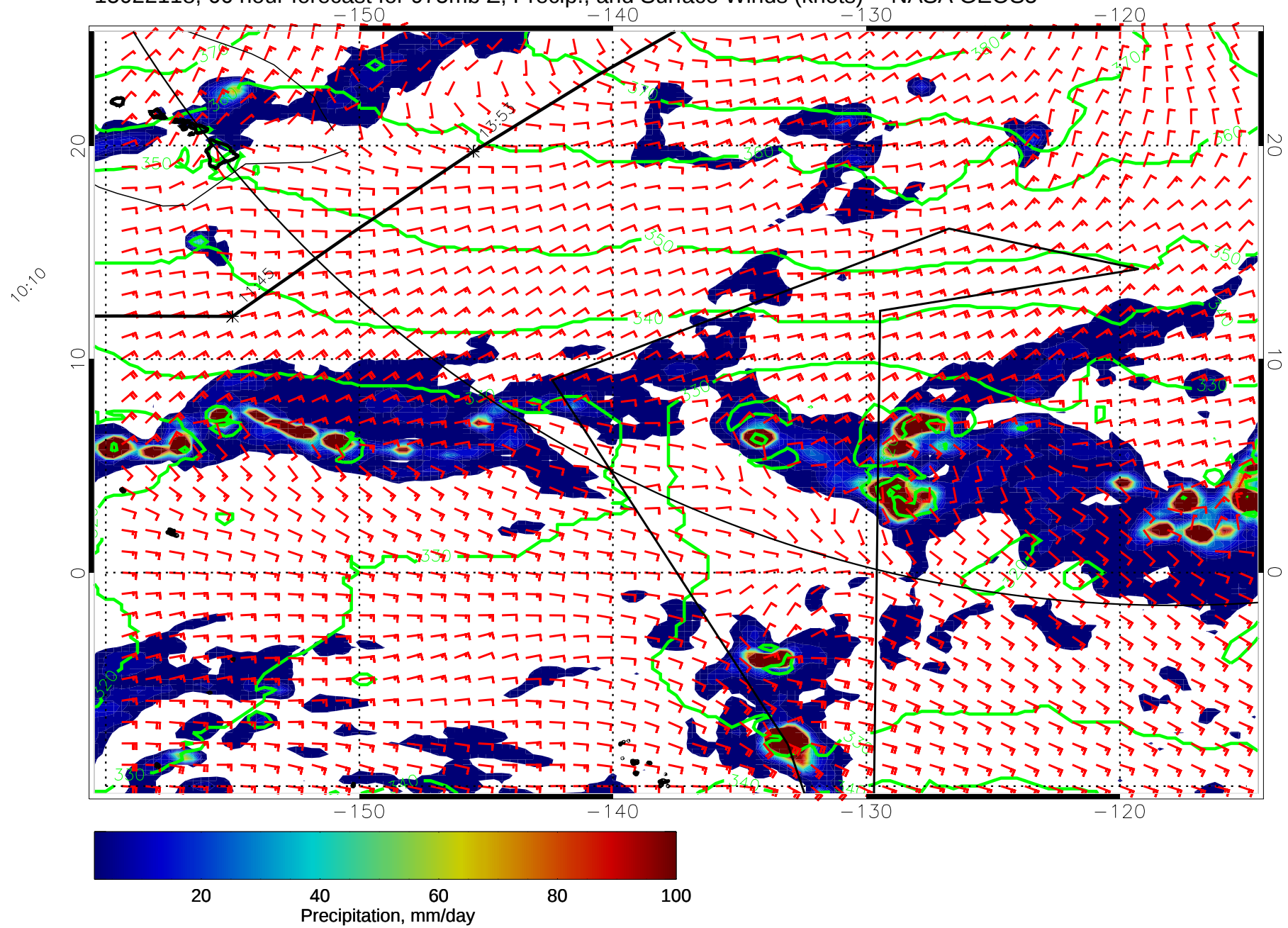
15022118, 66 hour forecast for 975mb Z, Precip., and Surface Winds (knots) -- NASA GEOS5
