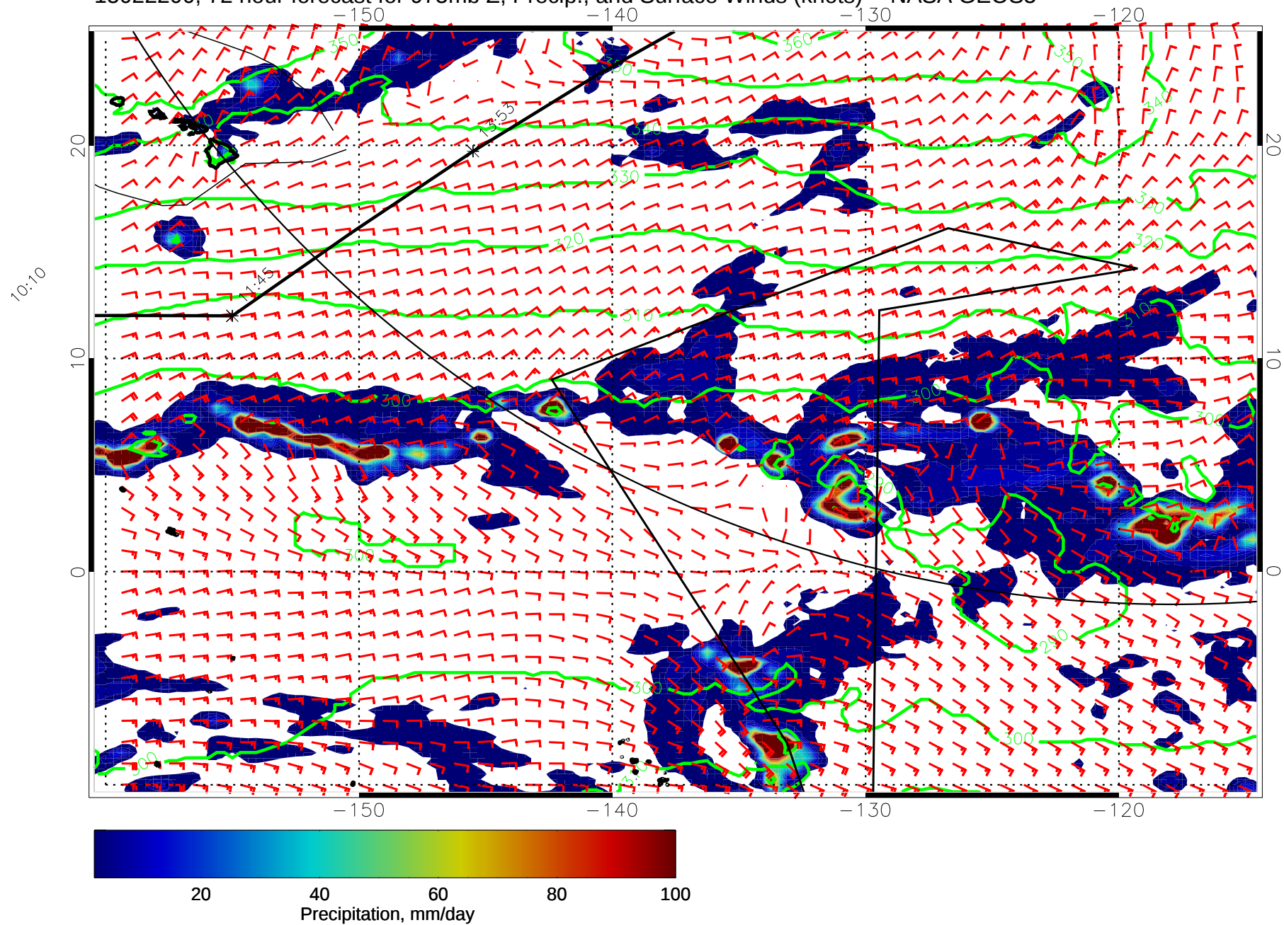
15022200, 72 hour forecast for 975mb Z, Precip., and Surface Winds (knots) -- NASA GEOS5
