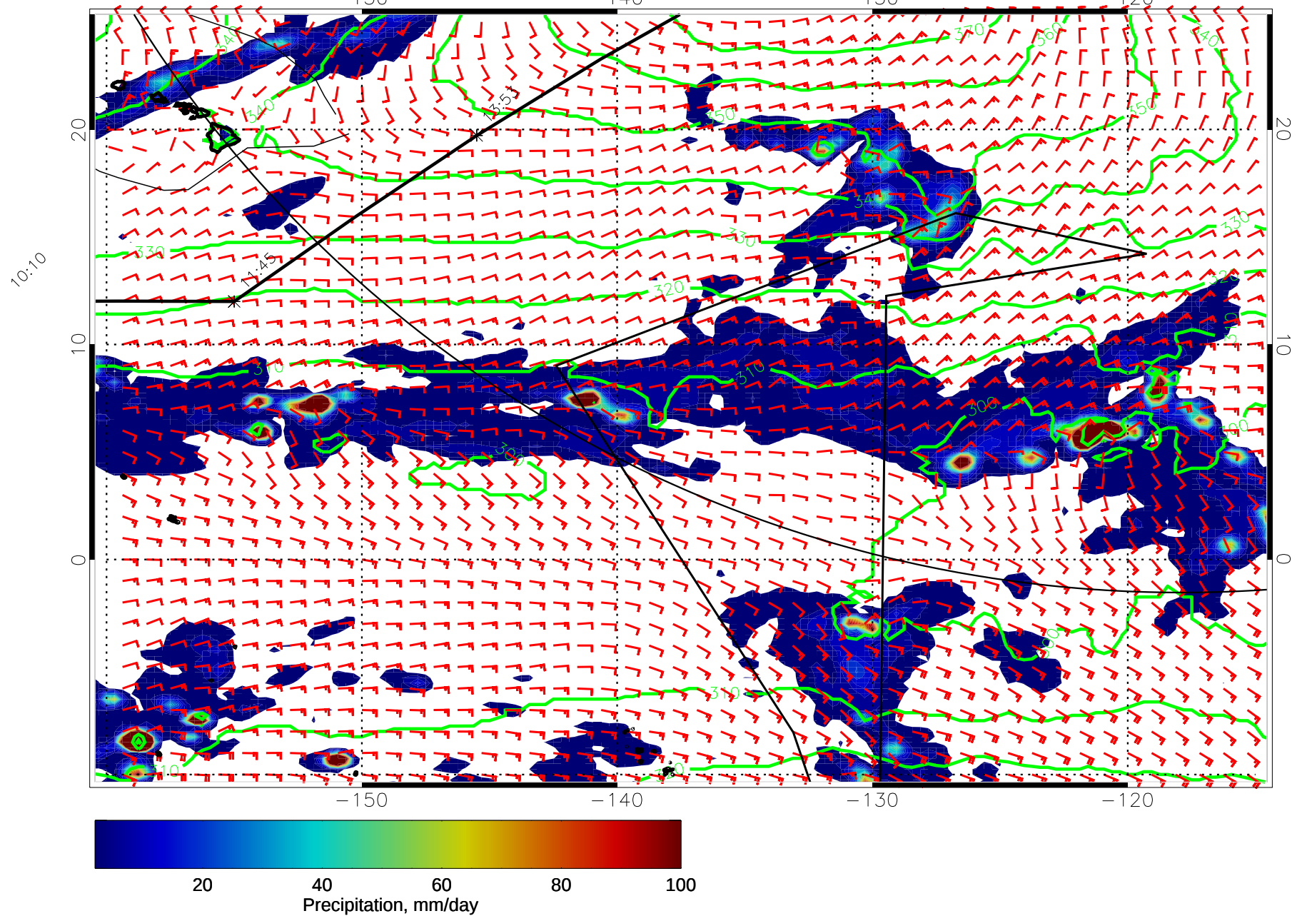
15022100, 48 hour forecast for 975mb Z, Precip., and Surface Winds (knots) -- NASA GEOS5
