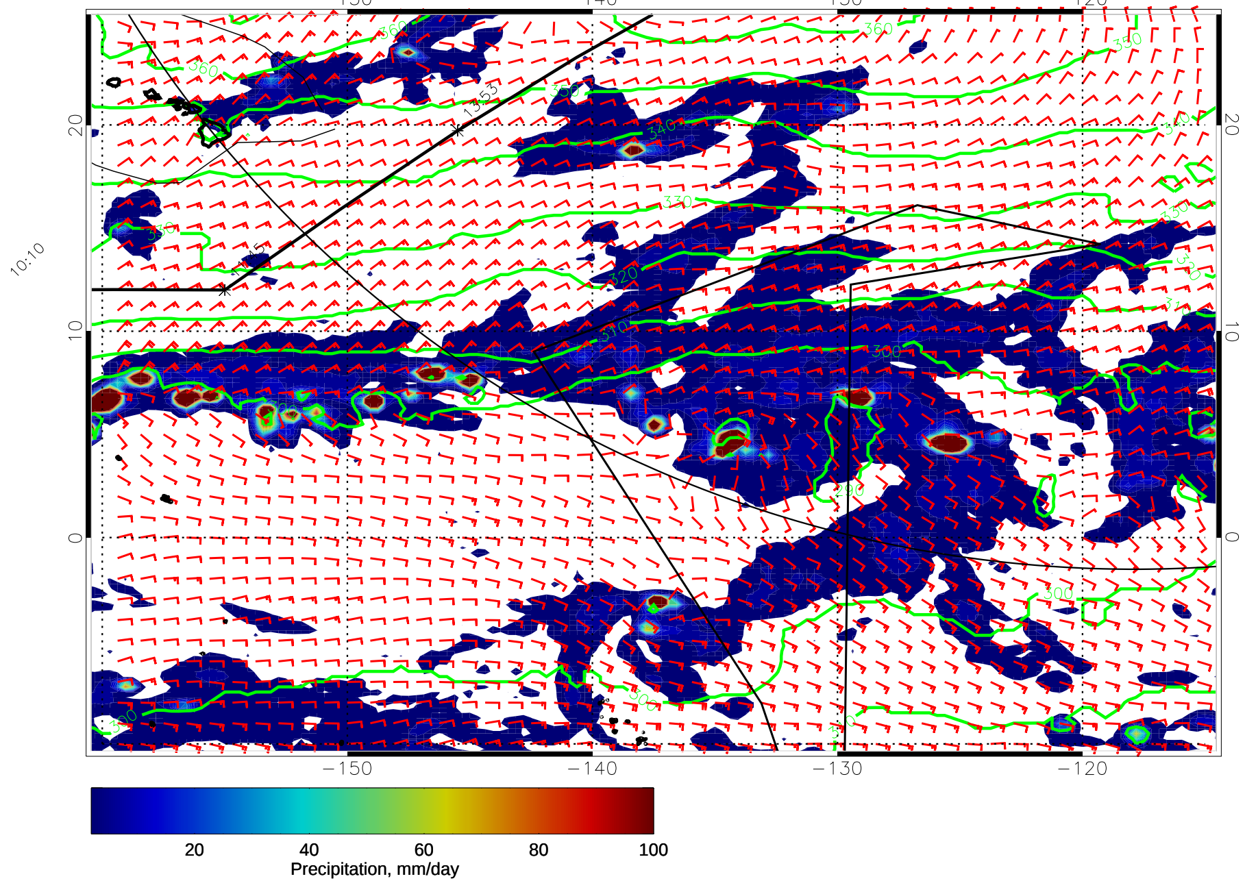
15022212, 84 hour forecast for 975mb Z, Precip., and Surface Winds (knots) -- NASA GEOS5
