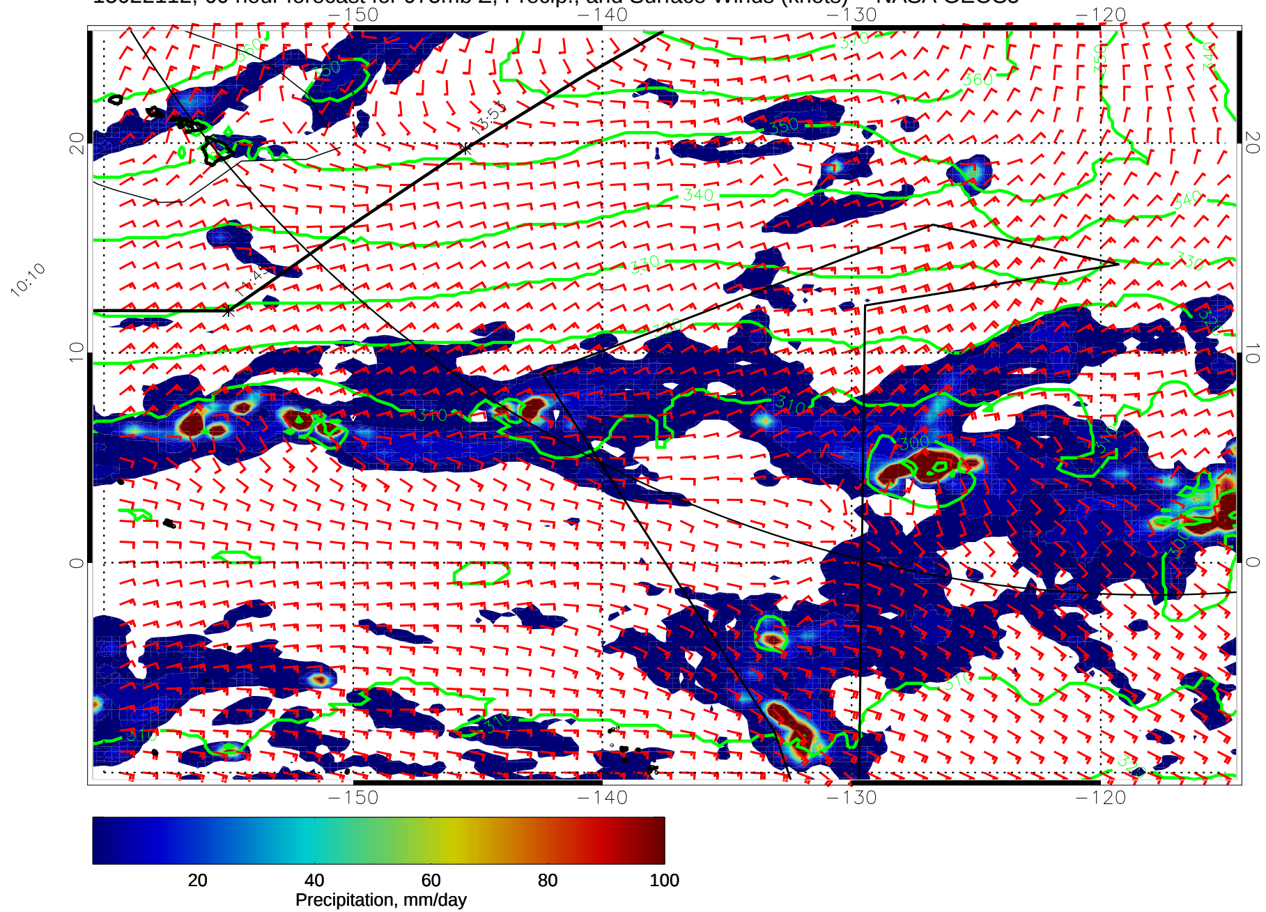
15022112, 60 hour forecast for 975mb Z, Precip., and Surface Winds (knots) -- NASA GEOS5
