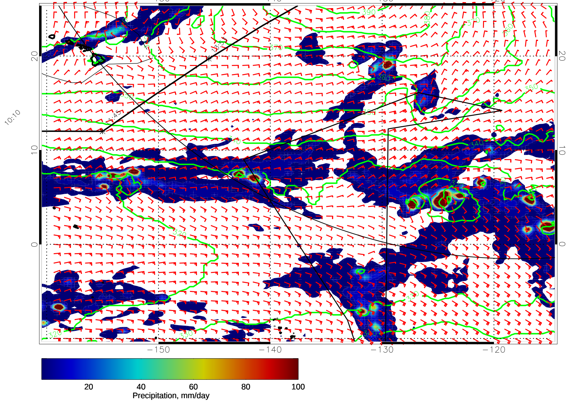
15022106, 54 hour forecast for 975mb Z, Precip., and Surface Winds (knots) -- NASA GEOS5
