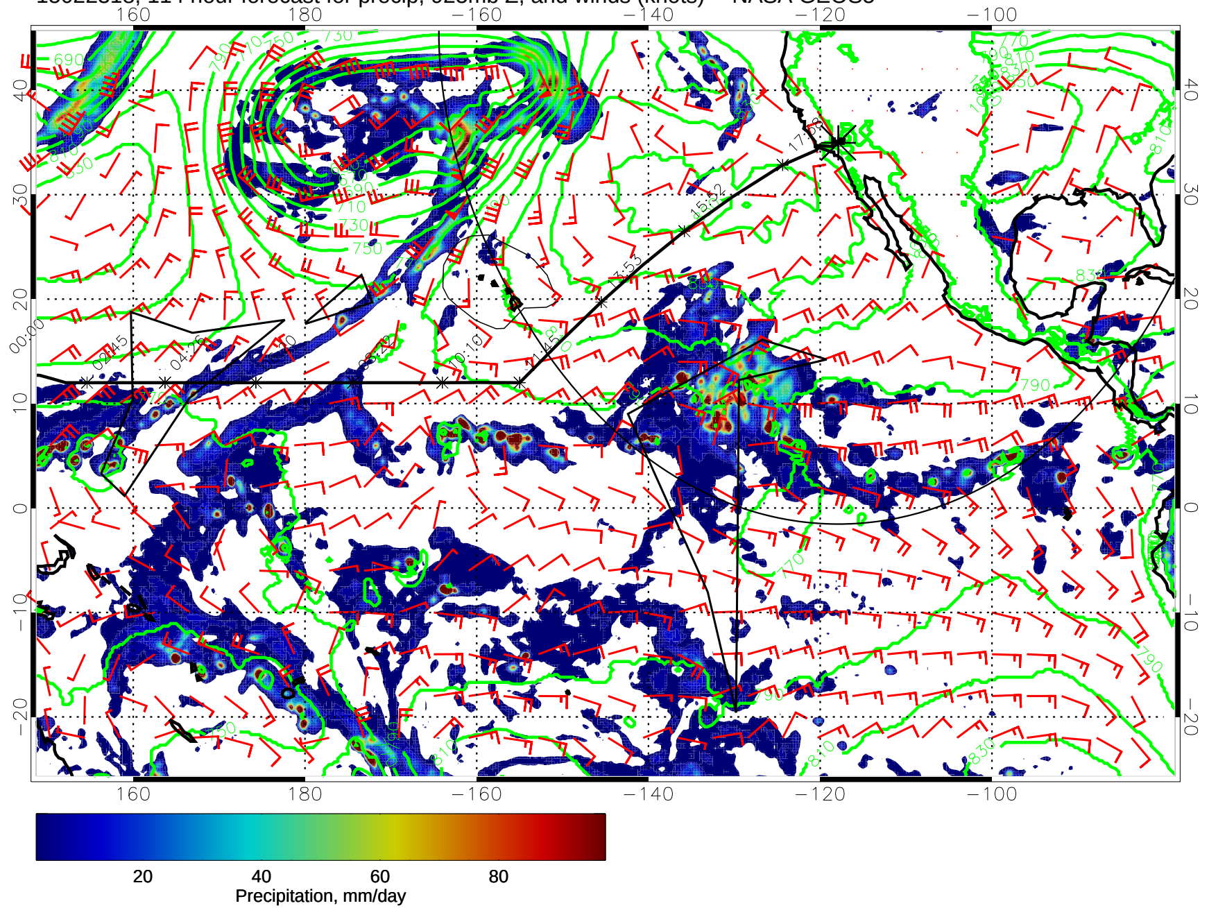
15022318, 114 hour forecast for precip, 925mb Z, and winds (knots) -- NASA GEOS5
