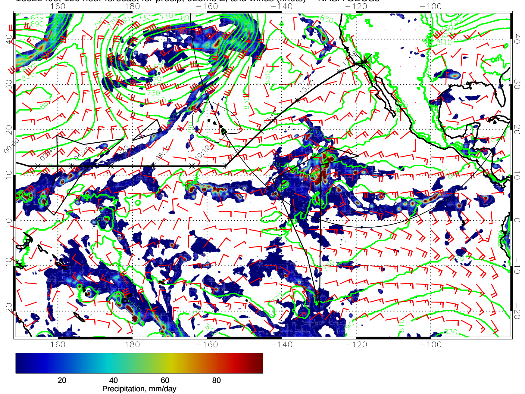
15022400, 120 hour forecast for precip, 925mb Z, and winds (knots) -- NASA GEOS5
