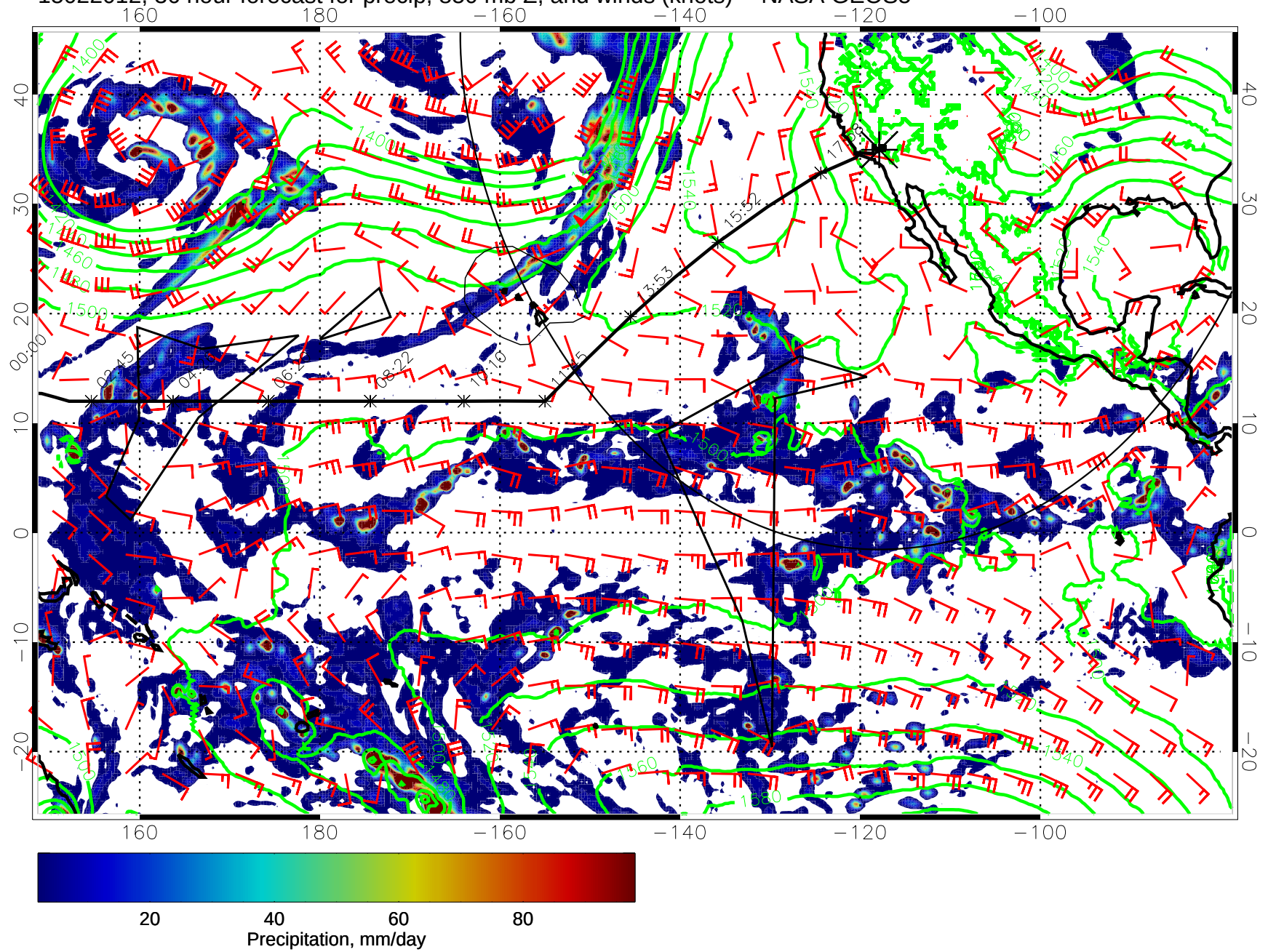
15022012, 36 hour forecast for precip, 850 mb Z, and winds (knots) -- NASA GEOS5
