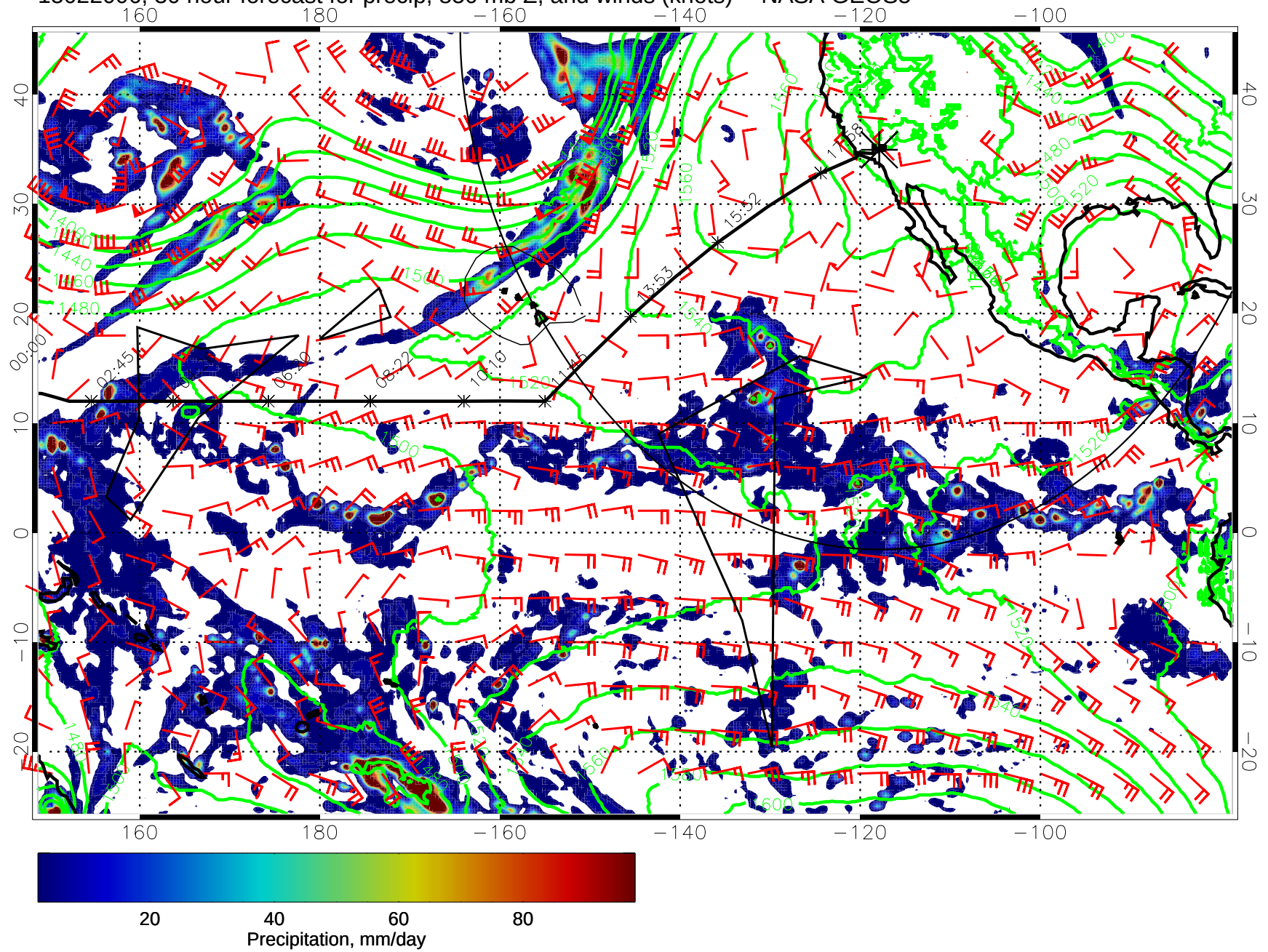
15022006, 30 hour forecast for precip, 850 mb Z, and winds (knots) -- NASA GEOS5
