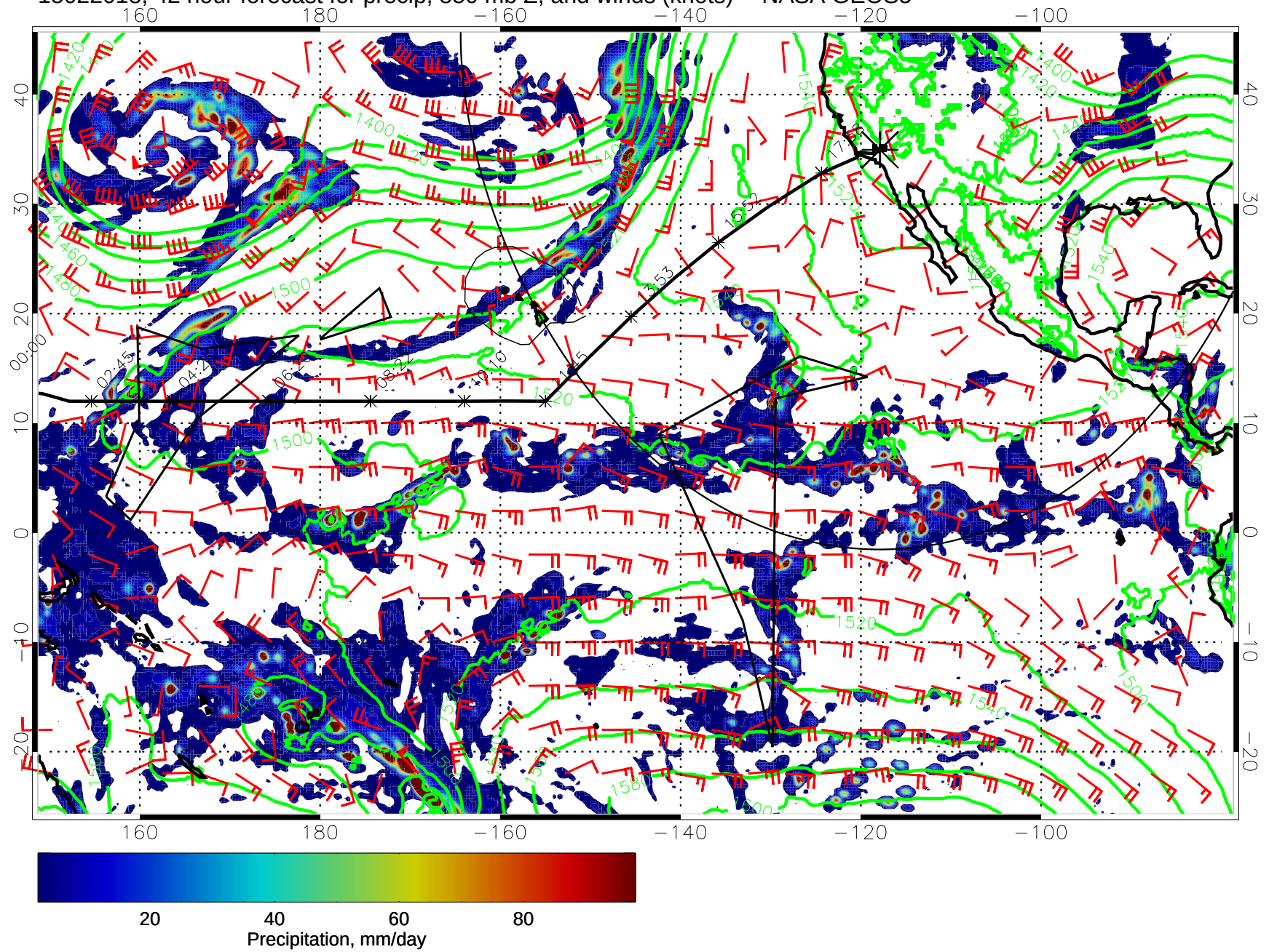
15022018, 42 hour forecast for precip, 850 mb Z, and winds (knots) -- NASA GEOS5
