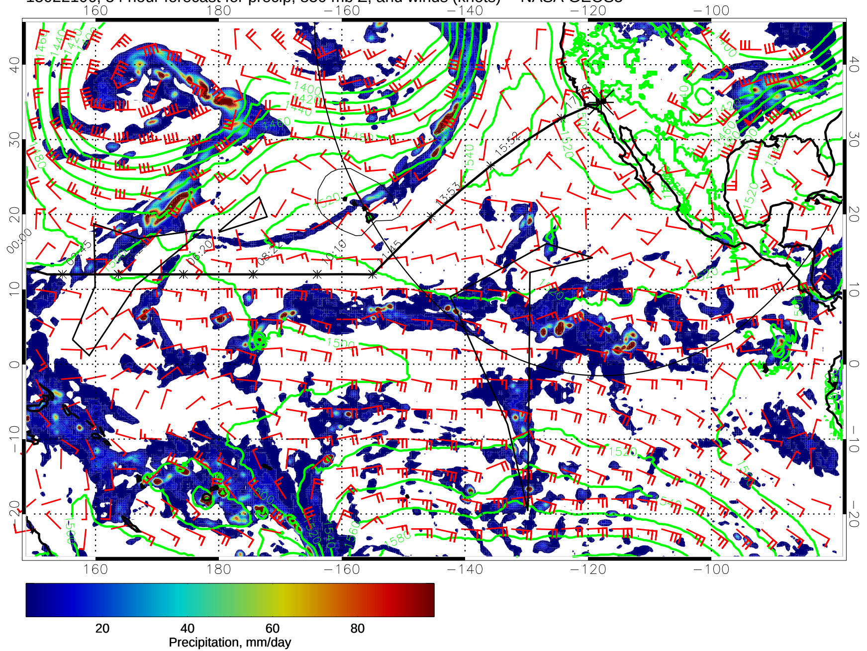
15022106, 54 hour forecast for precip, 850 mb Z, and winds (knots) -- NASA GEOS5
