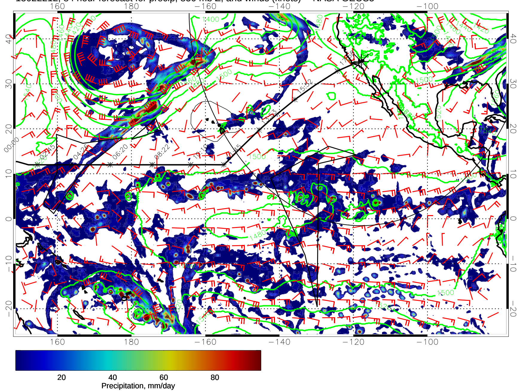
15022212, 84 hour forecast for precip, 850 mb Z, and winds (knots) -- NASA GEOS5
