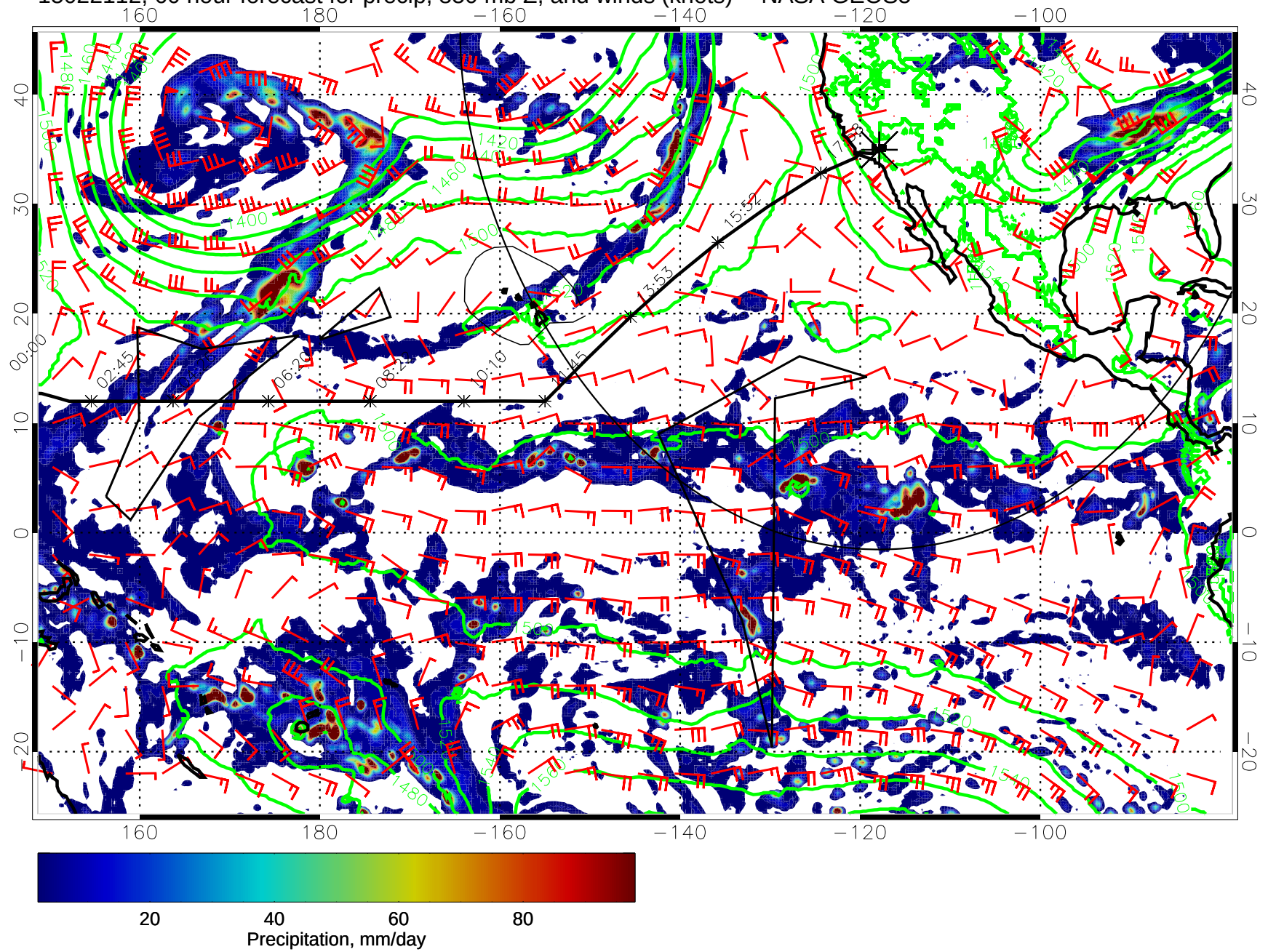
15022112, 60 hour forecast for precip, 850 mb Z, and winds (knots) -- NASA GEOS5
