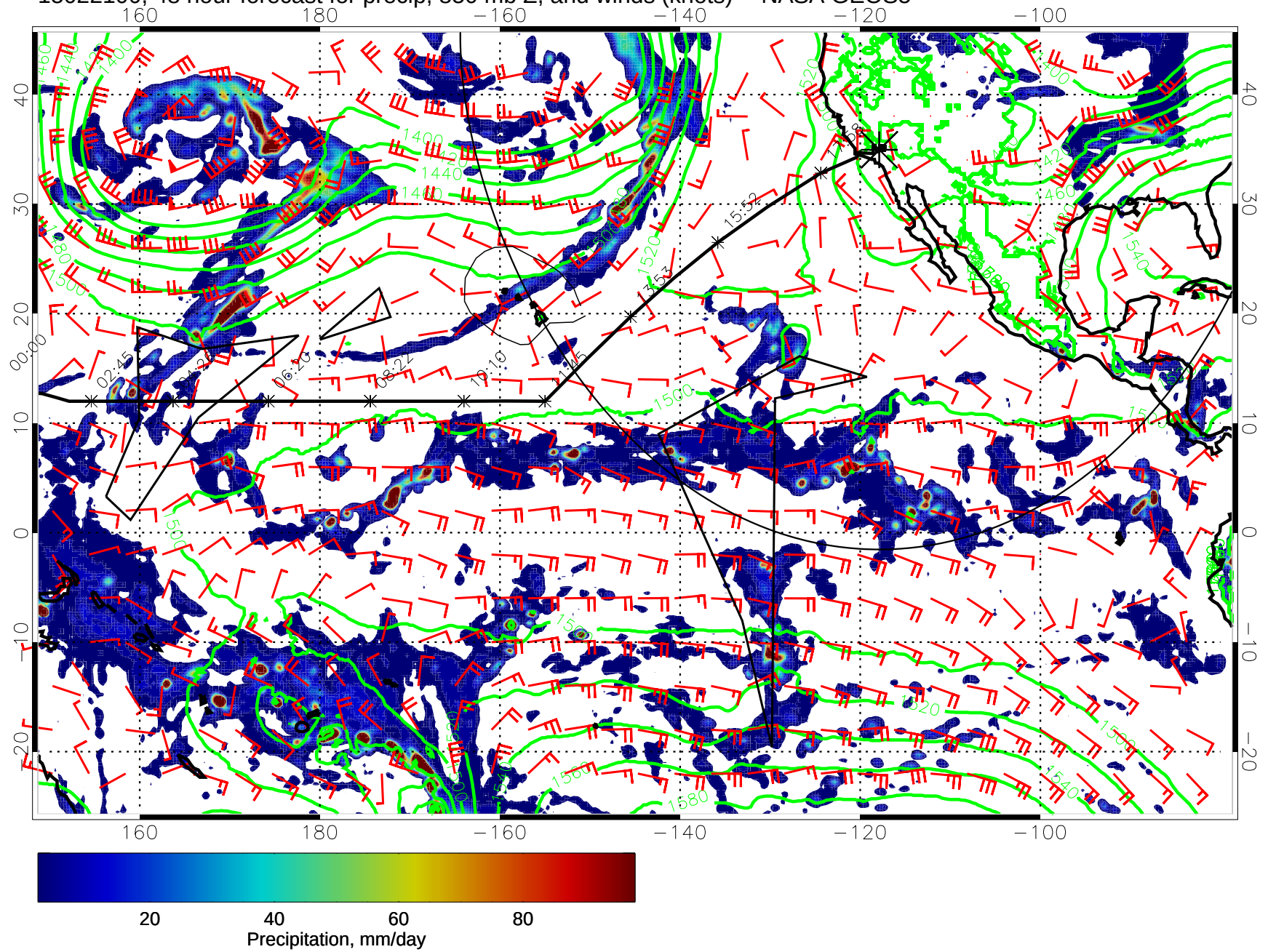
15022100, 48 hour forecast for precip, 850 mb Z, and winds (knots) -- NASA GEOS5
