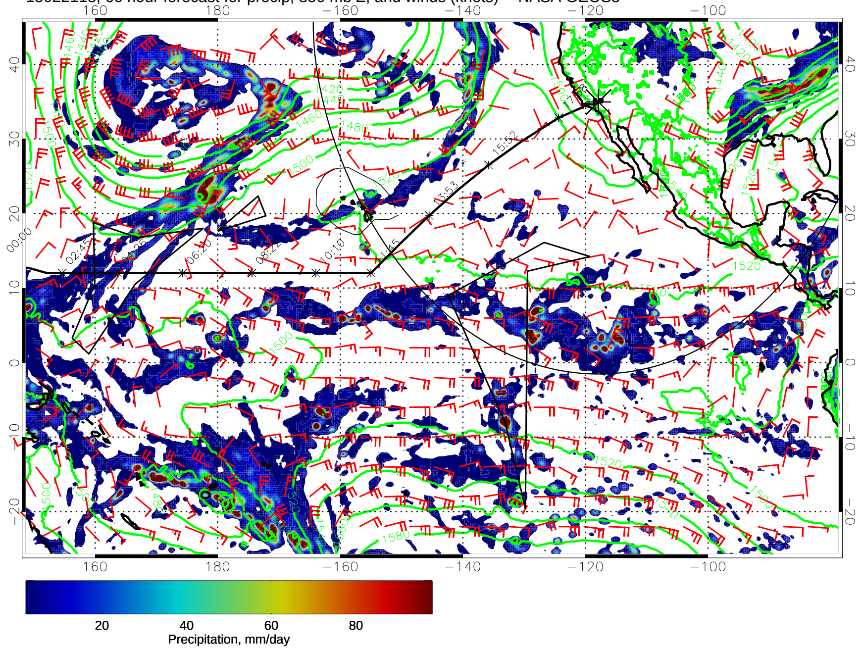
15022118, 66 hour forecast for precip, 850 mb Z, and winds (knots) -- NASA GEOS5
