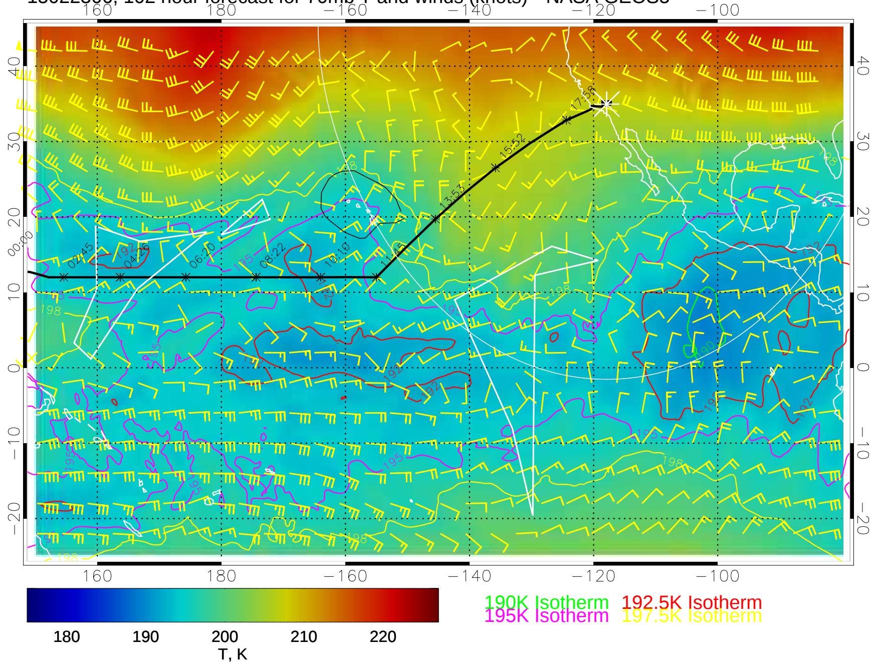
15022306, 102 hour forecast for 70mb T and winds (knots)-- NASA GEOS5
