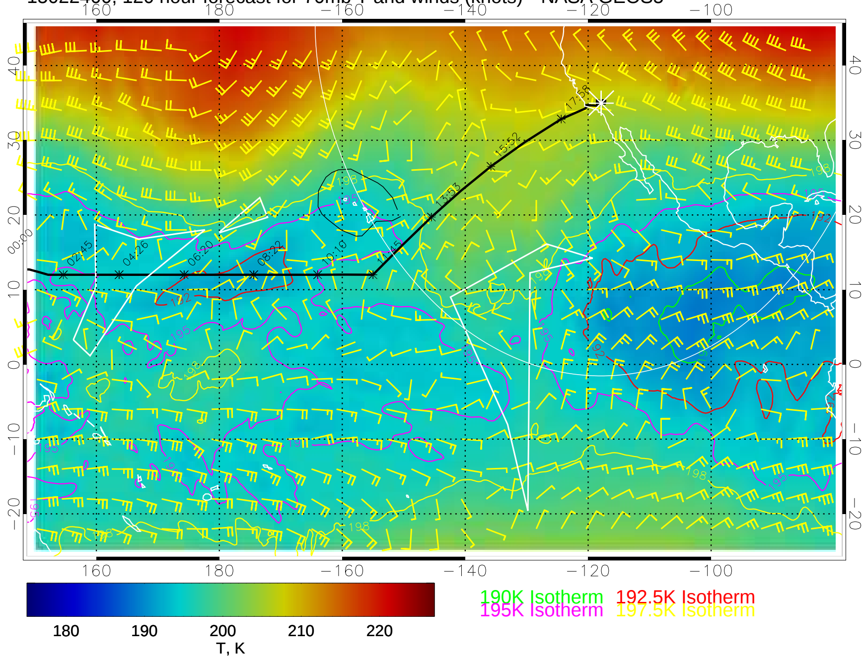
15022400, 120 hour forecast for 70mb T and winds (knots)-- NASA GEOS5
