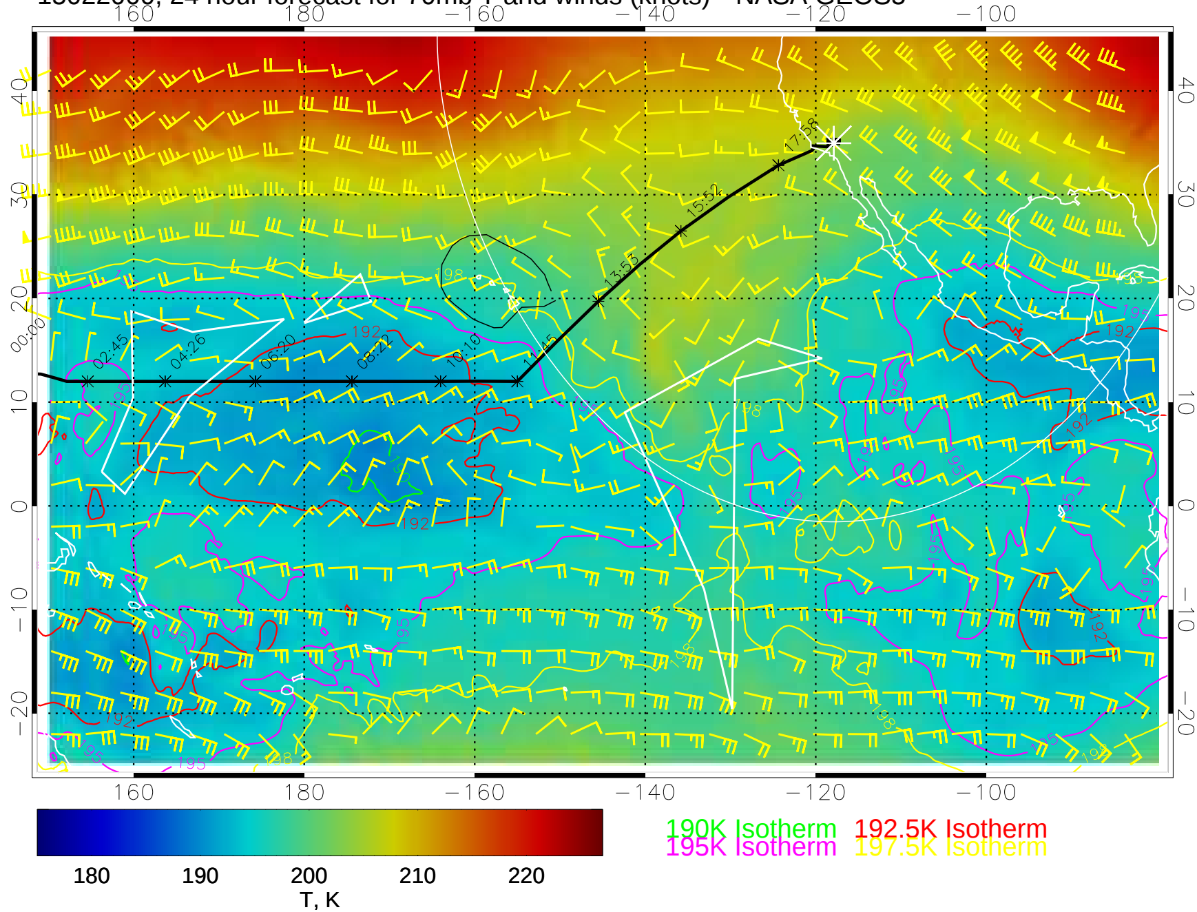
15022000, 24 hour forecast for 70mb T and winds (knots)-- NASA GEOS5
