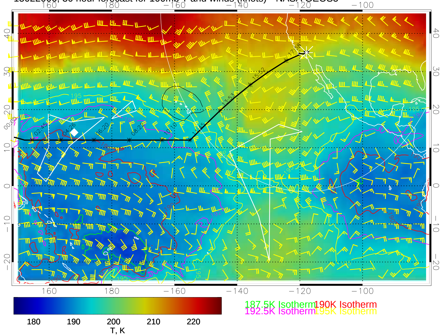
15022006, 30 hour forecast for 100mb T and winds (knots)-- NASA GEOS5
