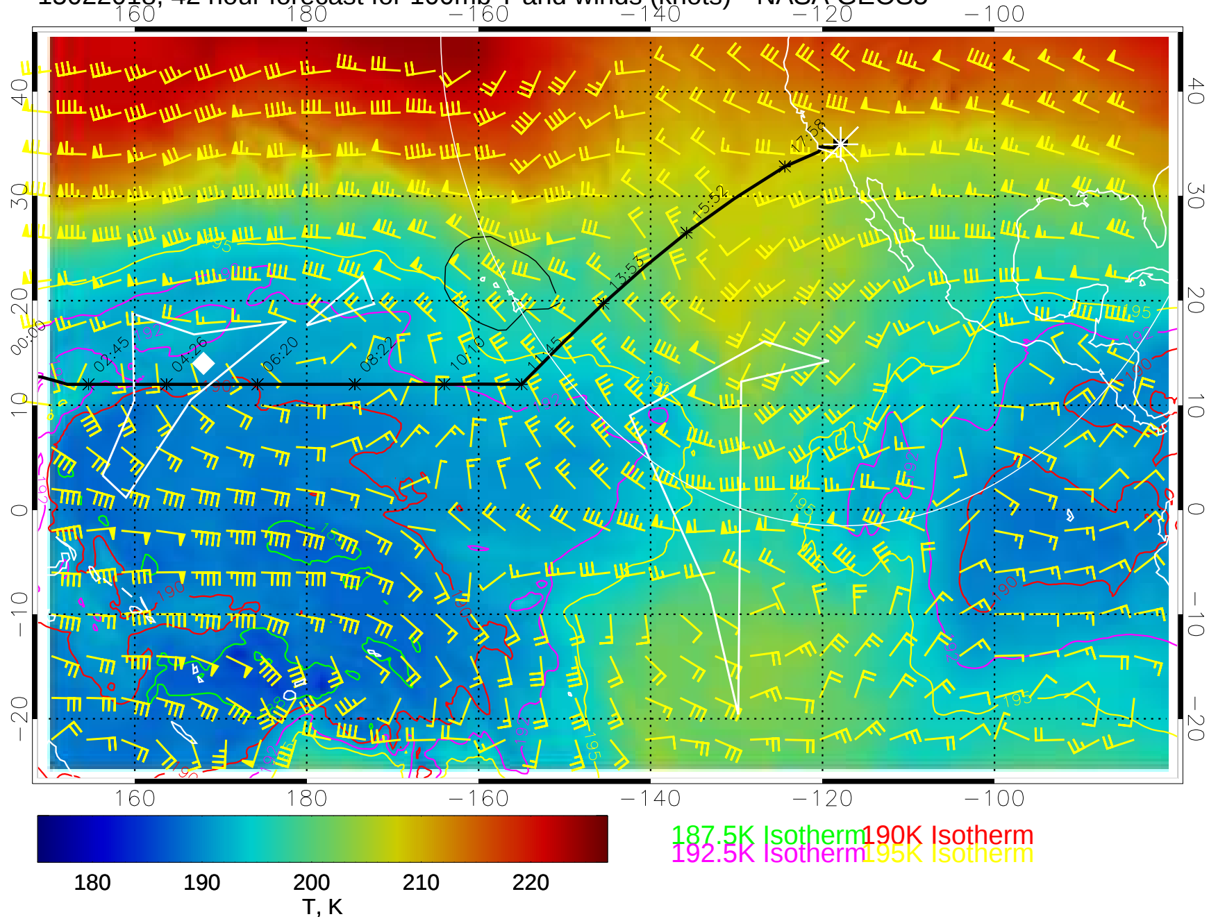
15022018, 42 hour forecast for 100mb T and winds (knots)-- NASA GEOS5
