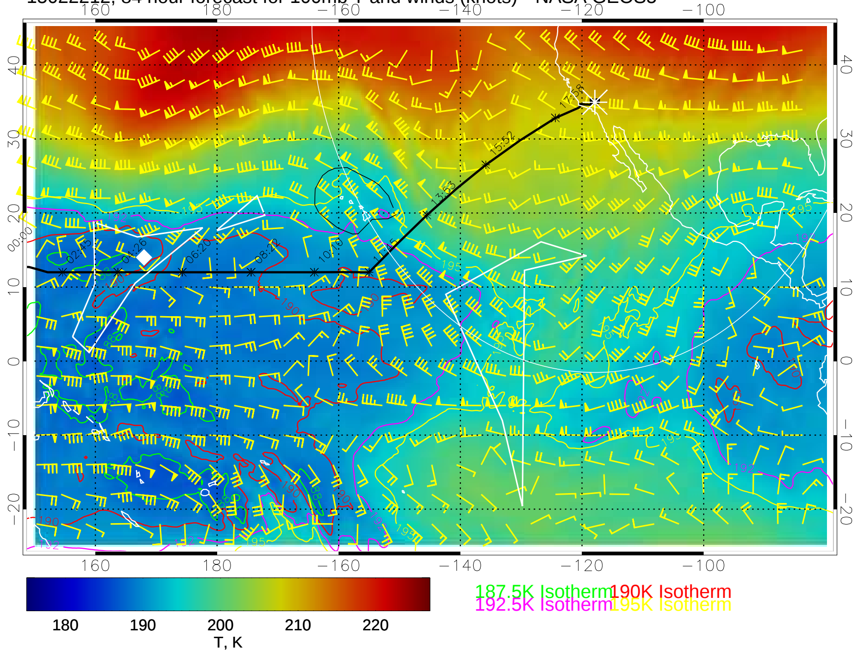
15022212, 84 hour forecast for 100mb T and winds (knots)-- NASA GEOS5
