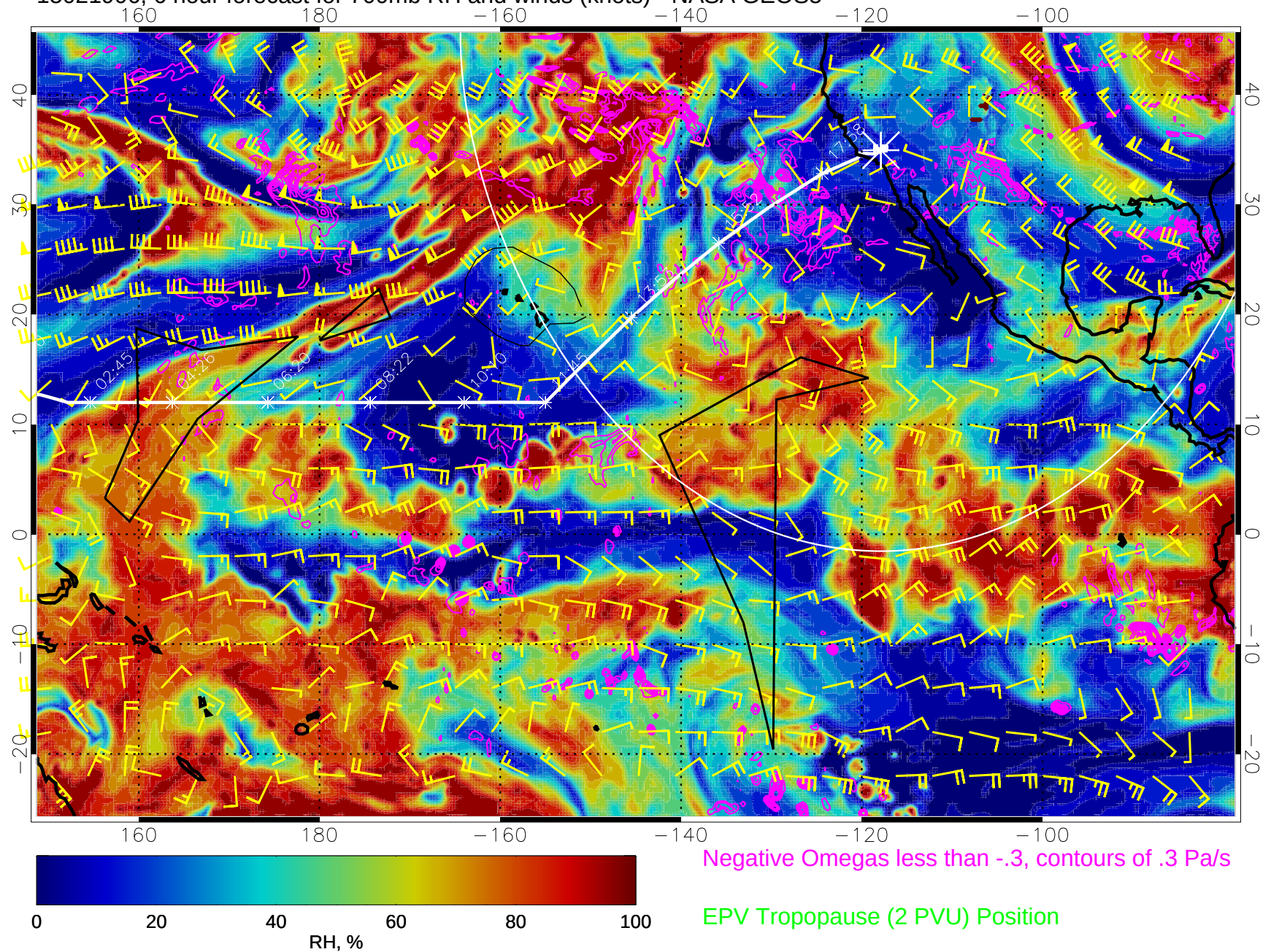
15021906, 6 hour forecast for 700mb RH and winds (knots) - NASA GEOS5
