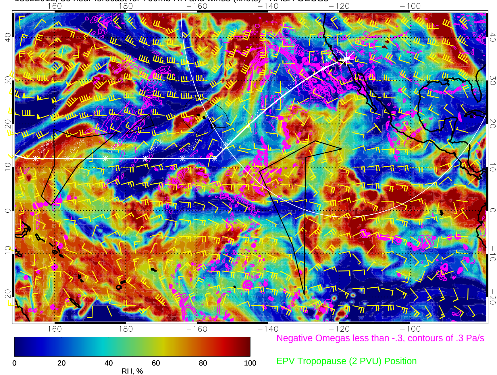
15022012, 36 hour forecast for 700mb RH and winds (knots) - NASA GEOS5
