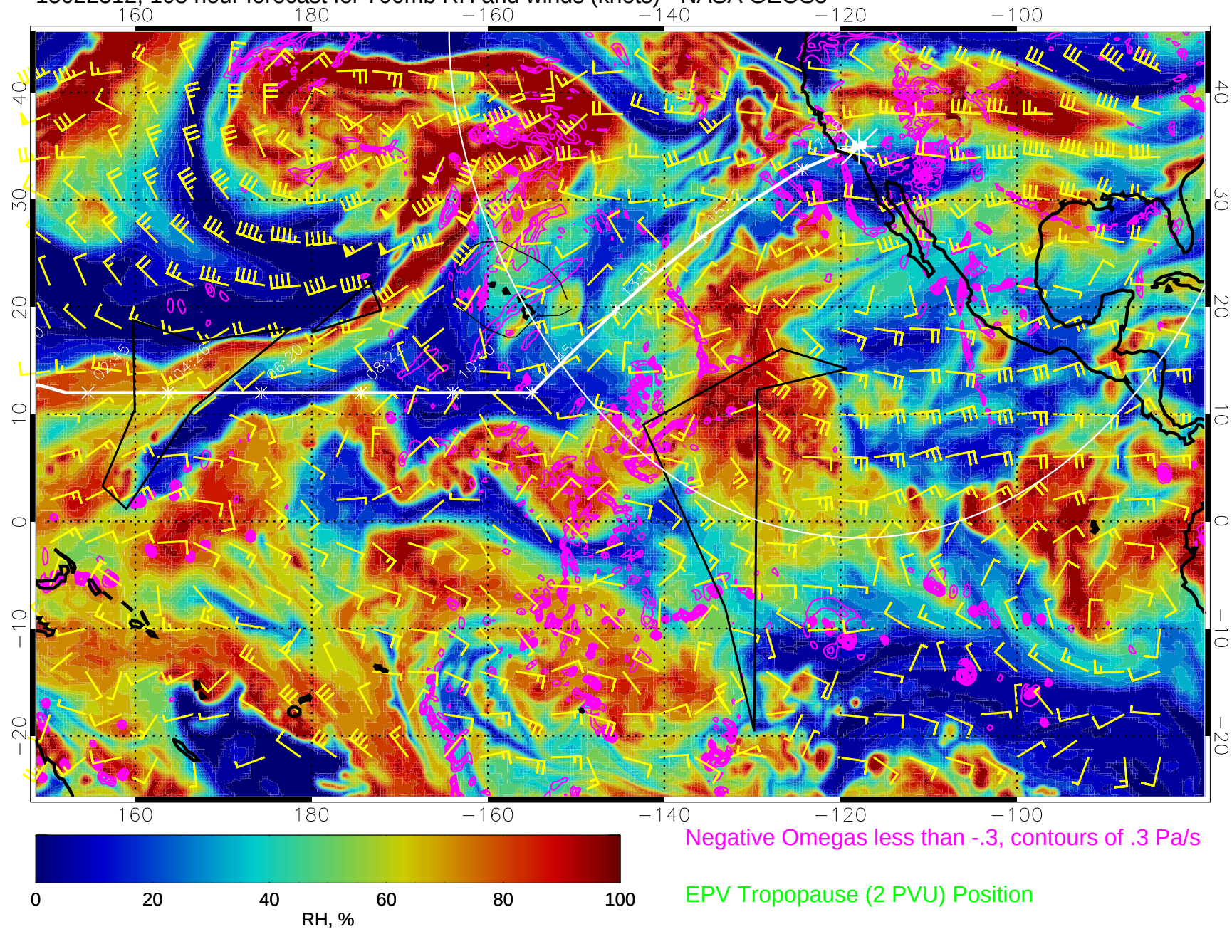
15022312, 108 hour forecast for 700mb RH and winds (knots) - NASA GEOS5
