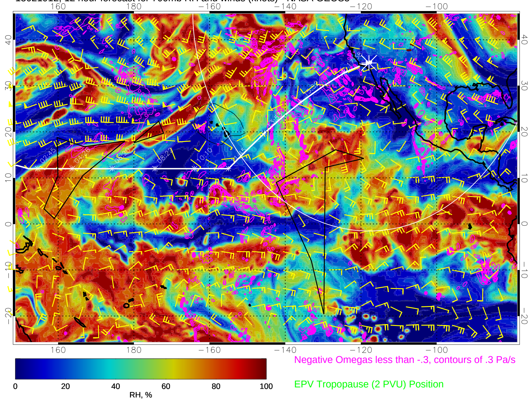
15021912, 12 hour forecast for 700mb RH and winds (knots) - NASA GEOS5
