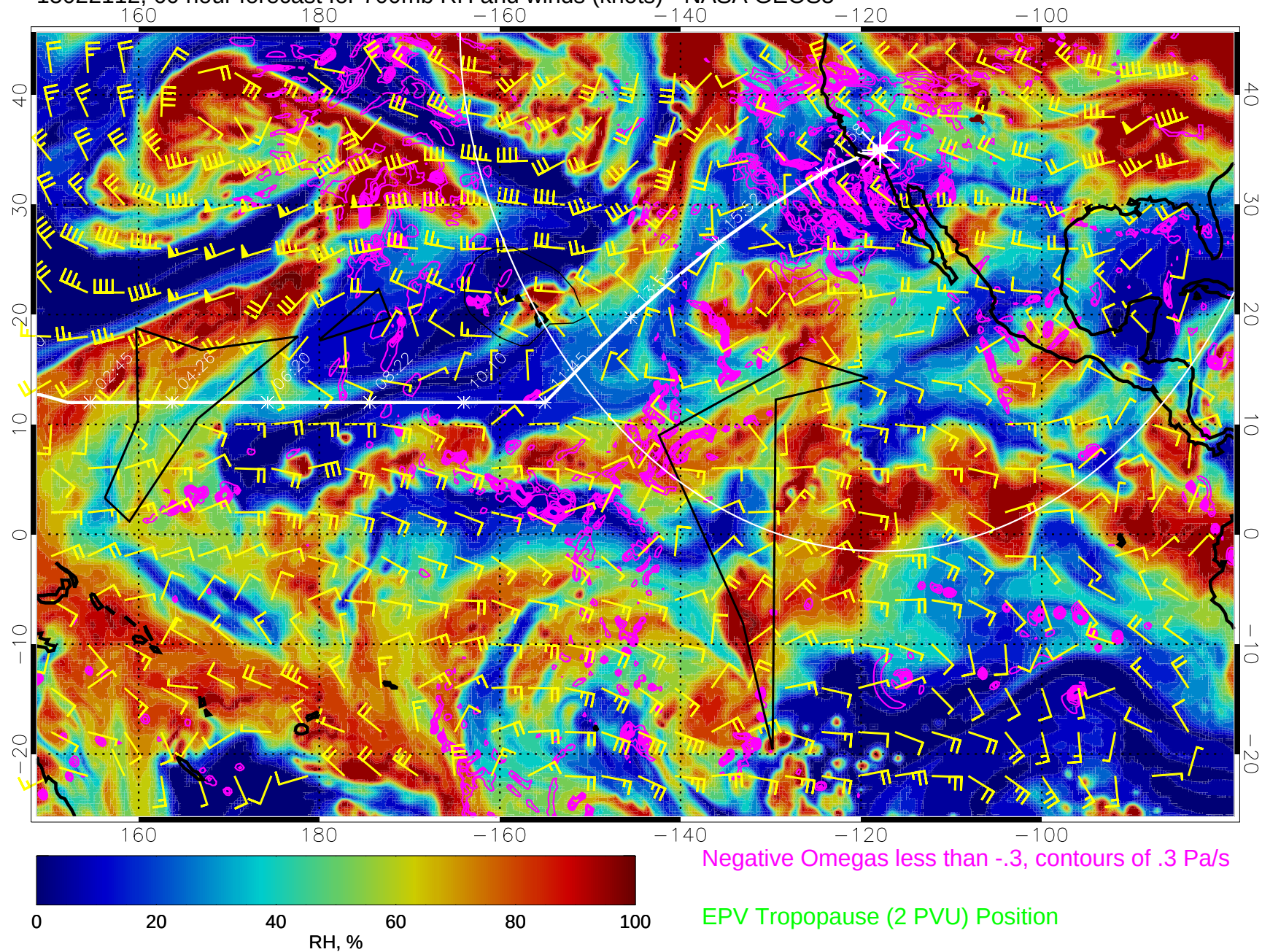
15022112, 60 hour forecast for 700mb RH and winds (knots) - NASA GEOS5
