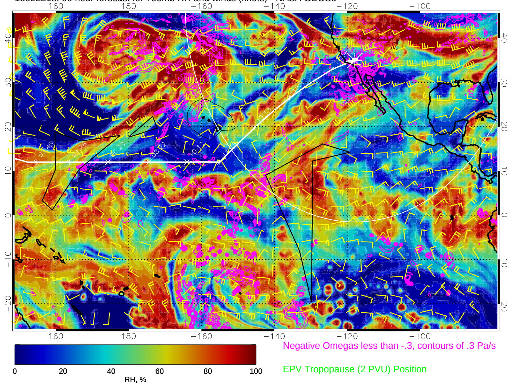
15022218, 90 hour forecast for 700mb RH and winds (knots) - NASA GEOS5
