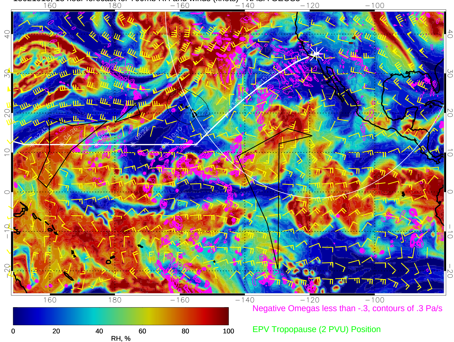
15021918, 18 hour forecast for 700mb RH and winds (knots) - NASA GEOS5
