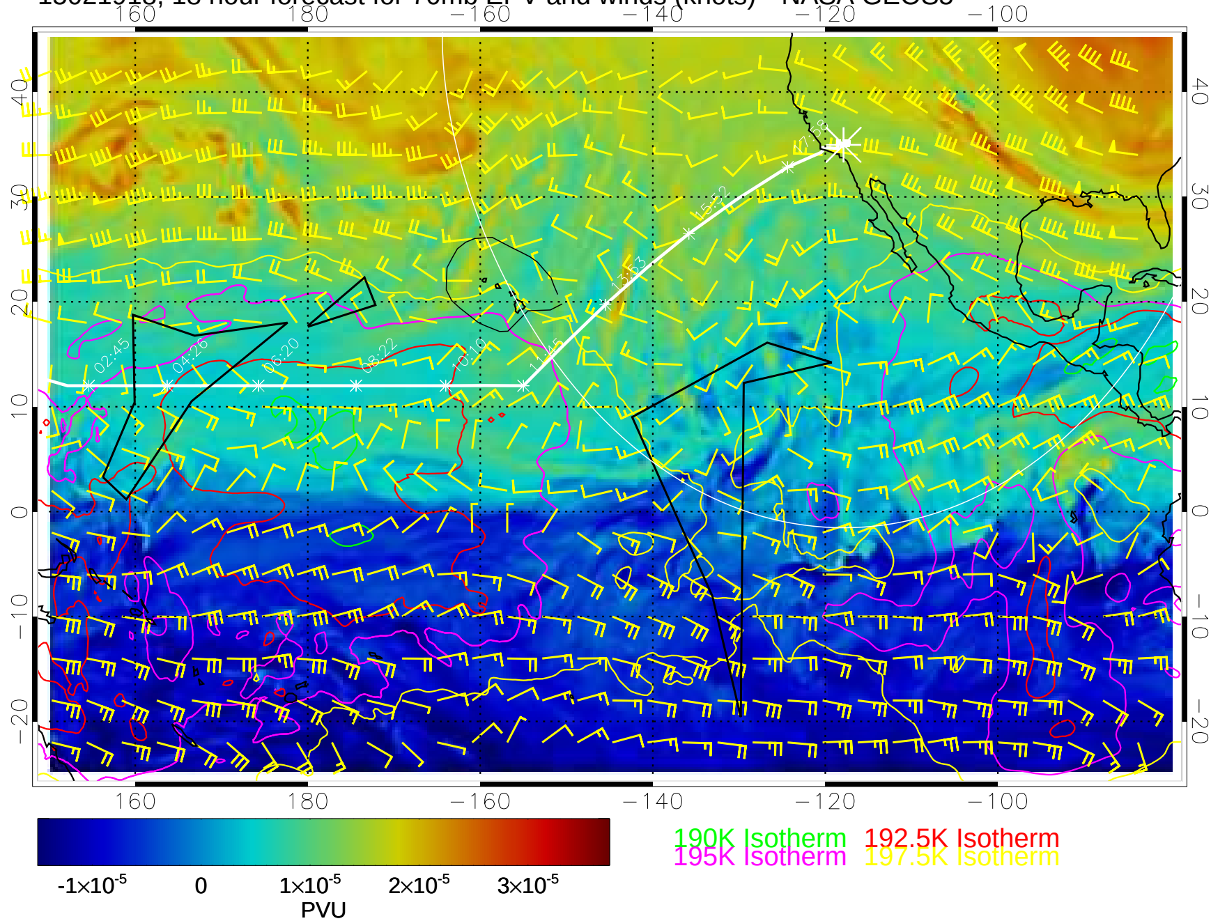
15021918, 18 hour forecast for 70mb EPV and winds (knots)-- NASA GEOS5
