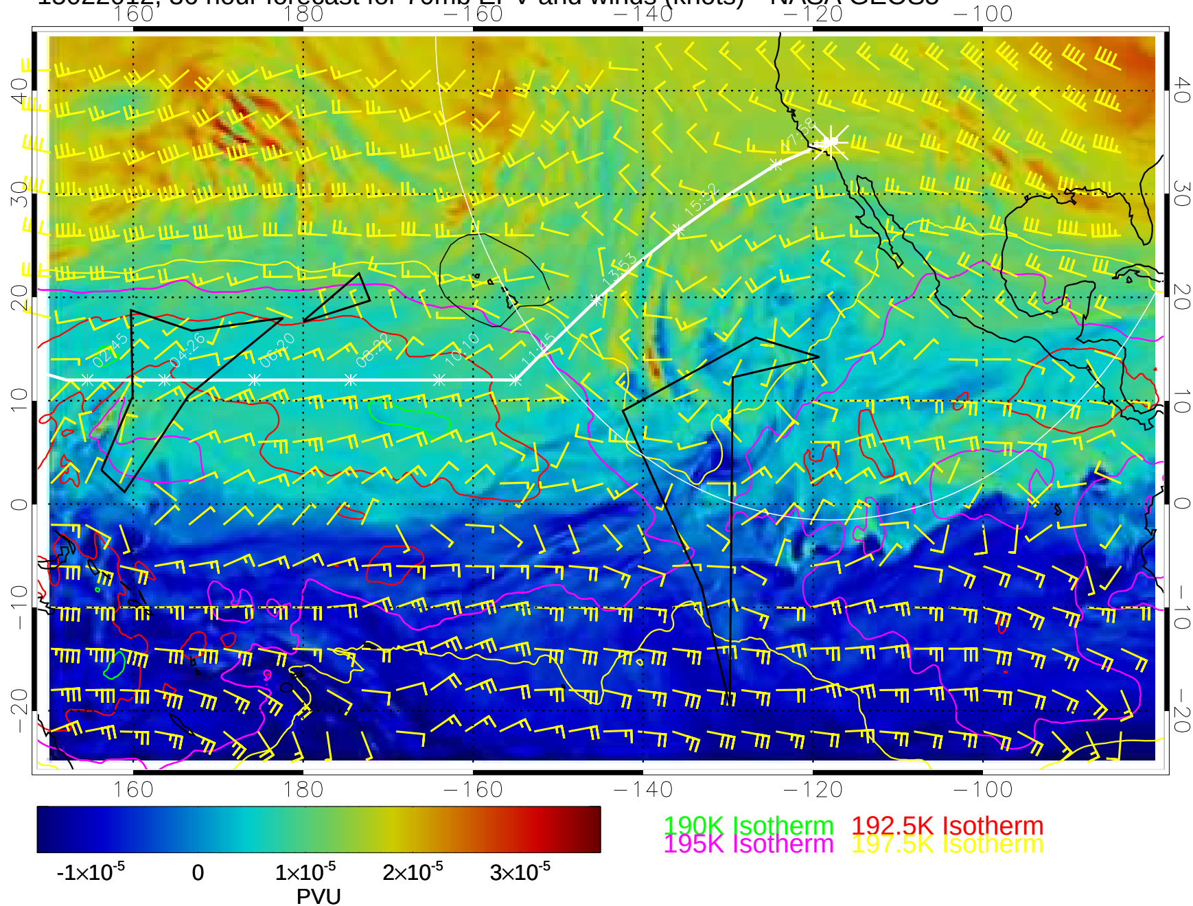
15022012, 36 hour forecast for 70mb EPV and winds (knots)-- NASA GEOS5
