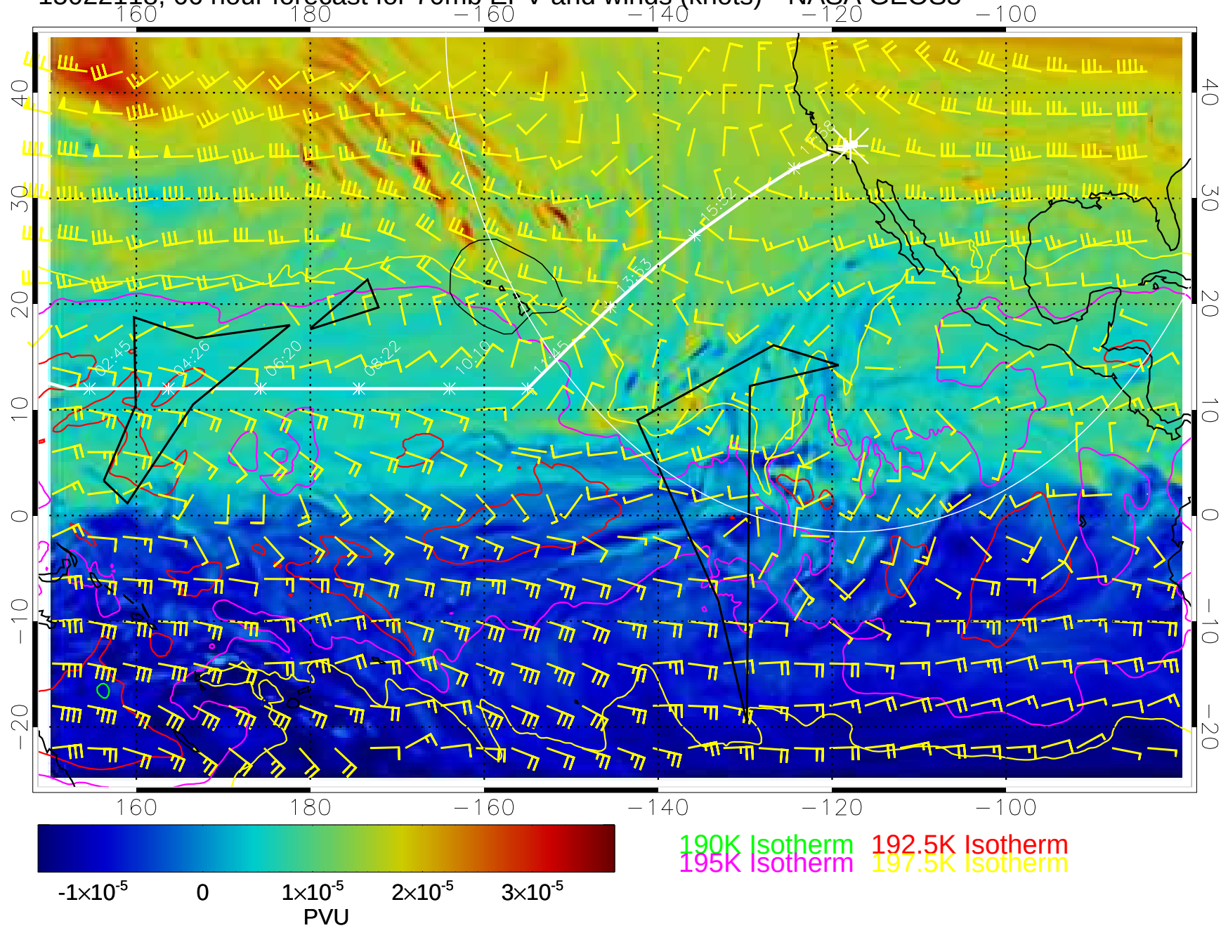
15022118, 66 hour forecast for 70mb EPV and winds (knots)-- NASA GEOS5
