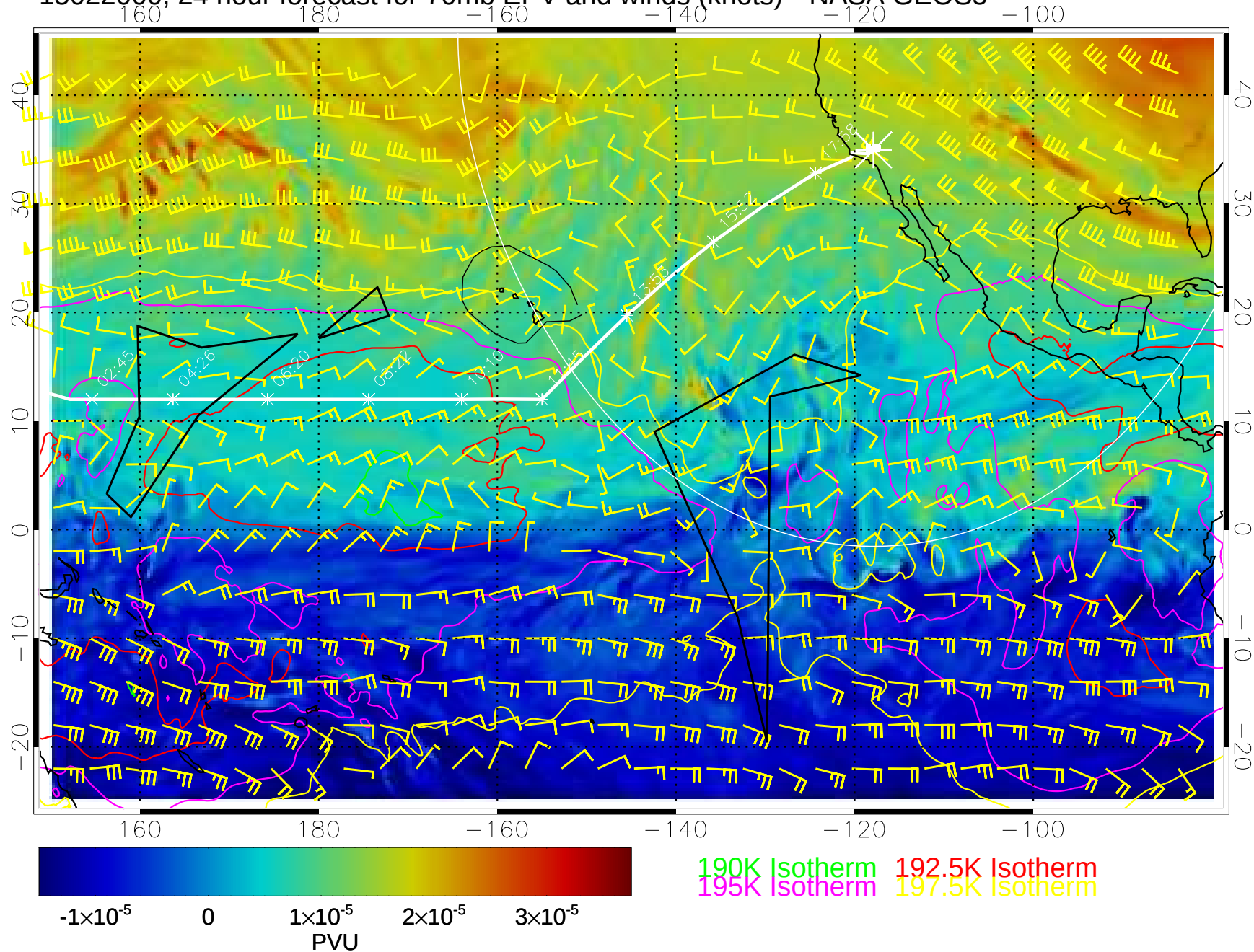
15022000, 24 hour forecast for 70mb EPV and winds (knots)-- NASA GEOS5
