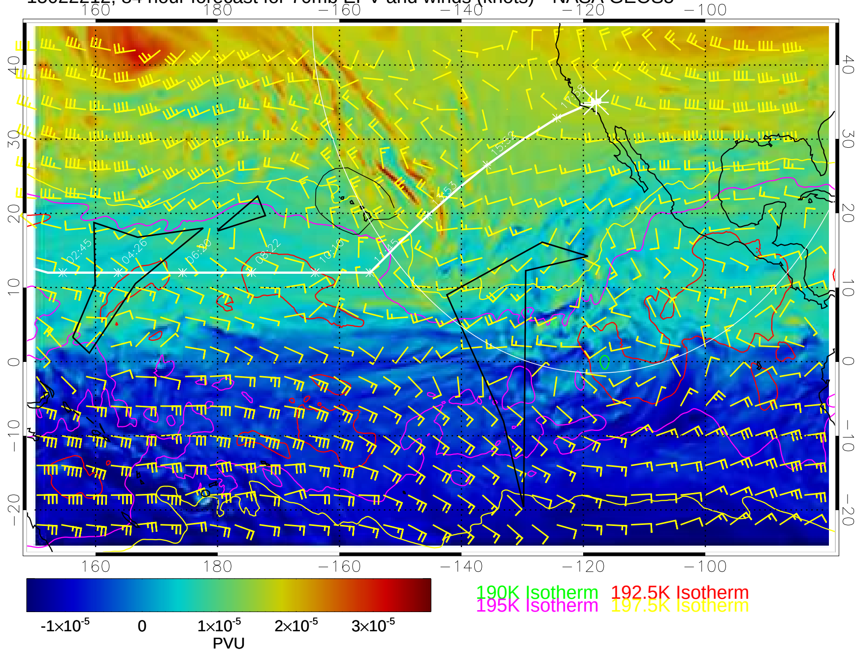
15022212, 84 hour forecast for 70mb EPV and winds (knots)-- NASA GEOS5
