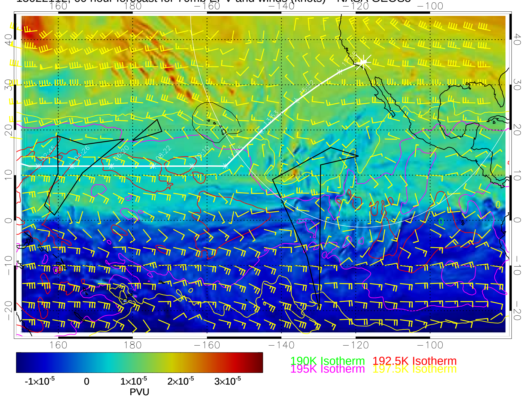
15022112, 60 hour forecast for 70mb EPV and winds (knots)-- NASA GEOS5
