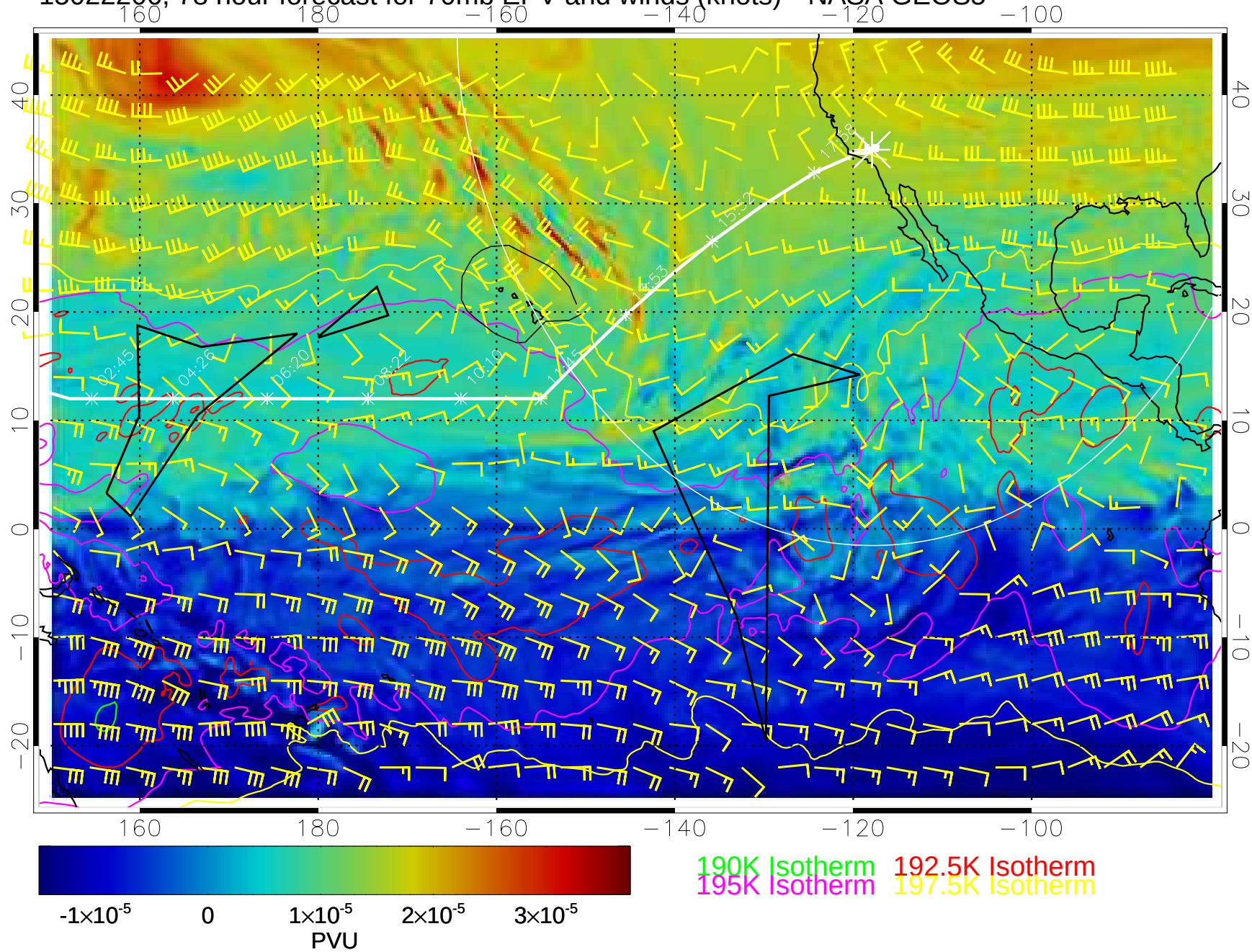
15022206, 78 hour forecast for 70mb EPV and winds (knots)-- NASA GEOS5
