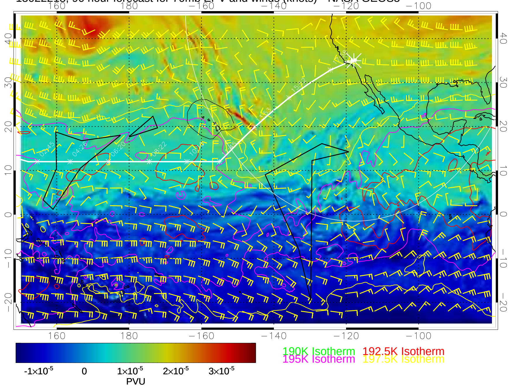
15022218, 90 hour forecast for 70mb EPV and winds (knots)-- NASA GEOS5
