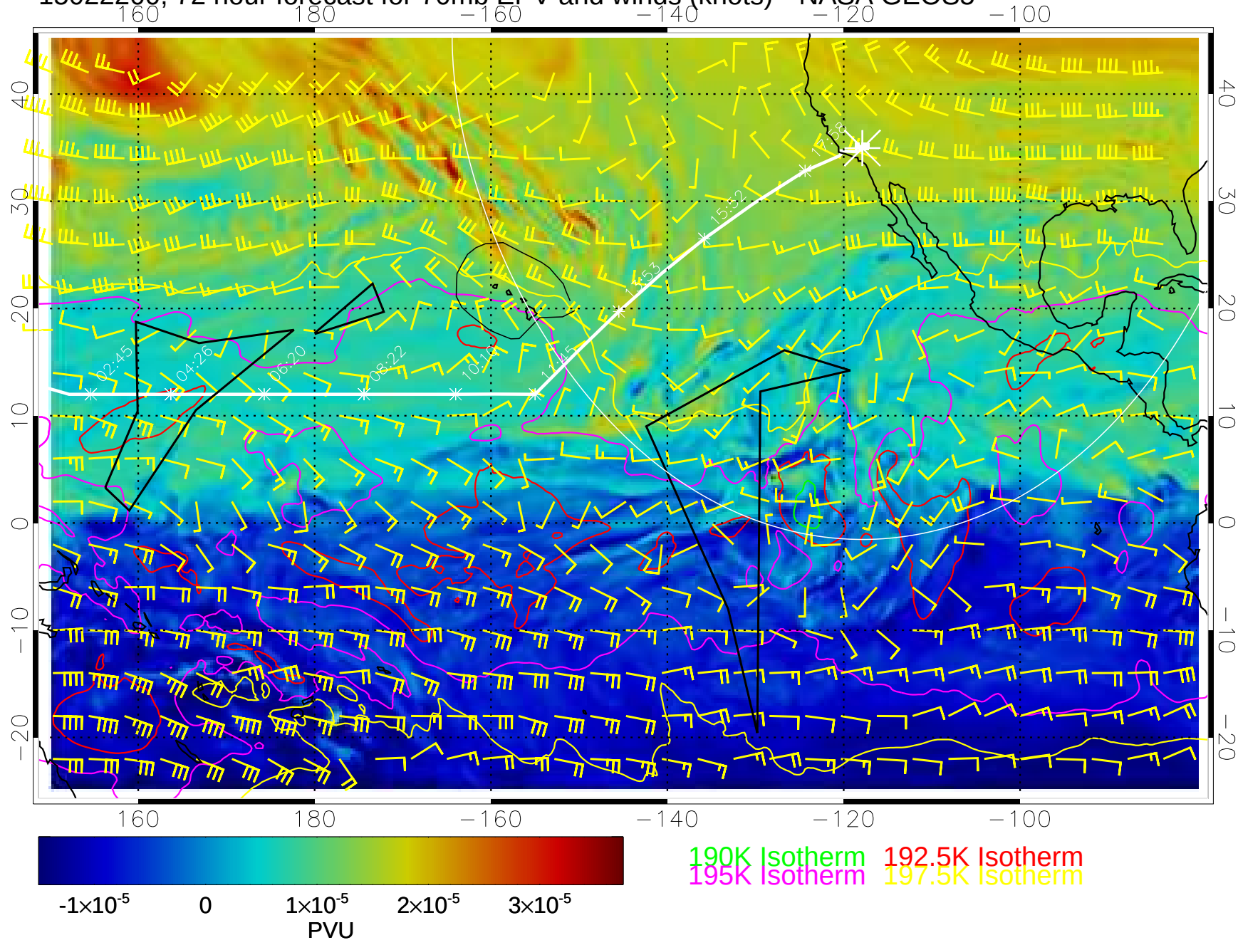
15022200, 72 hour forecast for 70mb EPV and winds (knots)-- NASA GEOS5
