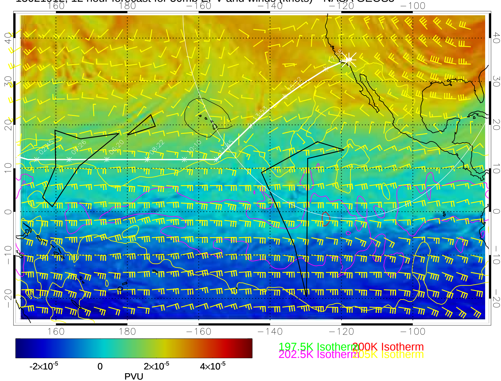
15021912, 12 hour forecast for 50mb EPV and winds (knots)-- NASA GEOS5
