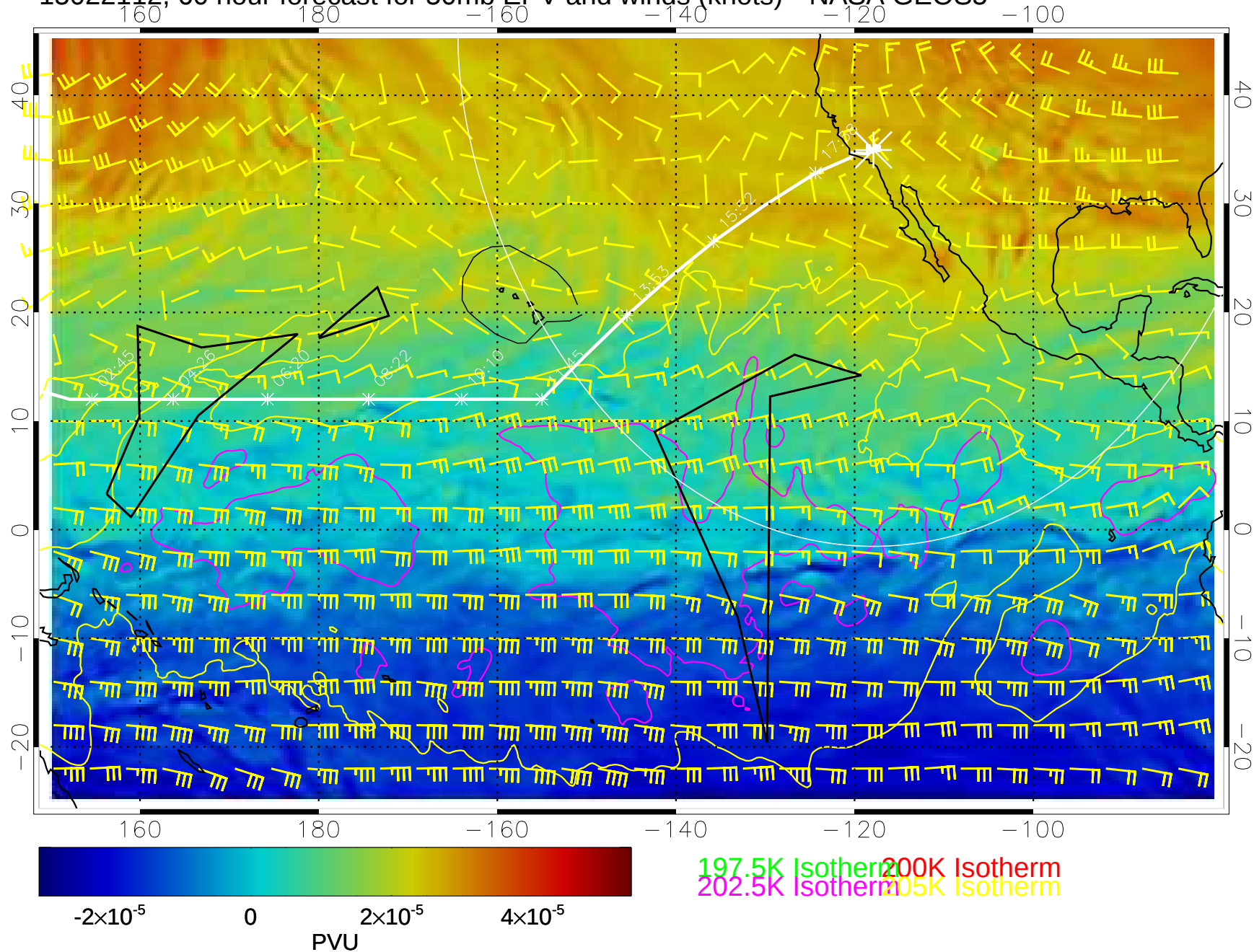
15022112, 60 hour forecast for 50mb EPV and winds (knots)-- NASA GEOS5
