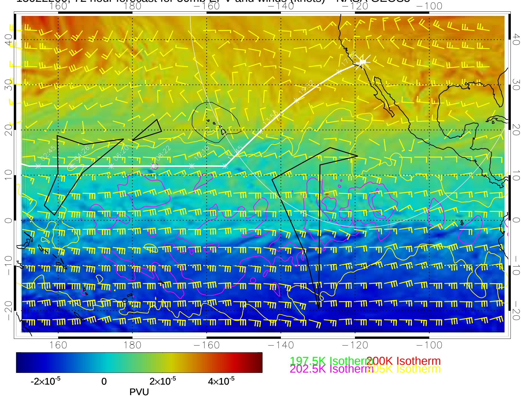
15022200, 72 hour forecast for 50mb EPV and winds (knots)-- NASA GEOS5
