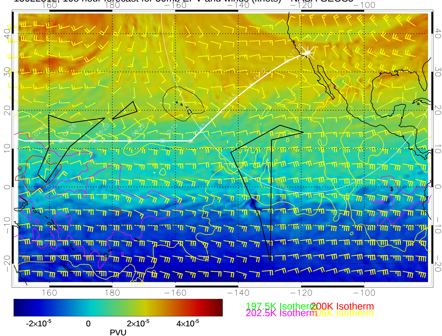
15022312, 108 hour forecast for 50mb EPV and winds (knots)-- NASA GEOS5
