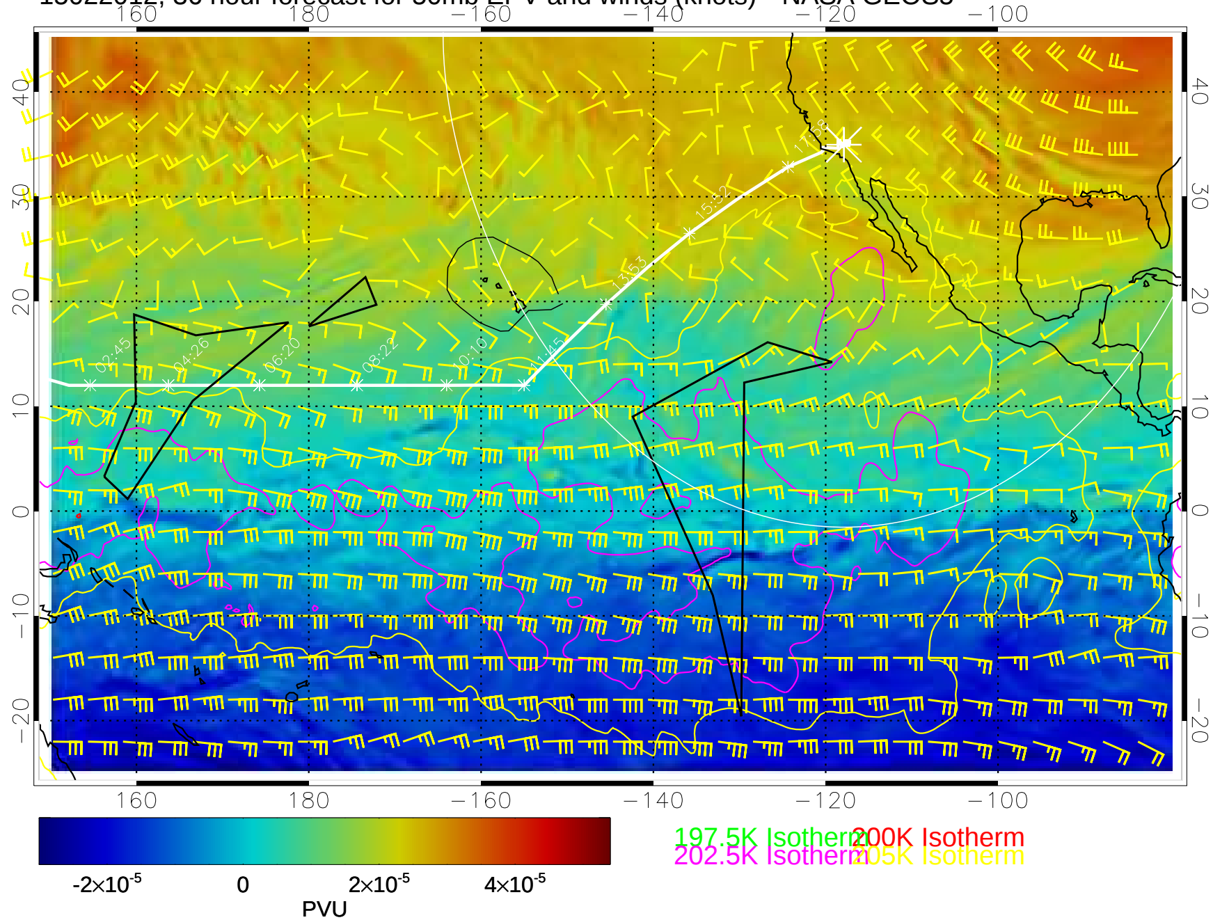
15022012, 36 hour forecast for 50mb EPV and winds (knots)-- NASA GEOS5
