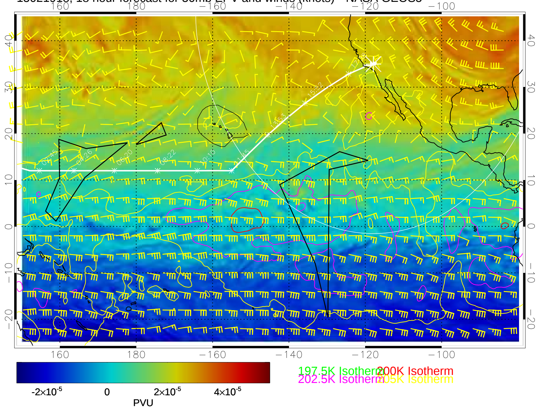
15021918, 18 hour forecast for 50mb EPV and winds (knots)-- NASA GEOS5
