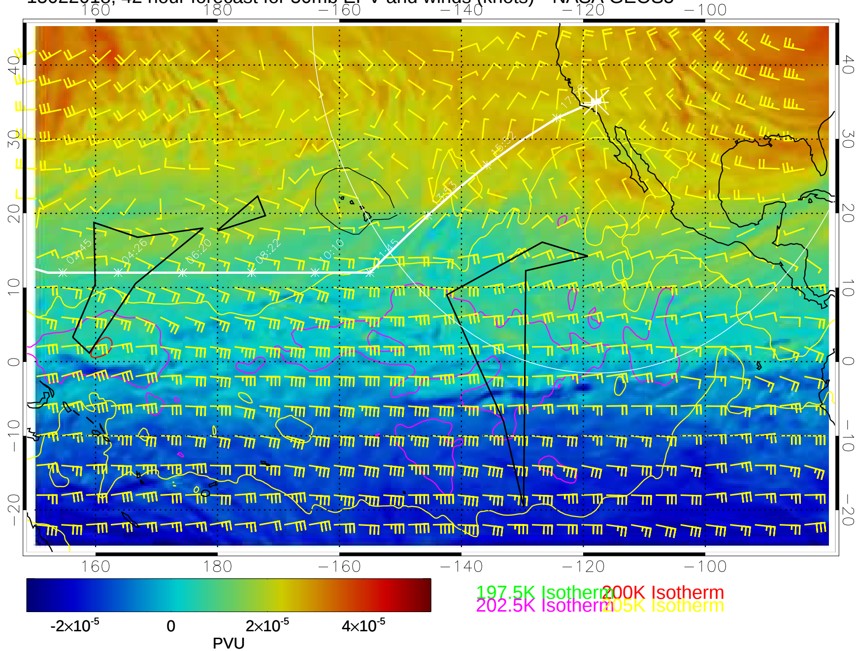
15022018, 42 hour forecast for 50mb EPV and winds (knots)-- NASA GEOS5
