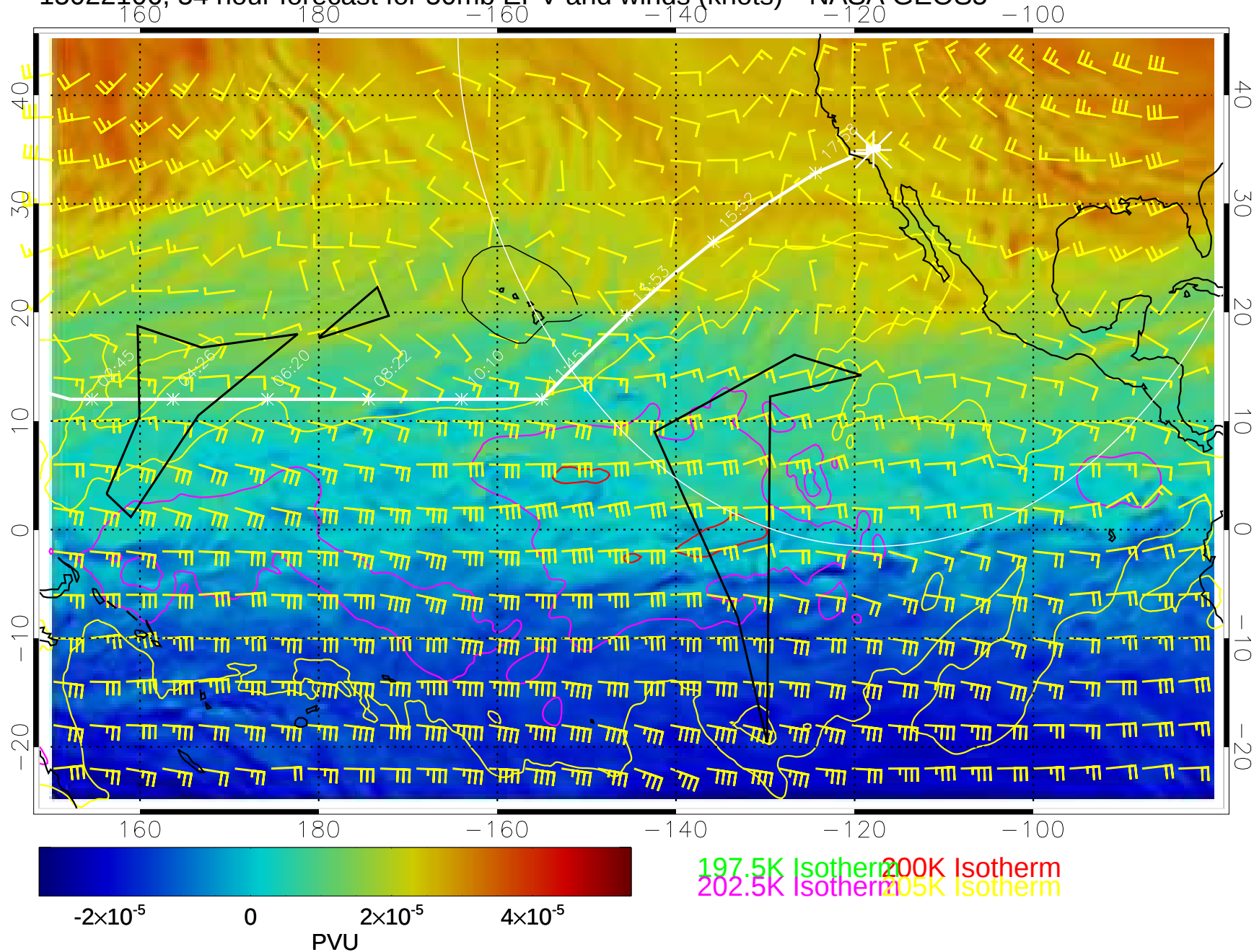
15022106, 54 hour forecast for 50mb EPV and winds (knots)-- NASA GEOS5
