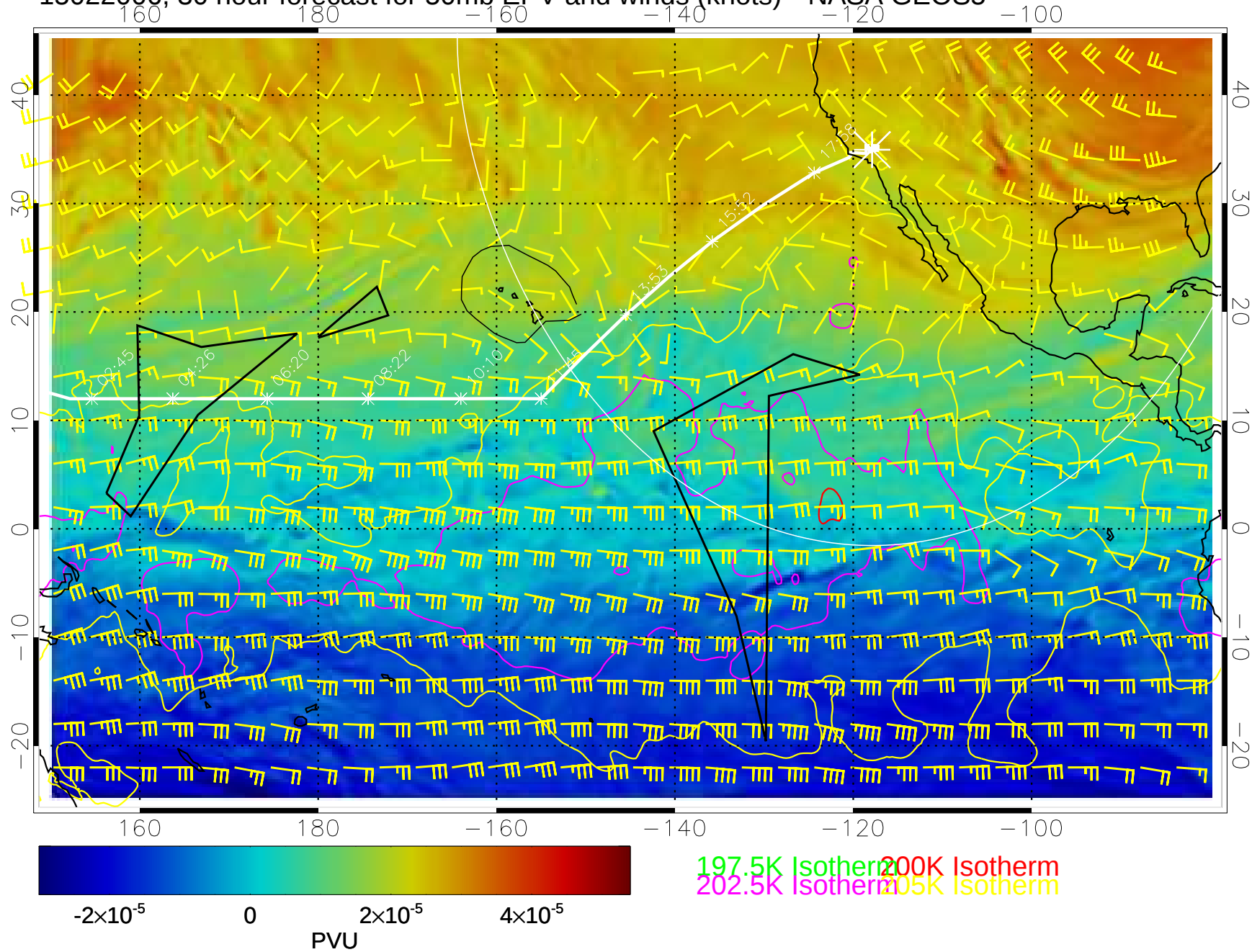
15022006, 30 hour forecast for 50mb EPV and winds (knots)-- NASA GEOS5
