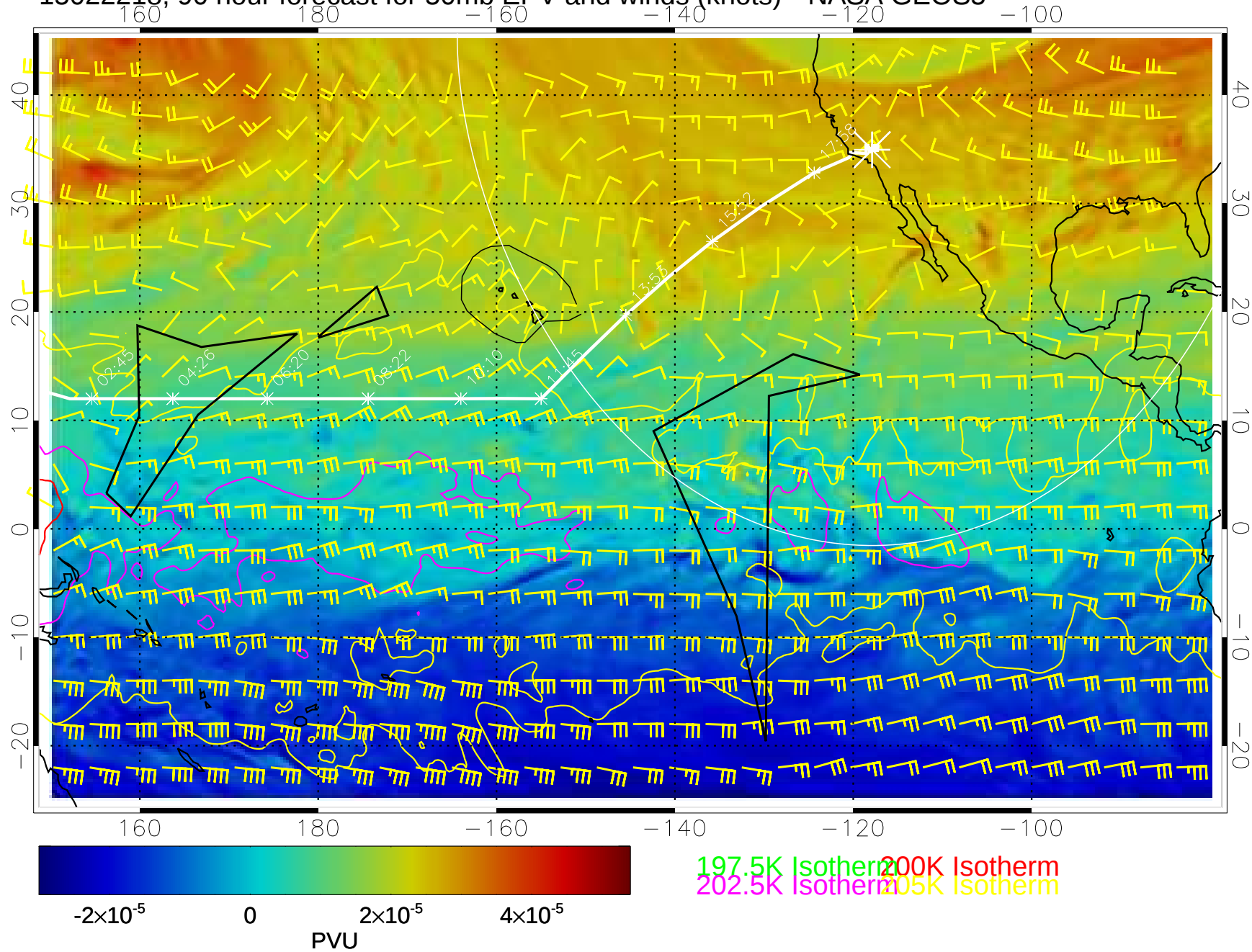
15022218, 90 hour forecast for 50mb EPV and winds (knots)-- NASA GEOS5
