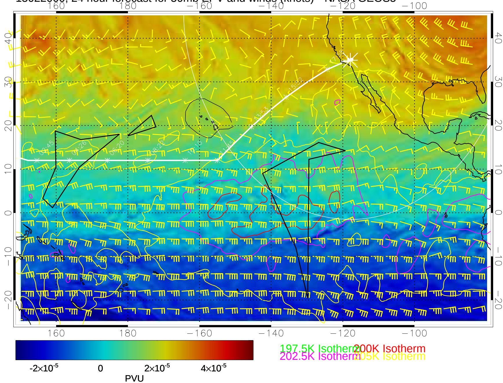
15022000, 24 hour forecast for 50mb EPV and winds (knots)-- NASA GEOS5
