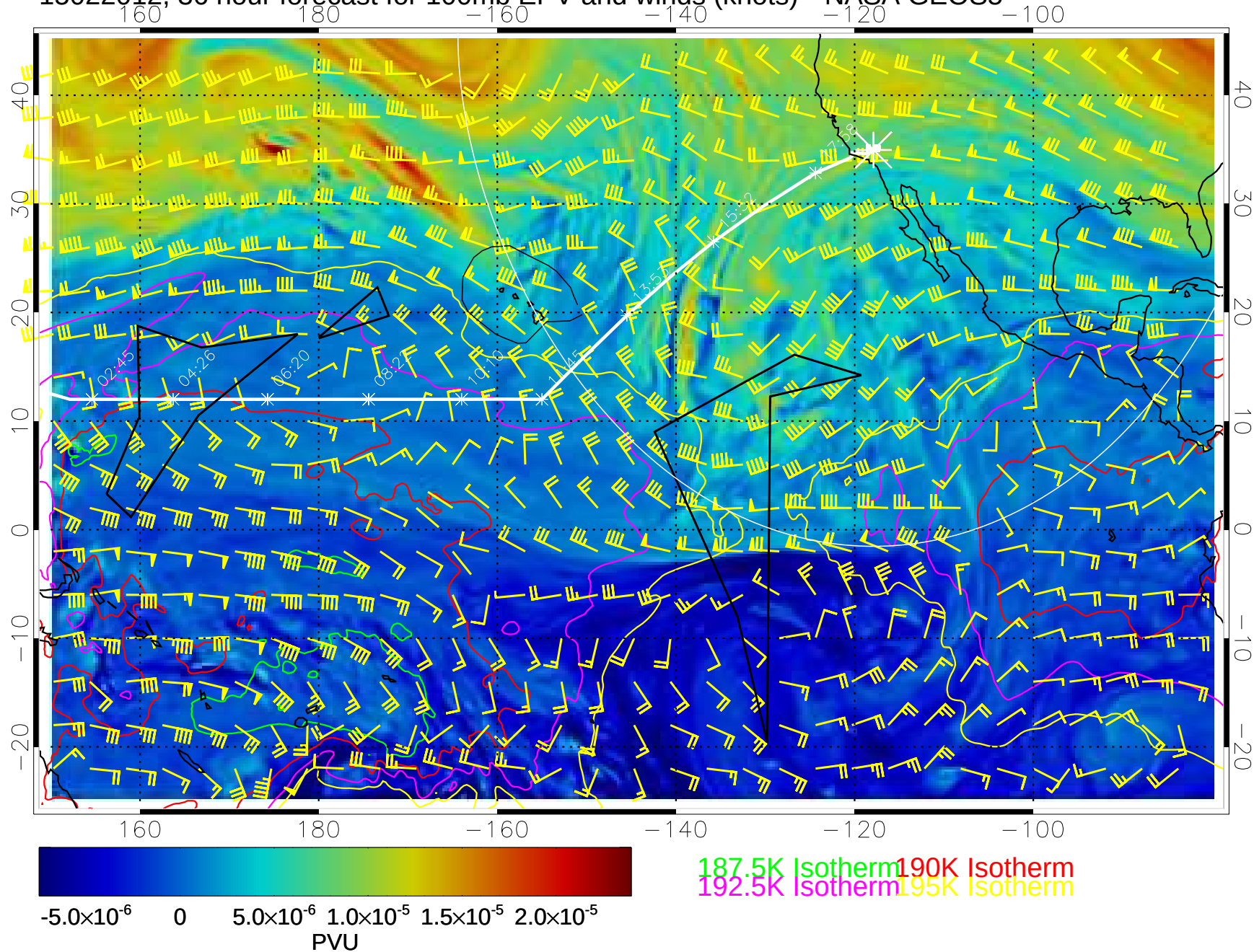
15022012, 36 hour forecast for 100mb EPV and winds (knots)-- NASA GEOS5
