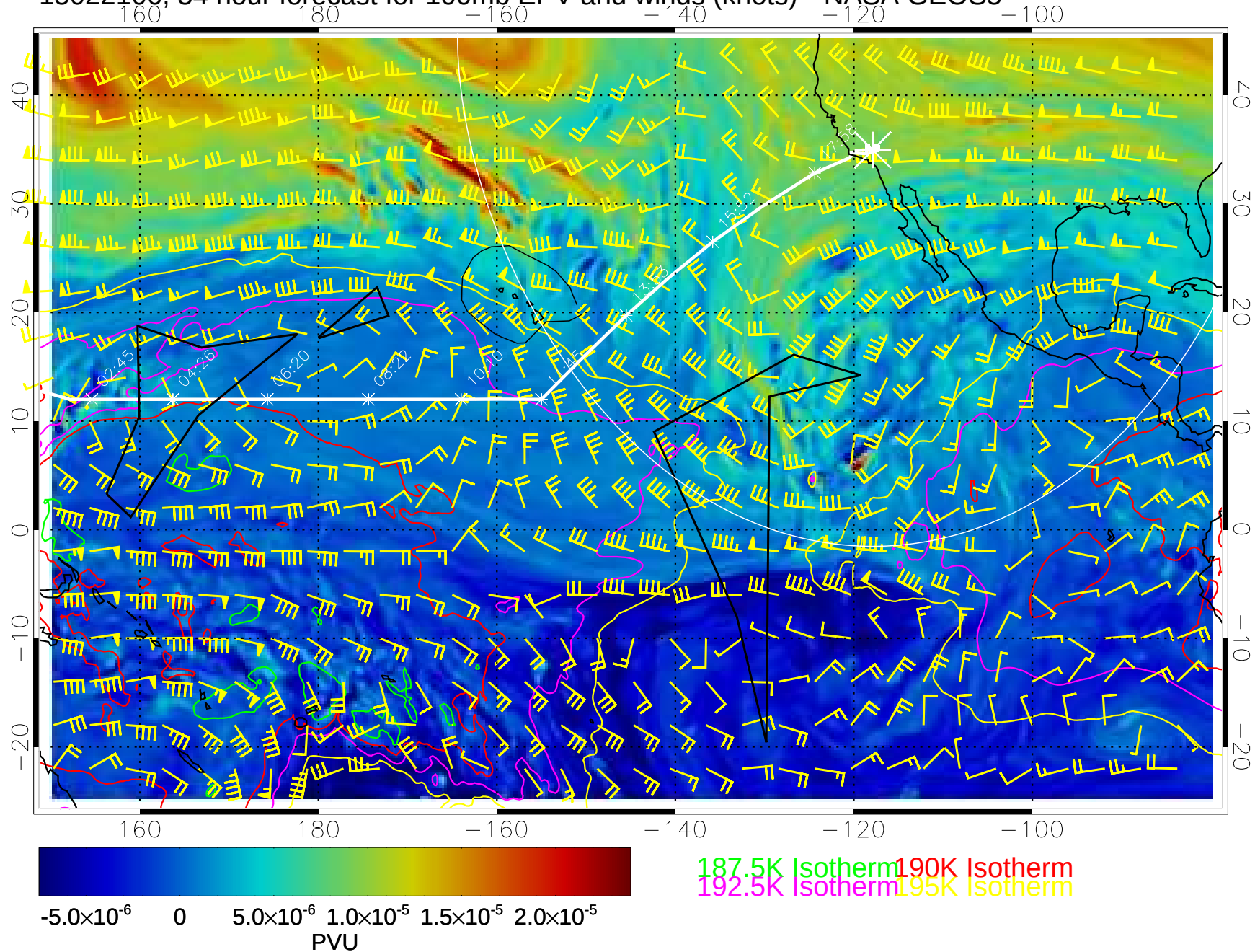
15022106, 54 hour forecast for 100mb EPV and winds (knots)-- NASA GEOS5
