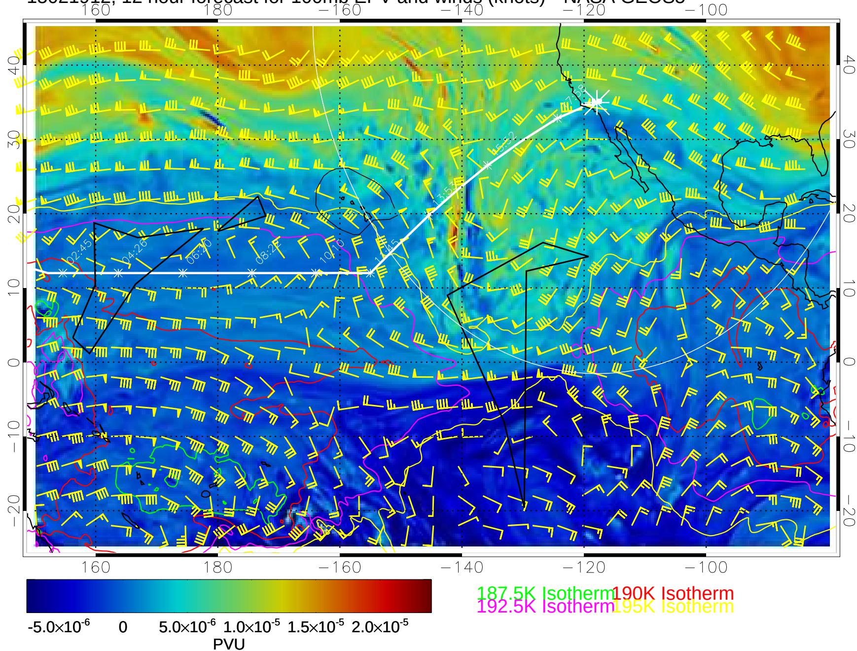
15021912, 12 hour forecast for 100mb EPV and winds (knots)-- NASA GEOS5
