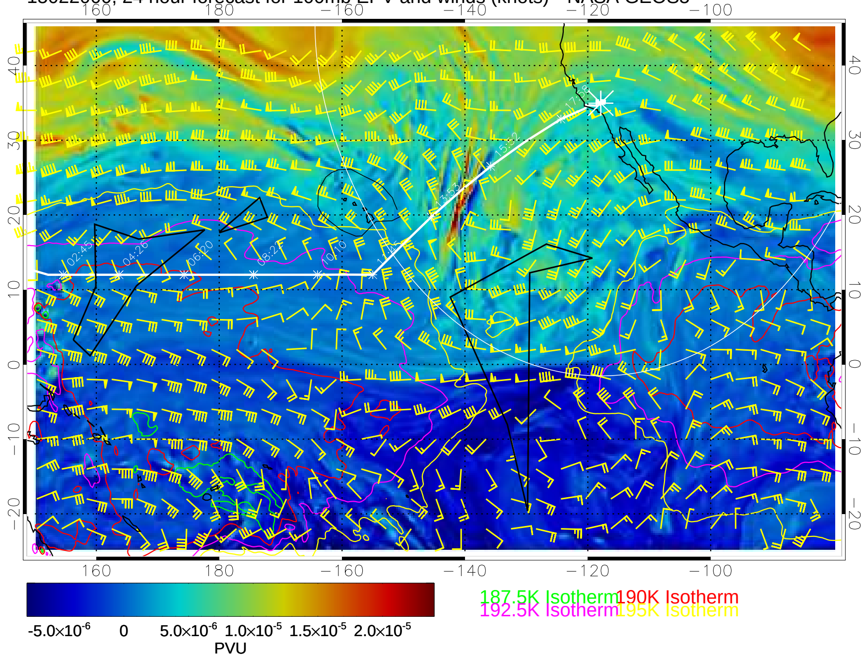
15022000, 24 hour forecast for 100mb EPV and winds (knots)-- NASA GEOS5
