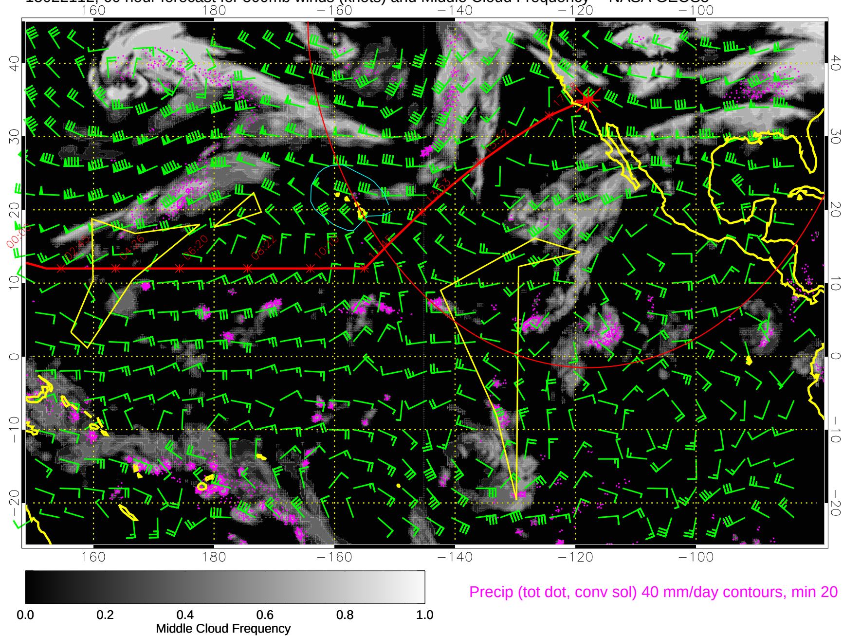
15022112, 60 hour forecast for 500mb winds (knots) and Middle Cloud Frequency -- NASA GEOS5
