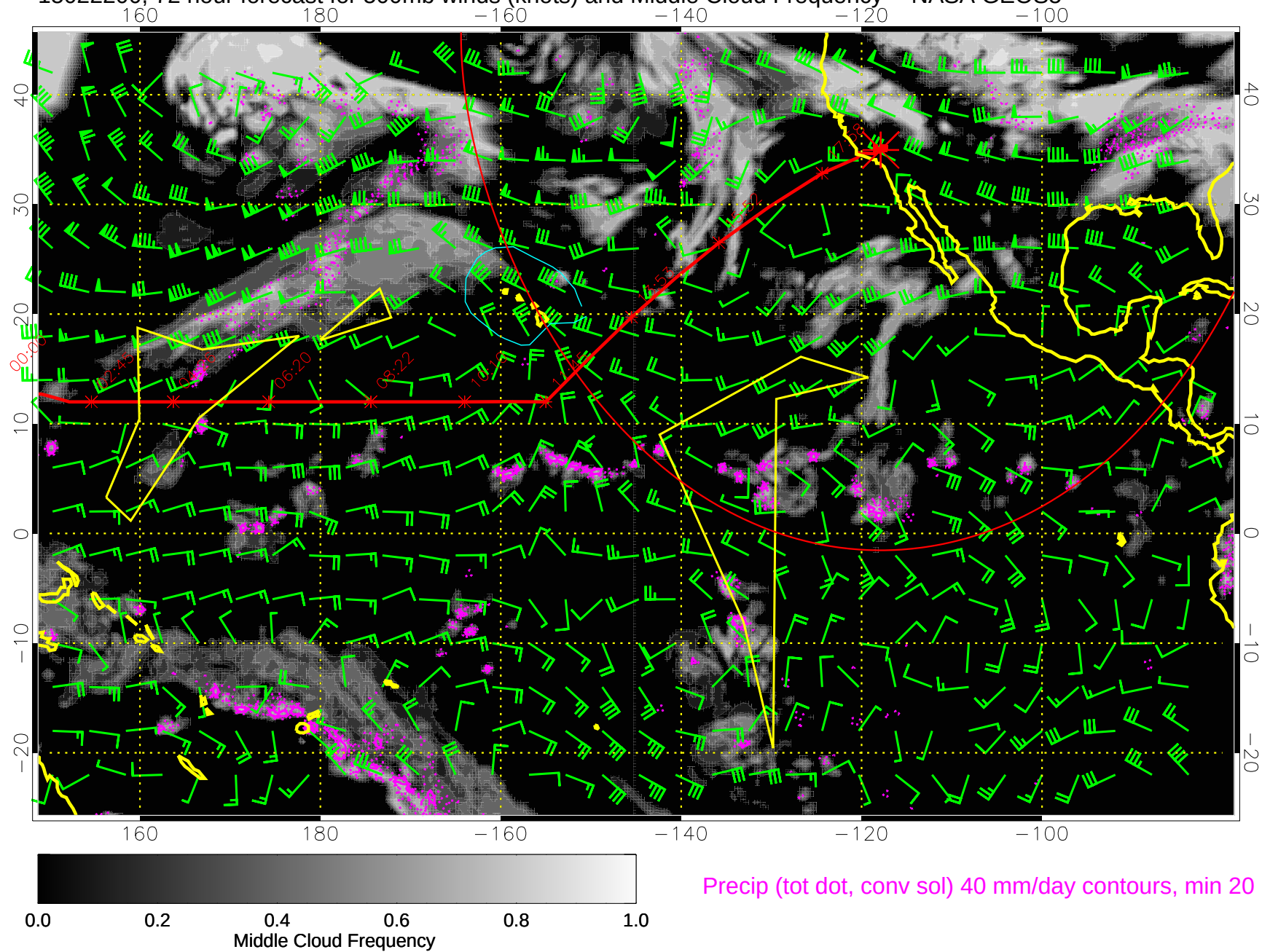
15022200, 72 hour forecast for 500mb winds (knots) and Middle Cloud Frequency -- NASA GEOS5
