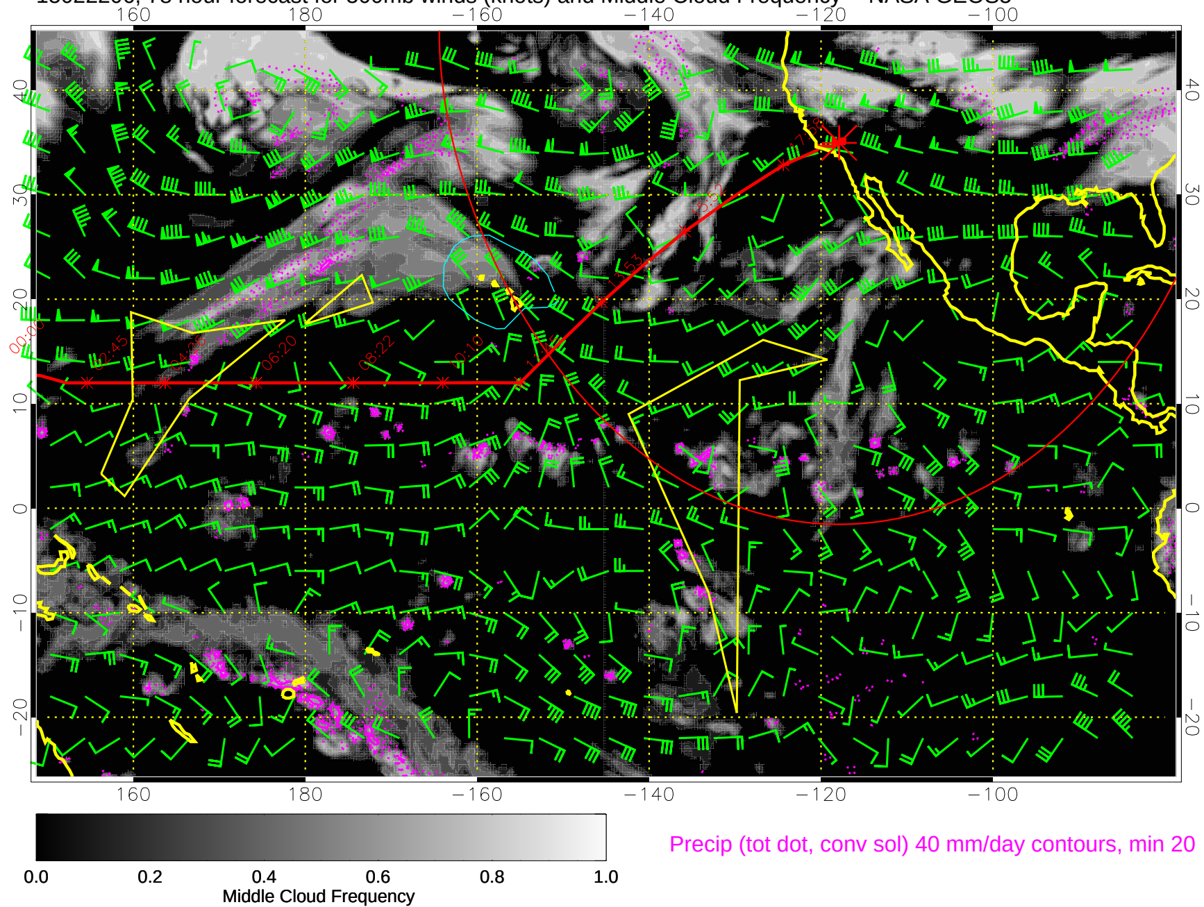
15022206, 78 hour forecast for 500mb winds (knots) and Middle Cloud Frequency -- NASA GEOS5
