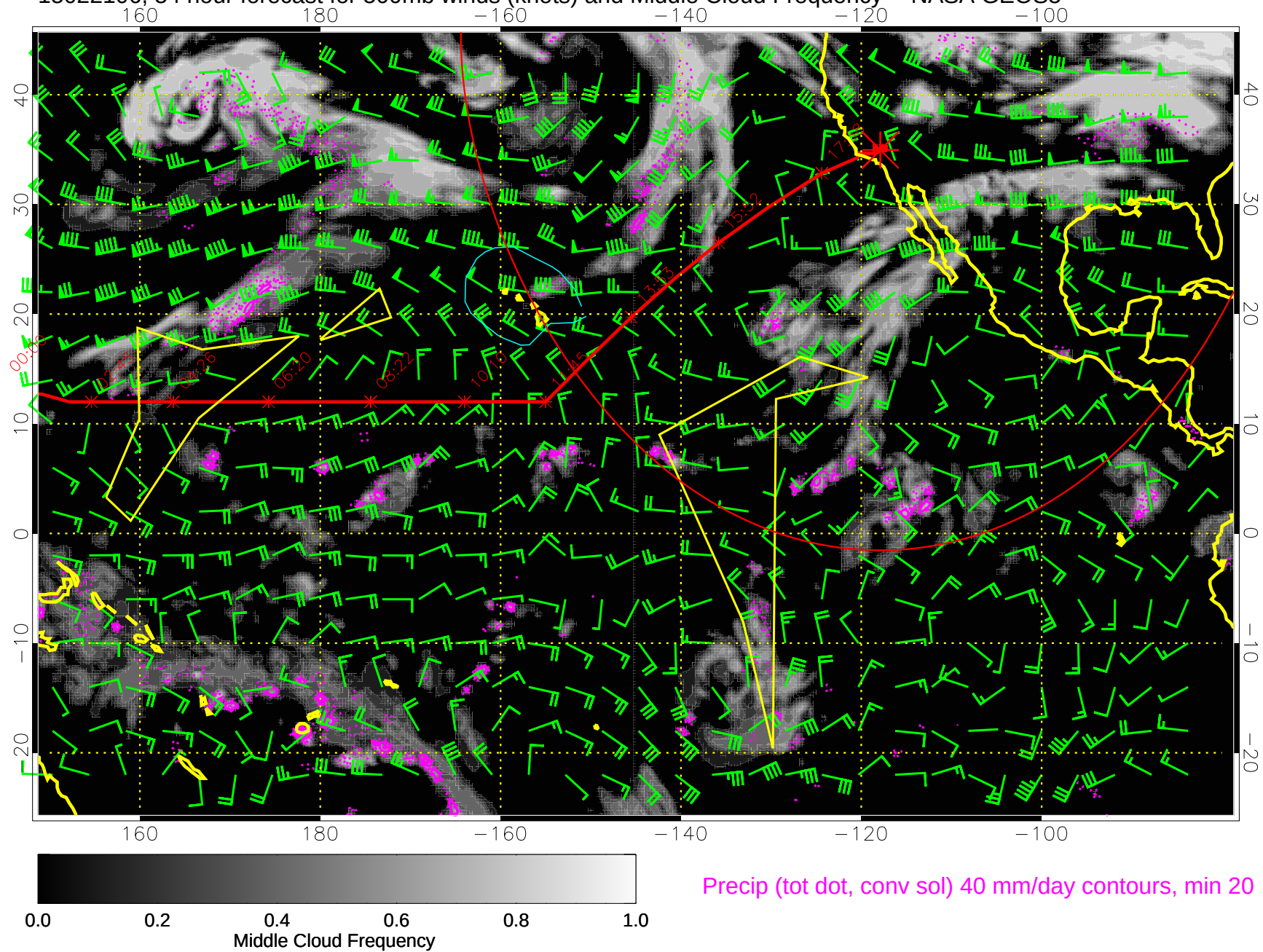
15022106, 54 hour forecast for 500mb winds (knots) and Middle Cloud Frequency -- NASA GEOS5
