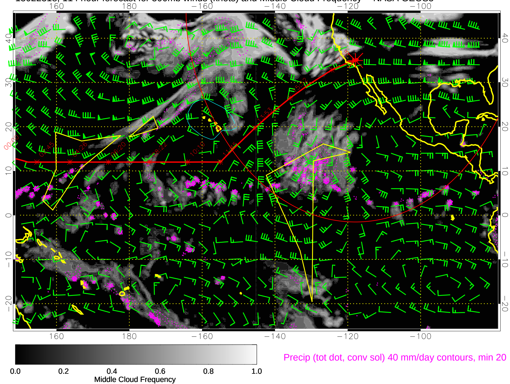
15022318, 114 hour forecast for 500mb winds (knots) and Middle Cloud Frequency -- NASA GEOS5
