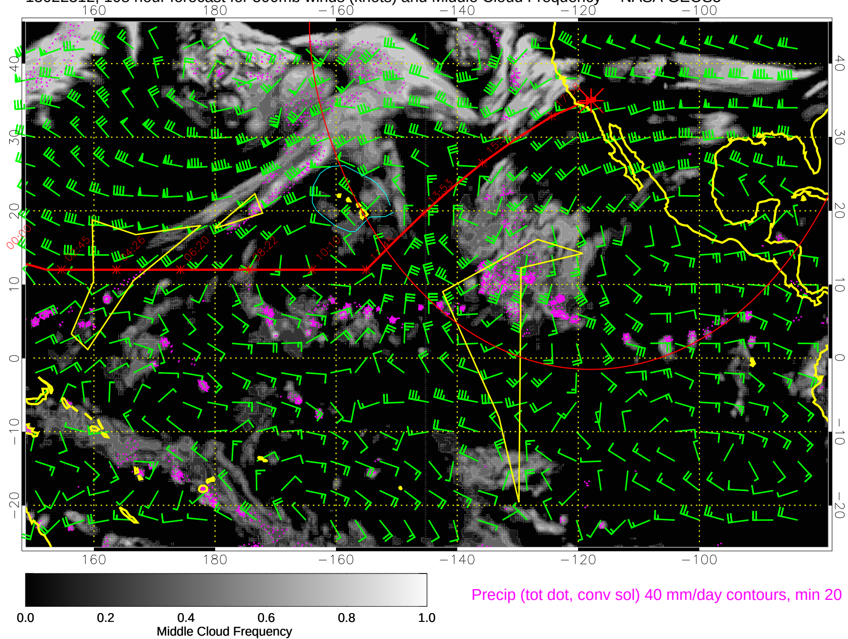
15022312, 108 hour forecast for 500mb winds (knots) and Middle Cloud Frequency -- NASA GEOS5
