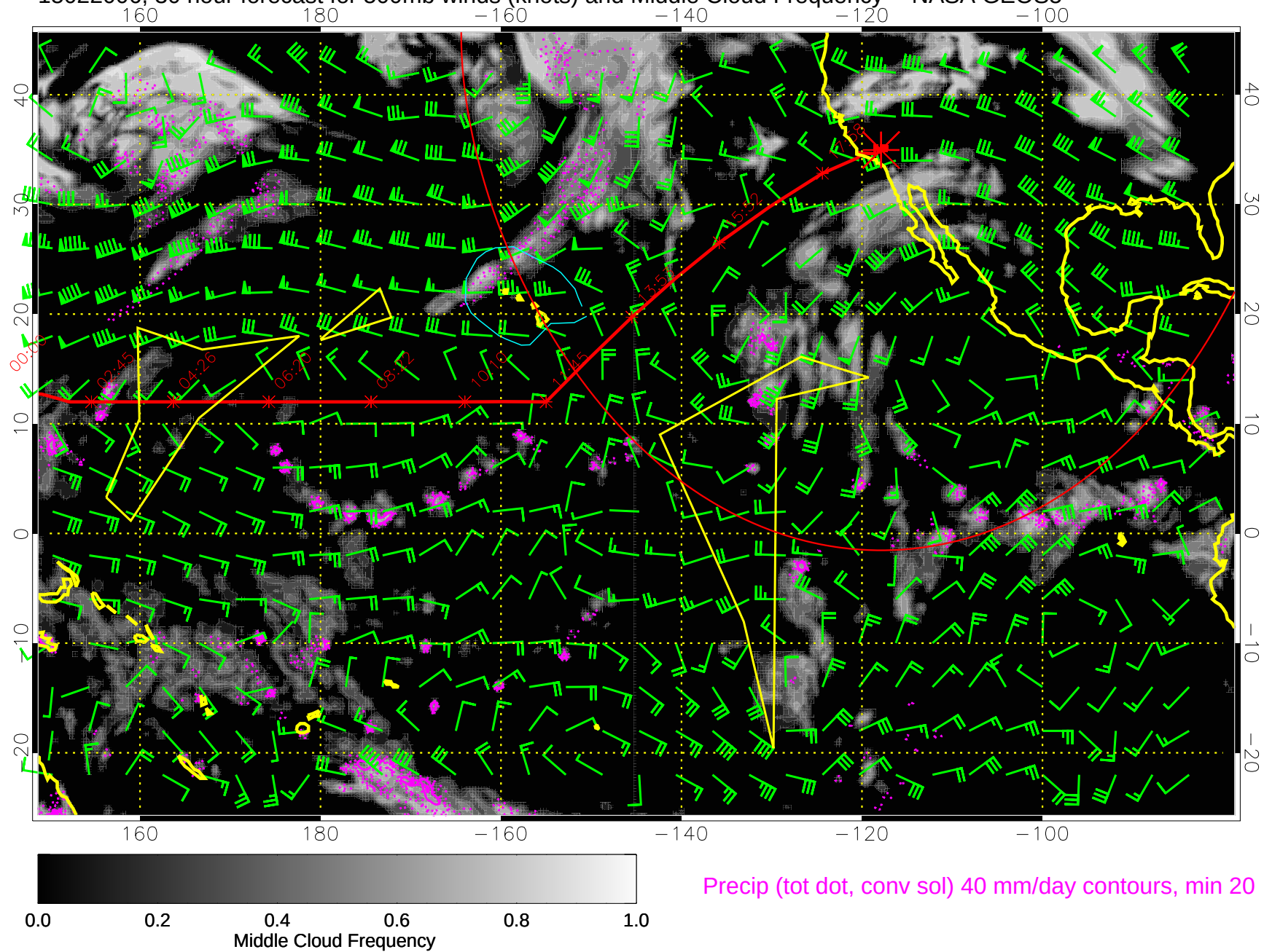
15022006, 30 hour forecast for 500mb winds (knots) and Middle Cloud Frequency -- NASA GEOS5
