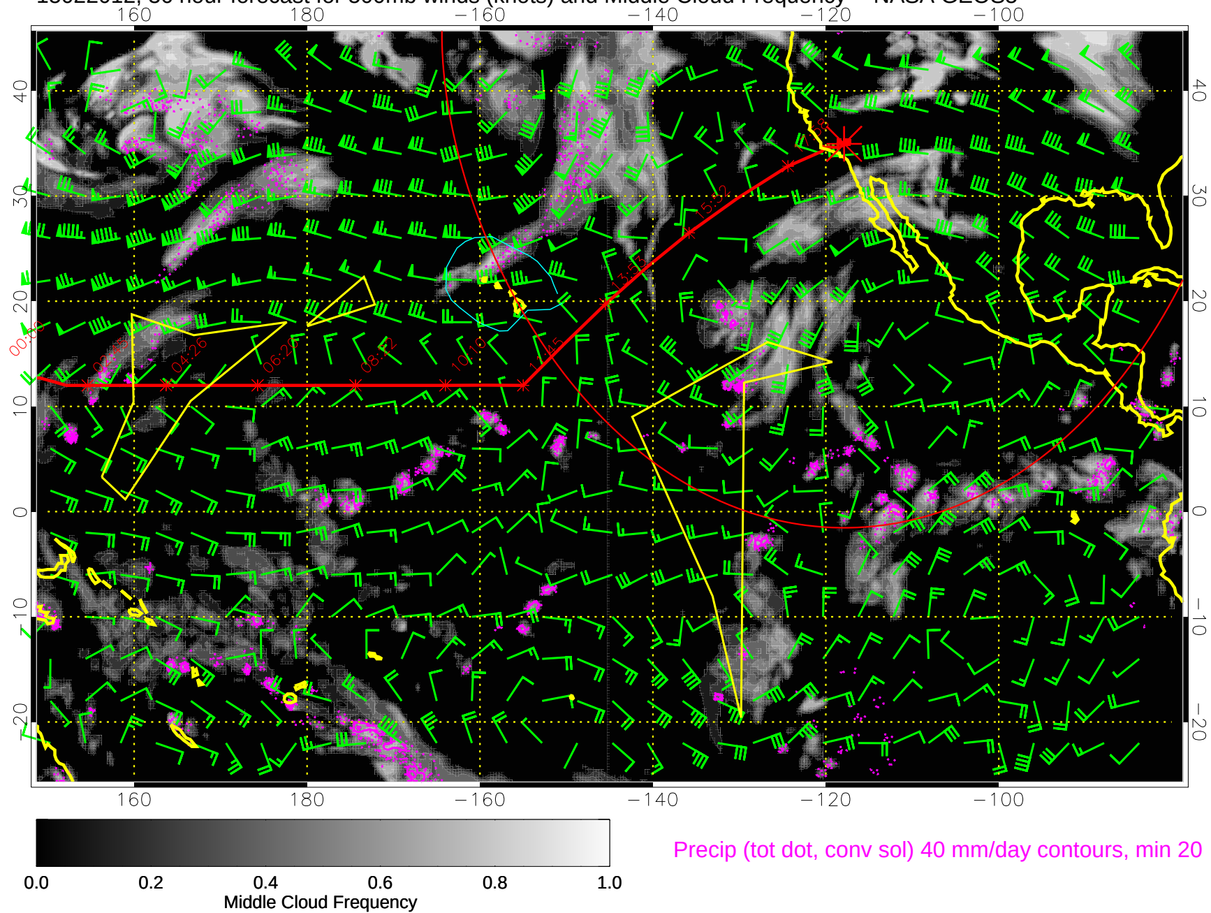
15022012, 36 hour forecast for 500mb winds (knots) and Middle Cloud Frequency -- NASA GEOS5
