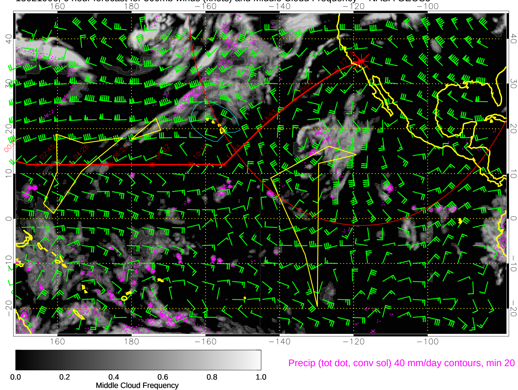
15021906, 6 hour forecast for 500mb winds (knots) and Middle Cloud Frequency -- NASA GEOS5
