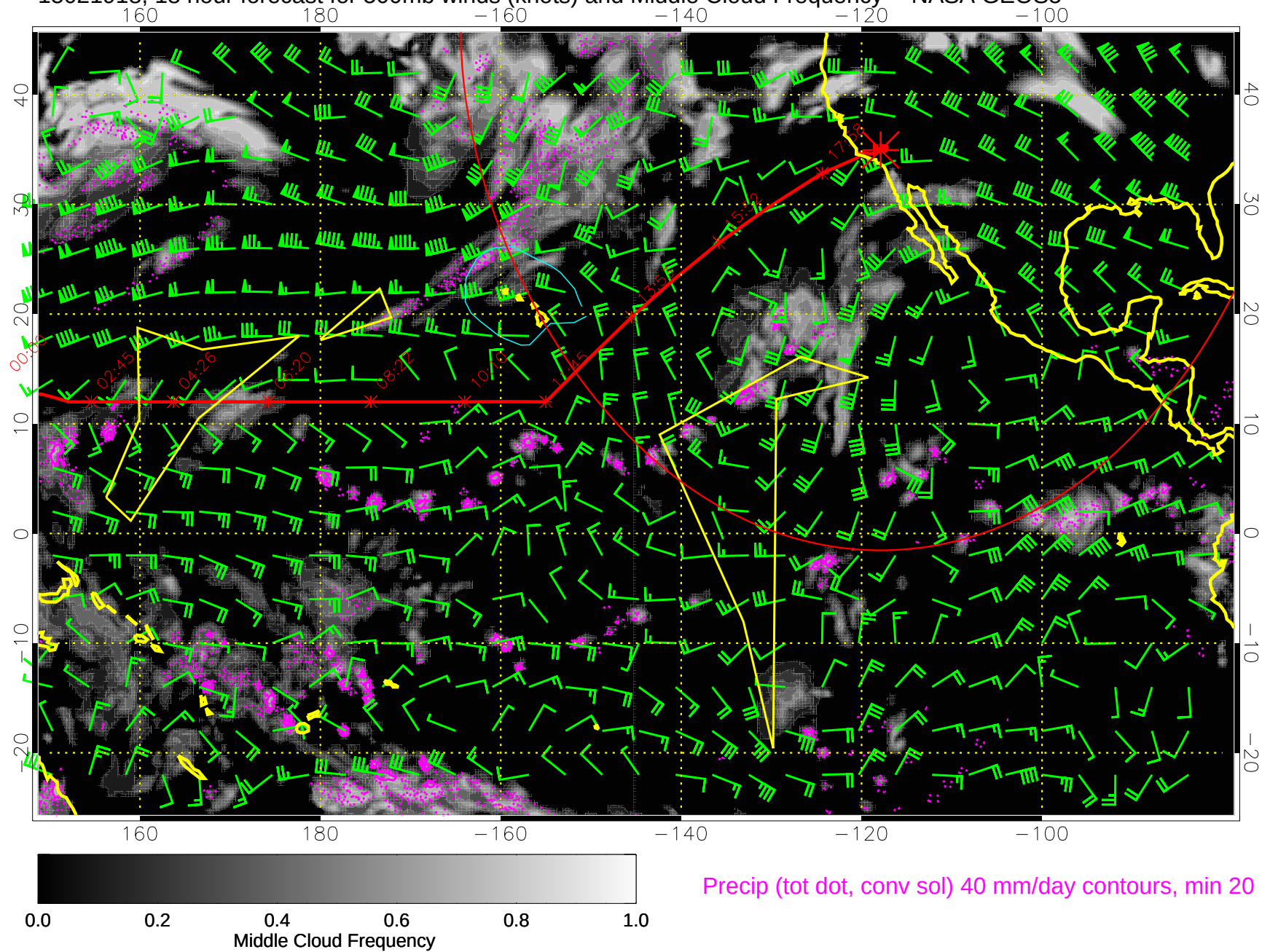
15021918, 18 hour forecast for 500mb winds (knots) and Middle Cloud Frequency -- NASA GEOS5
