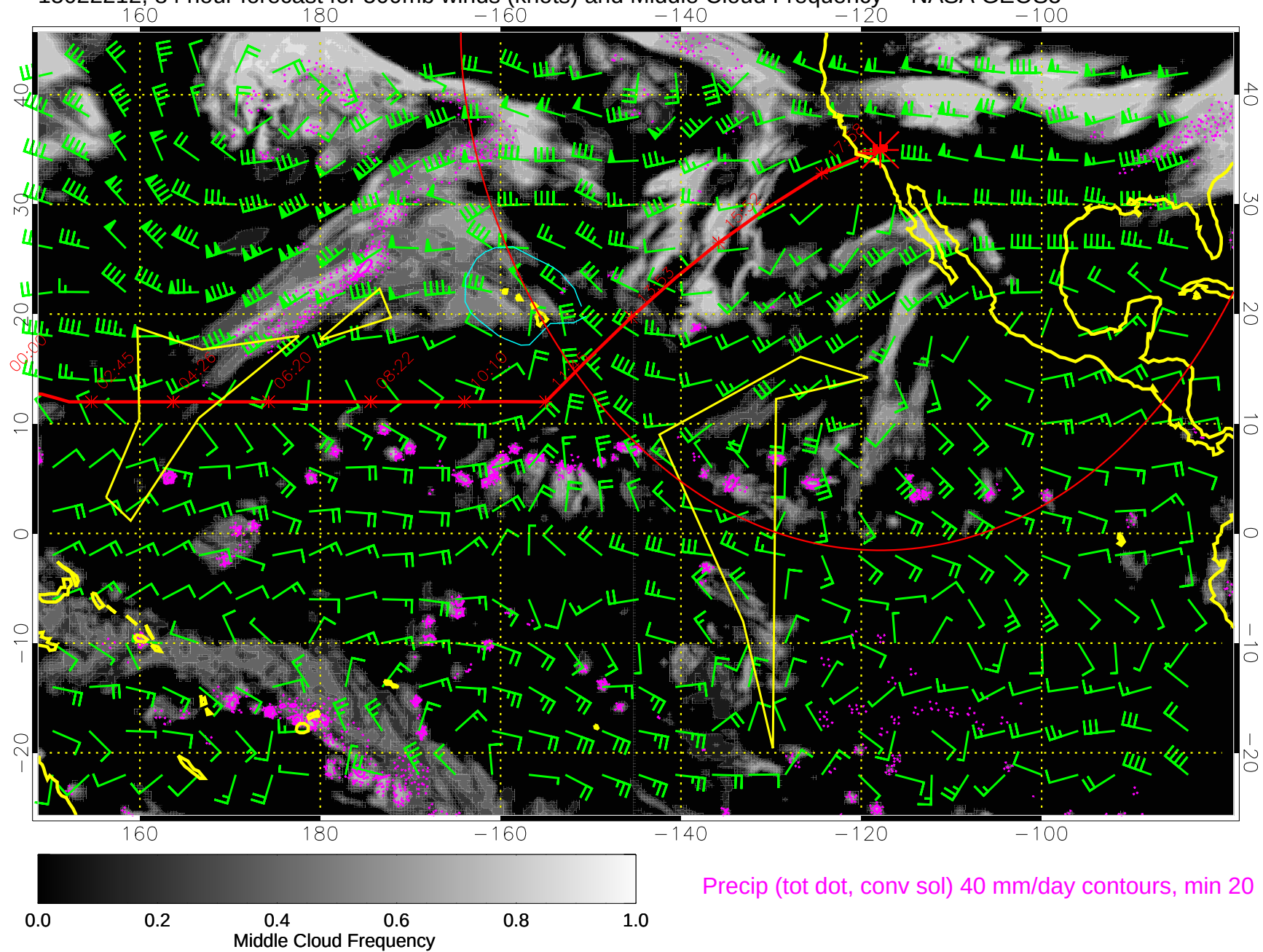
15022212, 84 hour forecast for 500mb winds (knots) and Middle Cloud Frequency -- NASA GEOS5
