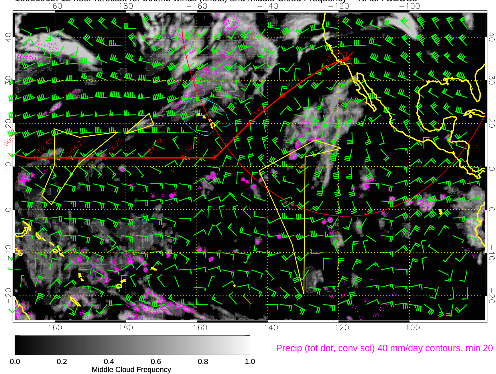
15021912, 12 hour forecast for 500mb winds (knots) and Middle Cloud Frequency -- NASA GEOS5
