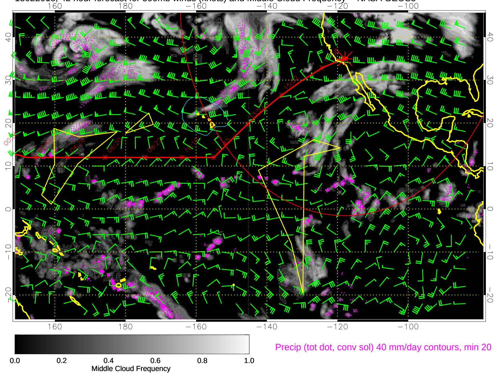
15022018, 42 hour forecast for 500mb winds (knots) and Middle Cloud Frequency -- NASA GEOS5
