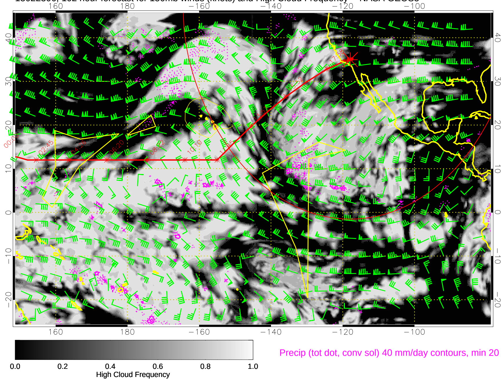
15022306, 102 hour forecast for 150mb winds (knots) and High Cloud Frequency -- NASA GEOS5
