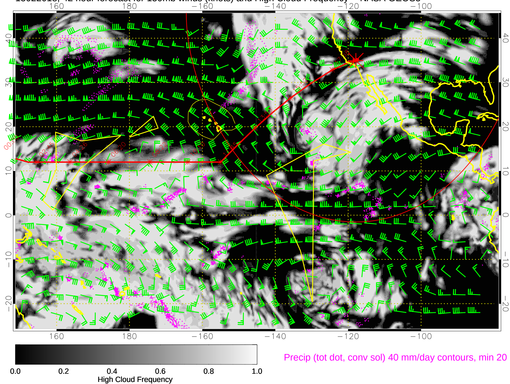
15022018, 42 hour forecast for 150mb winds (knots) and High Cloud Frequency -- NASA GEOS5
