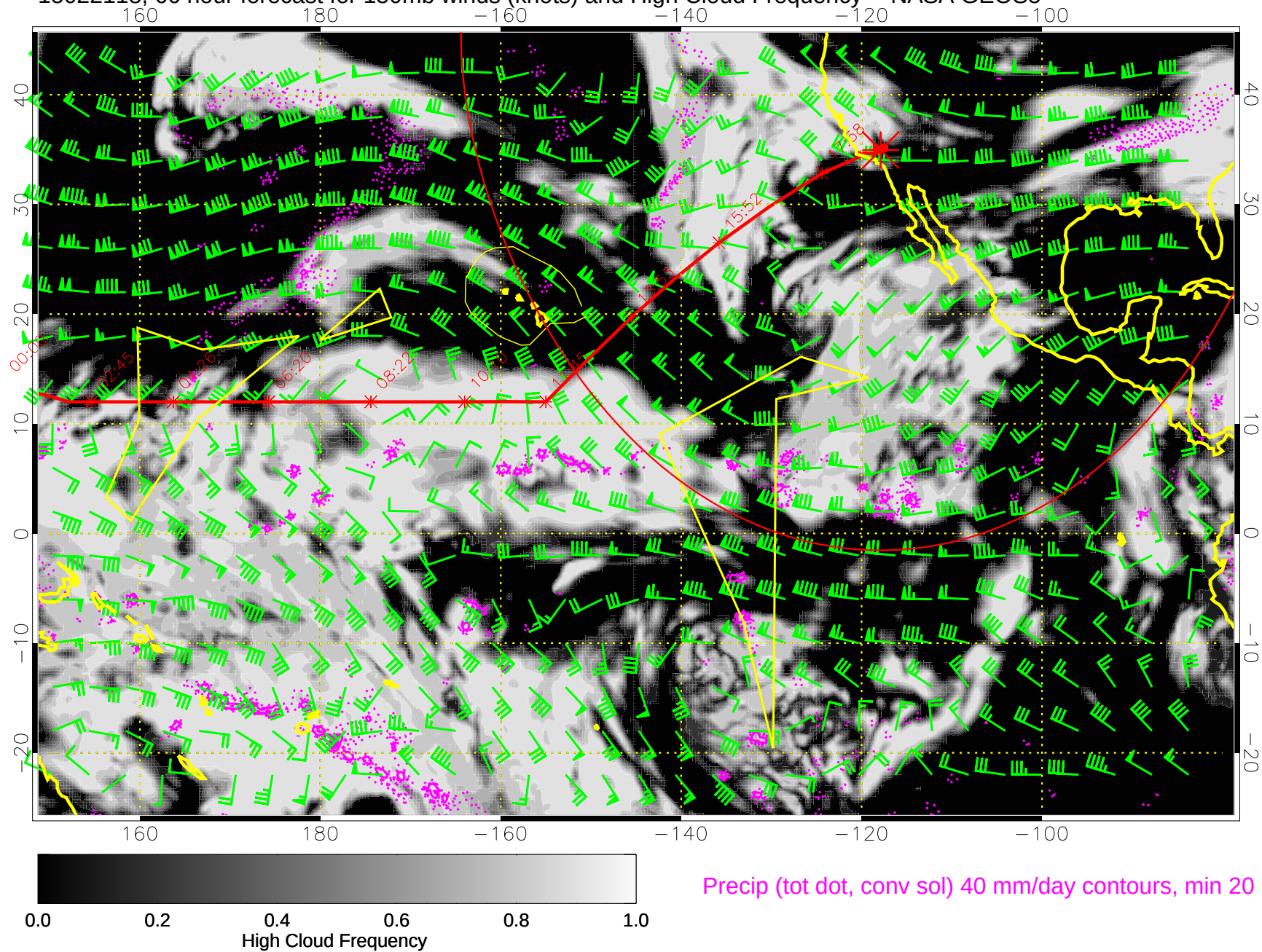
15022118, 66 hour forecast for 150mb winds (knots) and High Cloud Frequency -- NASA GEOS5
