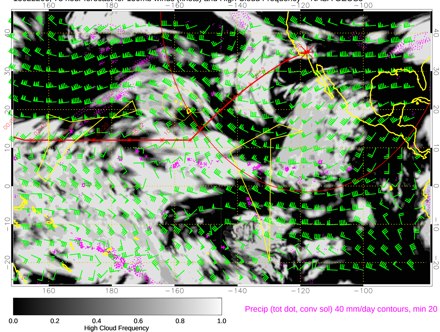
15022206, 78 hour forecast for 150mb winds (knots) and High Cloud Frequency -- NASA GEOS5
