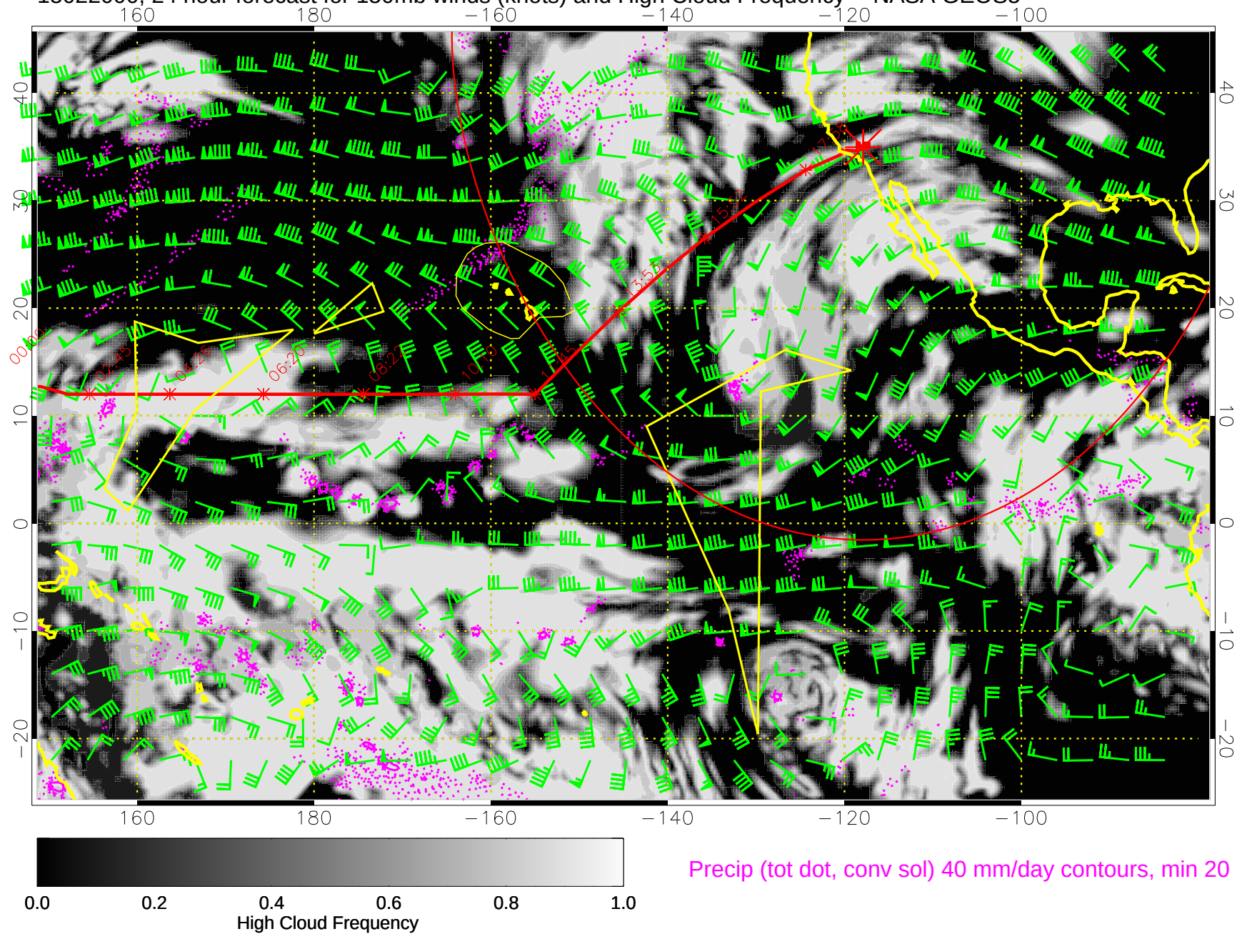
15022000, 24 hour forecast for 150mb winds (knots) and High Cloud Frequency -- NASA GEOS5
