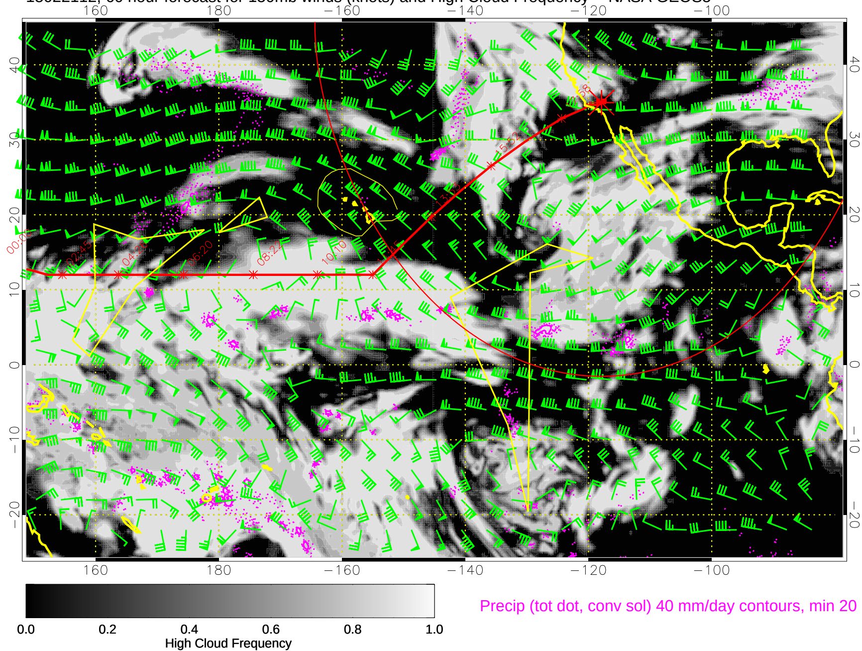
15022112, 60 hour forecast for 150mb winds (knots) and High Cloud Frequency -- NASA GEOS5
