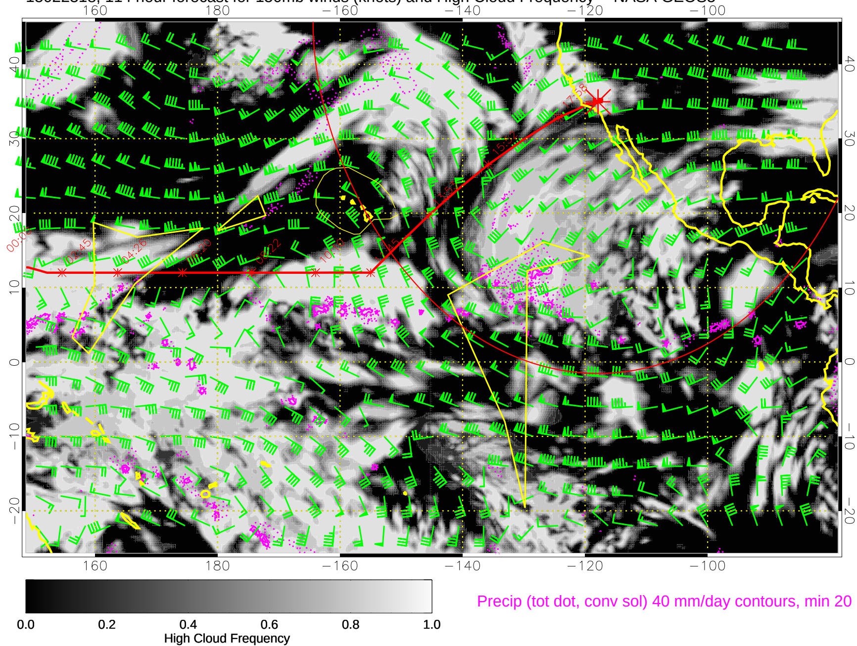
15022318, 114 hour forecast for 150mb winds (knots) and High Cloud Frequency -- NASA GEOS5
