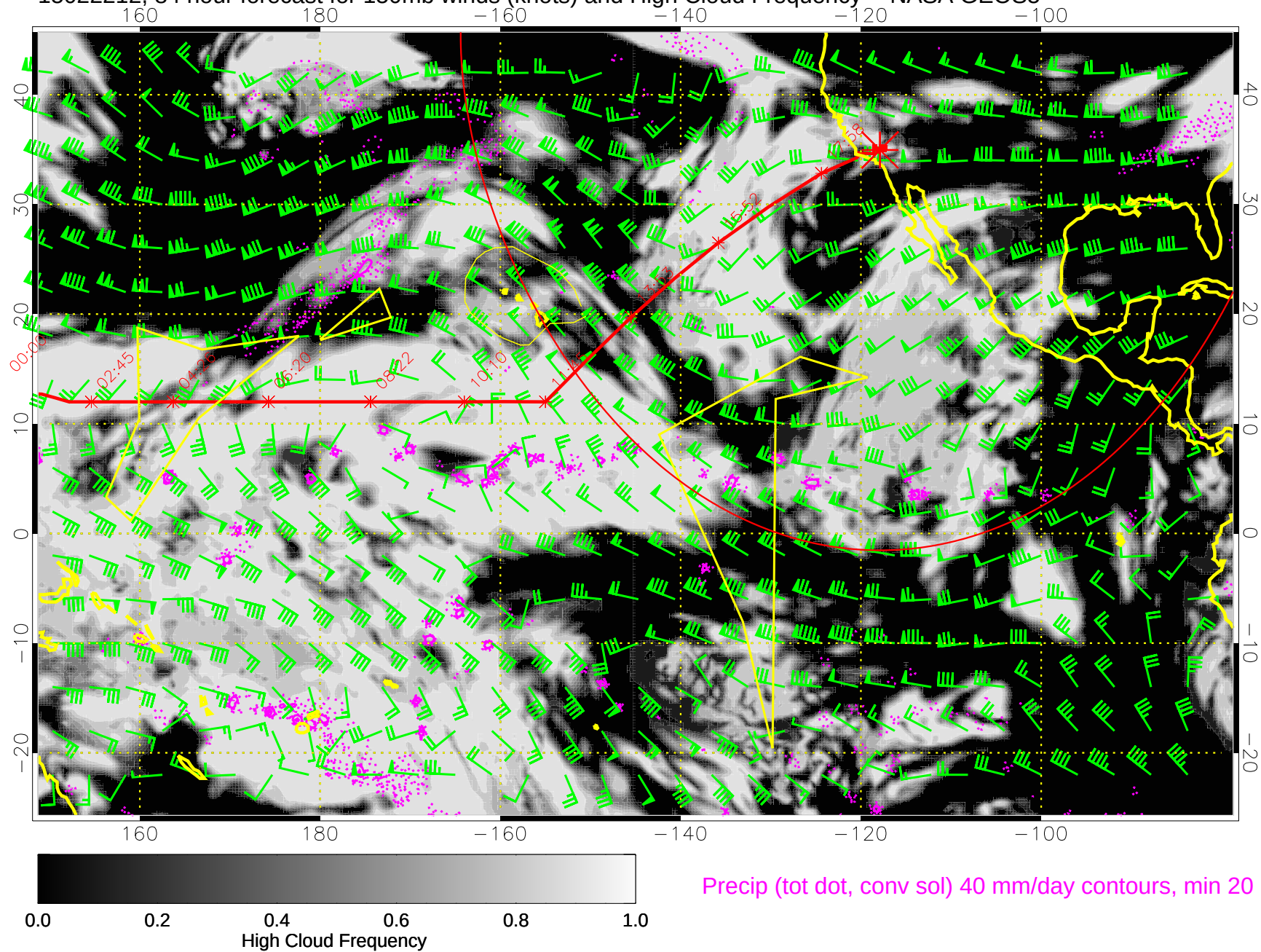
15022212, 84 hour forecast for 150mb winds (knots) and High Cloud Frequency -- NASA GEOS5
