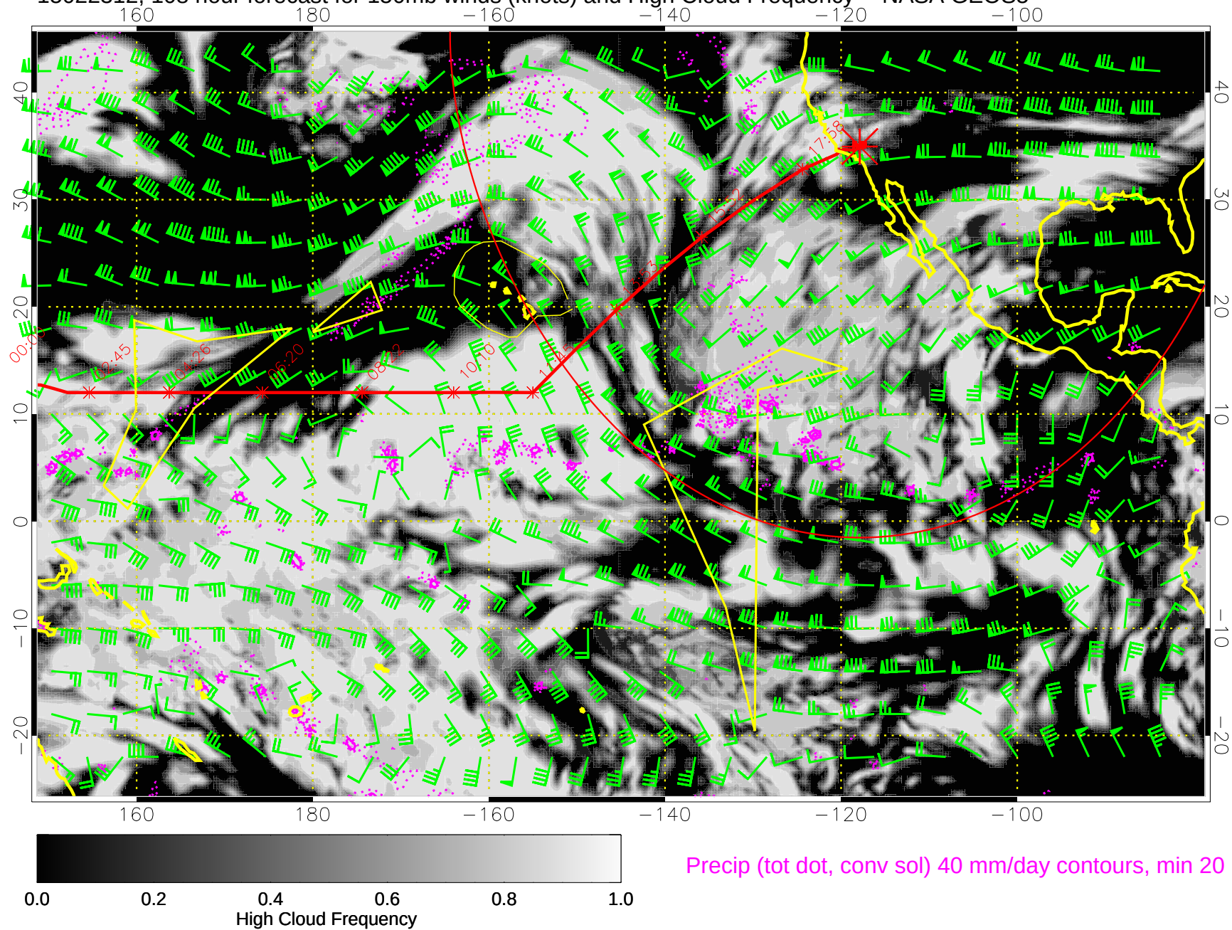
15022312, 108 hour forecast for 150mb winds (knots) and High Cloud Frequency -- NASA GEOS5
