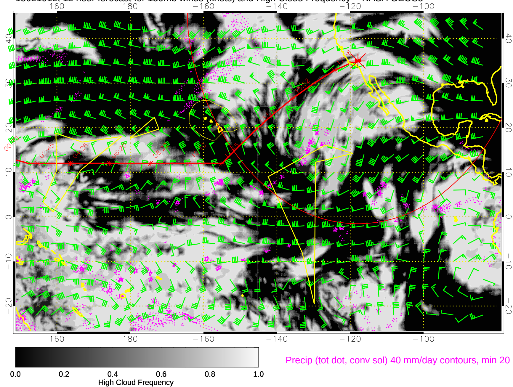
15021912, 12 hour forecast for 150mb winds (knots) and High Cloud Frequency -- NASA GEOS5
