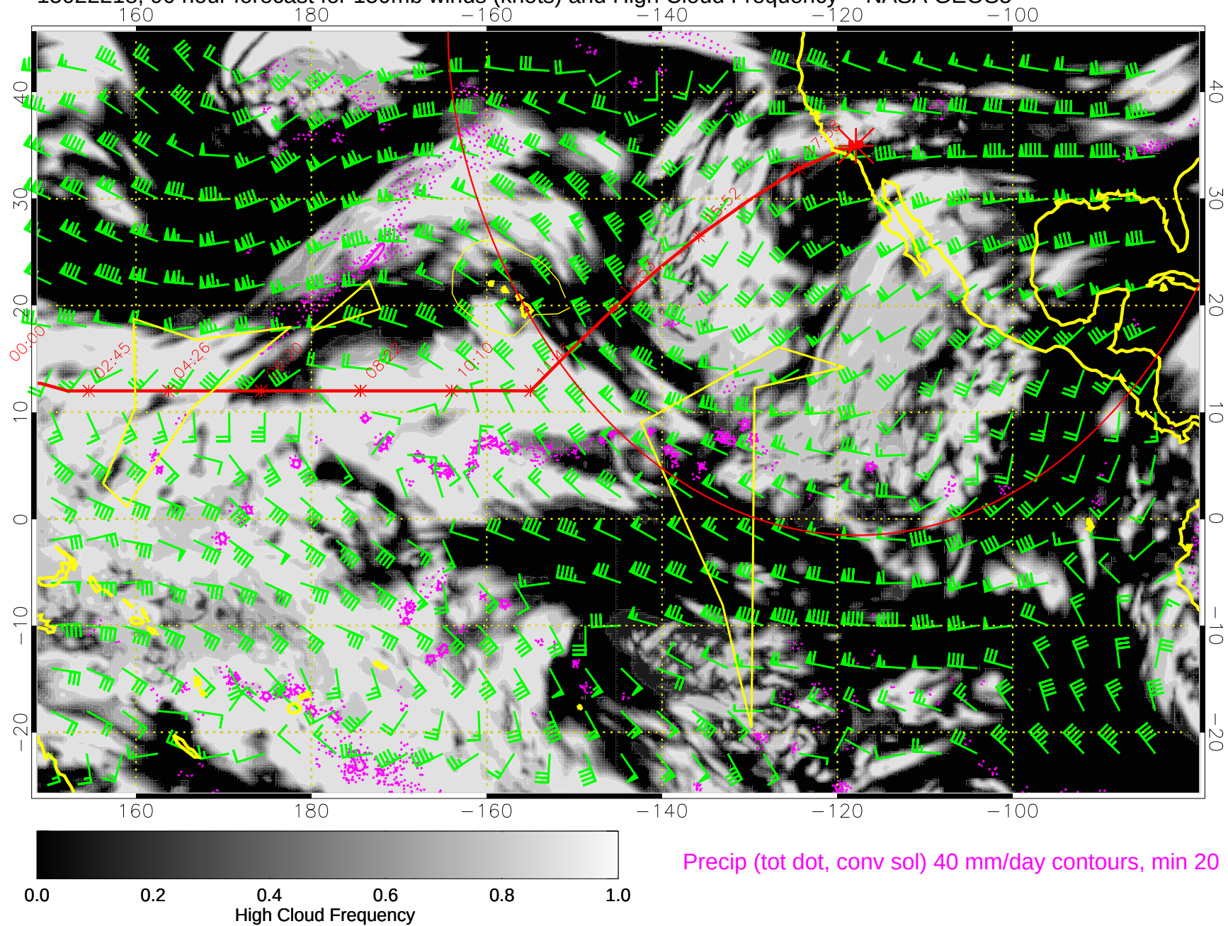
15022218, 90 hour forecast for 150mb winds (knots) and High Cloud Frequency -- NASA GEOS5
