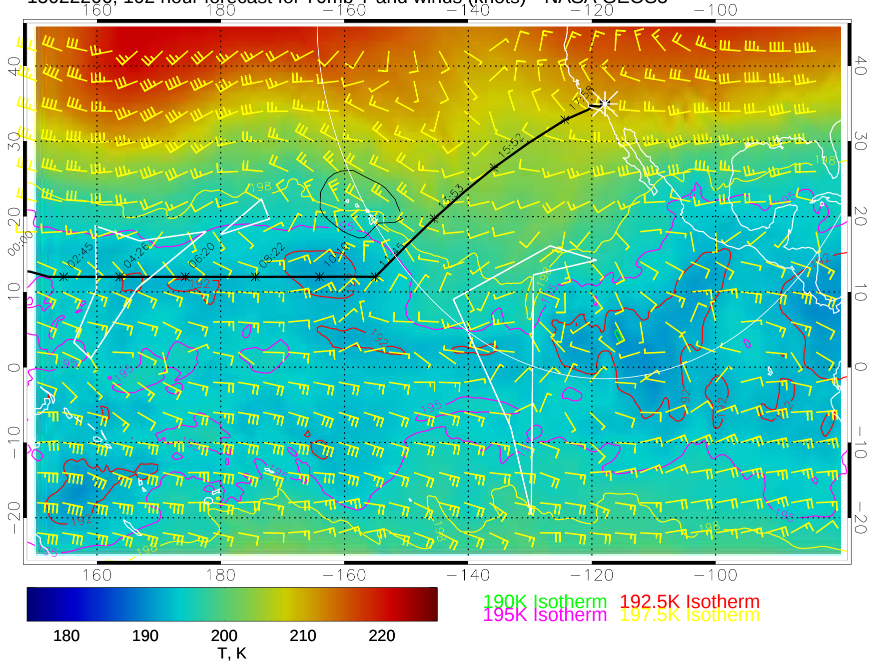
15022206, 102 hour forecast for 70mb T and winds (knots)-- NASA GEOS5
