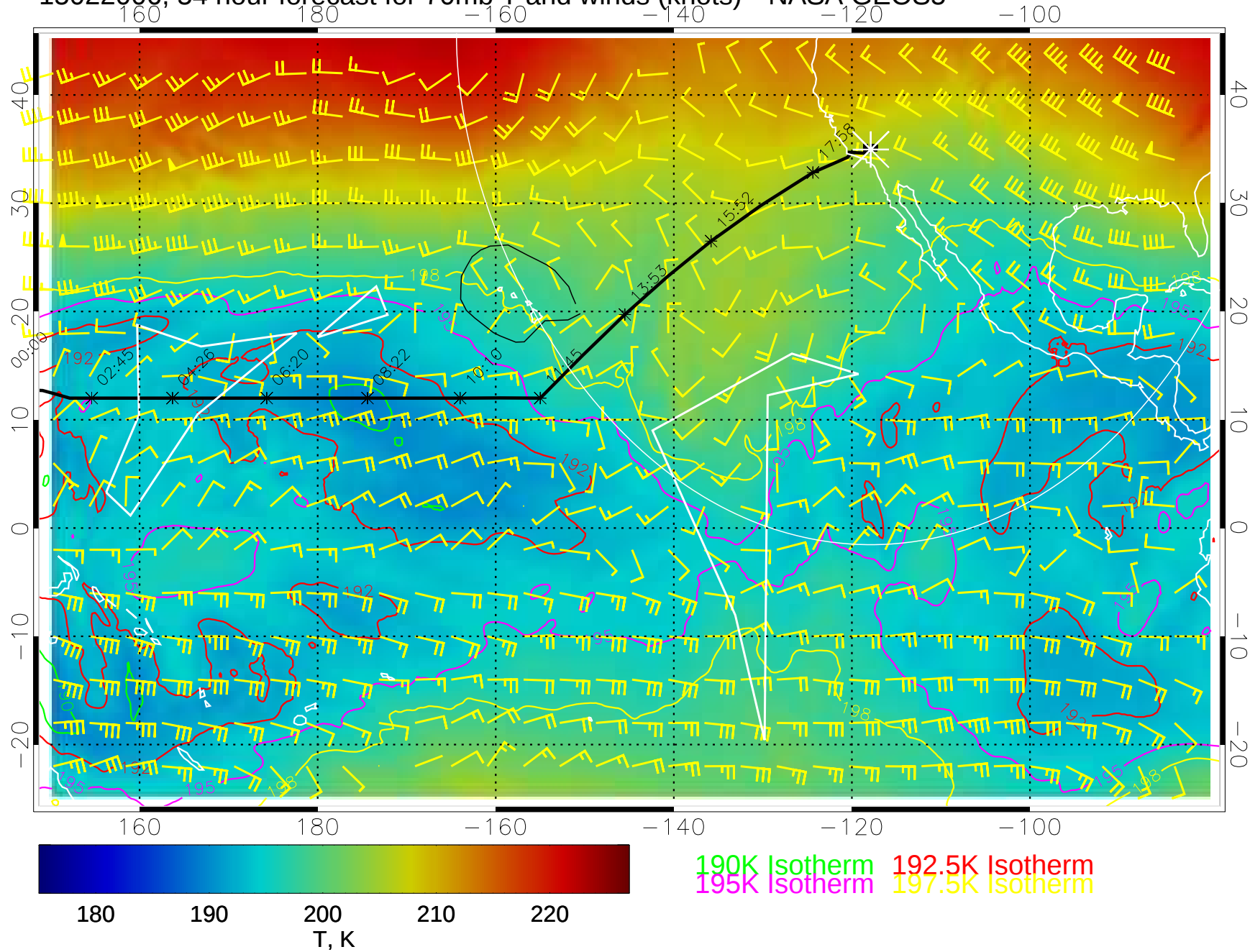
15022006, 54 hour forecast for 70mb T and winds (knots)-- NASA GEOS5
