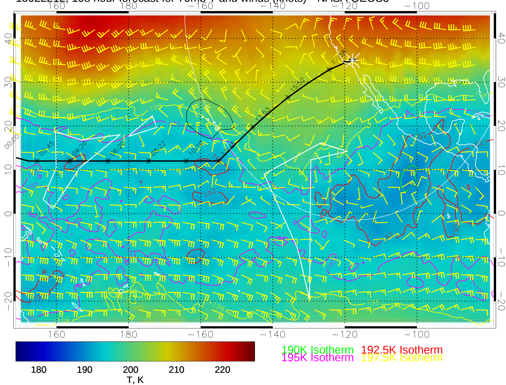
15022212, 108 hour forecast for 70mb T and winds (knots)-- NASA GEOS5
