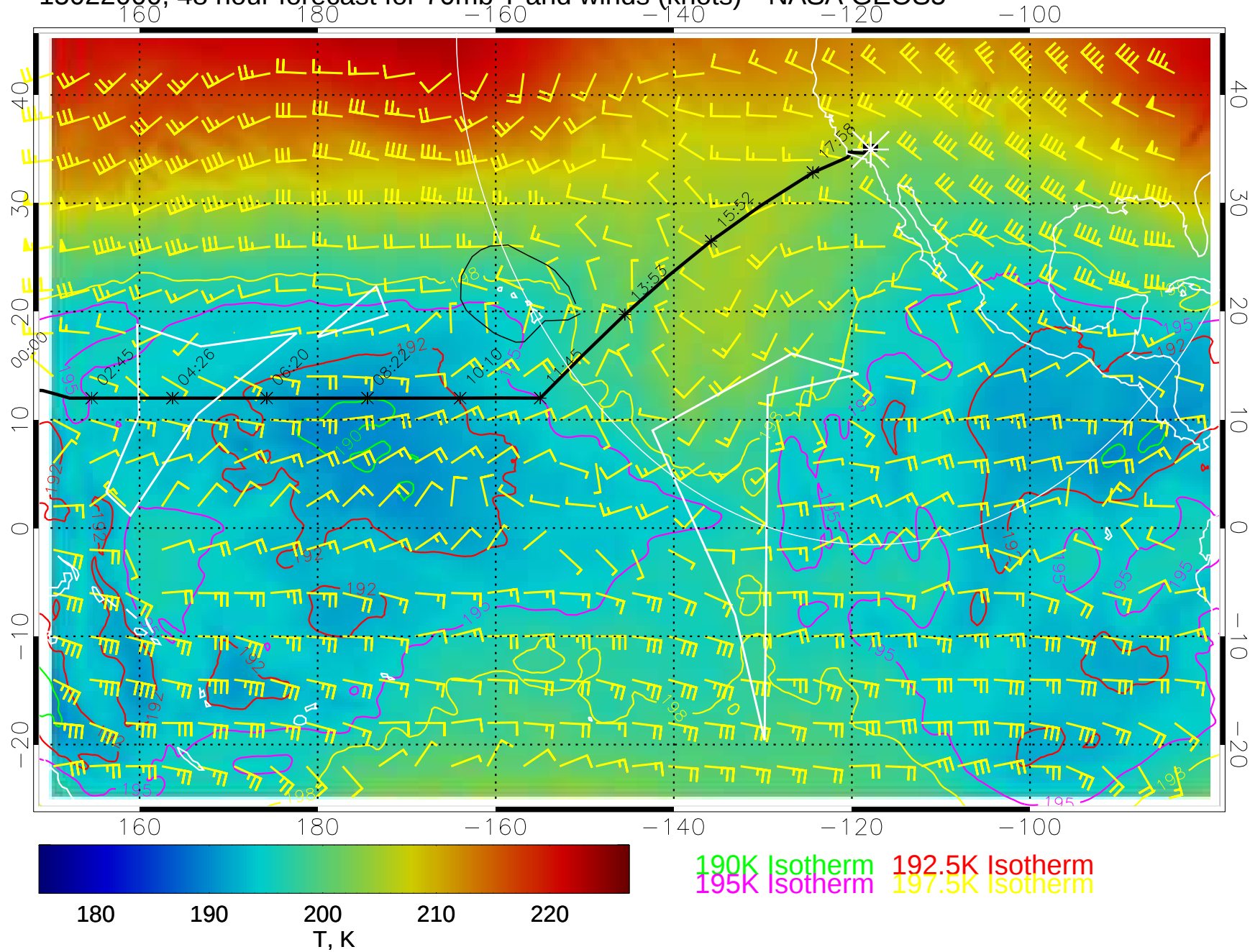
15022000, 48 hour forecast for 70mb T and winds (knots)-- NASA GEOS5
