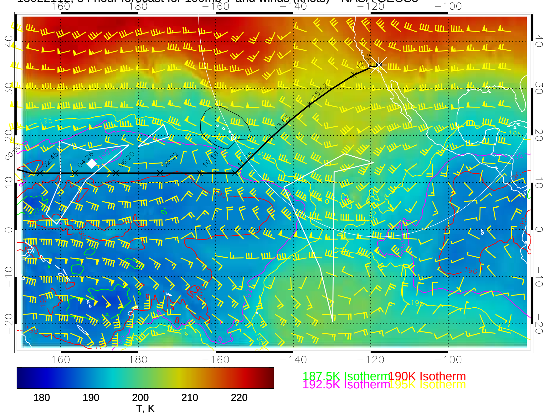
15022112, 84 hour forecast for 100mb T and winds (knots)-- NASA GEOS5
