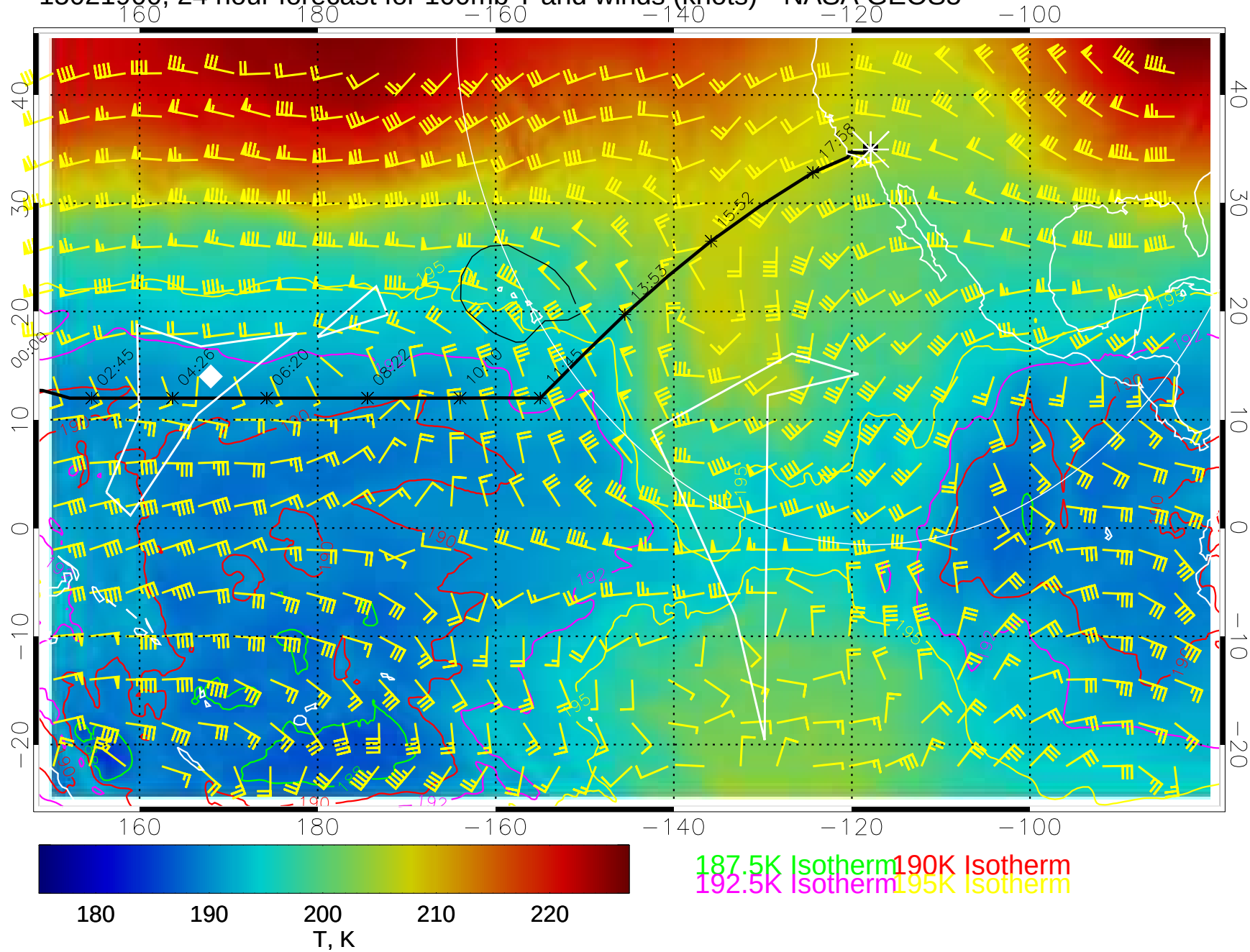
15021900, 24 hour forecast for 100mb T and winds (knots)-- NASA GEOS5
