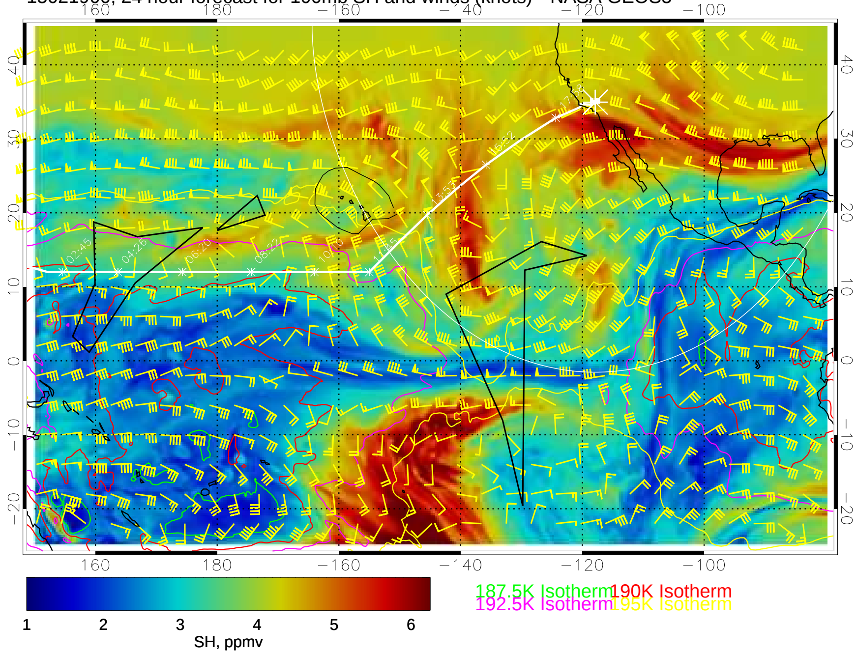
15021900, 24 hour forecast for 100mb SH and winds (knots)-- NASA GEOS5
