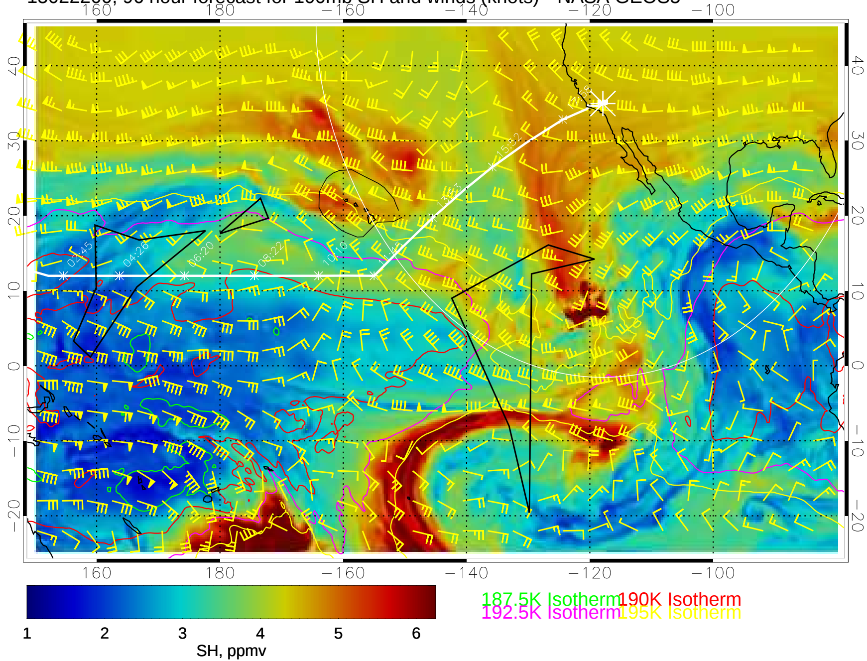
15022200, 96 hour forecast for 100mb SH and winds (knots)-- NASA GEOS5
