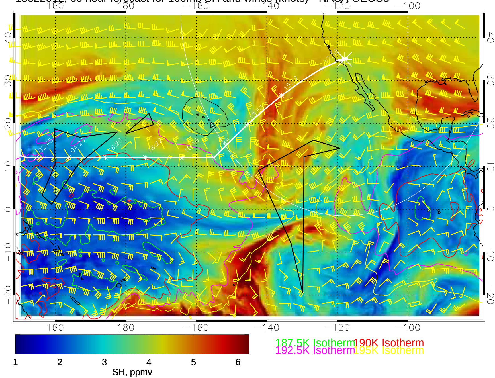
15022012, 60 hour forecast for 100mb SH and winds (knots)-- NASA GEOS5
