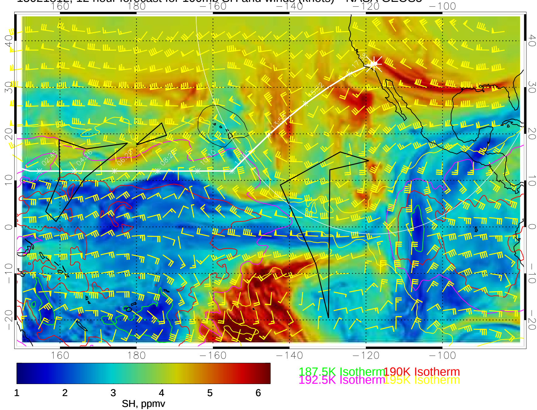
15021812, 12 hour forecast for 100mb SH and winds (knots)-- NASA GEOS5
