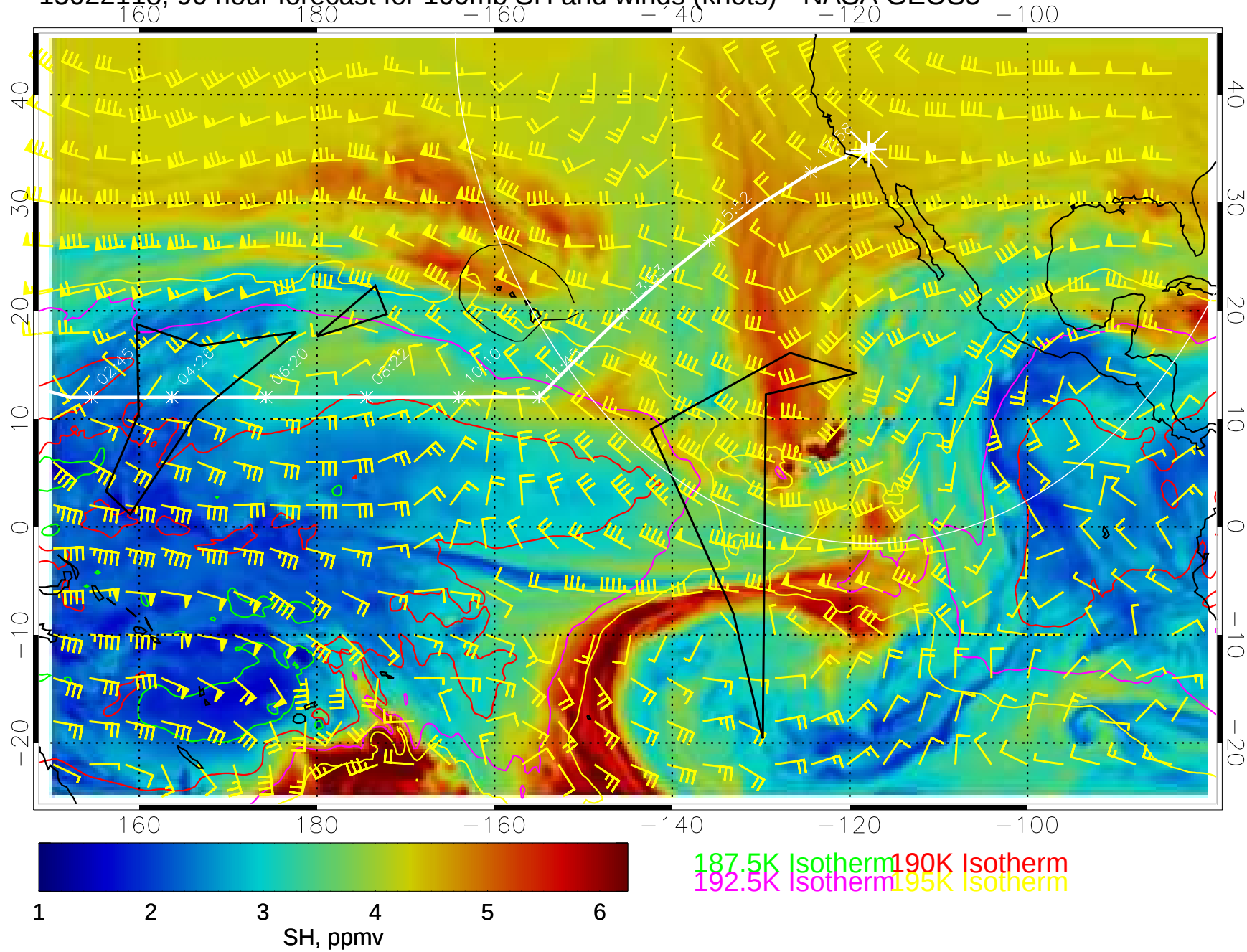
15022118, 90 hour forecast for 100mb SH and winds (knots)-- NASA GEOS5
