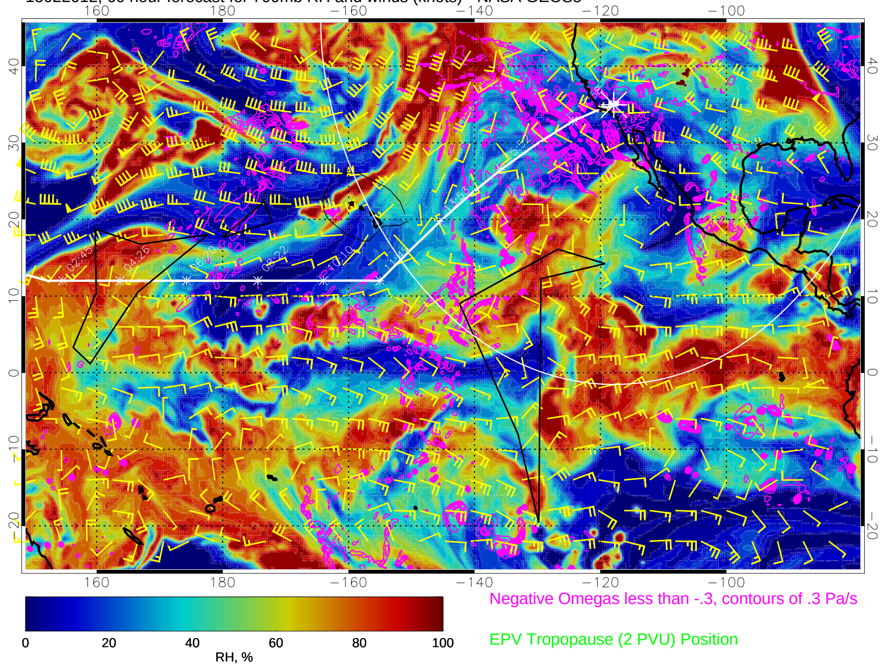
15022012, 60 hour forecast for 700mb RH and winds (knots) - NASA GEOS5
