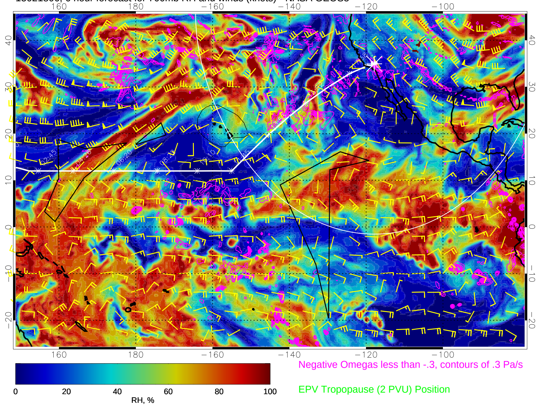
15021806, 6 hour forecast for 700mb RH and winds (knots) - NASA GEOS5
