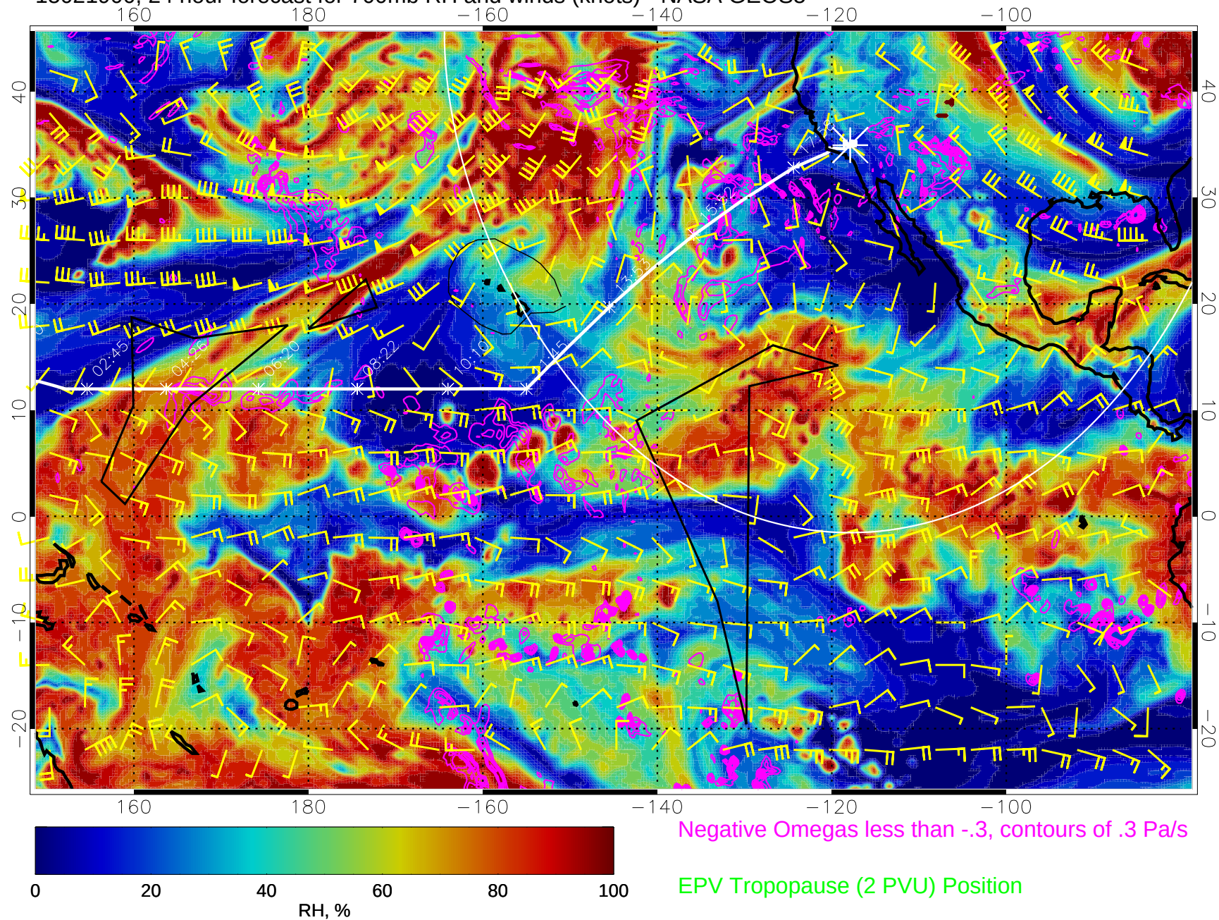
15021900, 24 hour forecast for 700mb RH and winds (knots) - NASA GEOS5
