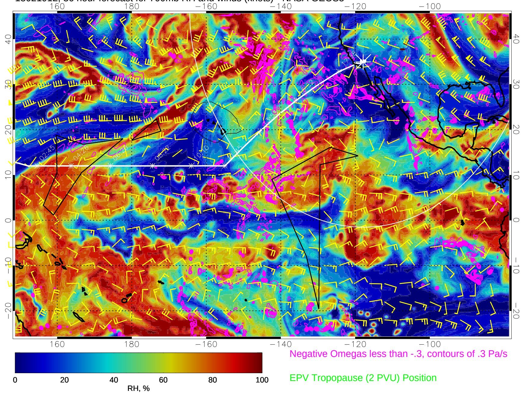
15021912, 36 hour forecast for 700mb RH and winds (knots) - NASA GEOS5
