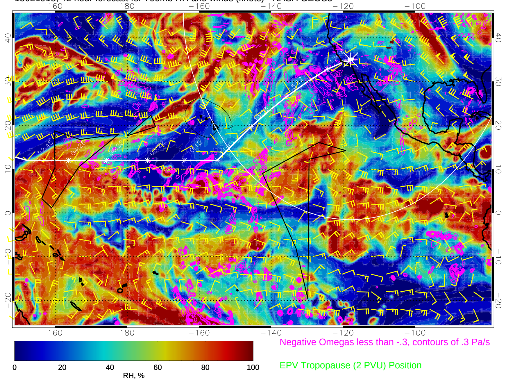
15021918, 42 hour forecast for 700mb RH and winds (knots) - NASA GEOS5
