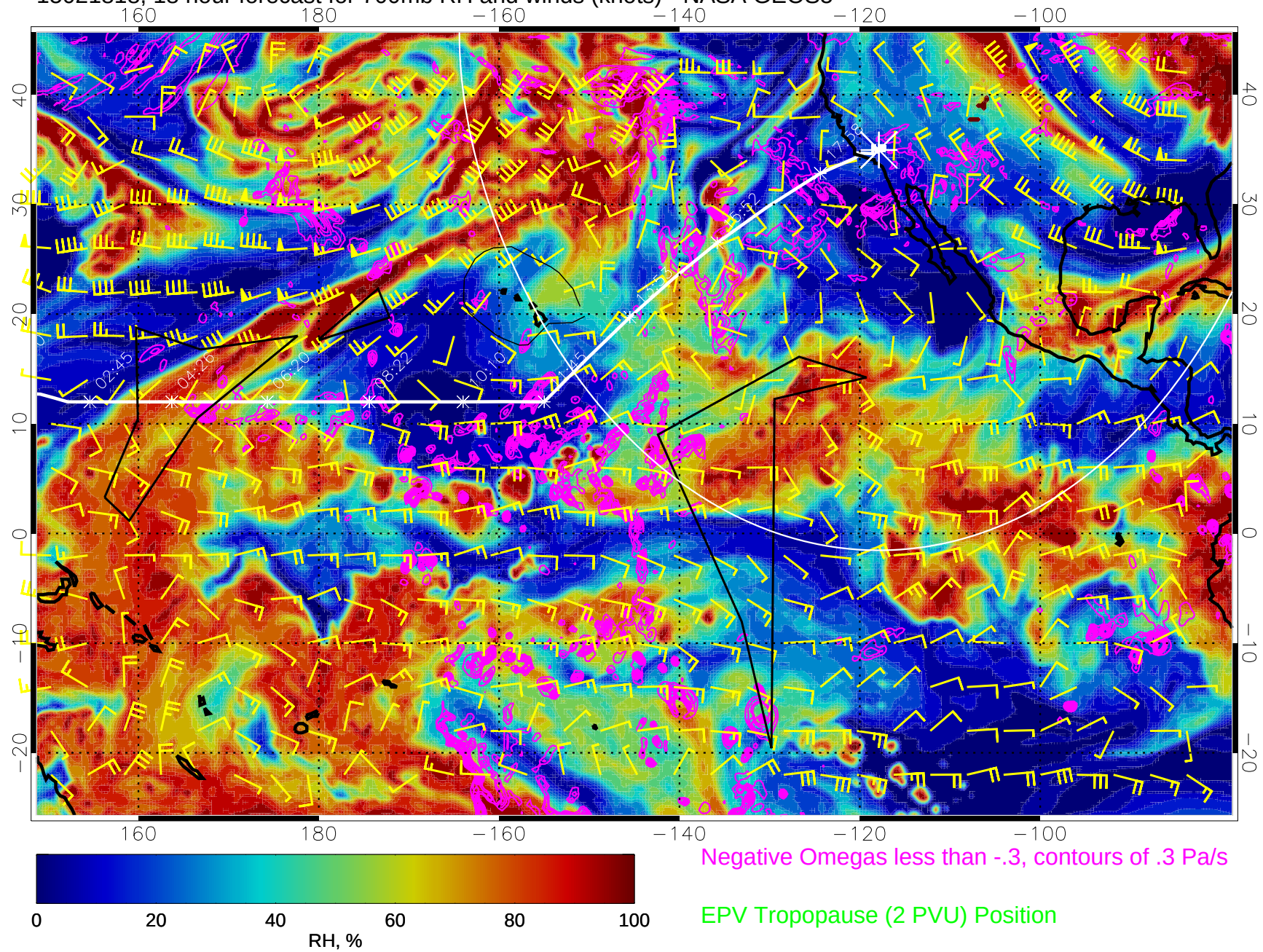
15021818, 18 hour forecast for 700mb RH and winds (knots) - NASA GEOS5
