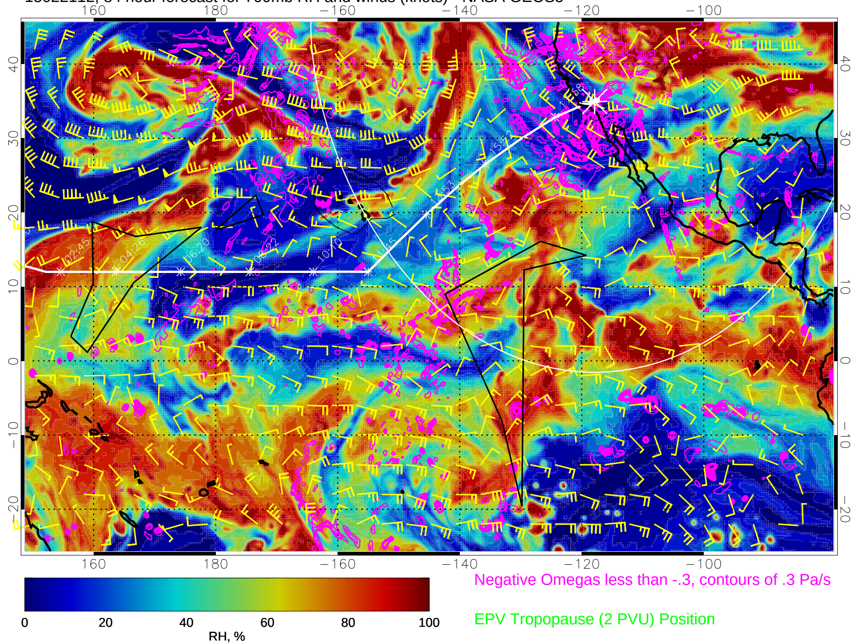
15022112, 84 hour forecast for 700mb RH and winds (knots) - NASA GEOS5
