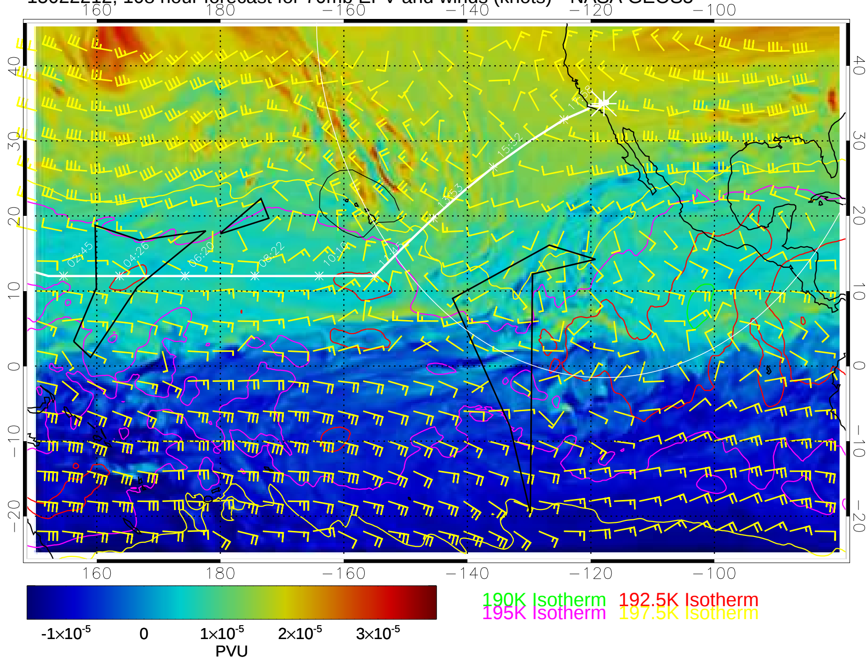
15022212, 108 hour forecast for 70mb EPV and winds (knots)-- NASA GEOS5
