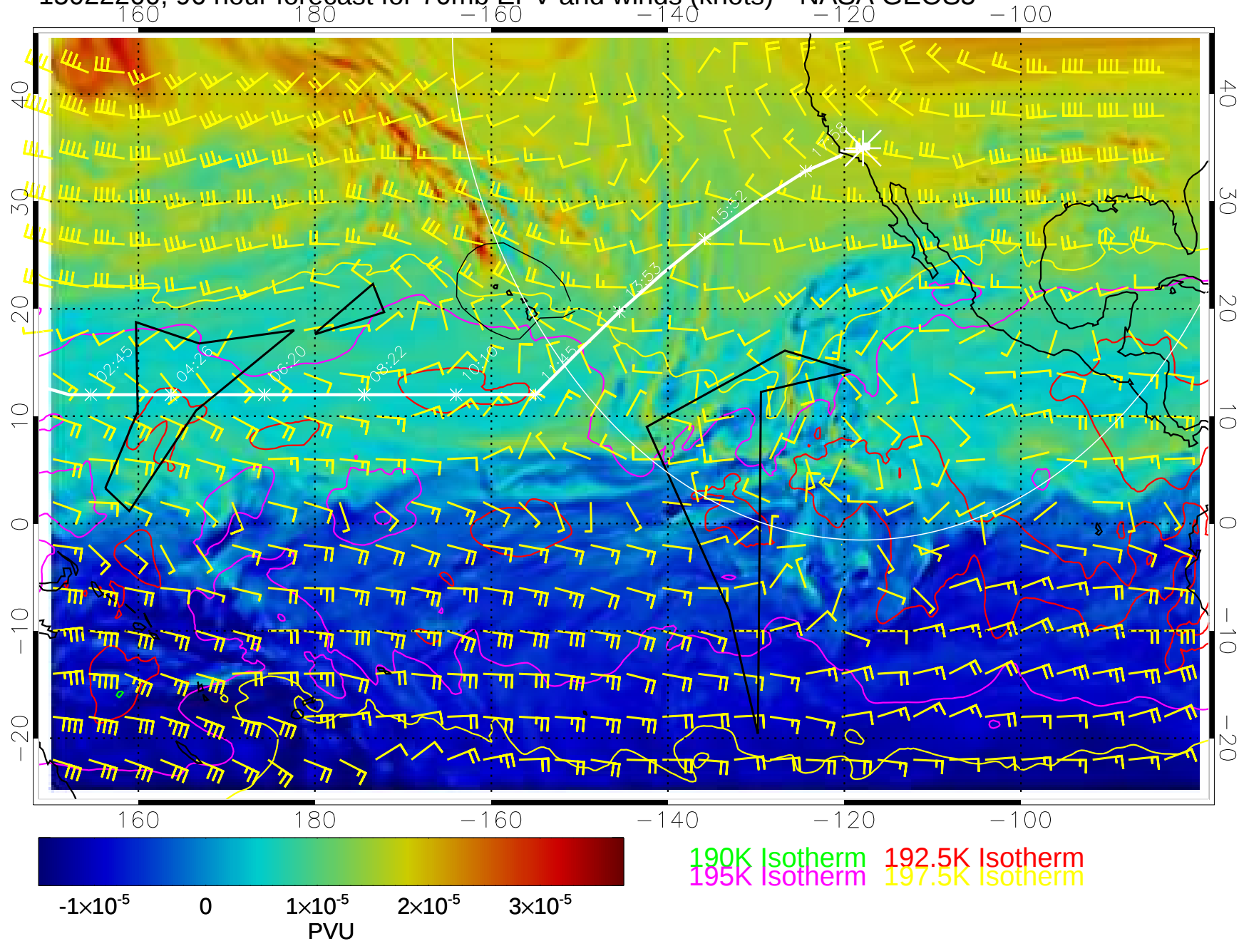
15022200, 96 hour forecast for 70mb EPV and winds (knots)-- NASA GEOS5
