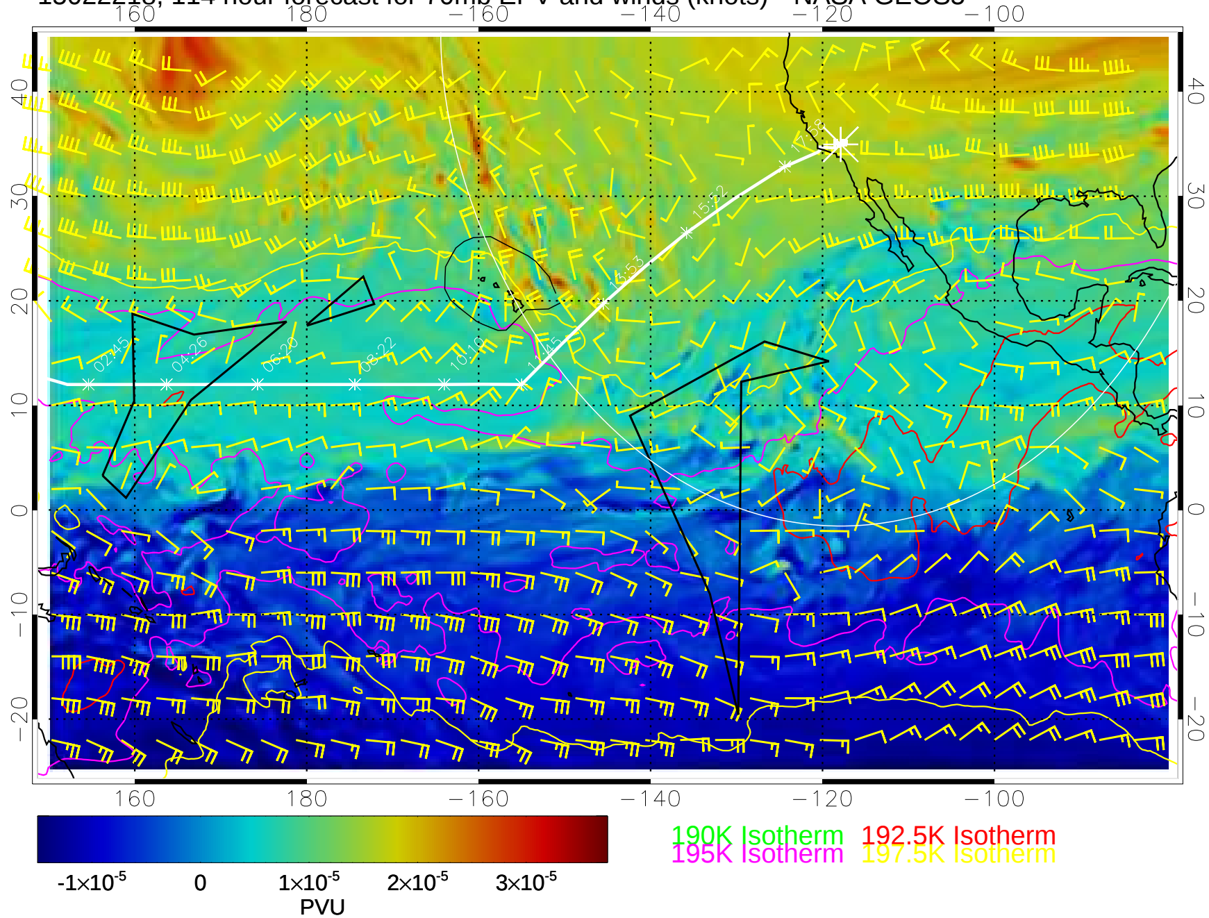
15022218, 114 hour forecast for 70mb EPV and winds (knots)-- NASA GEOS5
