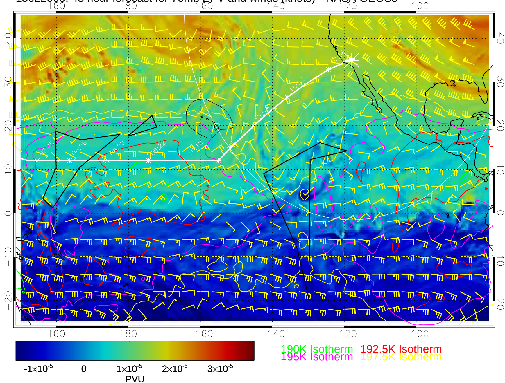
15022000, 48 hour forecast for 70mb EPV and winds (knots)-- NASA GEOS5
