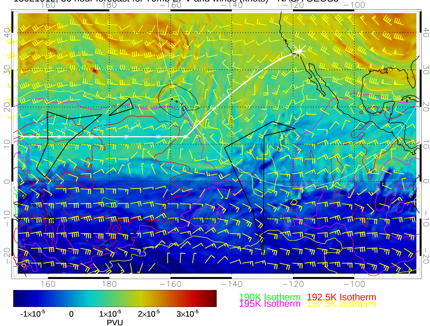
15021912, 36 hour forecast for 70mb EPV and winds (knots)-- NASA GEOS5
