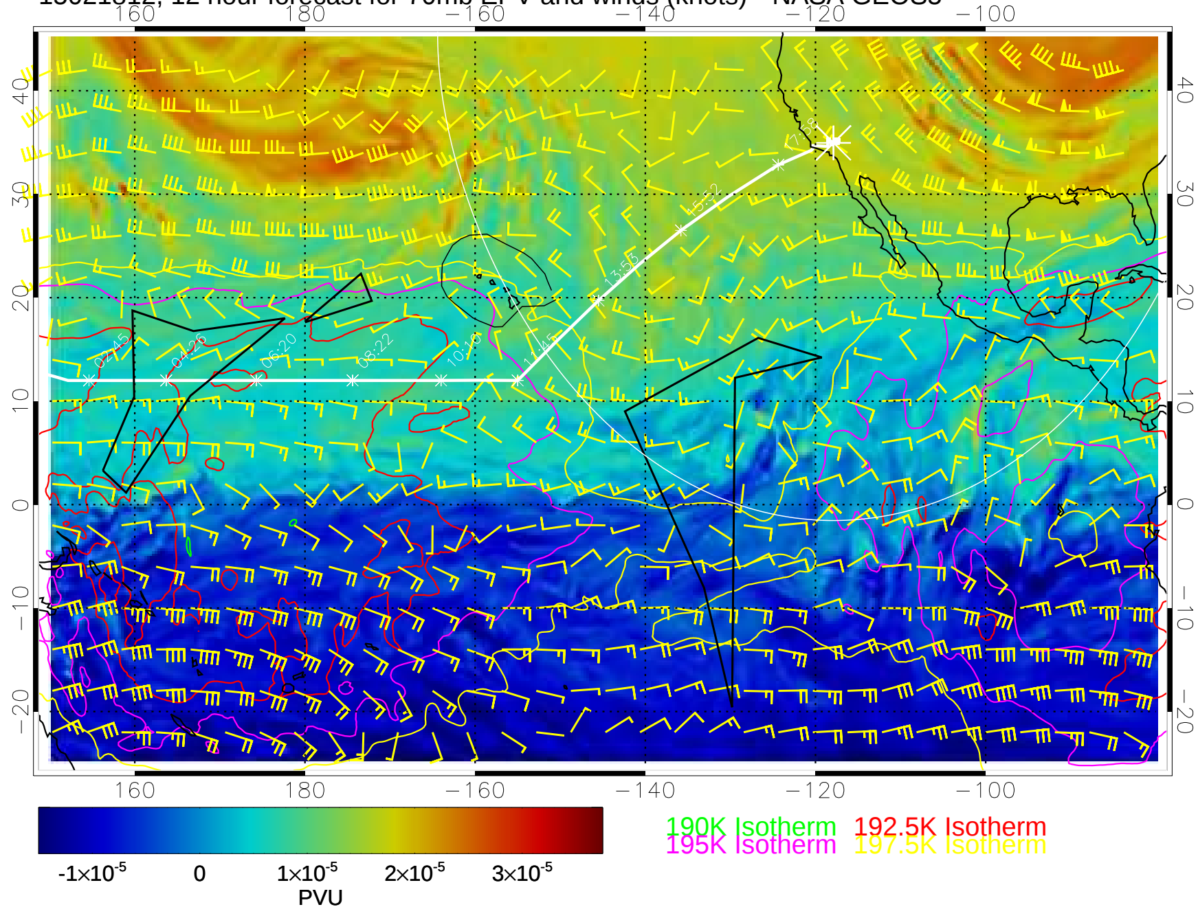
15021812, 12 hour forecast for 70mb EPV and winds (knots)-- NASA GEOS5
