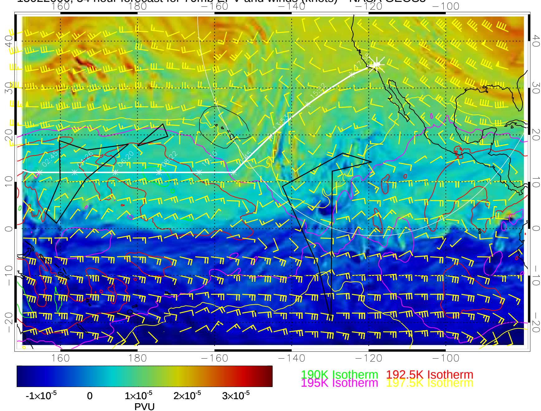
15022006, 54 hour forecast for 70mb EPV and winds (knots)-- NASA GEOS5
