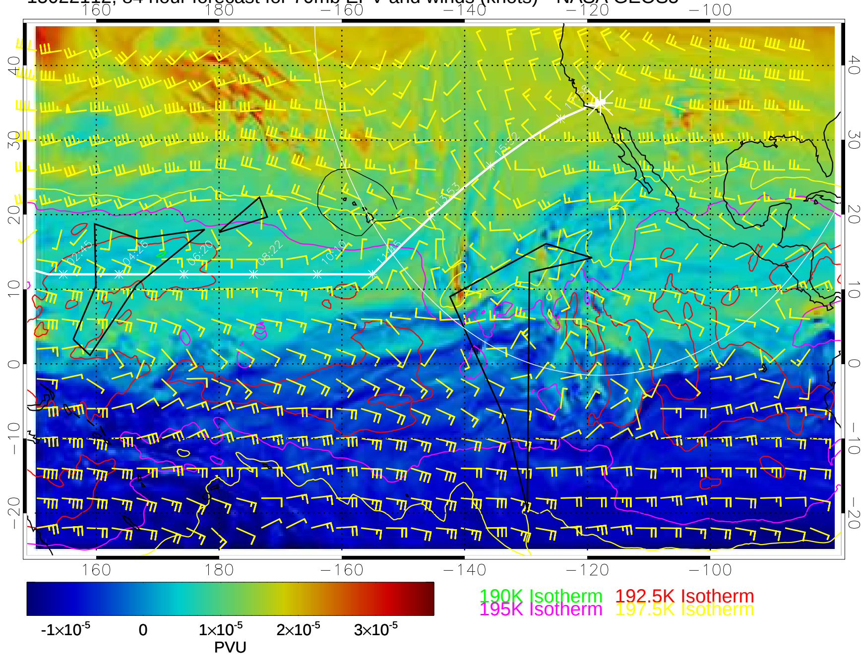
15022112, 84 hour forecast for 70mb EPV and winds (knots)-- NASA GEOS5
