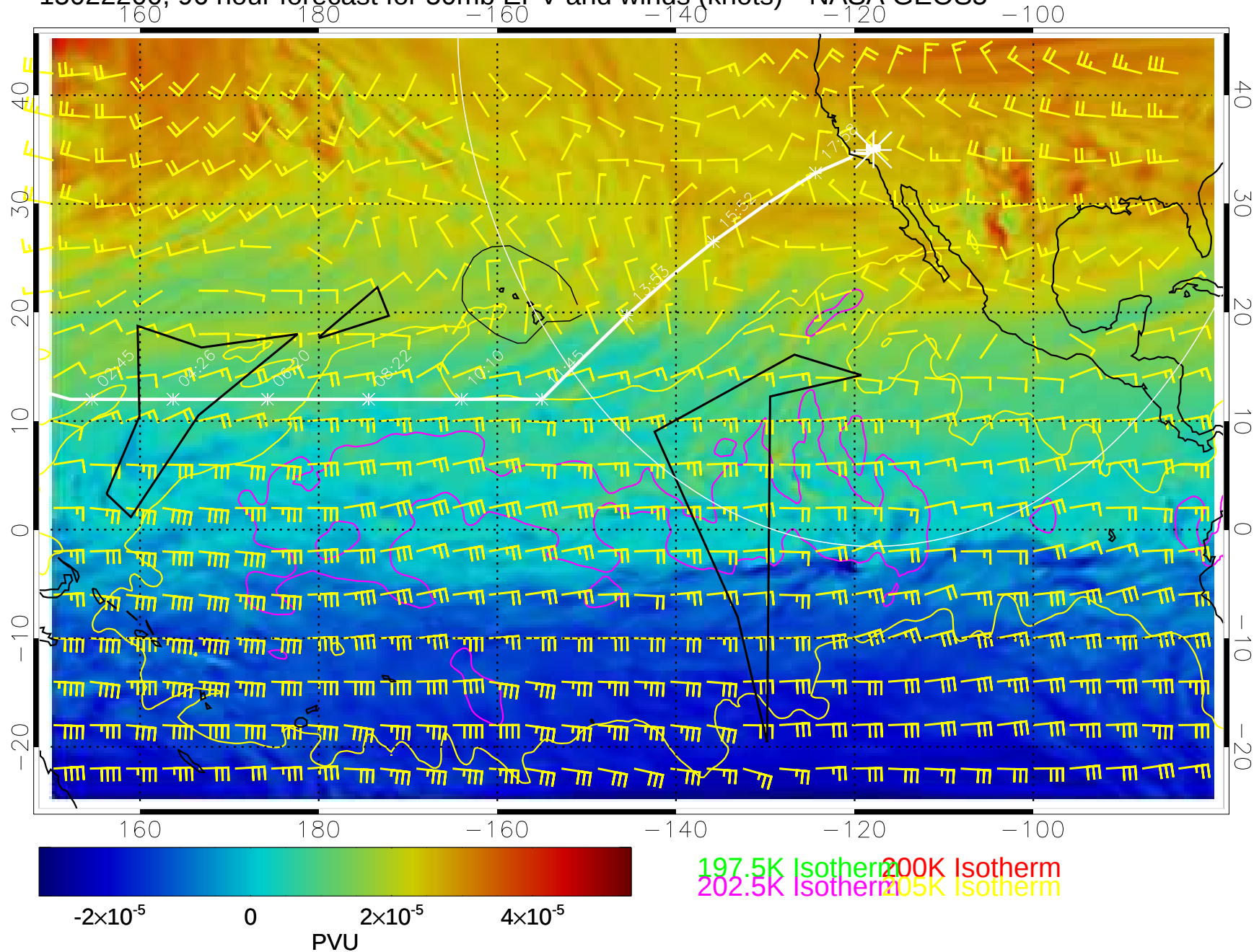
15022200, 96 hour forecast for 50mb EPV and winds (knots)-- NASA GEOS5
