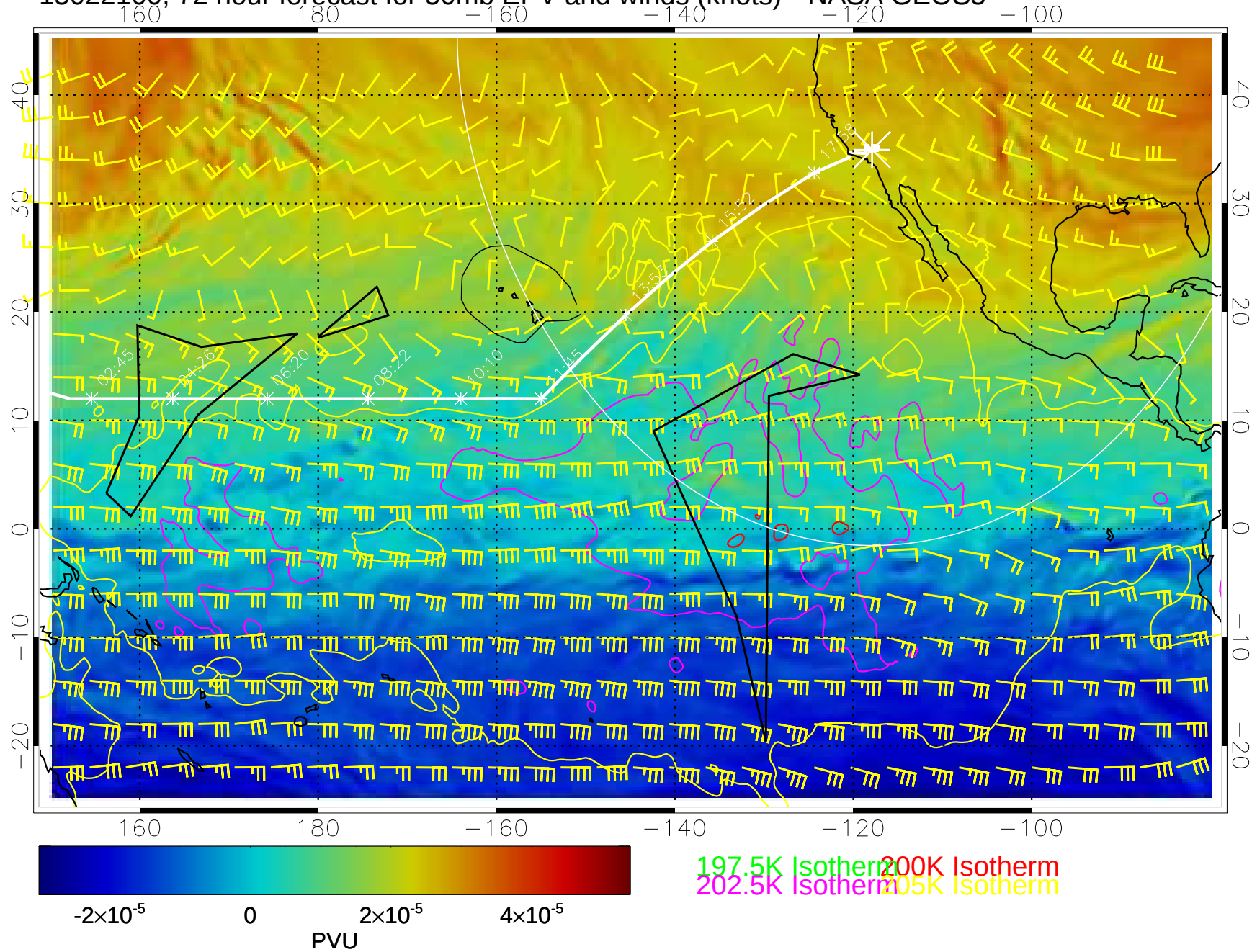
15022100, 72 hour forecast for 50mb EPV and winds (knots)-- NASA GEOS5
