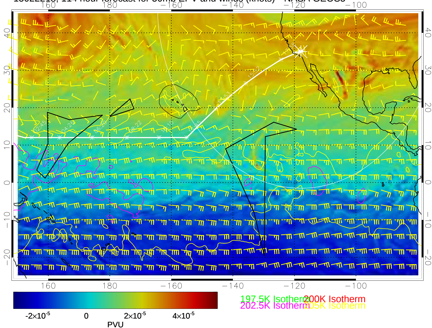
15022218, 114 hour forecast for 50mb EPV and winds (knots)-- NASA GEOS5
