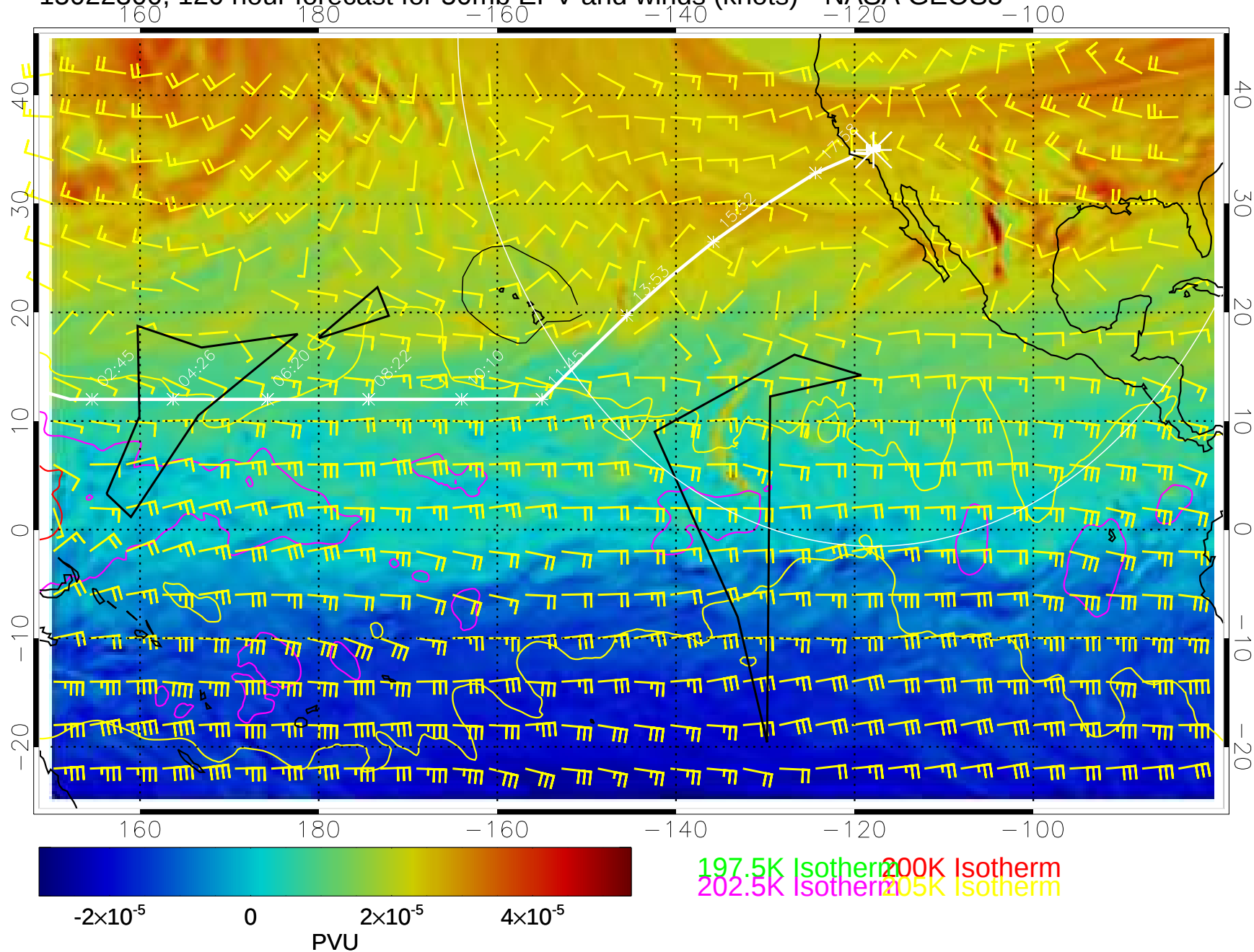
15022300, 120 hour forecast for 50mb EPV and winds (knots)-- NASA GEOS5
