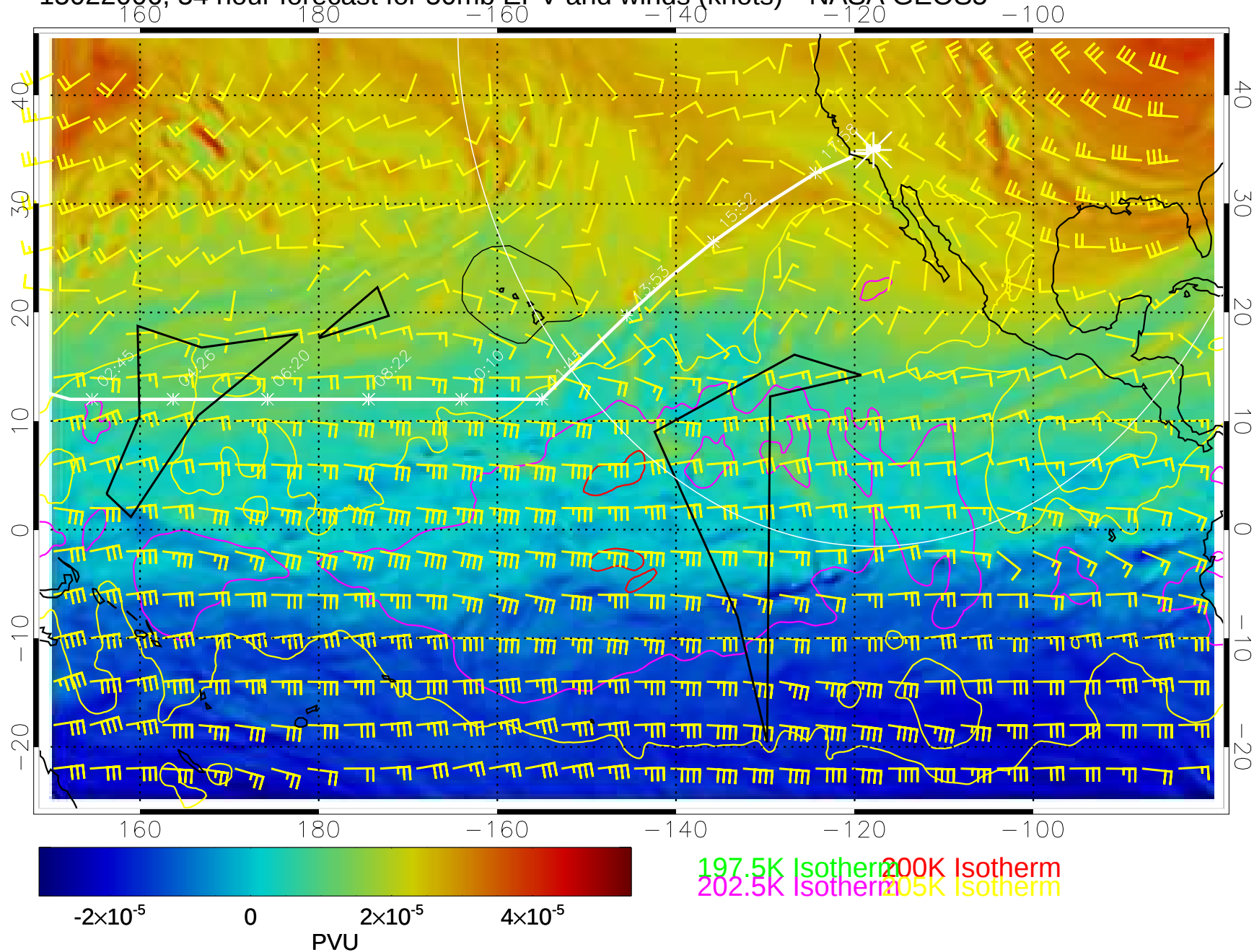
15022006, 54 hour forecast for 50mb EPV and winds (knots)-- NASA GEOS5
