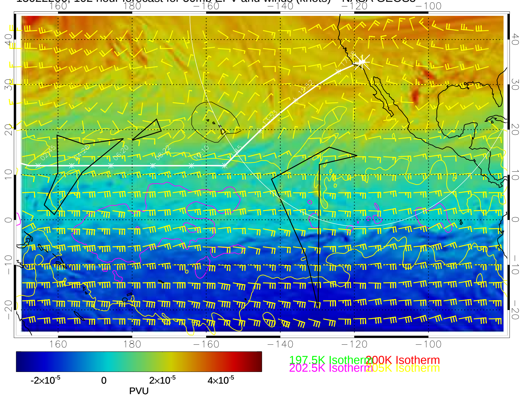
15022206, 102 hour forecast for 50mb EPV and winds (knots)-- NASA GEOS5
