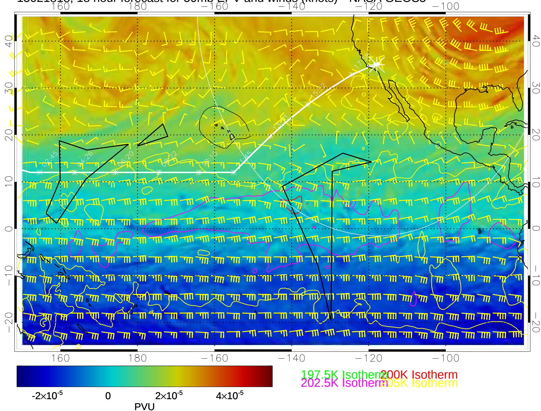
15021818, 18 hour forecast for 50mb EPV and winds (knots)-- NASA GEOS5
