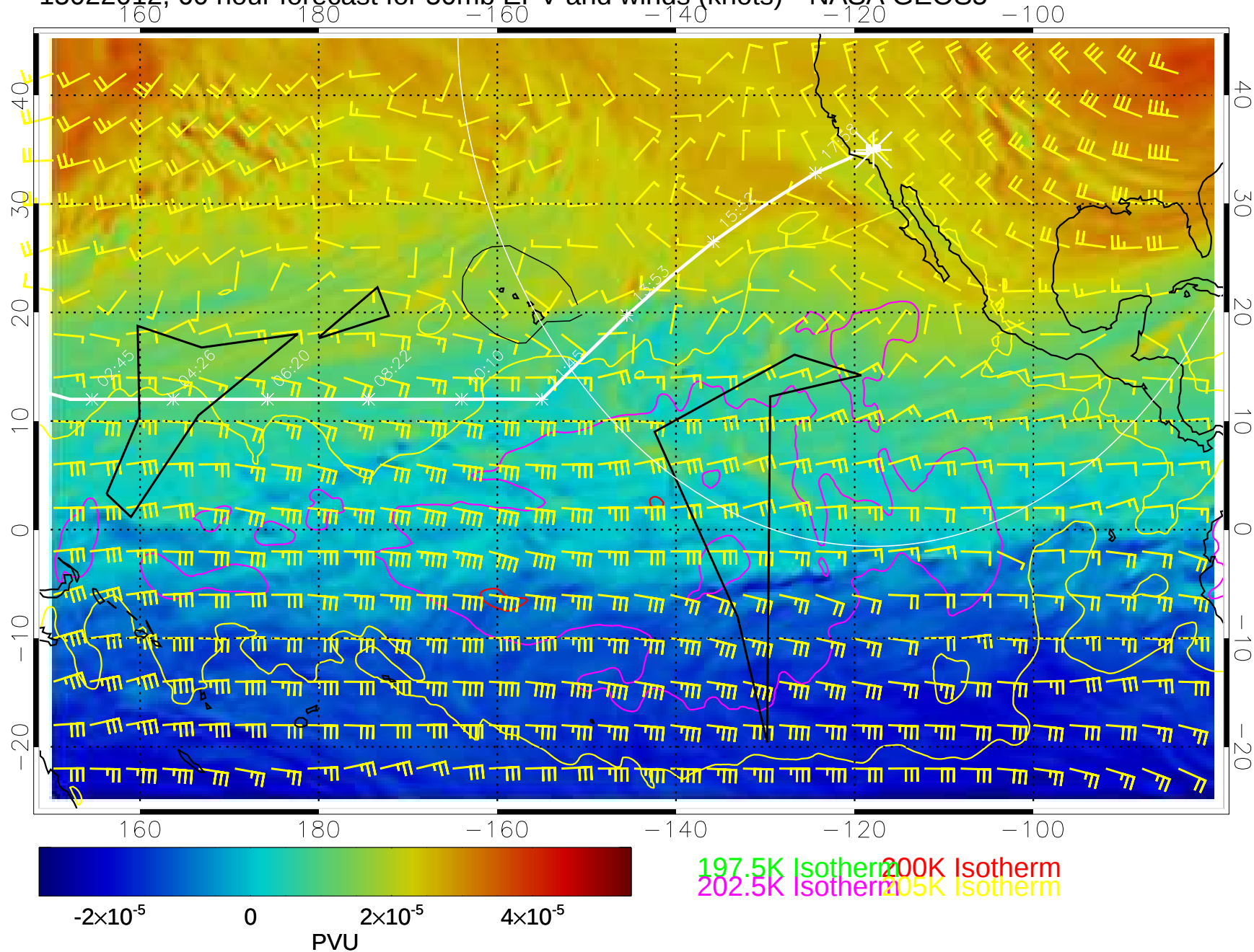
15022012, 60 hour forecast for 50mb EPV and winds (knots)-- NASA GEOS5
