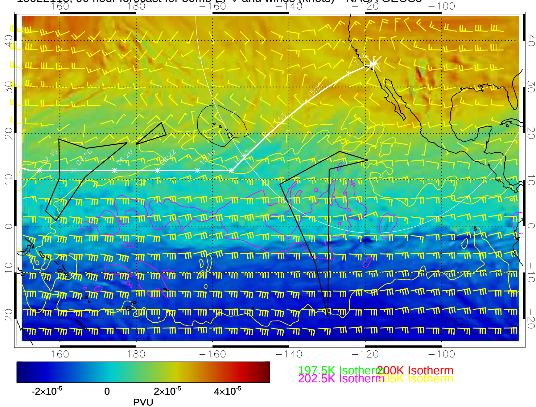
15022118, 90 hour forecast for 50mb EPV and winds (knots)-- NASA GEOS5
