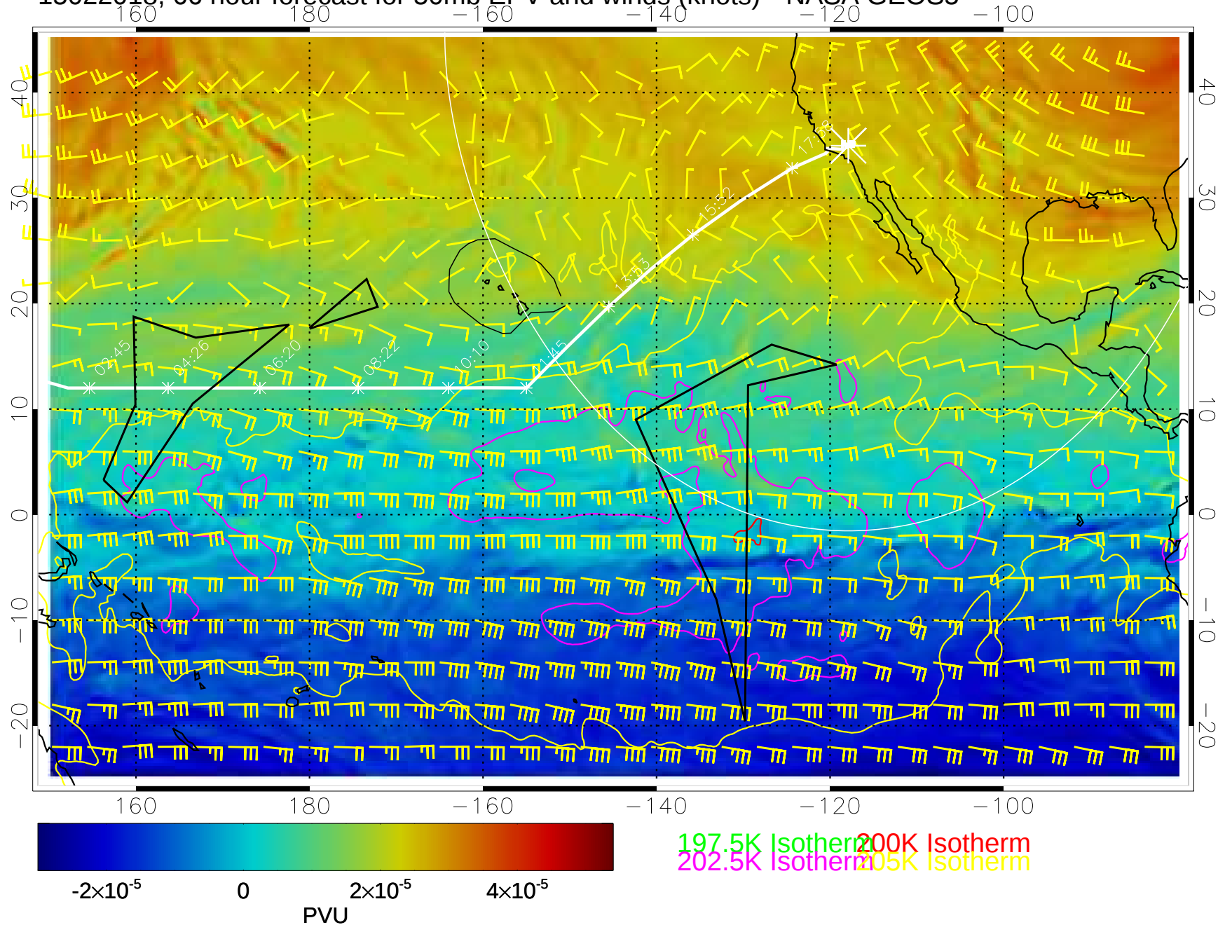
15022018, 66 hour forecast for 50mb EPV and winds (knots)-- NASA GEOS5
