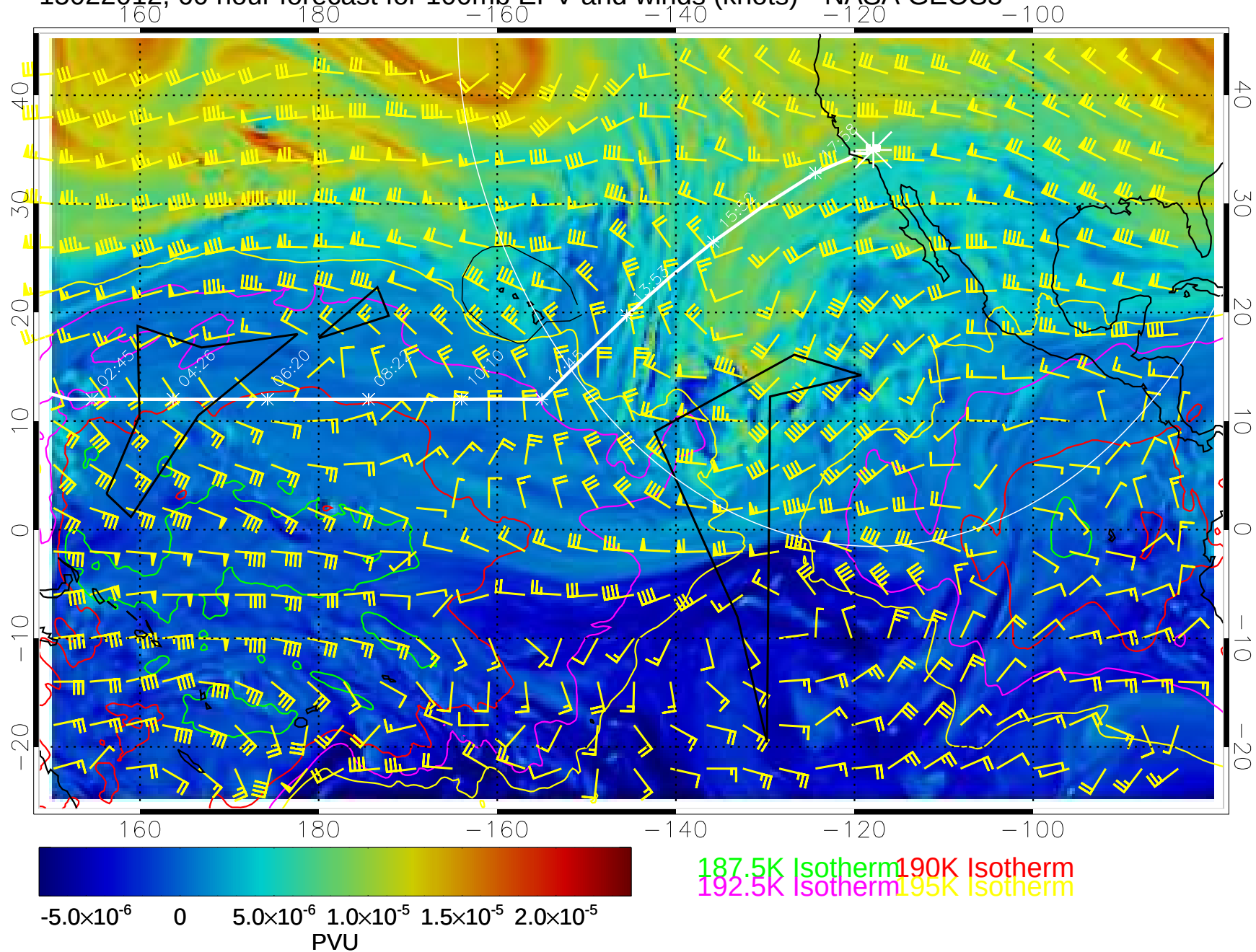
15022012, 60 hour forecast for 100mb EPV and winds (knots)-- NASA GEOS5
