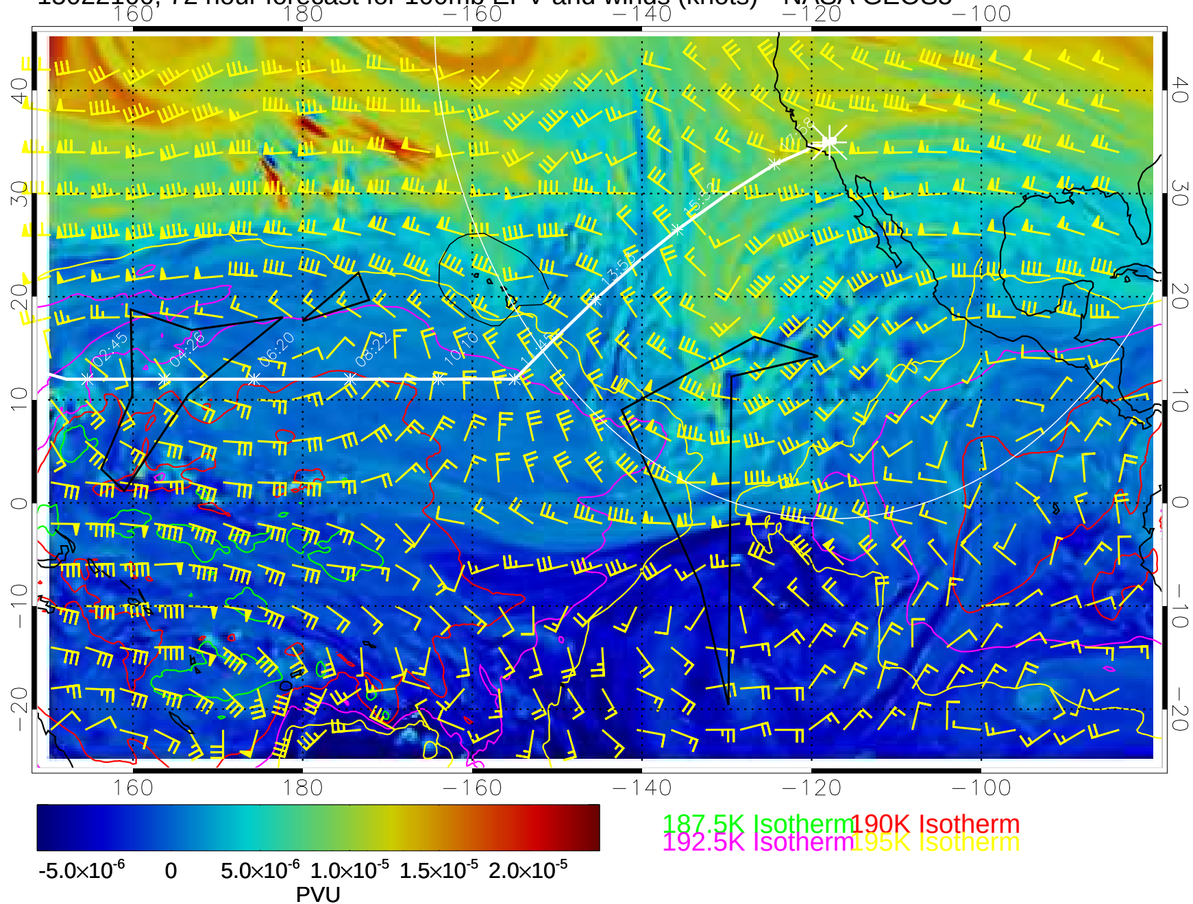
15022100, 72 hour forecast for 100mb EPV and winds (knots)-- NASA GEOS5
