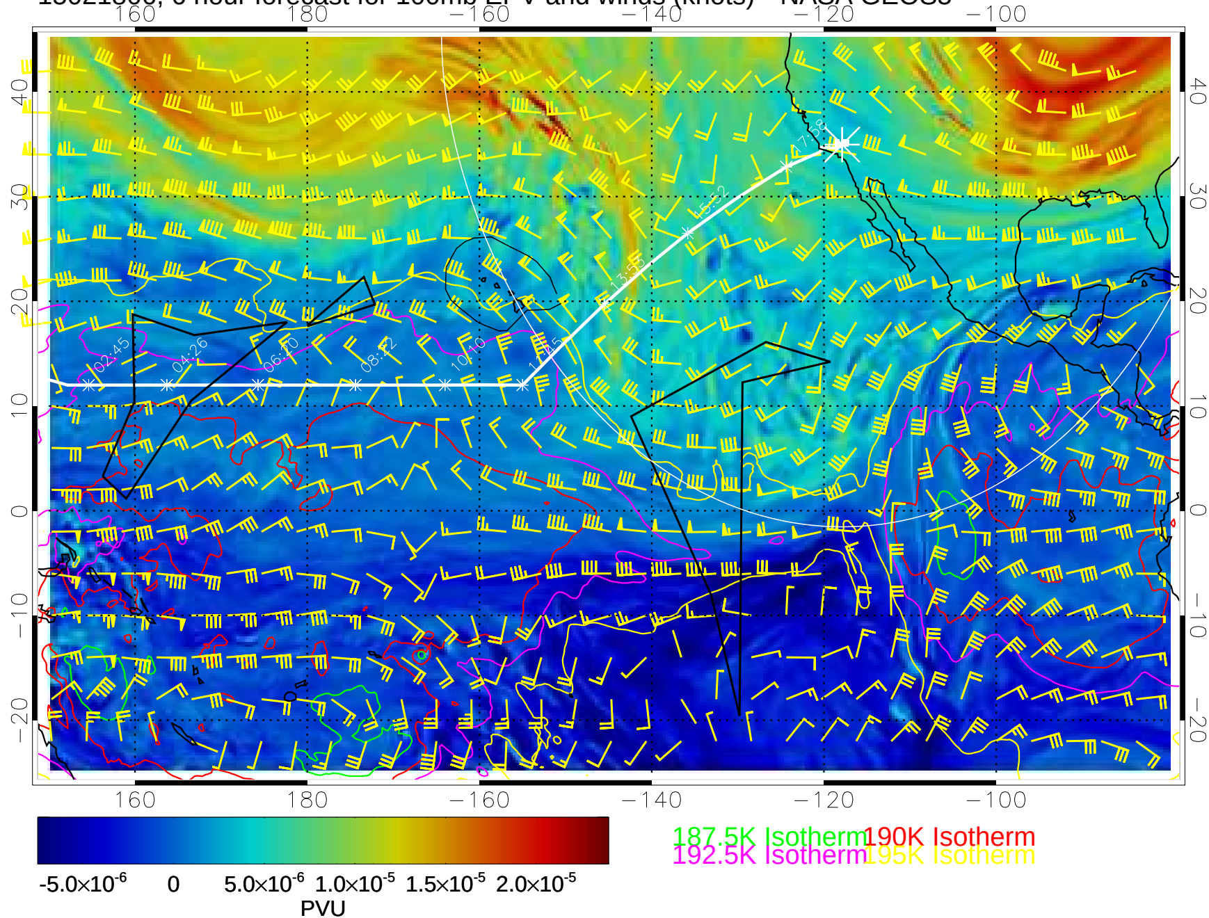
15021806, 6 hour forecast for 100mb EPV and winds (knots)-- NASA GEOS5
