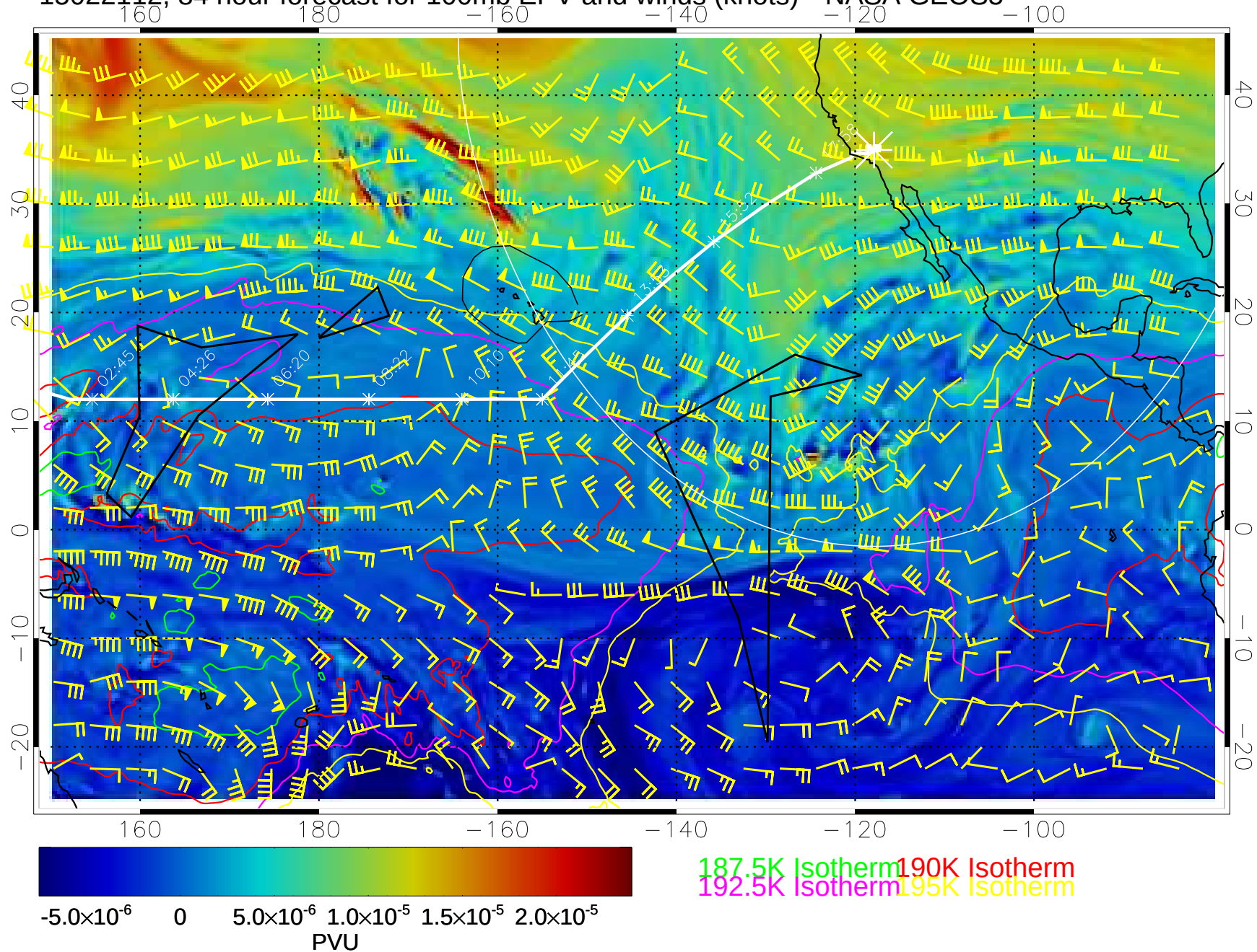
15022112, 84 hour forecast for 100mb EPV and winds (knots)-- NASA GEOS5
