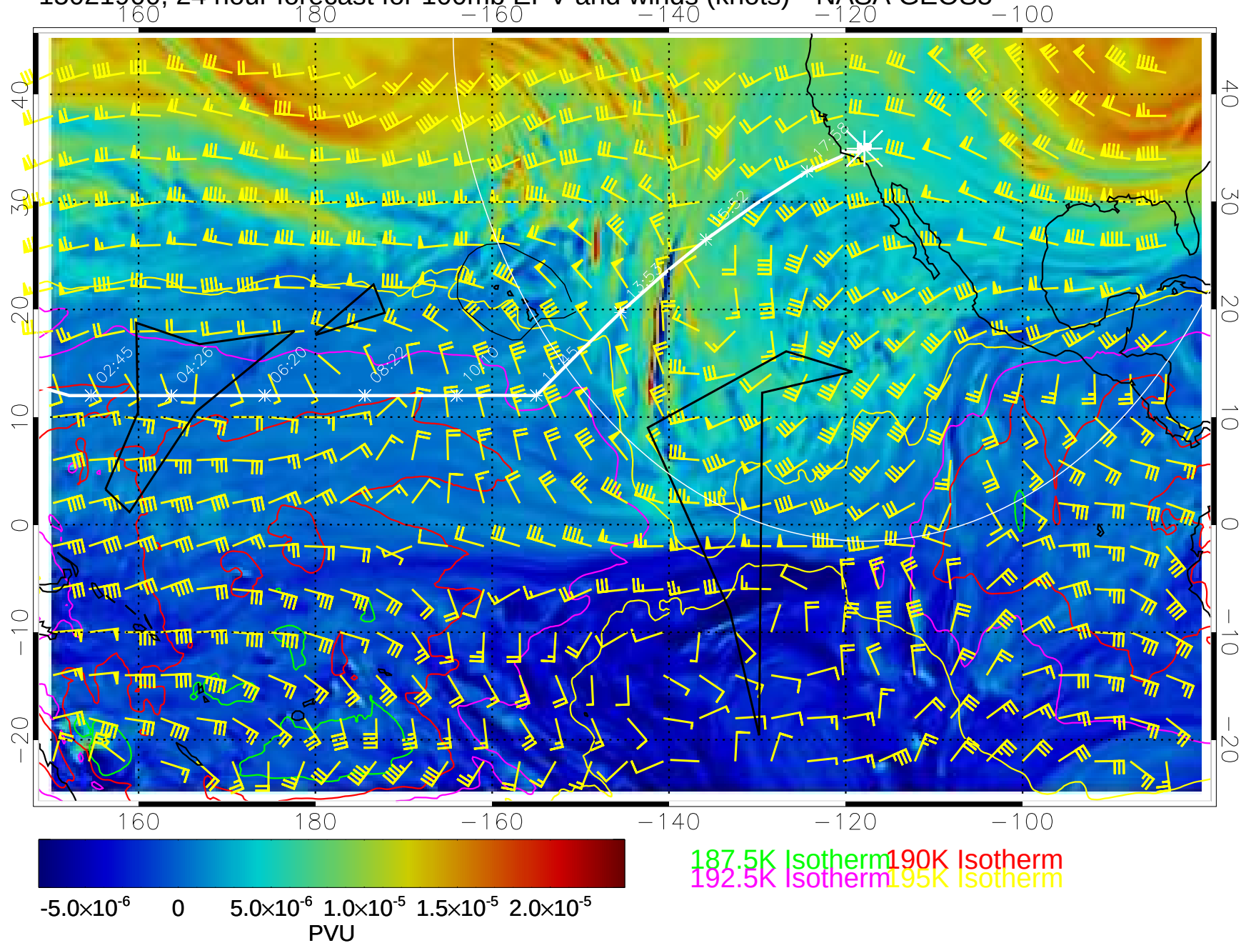
15021900, 24 hour forecast for 100mb EPV and winds (knots)-- NASA GEOS5
