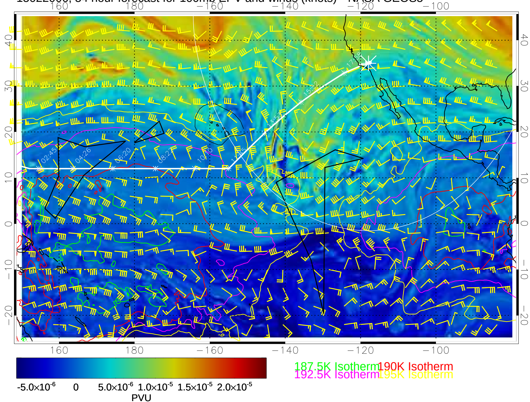
15022006, 54 hour forecast for 100mb EPV and winds (knots)-- NASA GEOS5
