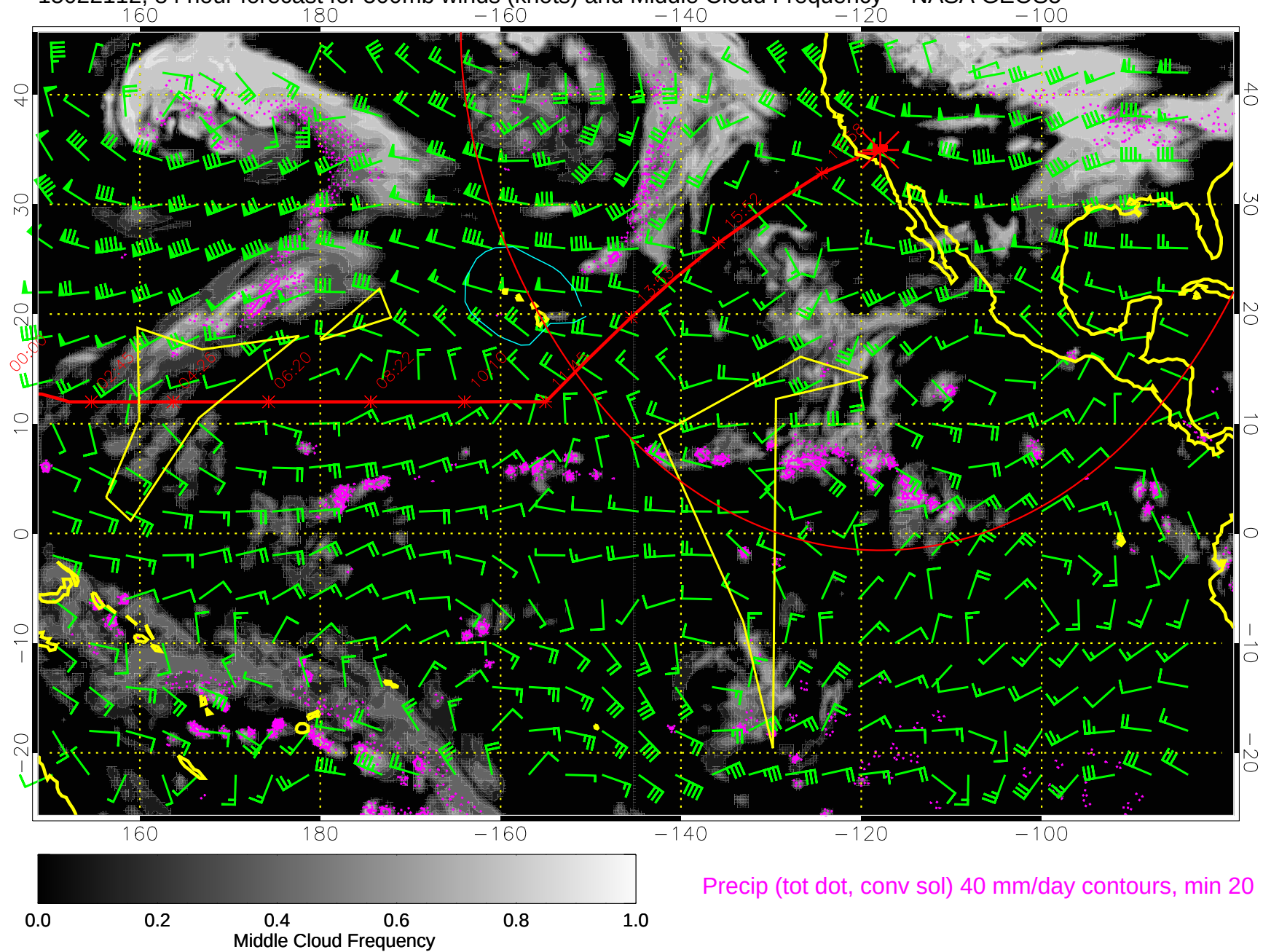
15022112, 84 hour forecast for 500mb winds (knots) and Middle Cloud Frequency -- NASA GEOS5
