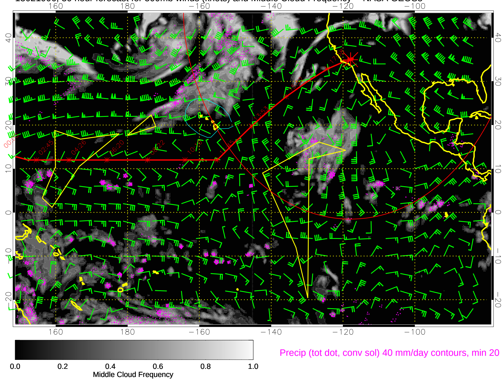
15021906, 30 hour forecast for 500mb winds (knots) and Middle Cloud Frequency -- NASA GEOS5
