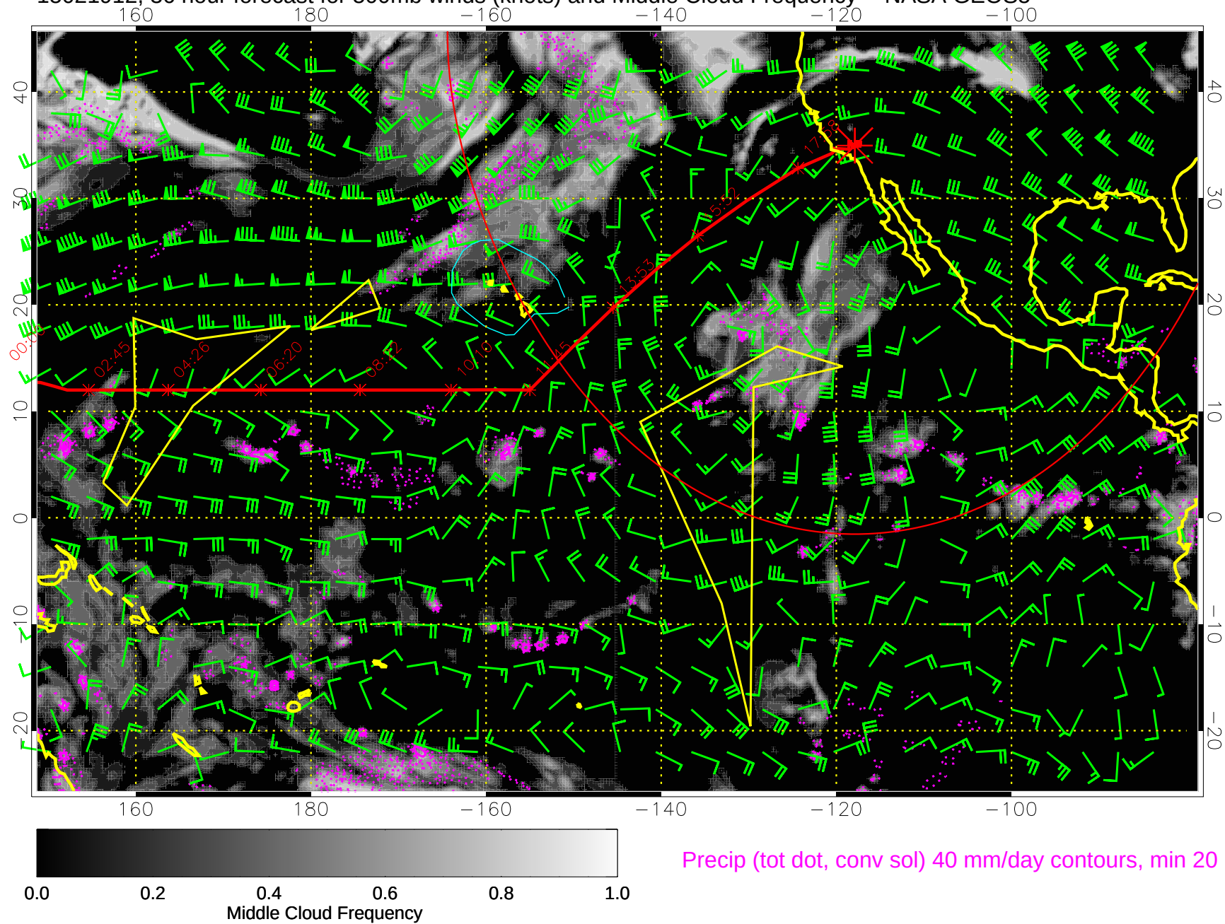
15021912, 36 hour forecast for 500mb winds (knots) and Middle Cloud Frequency -- NASA GEOS5
