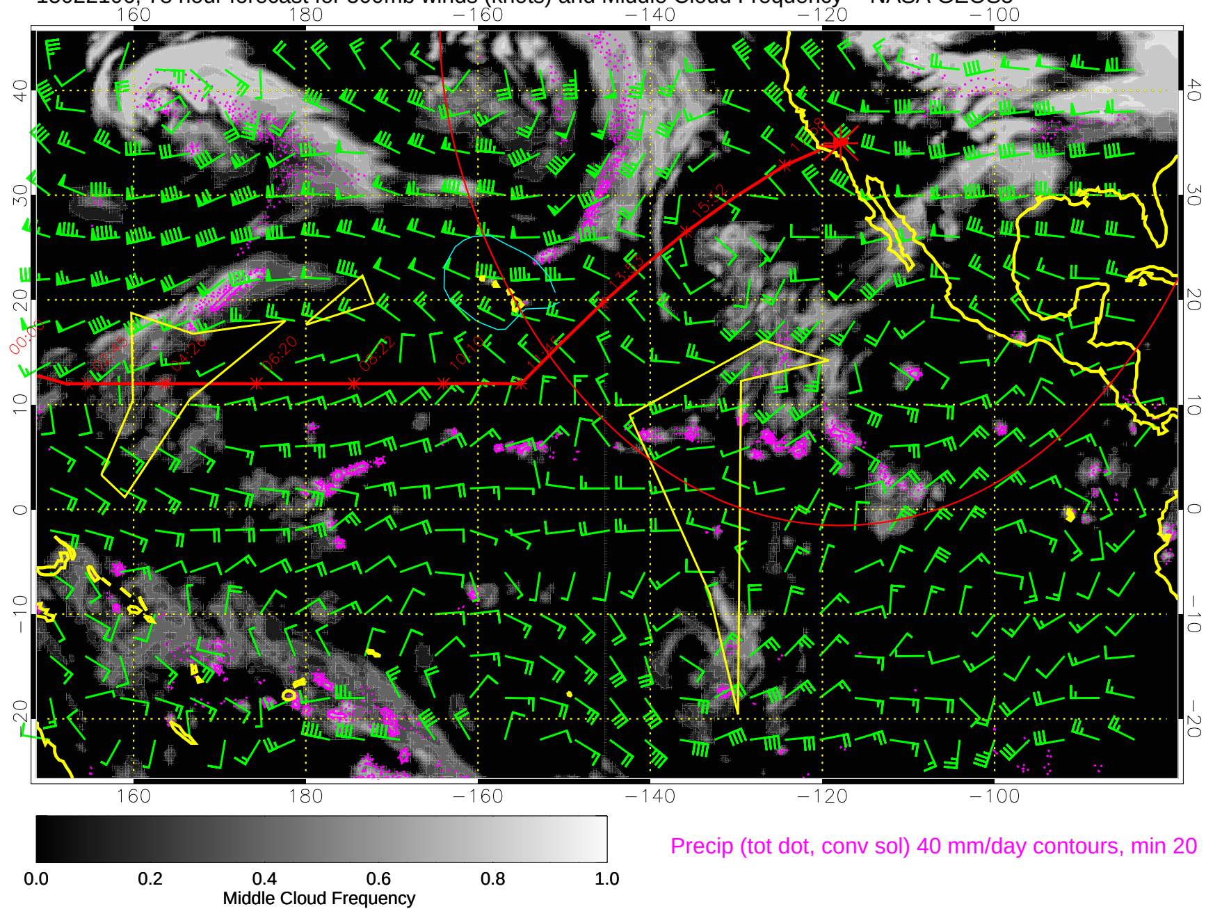
15022106, 78 hour forecast for 500mb winds (knots) and Middle Cloud Frequency -- NASA GEOS5
