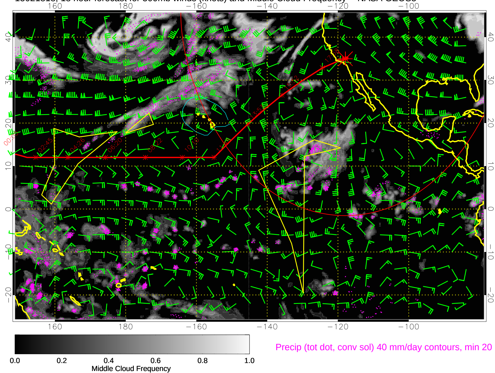
15021818, 18 hour forecast for 500mb winds (knots) and Middle Cloud Frequency -- NASA GEOS5
