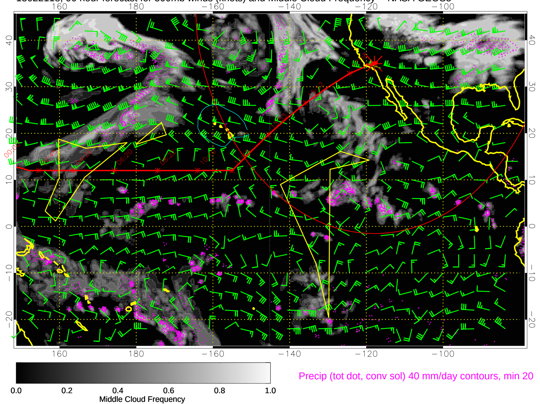
15022118, 90 hour forecast for 500mb winds (knots) and Middle Cloud Frequency -- NASA GEOS5
