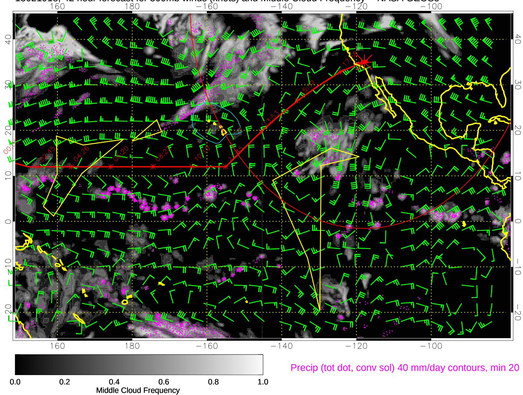
15021918, 42 hour forecast for 500mb winds (knots) and Middle Cloud Frequency -- NASA GEOS5
