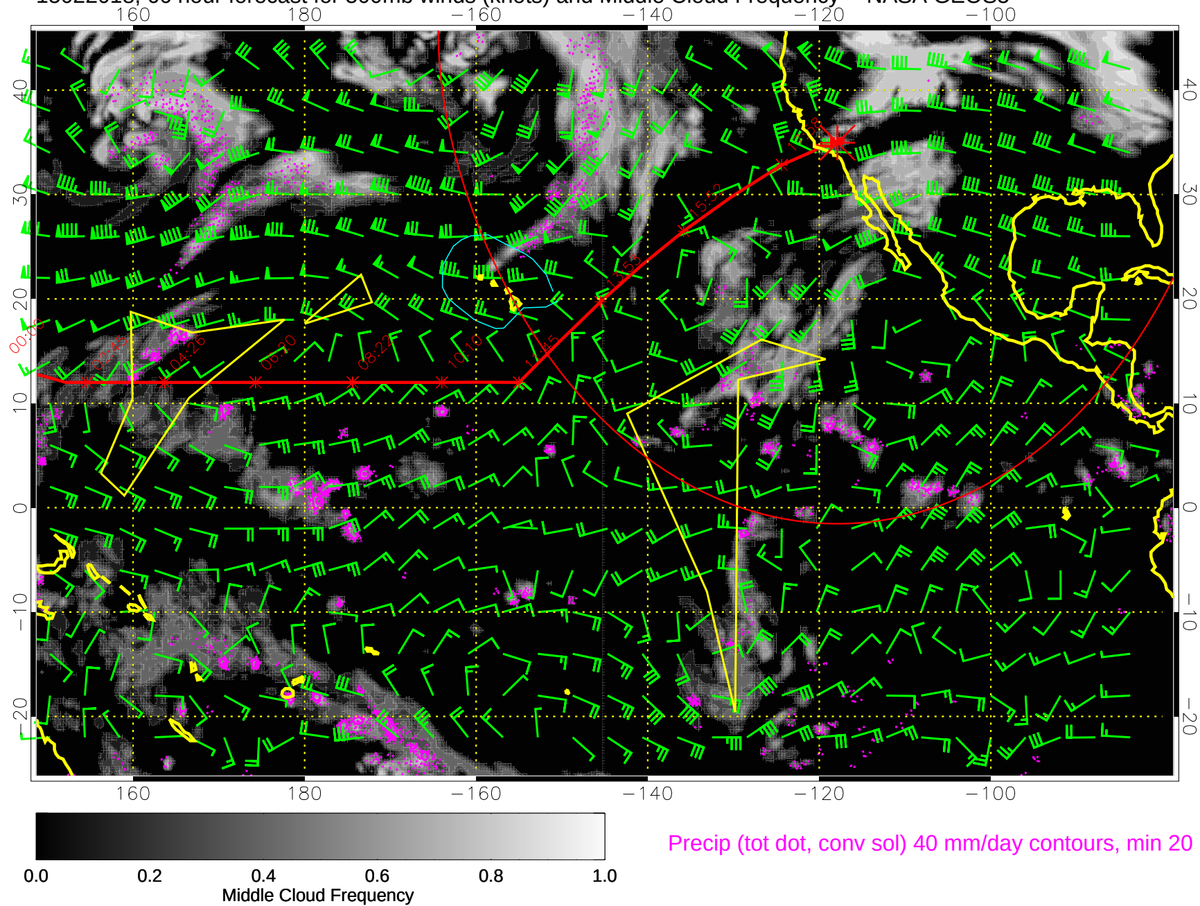
15022018, 66 hour forecast for 500mb winds (knots) and Middle Cloud Frequency -- NASA GEOS5
