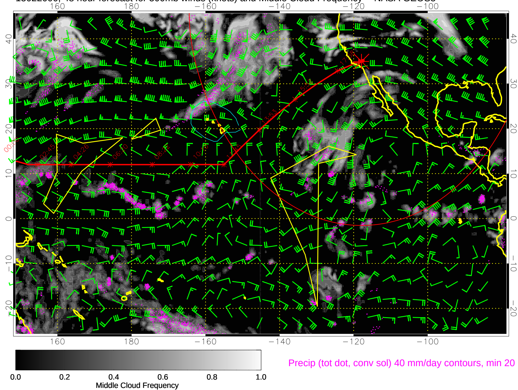
15022000, 48 hour forecast for 500mb winds (knots) and Middle Cloud Frequency -- NASA GEOS5
