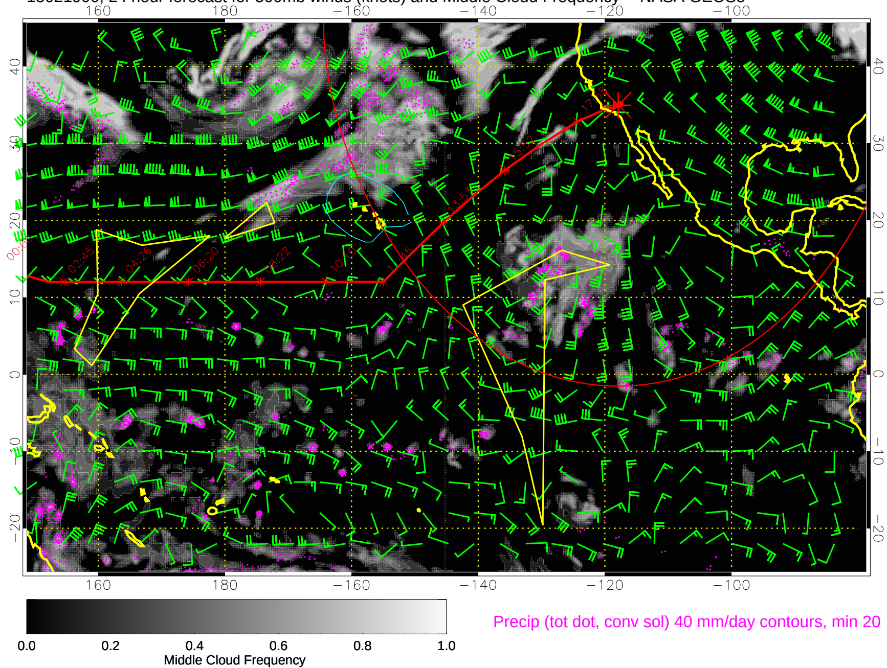
15021900, 24 hour forecast for 500mb winds (knots) and Middle Cloud Frequency -- NASA GEOS5
