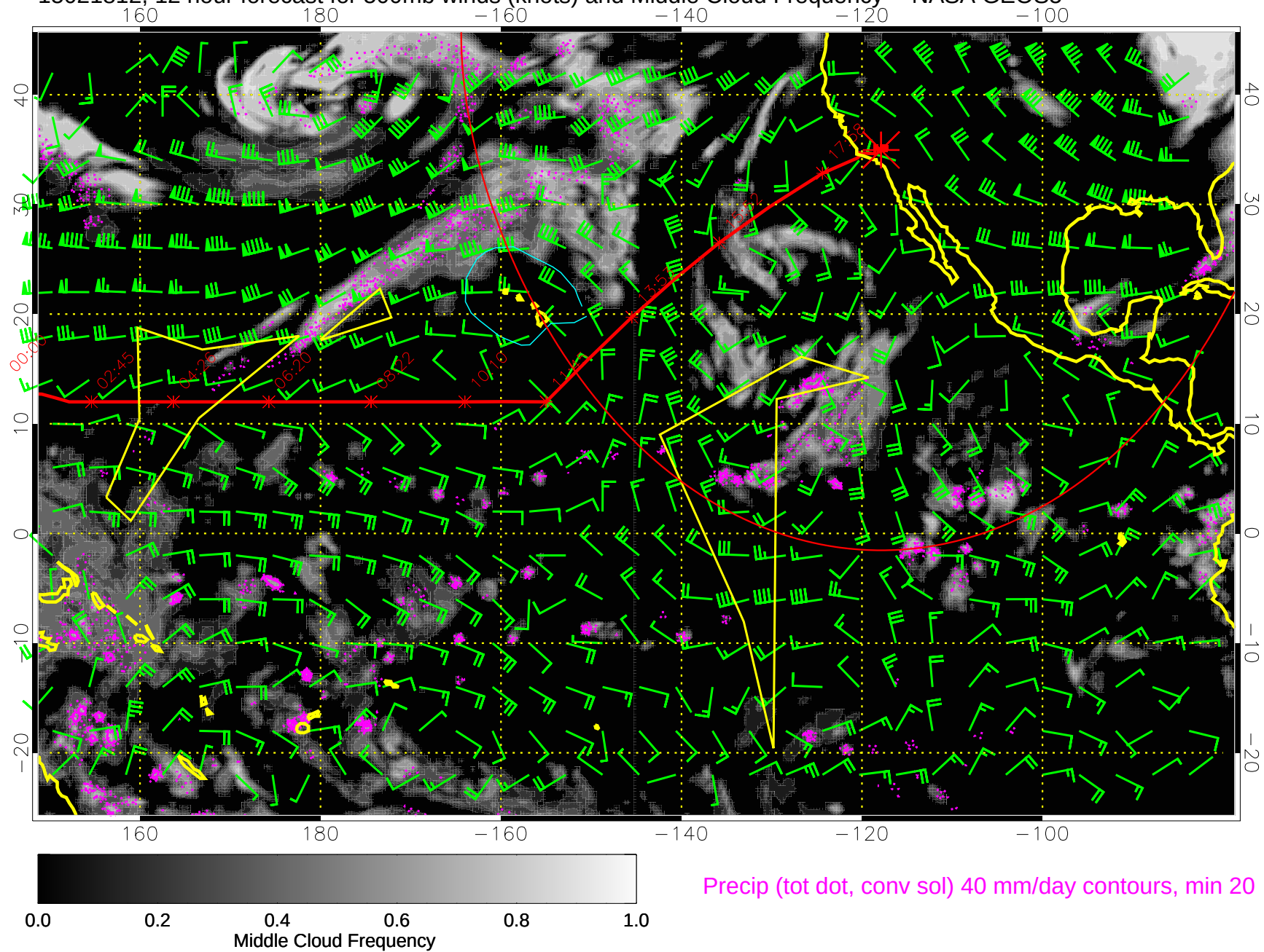
15021812, 12 hour forecast for 500mb winds (knots) and Middle Cloud Frequency -- NASA GEOS5
