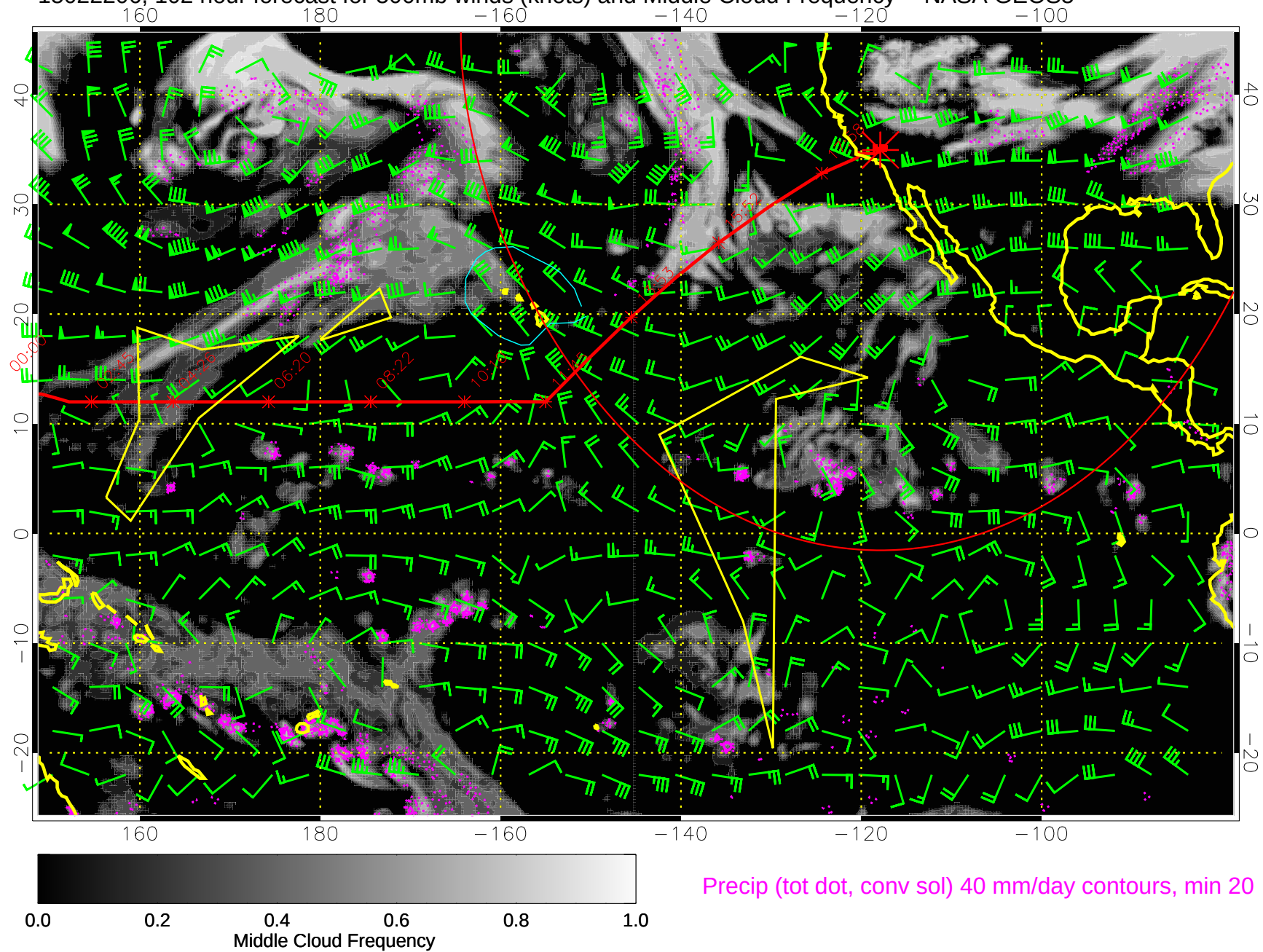
15022206, 102 hour forecast for 500mb winds (knots) and Middle Cloud Frequency -- NASA GEOS5
