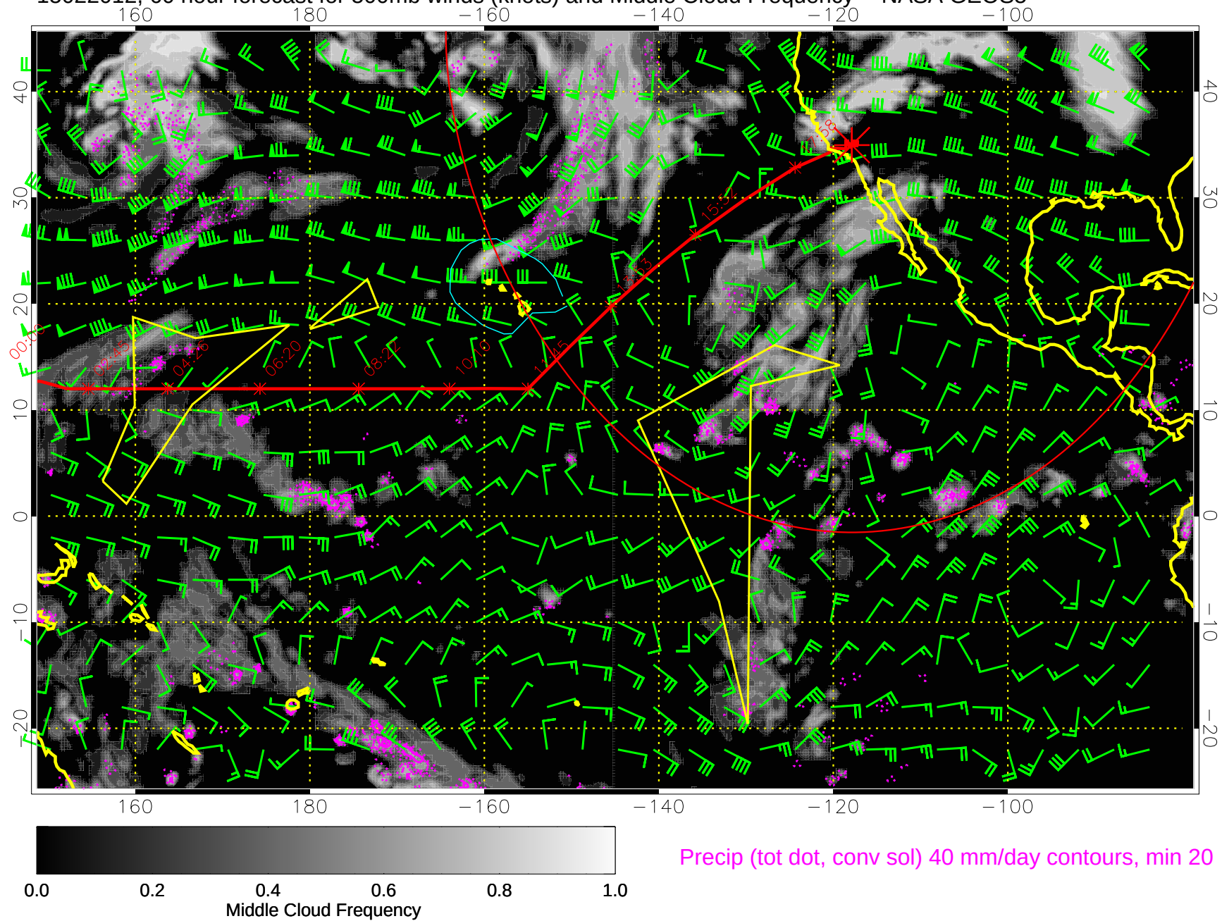
15022012, 60 hour forecast for 500mb winds (knots) and Middle Cloud Frequency -- NASA GEOS5
