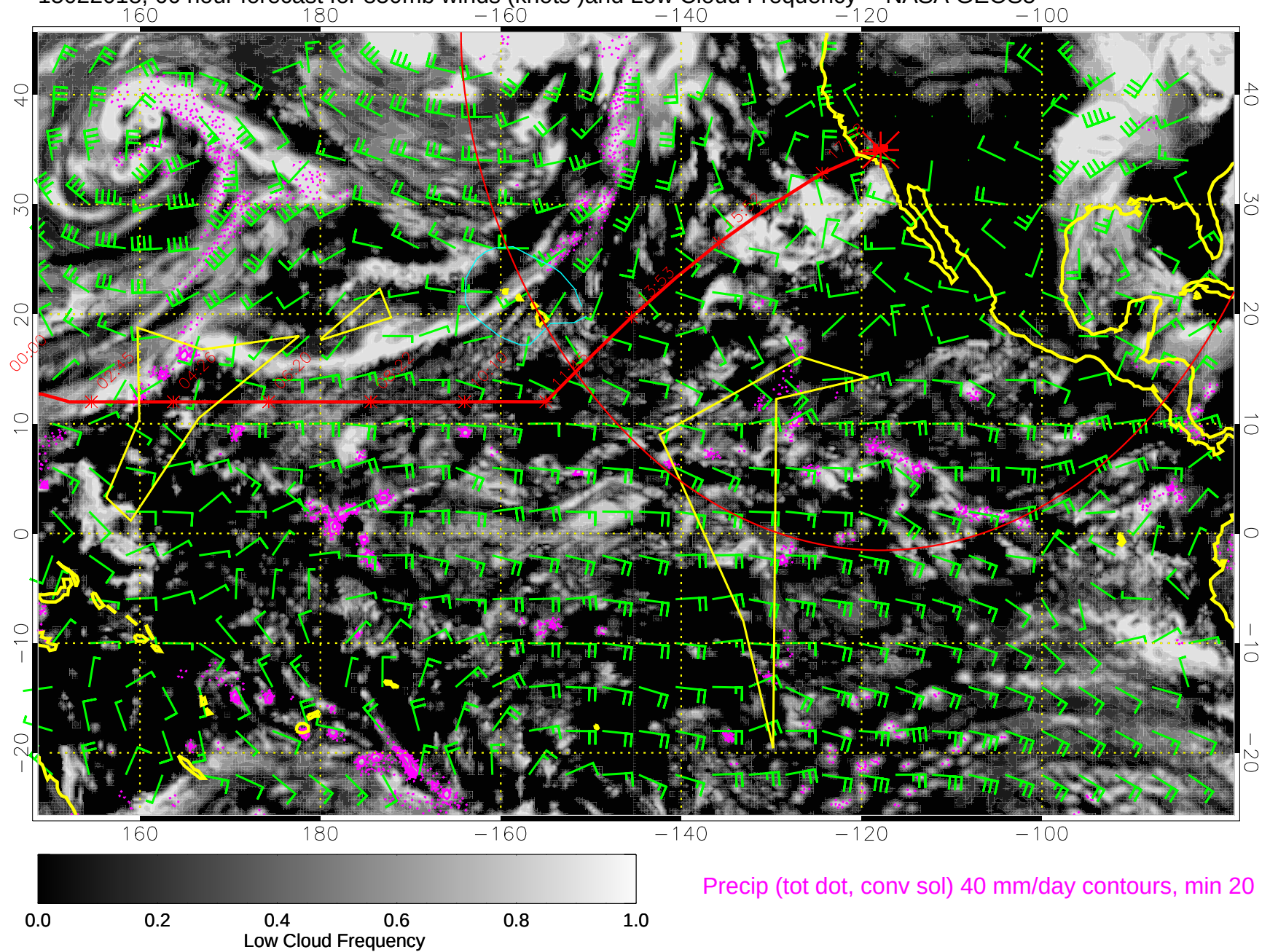
15022018, 66 hour forecast for 850mb winds (knots) and Low Cloud Frequency -- NASA GEOS5
