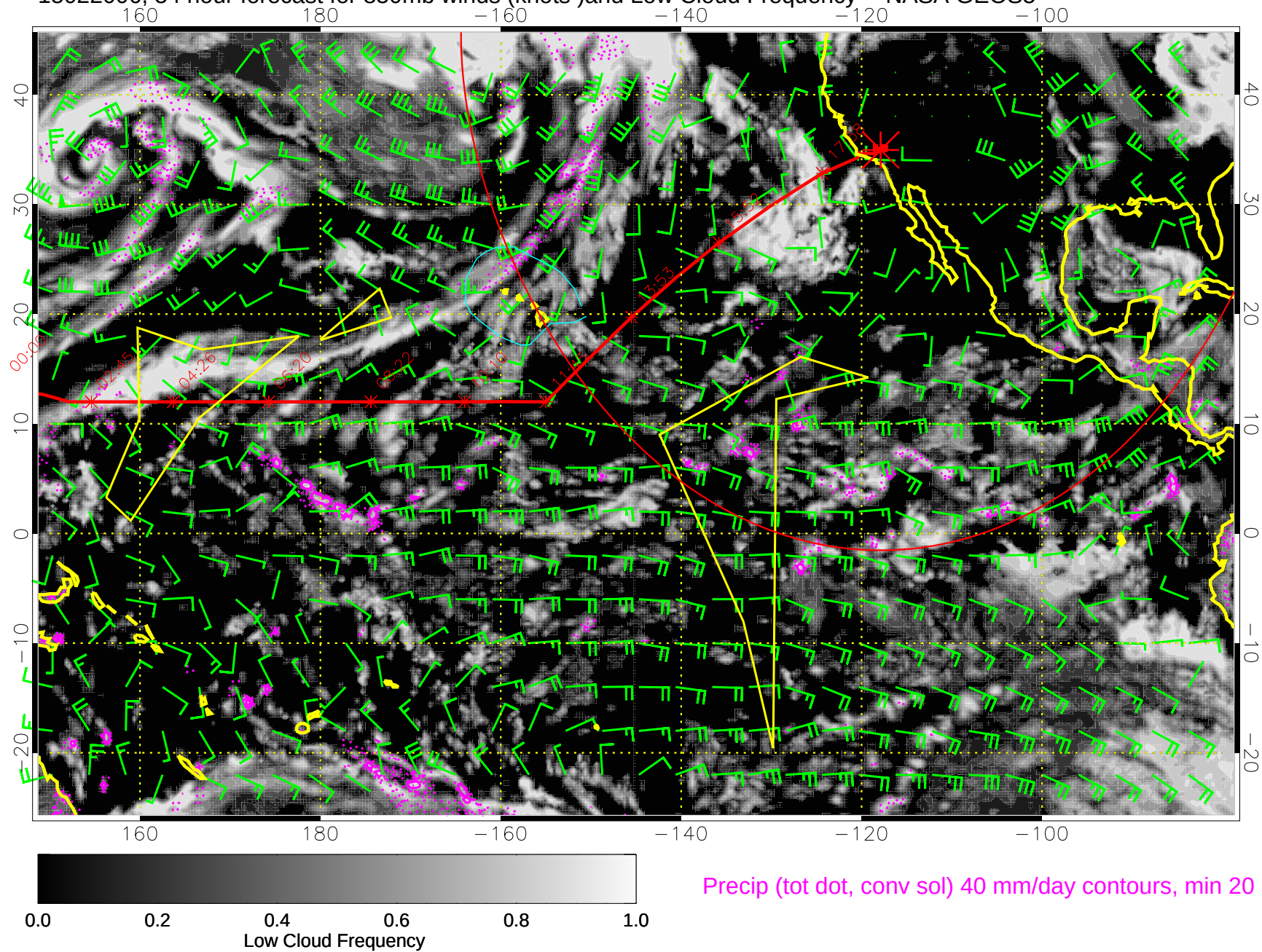
15022006, 54 hour forecast for 850mb winds (knots) and Low Cloud Frequency -- NASA GEOS5
