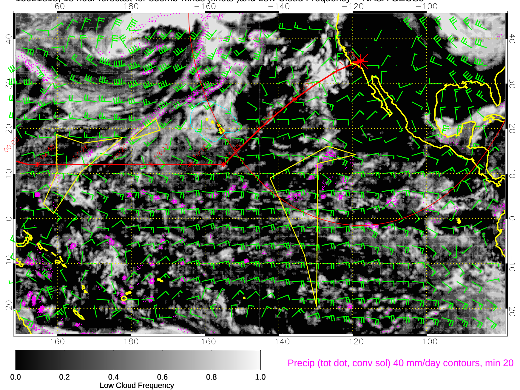
15021818, 18 hour forecast for 850mb winds (knots) and Low Cloud Frequency -- NASA GEOS5
