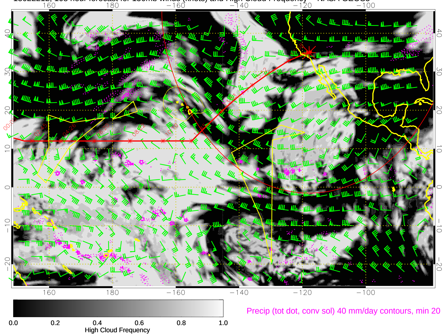
15022212, 108 hour forecast for 150mb winds (knots) and High Cloud Frequency -- NASA GEOS5
