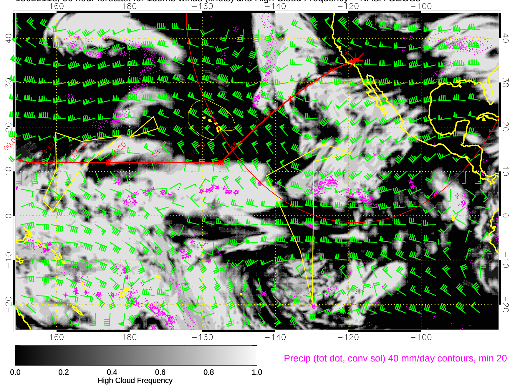
15022118, 90 hour forecast for 150mb winds (knots) and High Cloud Frequency -- NASA GEOS5
