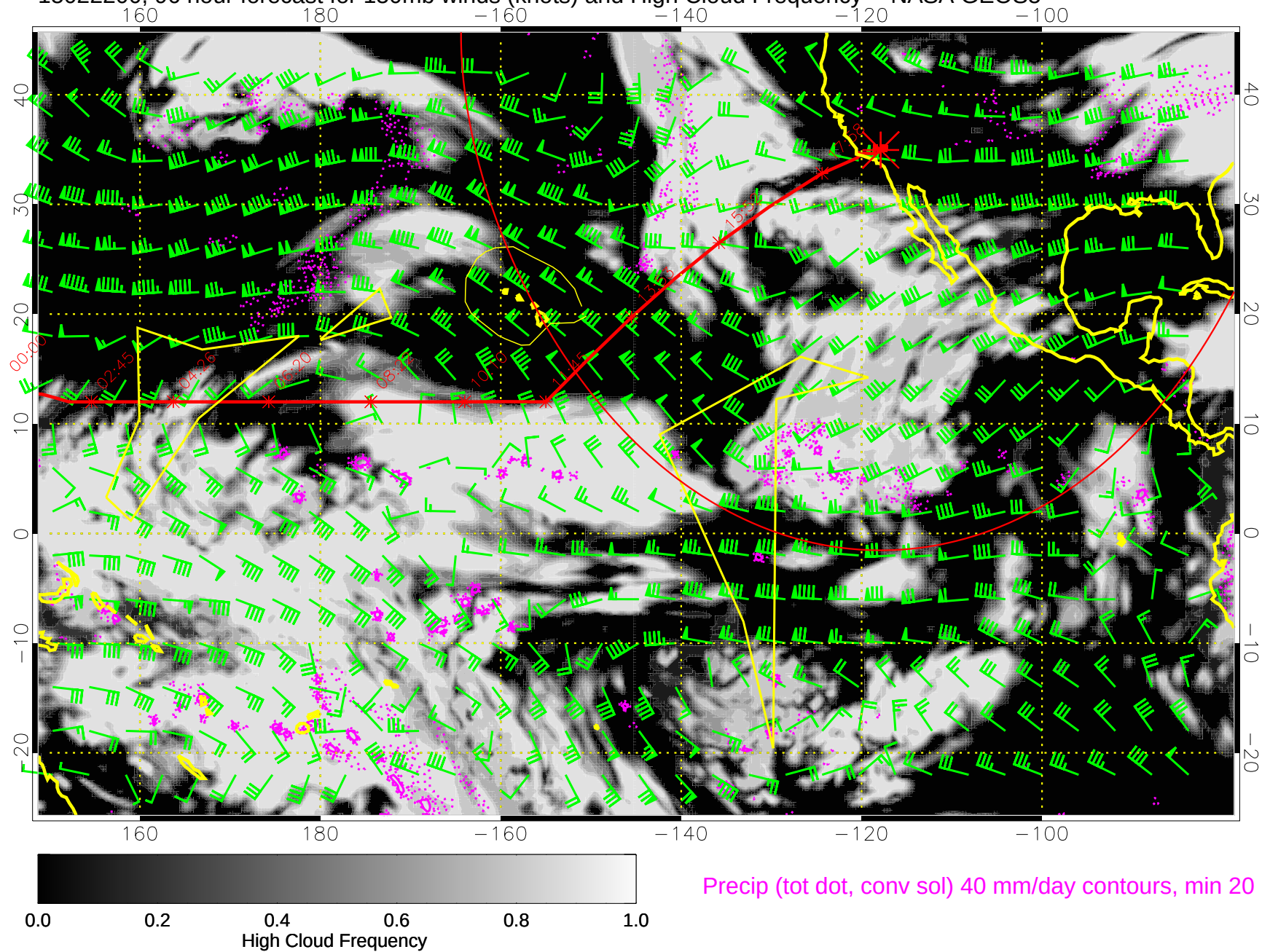
15022200, 96 hour forecast for 150mb winds (knots) and High Cloud Frequency -- NASA GEOS5
