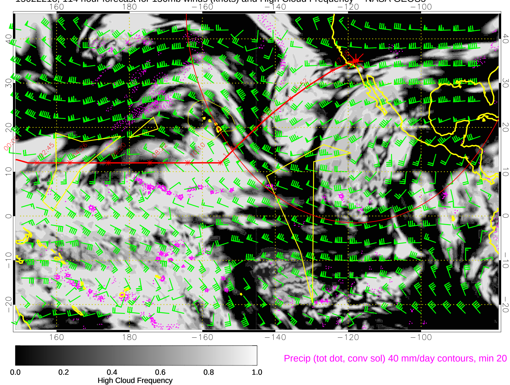
15022218, 114 hour forecast for 150mb winds (knots) and High Cloud Frequency -- NASA GEOS5
