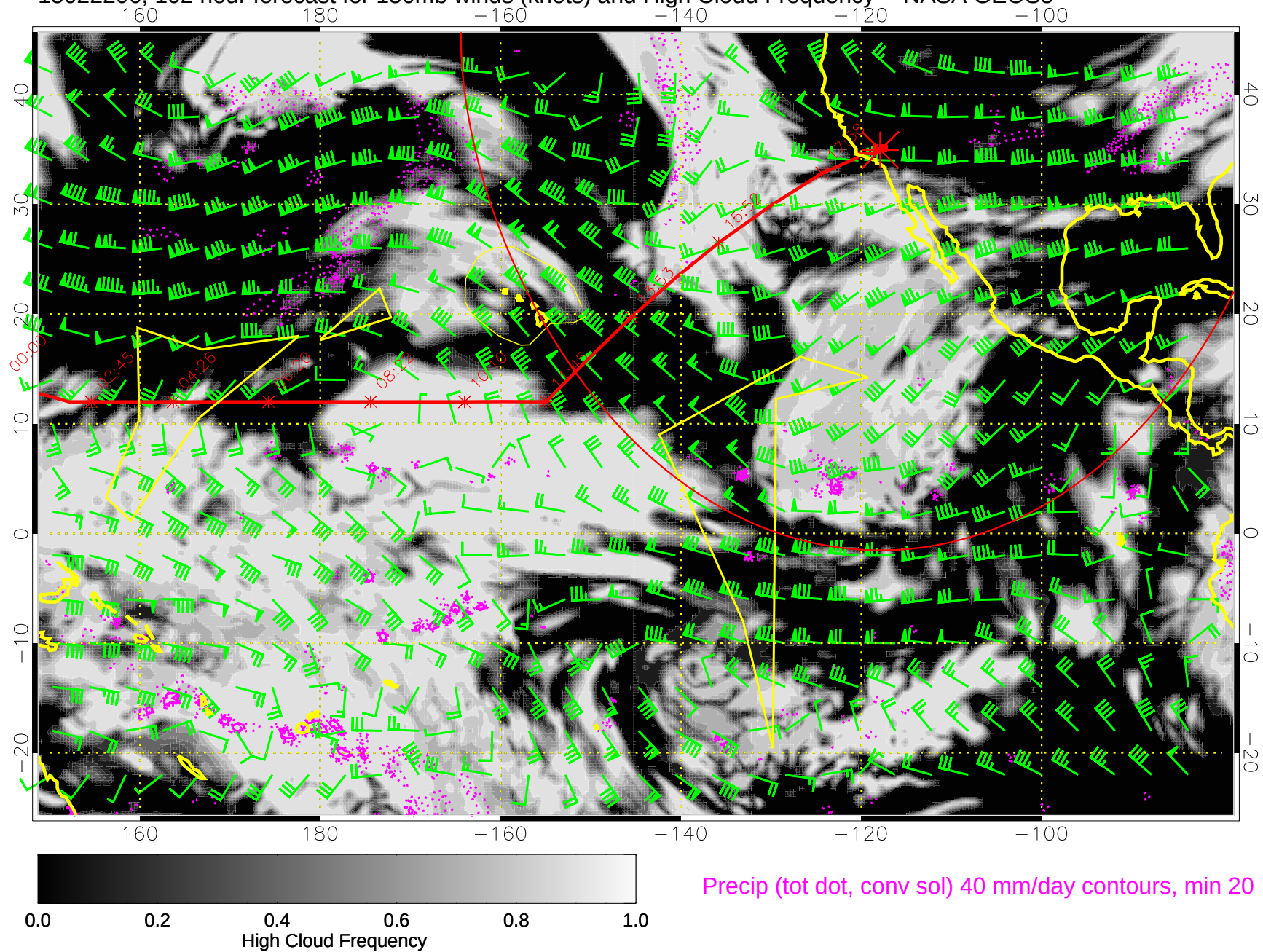
15022206, 102 hour forecast for 150mb winds (knots) and High Cloud Frequency -- NASA GEOS5
