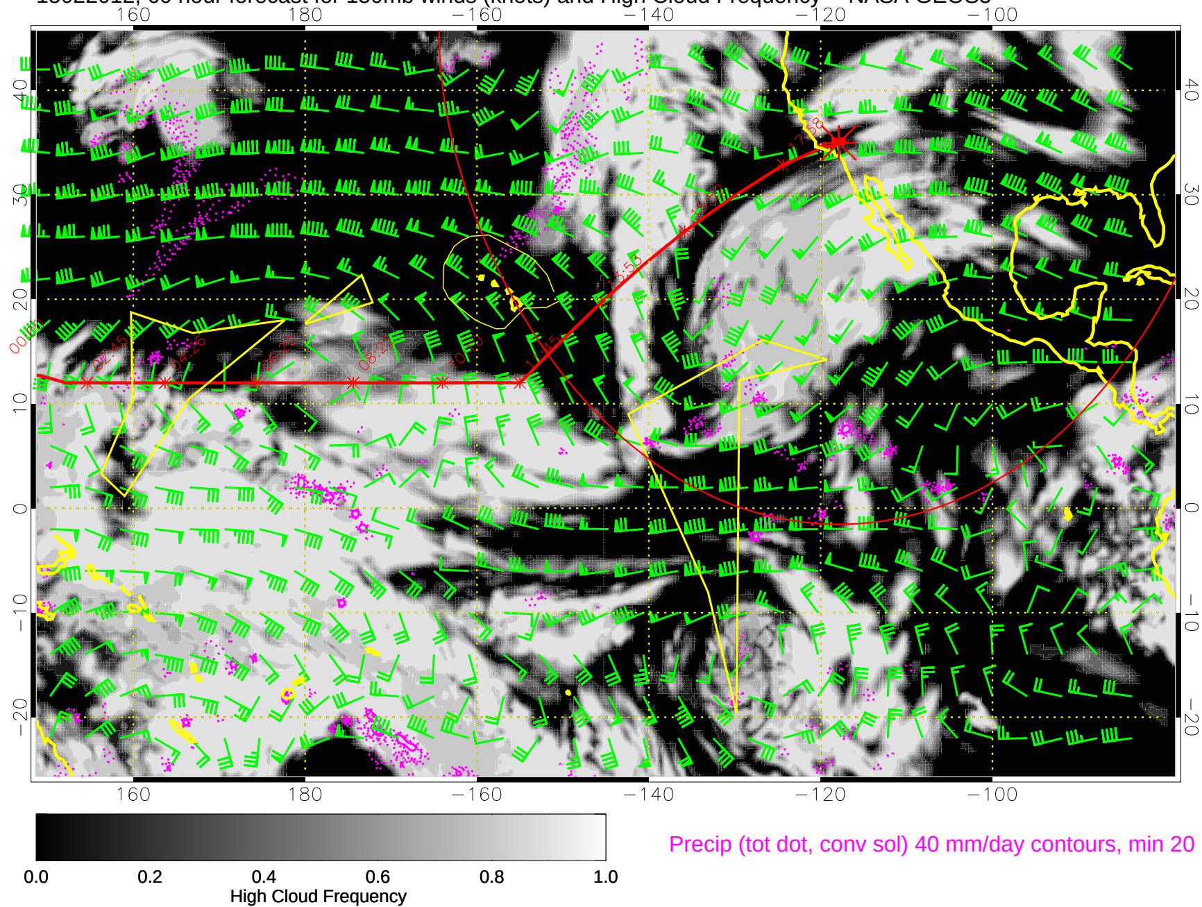
15022012, 60 hour forecast for 150mb winds (knots) and High Cloud Frequency -- NASA GEOS5
