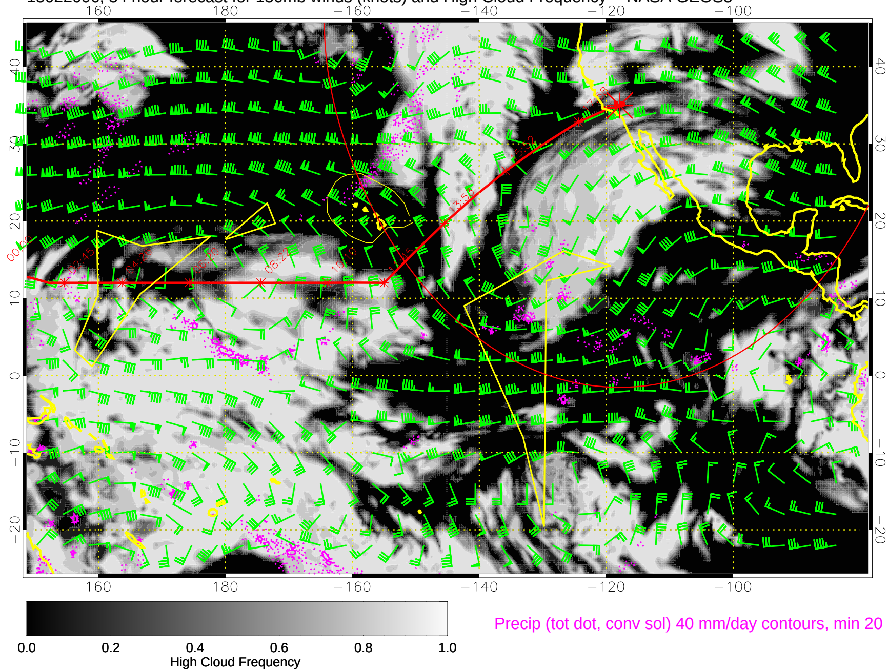
15022006, 54 hour forecast for 150mb winds (knots) and High Cloud Frequency -- NASA GEOS5
