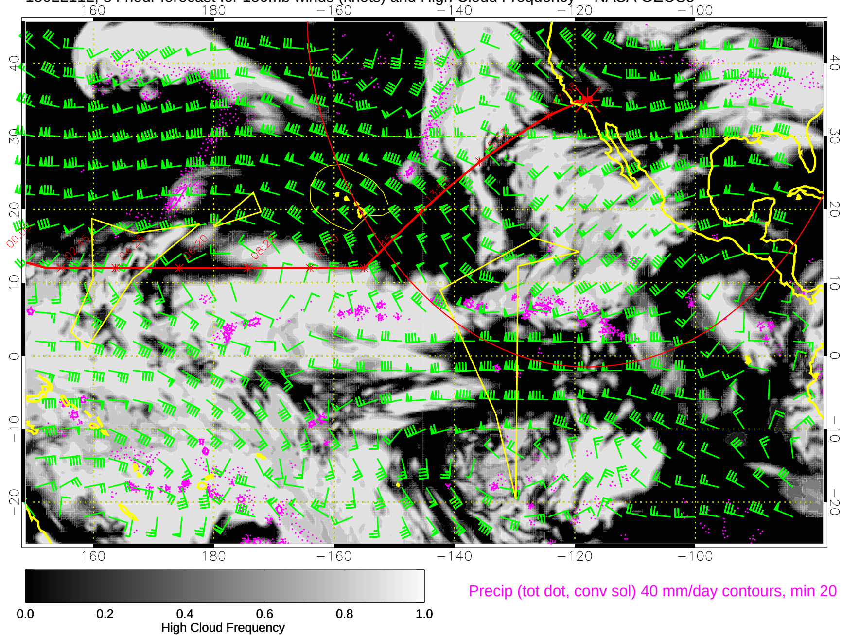
15022112, 84 hour forecast for 150mb winds (knots) and High Cloud Frequency -- NASA GEOS5
