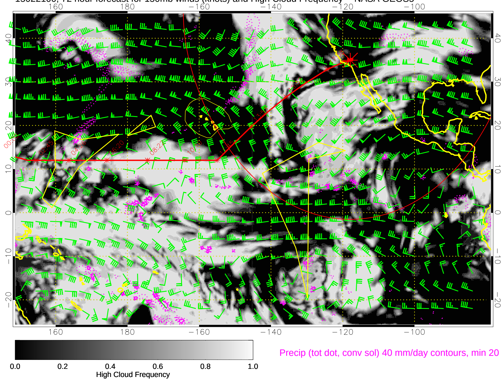
15022100, 72 hour forecast for 150mb winds (knots) and High Cloud Frequency -- NASA GEOS5
