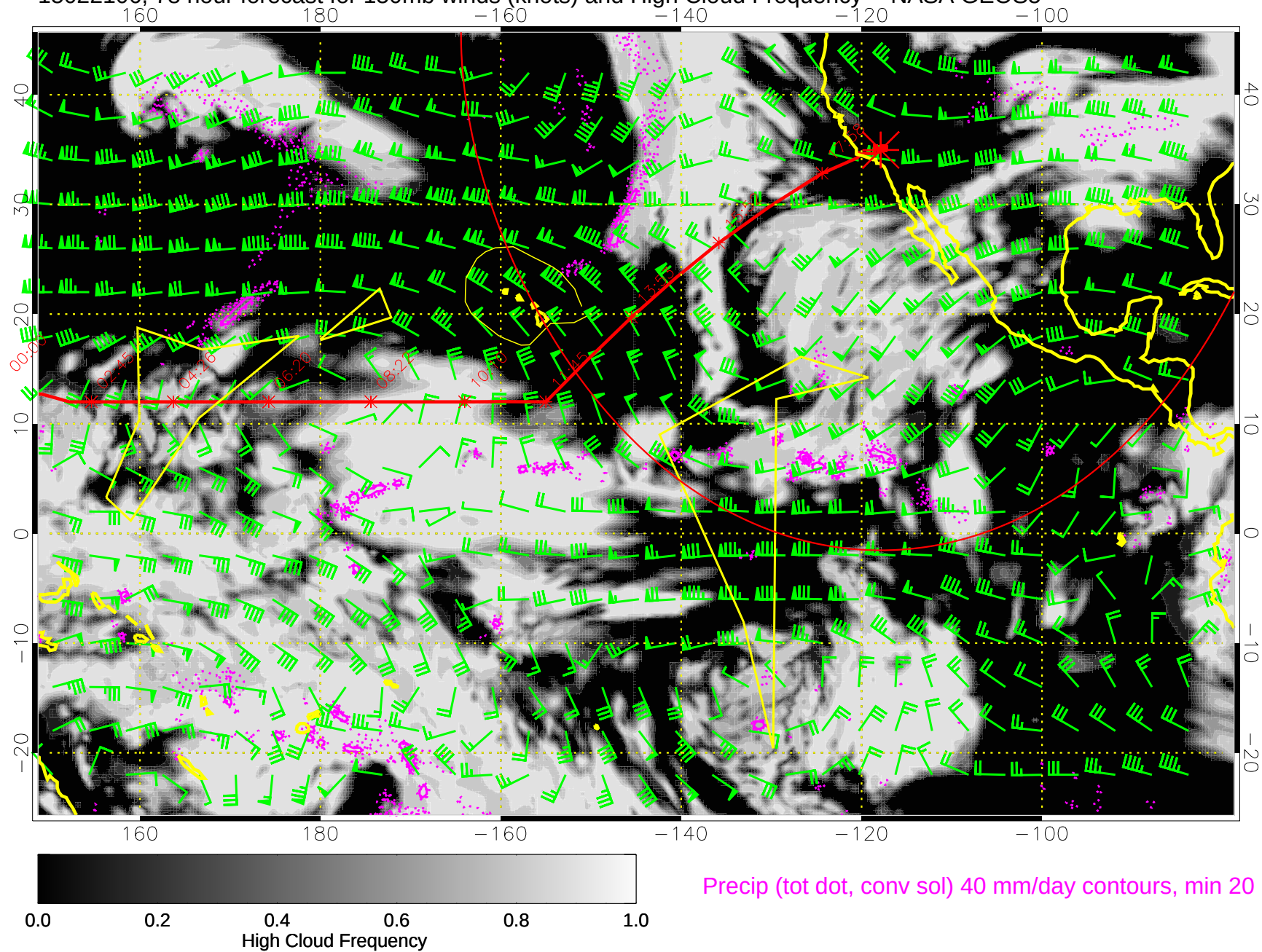
15022106, 78 hour forecast for 150mb winds (knots) and High Cloud Frequency -- NASA GEOS5
