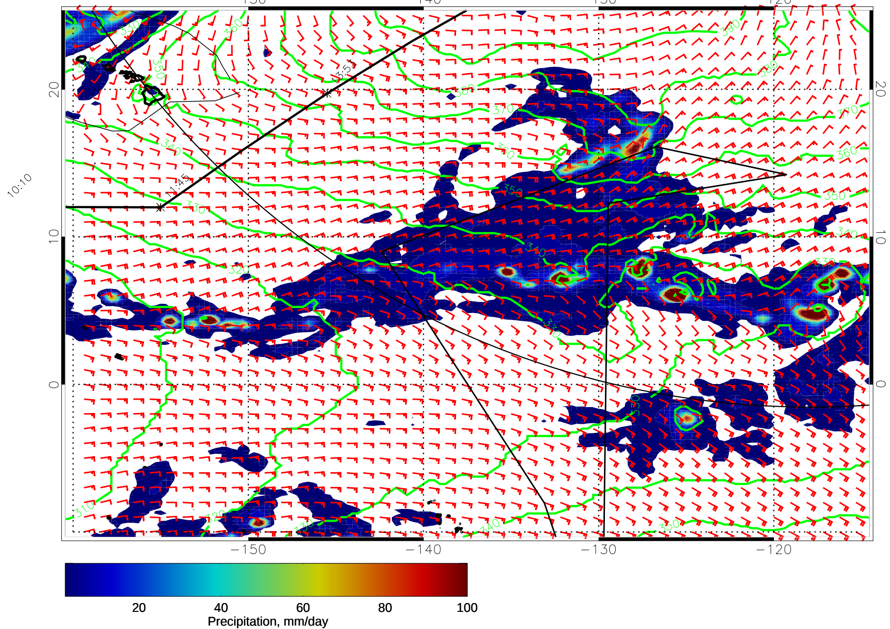
15022006, 78 hour forecast for 975mb Z, Precip., and Surface Winds (knots) -- NASA GEOS5
