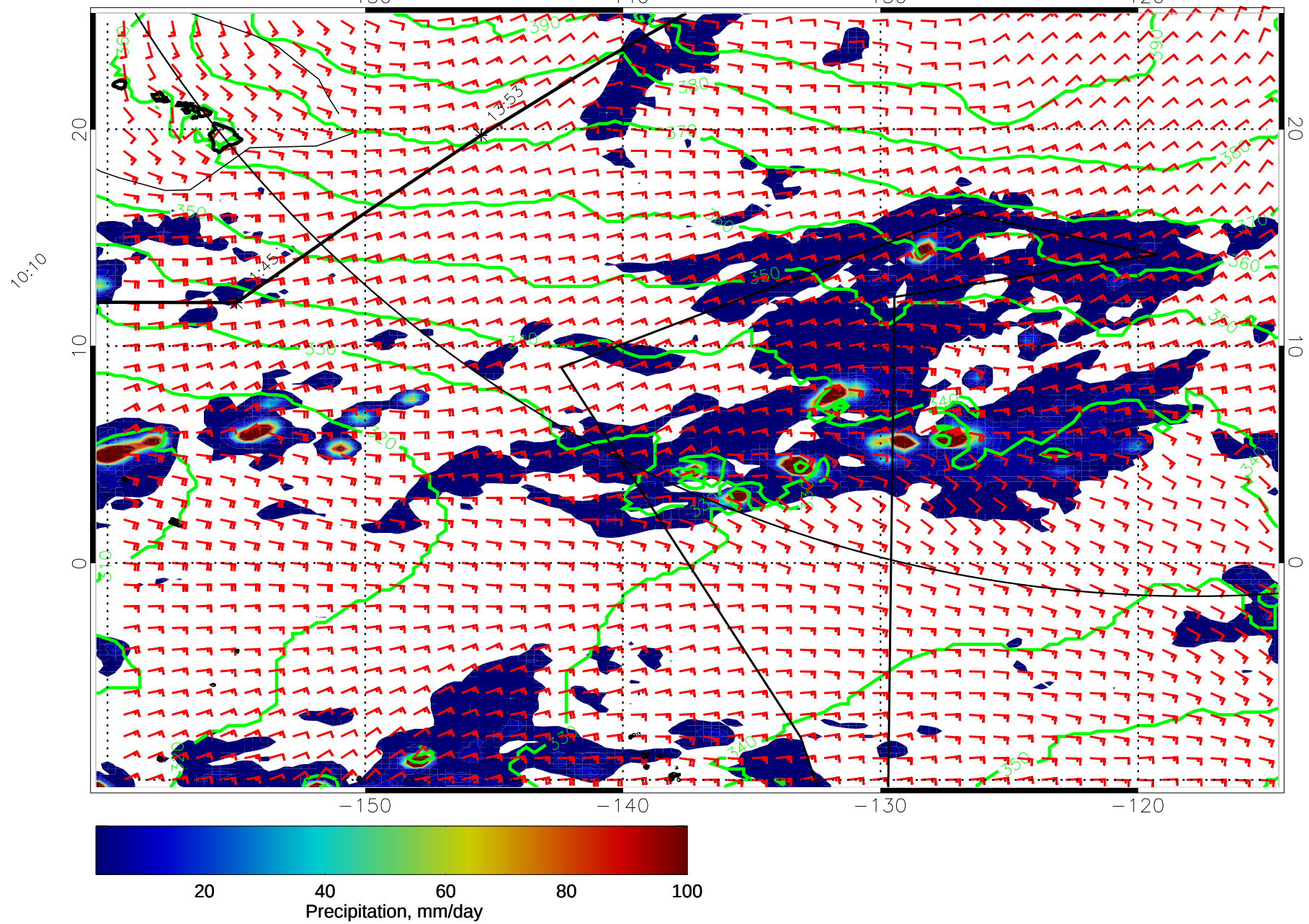
15021818, 42 hour forecast for 975mb Z, Precip., and Surface Winds (knots) -- NASA GEOS5
