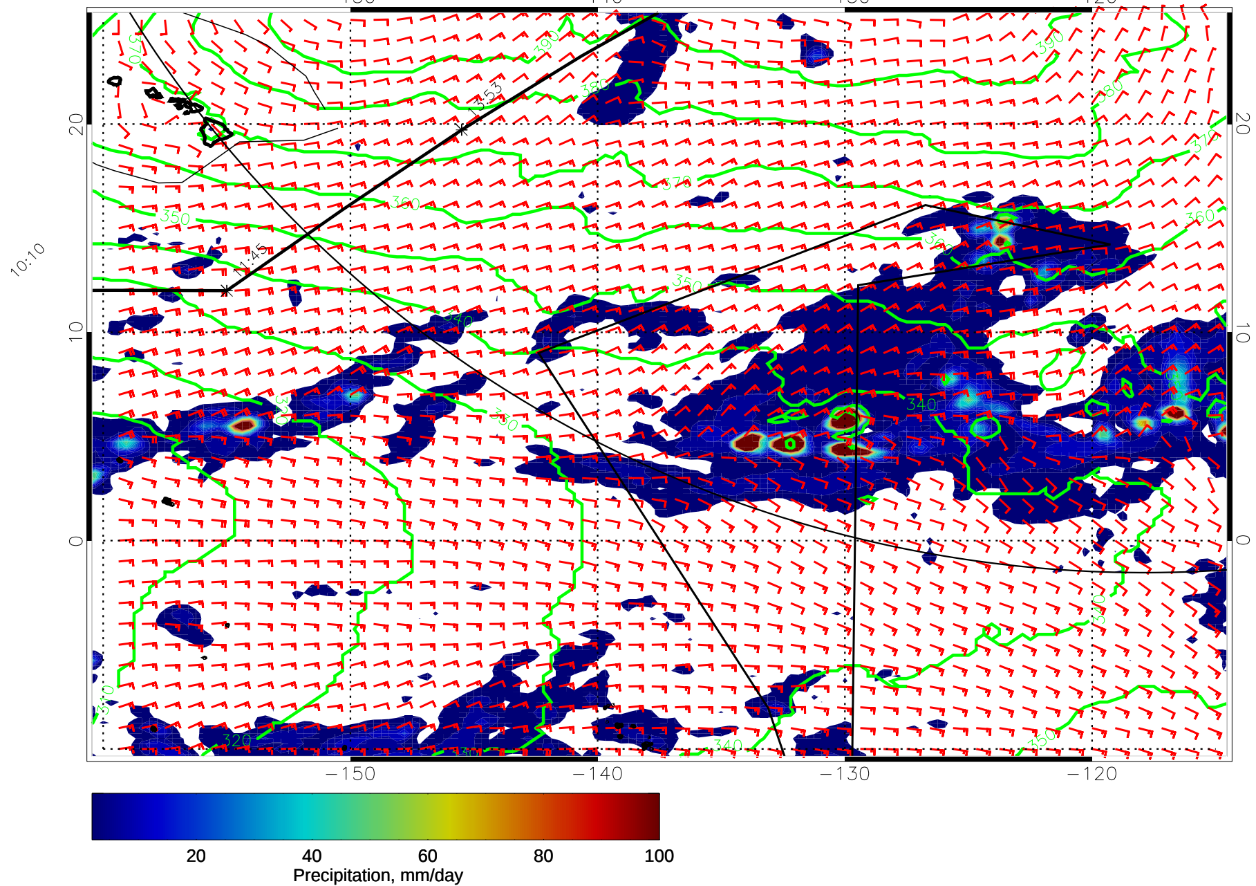
15021806, 30 hour forecast for 975mb Z, Precip., and Surface Winds (knots) -- NASA GEOS5
