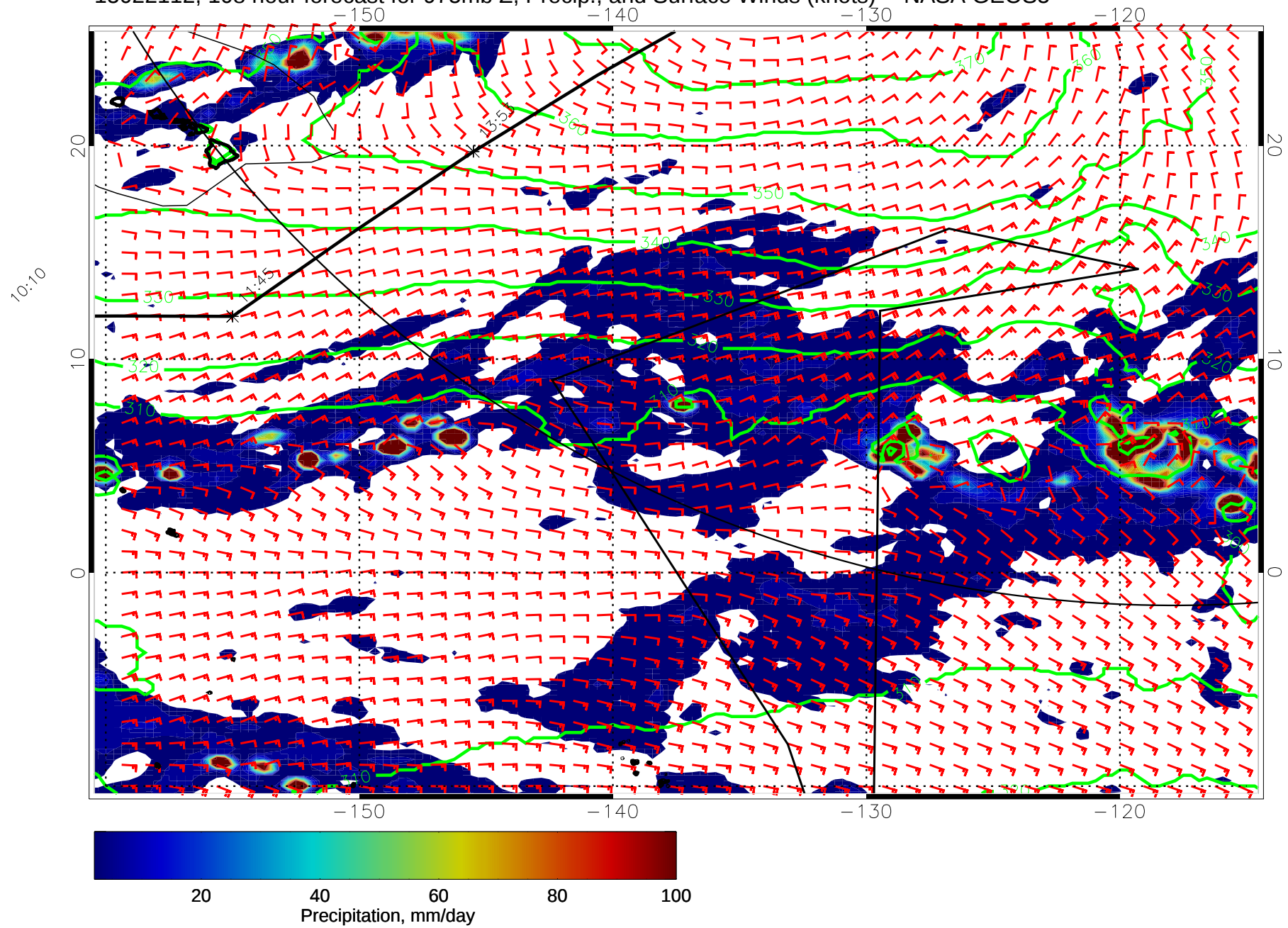
15022112, 108 hour forecast for 975mb Z, Precip., and Surface Winds (knots) -- NASA GEOS5
