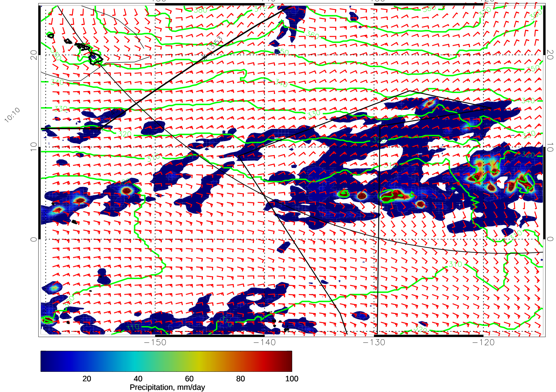
15021800, 24 hour forecast for 975mb Z, Precip., and Surface Winds (knots) -- NASA GEOS5
