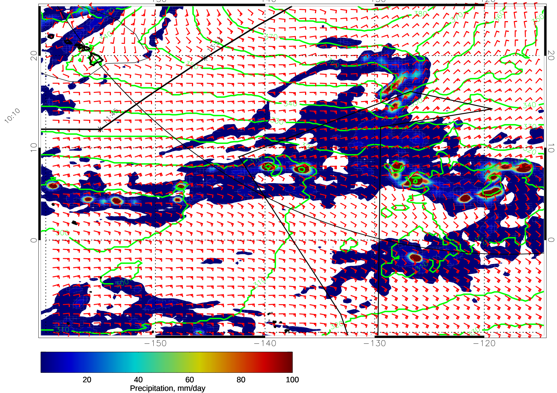
15022012, 84 hour forecast for 975mb Z, Precip., and Surface Winds (knots) -- NASA GEOS5
