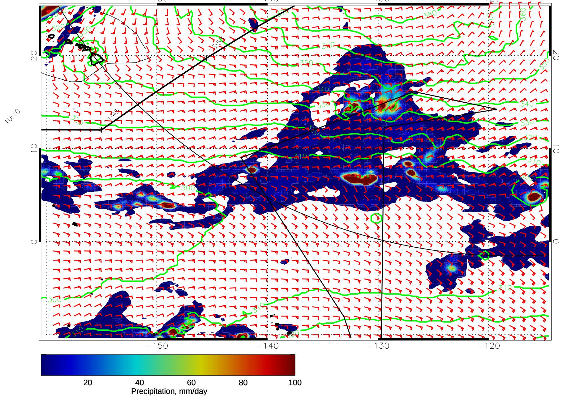
15022000, 72 hour forecast for 975mb Z, Precip., and Surface Winds (knots) -- NASA GEOS5
