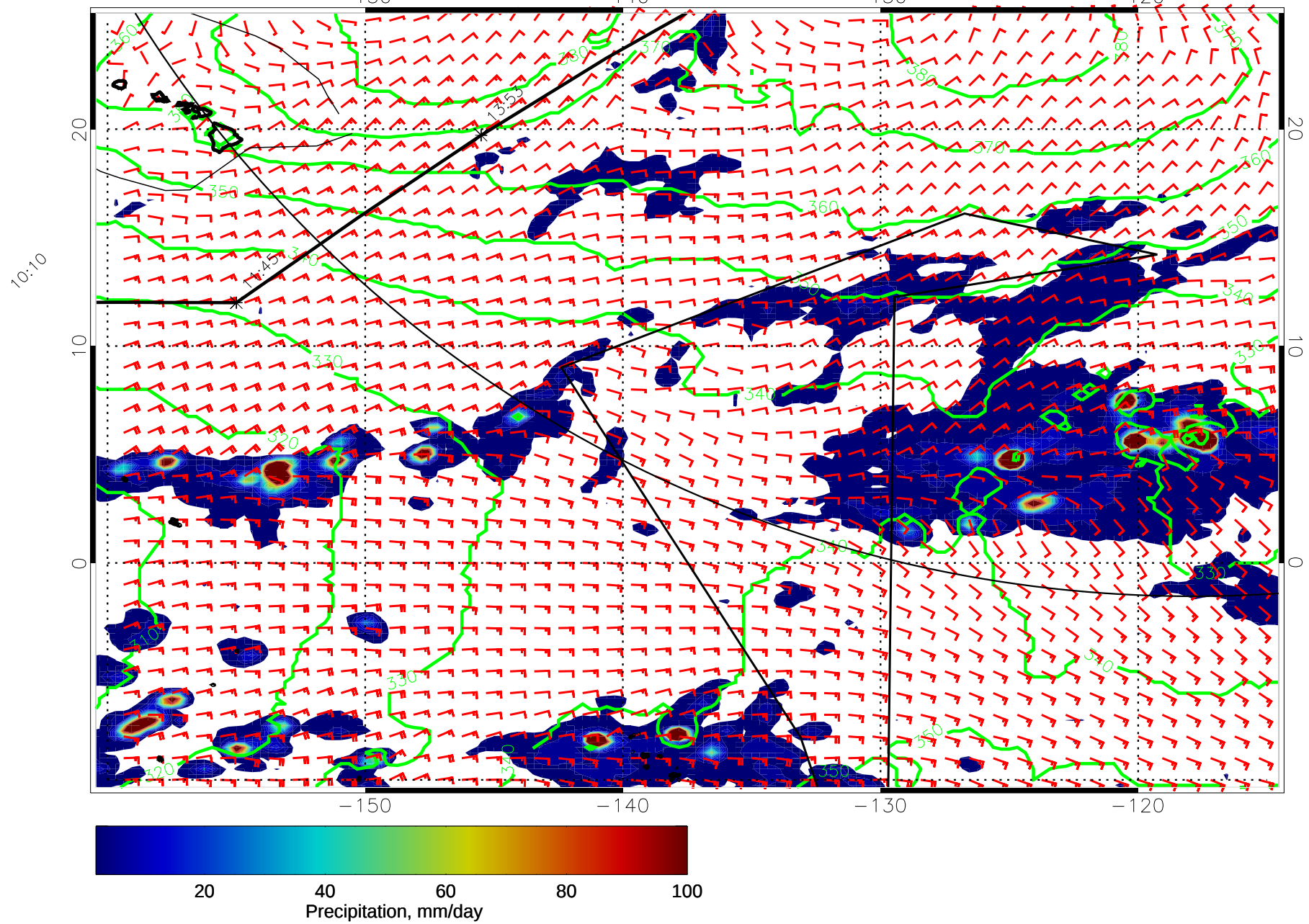
15021706, 6 hour forecast for 975mb Z, Precip., and Surface Winds (knots) -- NASA GEOS5
