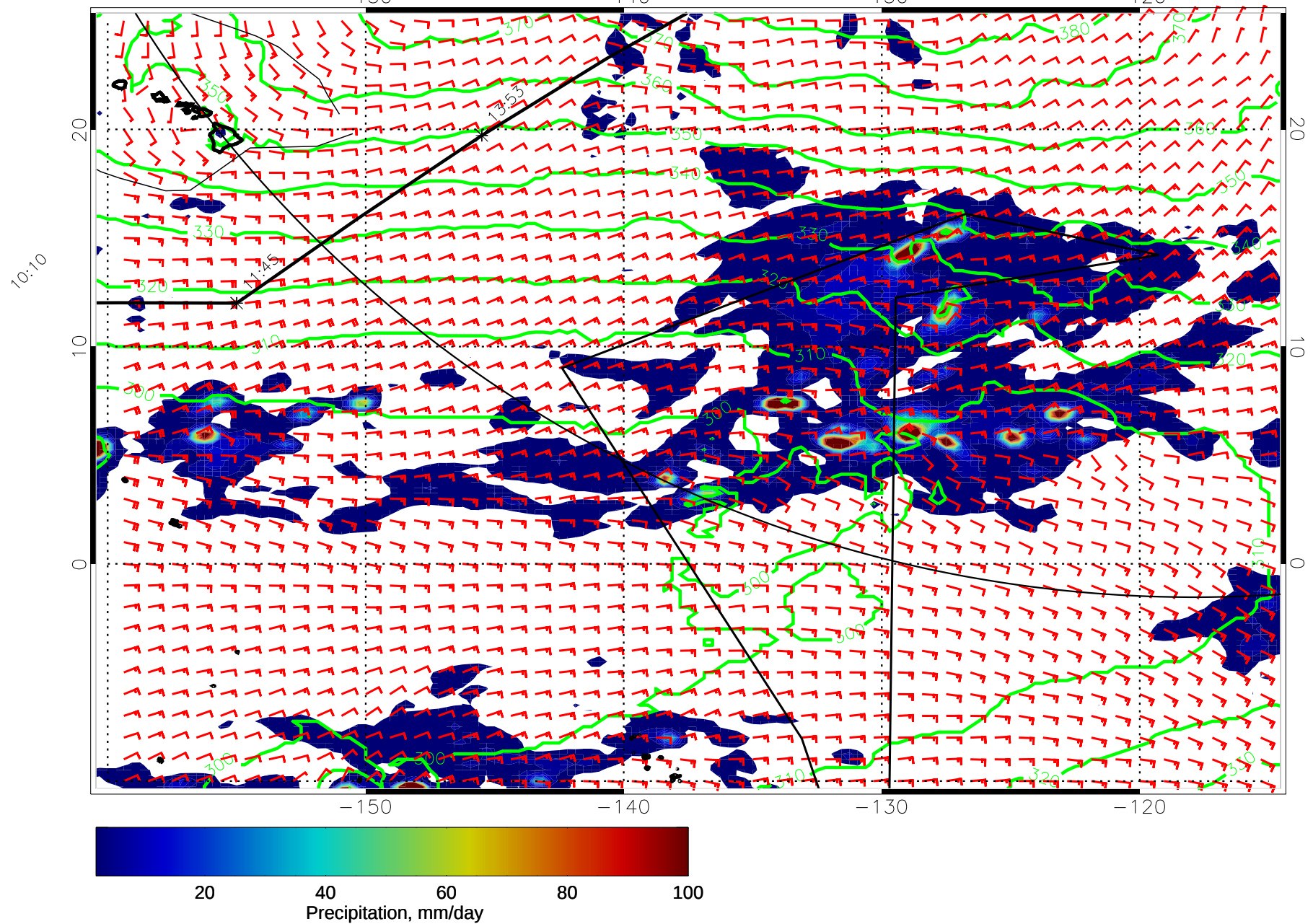
15021900, 48 hour forecast for 975mb Z, Precip., and Surface Winds (knots) -- NASA GEOS5
