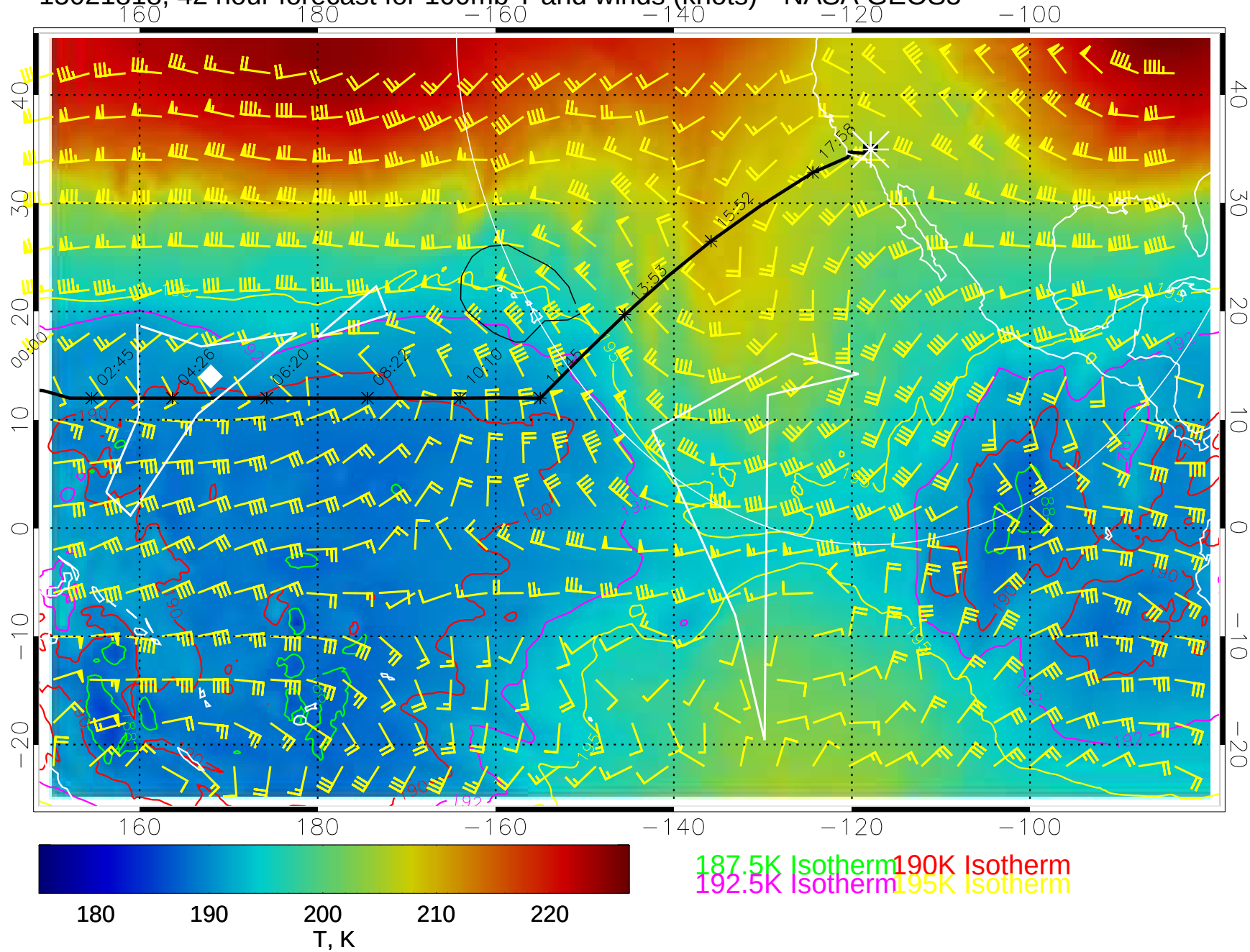
15021818, 42 hour forecast for 100mb T and winds (knots)-- NASA GEOS5
