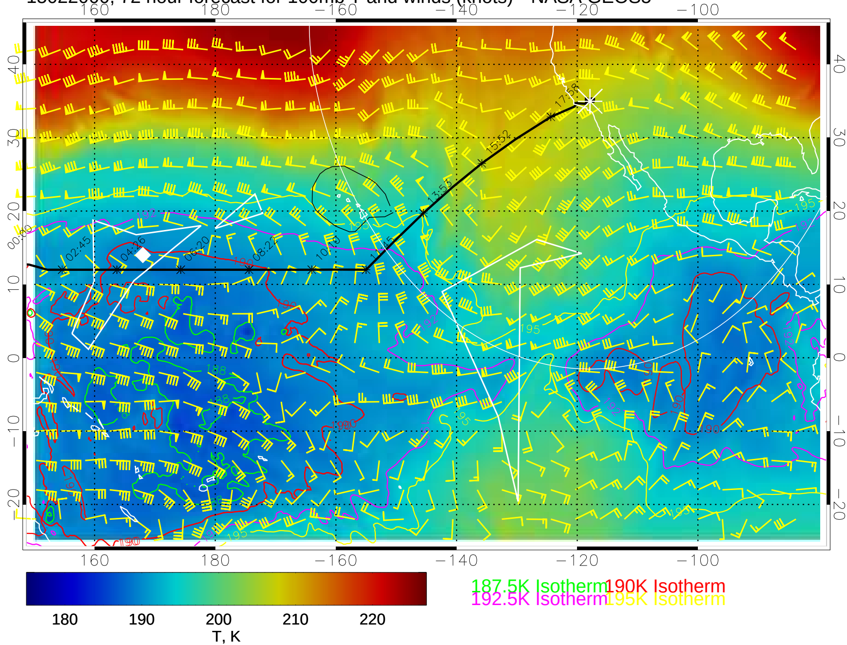
15022000, 72 hour forecast for 100mb T and winds (knots)-- NASA GEOS5
