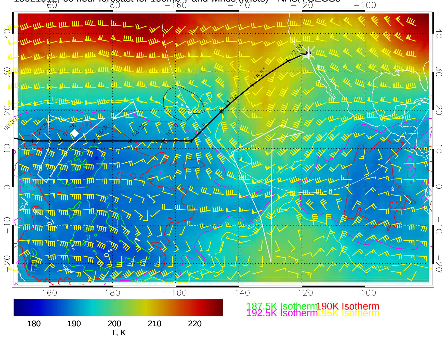
15021912, 60 hour forecast for 100mb T and winds (knots)-- NASA GEOS5
