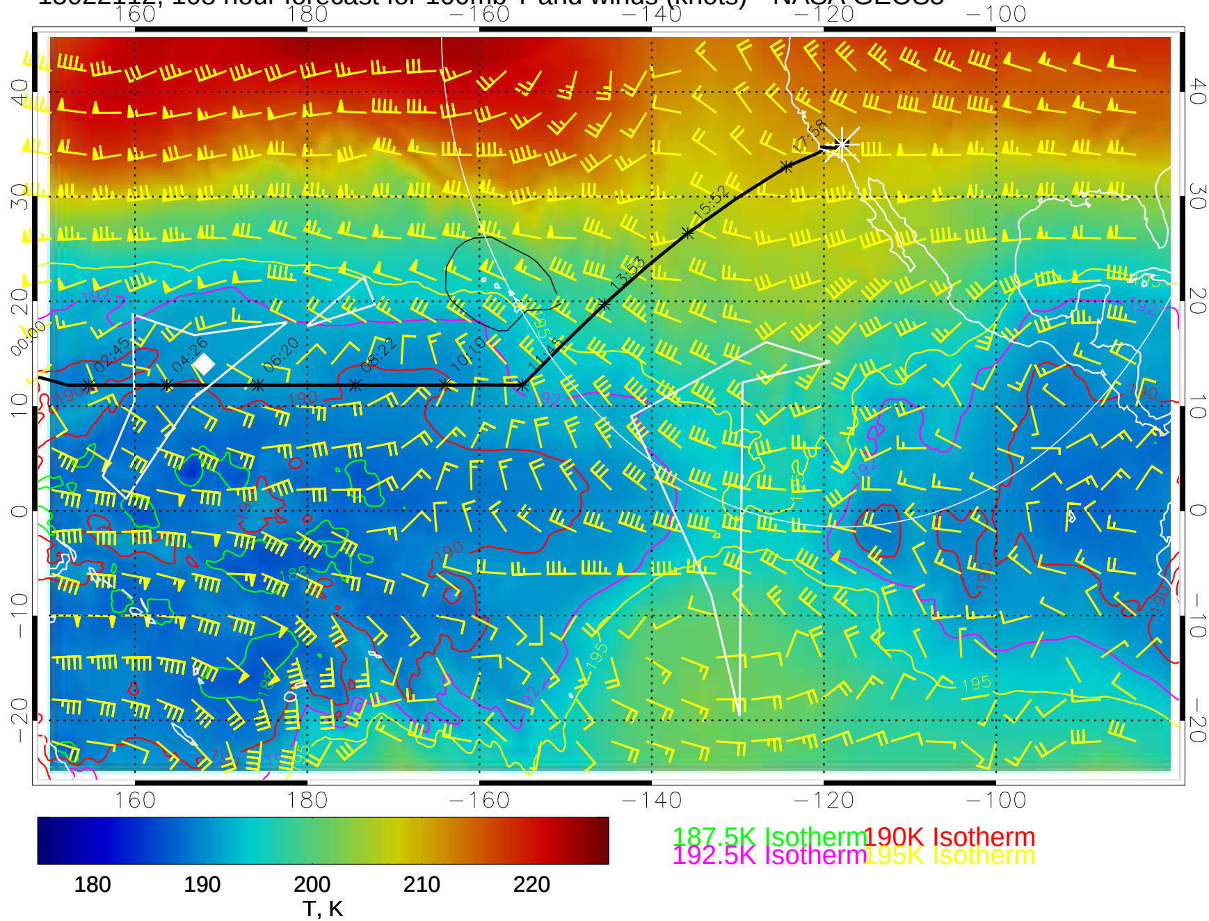
15022112, 108 hour forecast for 100mb T and winds (knots)-- NASA GEOS5
