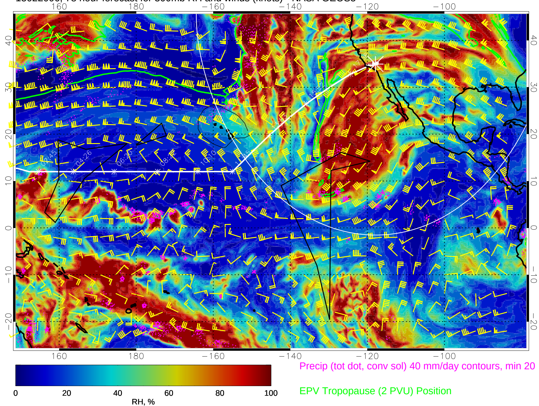
15022006, 78 hour forecast for 300mb RH and winds (knots) - NASA GEOS5
