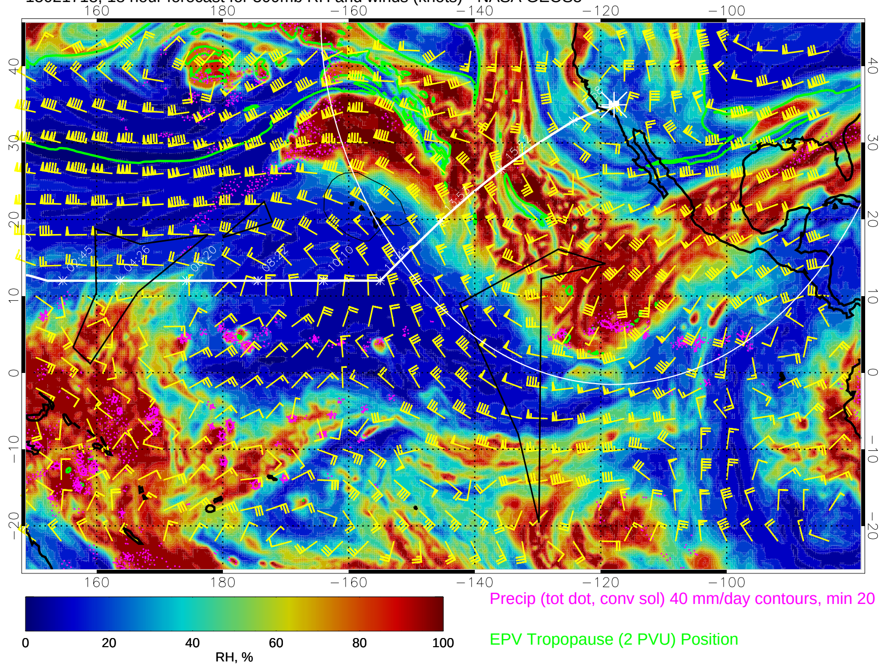
15021718, 18 hour forecast for 300mb RH and winds (knots) - NASA GEOS5
