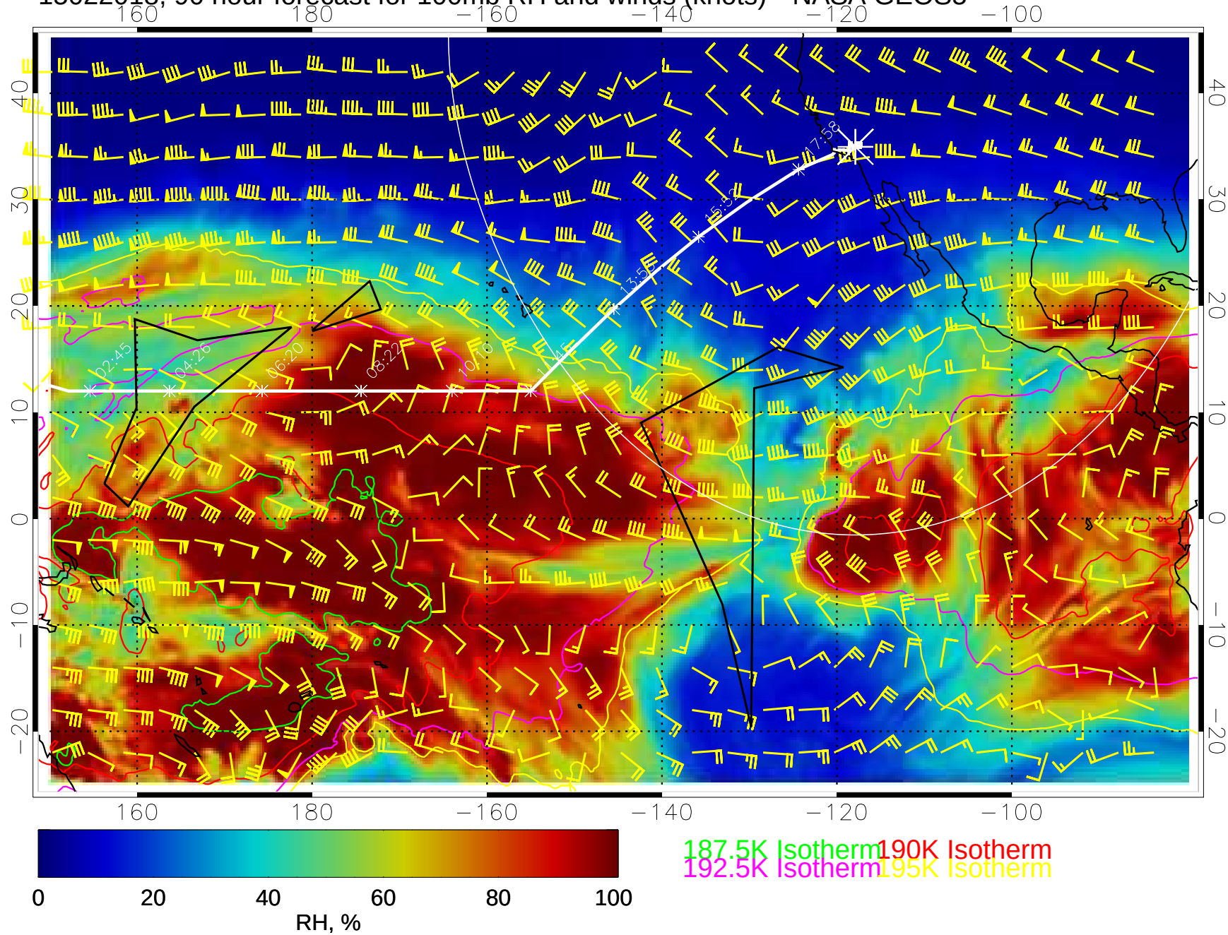
15022018, 90 hour forecast for 100mb RH and winds (knots)-- NASA GEOS5
