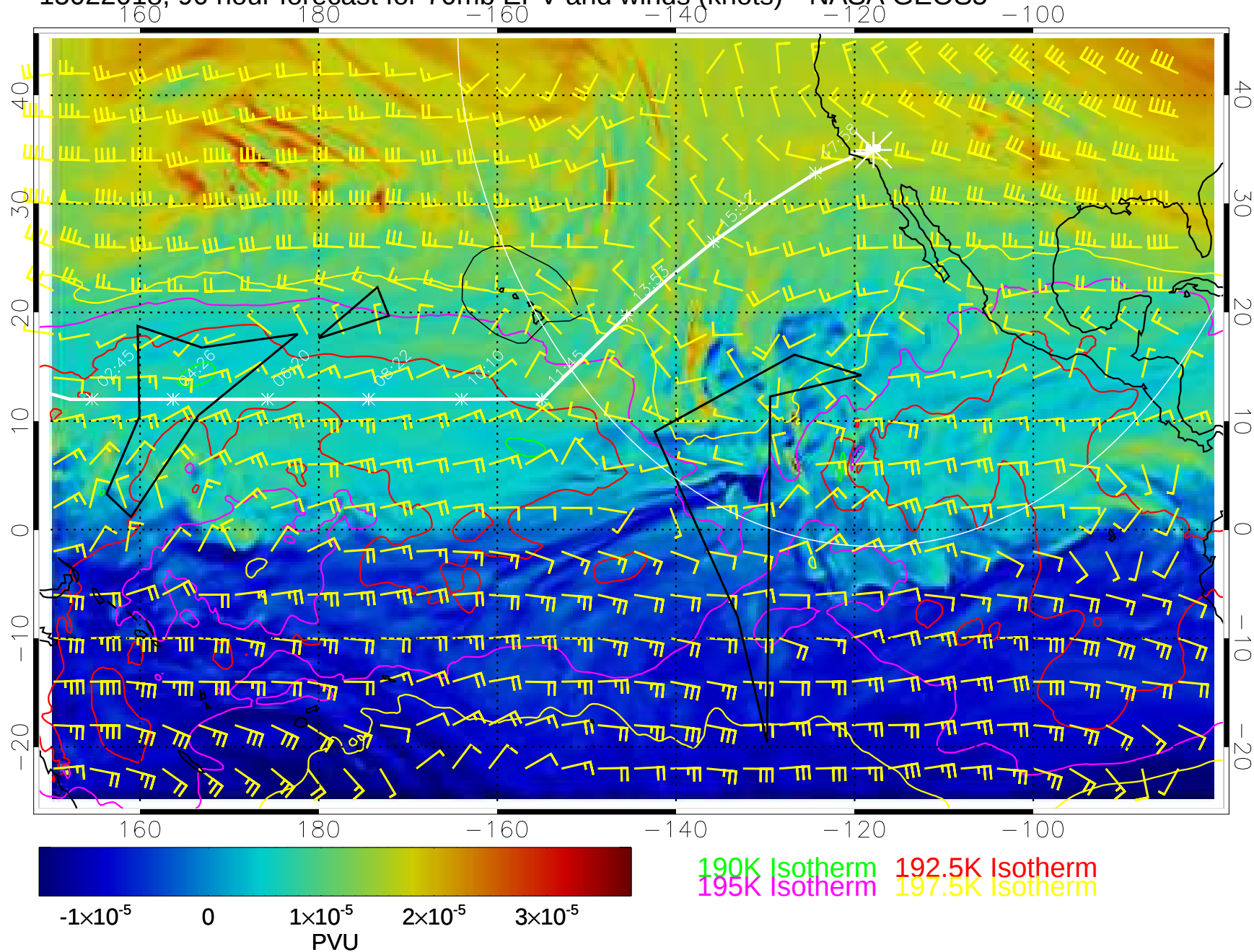
15022018, 90 hour forecast for 70mb EPV and winds (knots)-- NASA GEOS5
