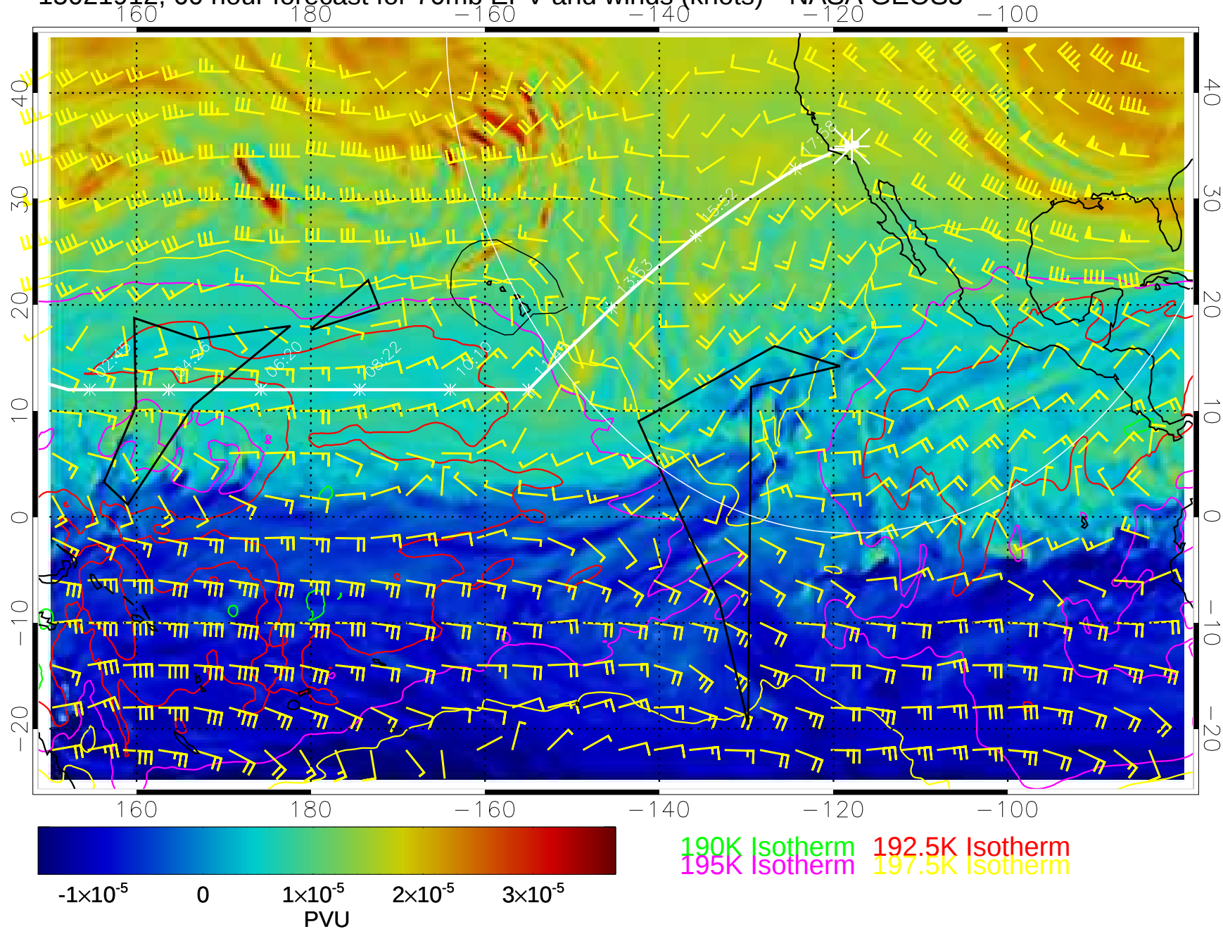
15021912, 60 hour forecast for 70mb EPV and winds (knots)-- NASA GEOS5
