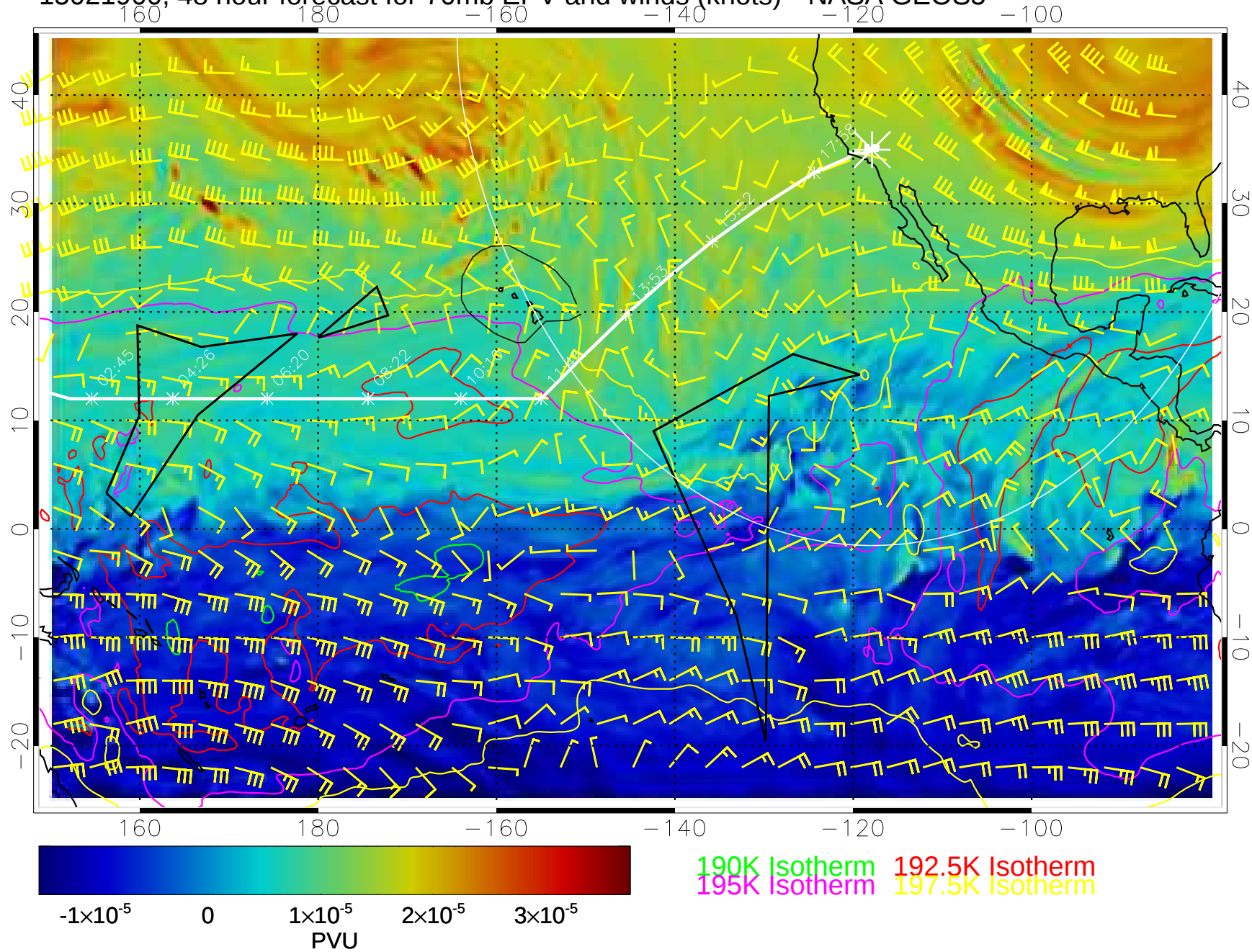
15021900, 48 hour forecast for 70mb EPV and winds (knots)-- NASA GEOS5
