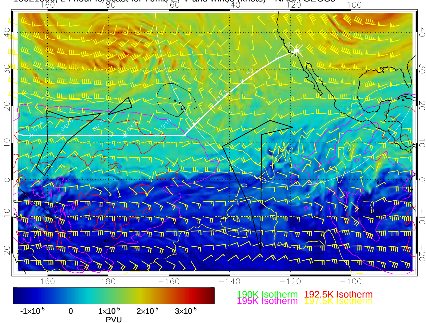
15021800, 24 hour forecast for 70mb EPV and winds (knots)-- NASA GEOS5
