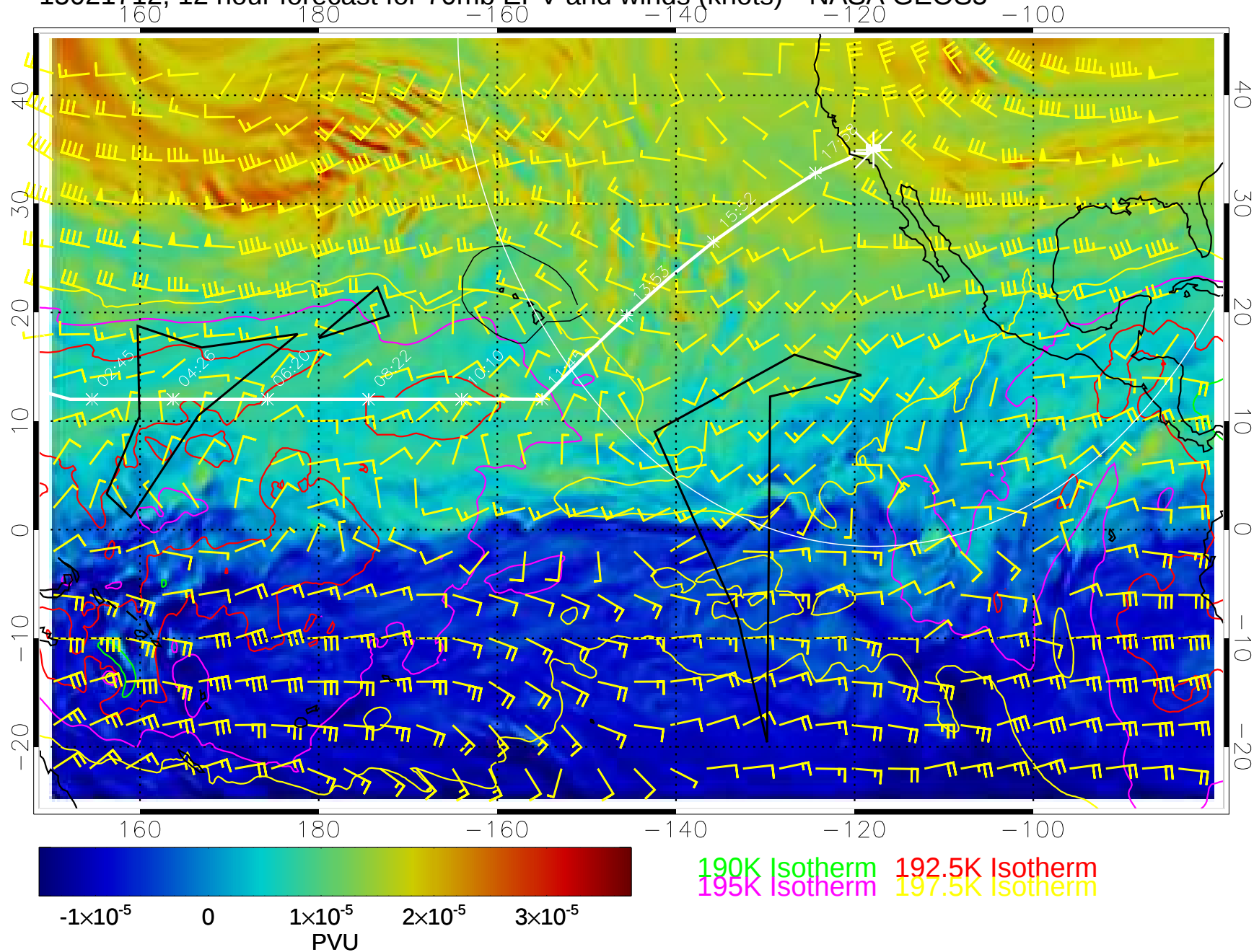
15021712, 12 hour forecast for 70mb EPV and winds (knots)-- NASA GEOS5
