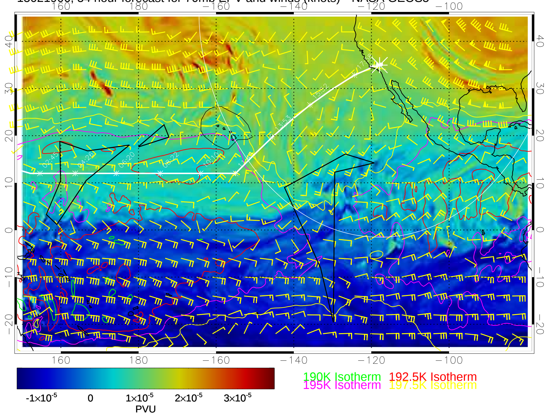
15021906, 54 hour forecast for 70mb EPV and winds (knots)-- NASA GEOS5
