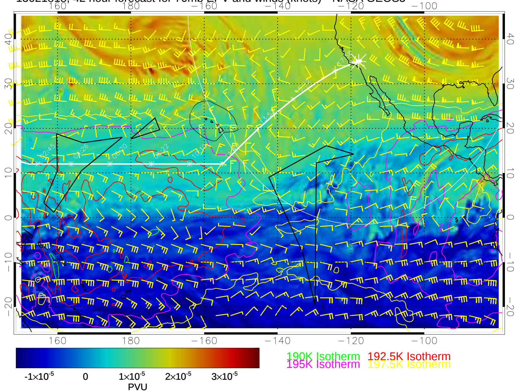
15021818, 42 hour forecast for 70mb EPV and winds (knots)-- NASA GEOS5
