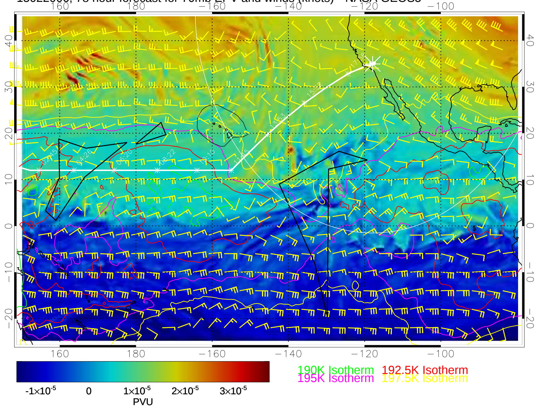
15022006, 78 hour forecast for 70mb EPV and winds (knots)-- NASA GEOS5
