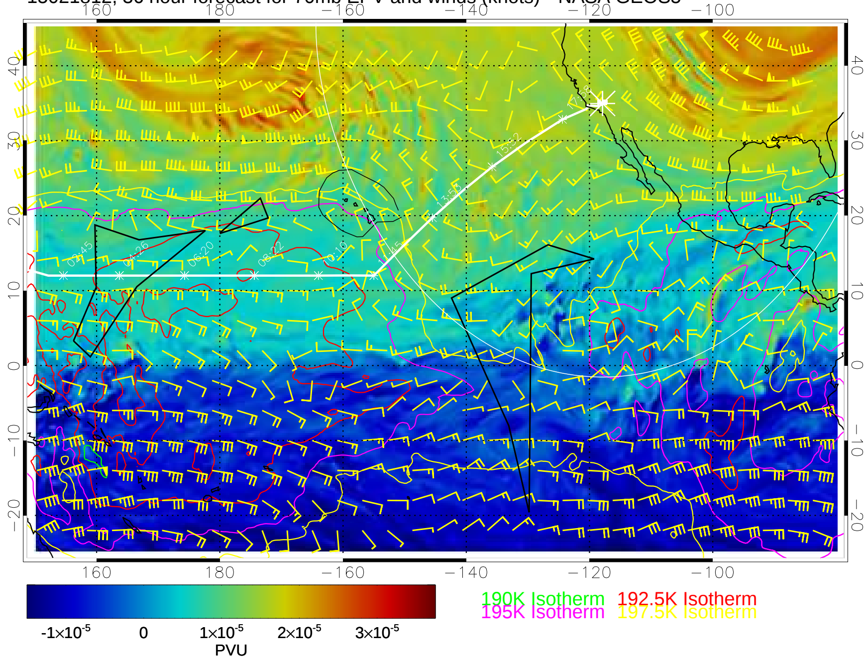
15021812, 36 hour forecast for 70mb EPV and winds (knots)-- NASA GEOS5
