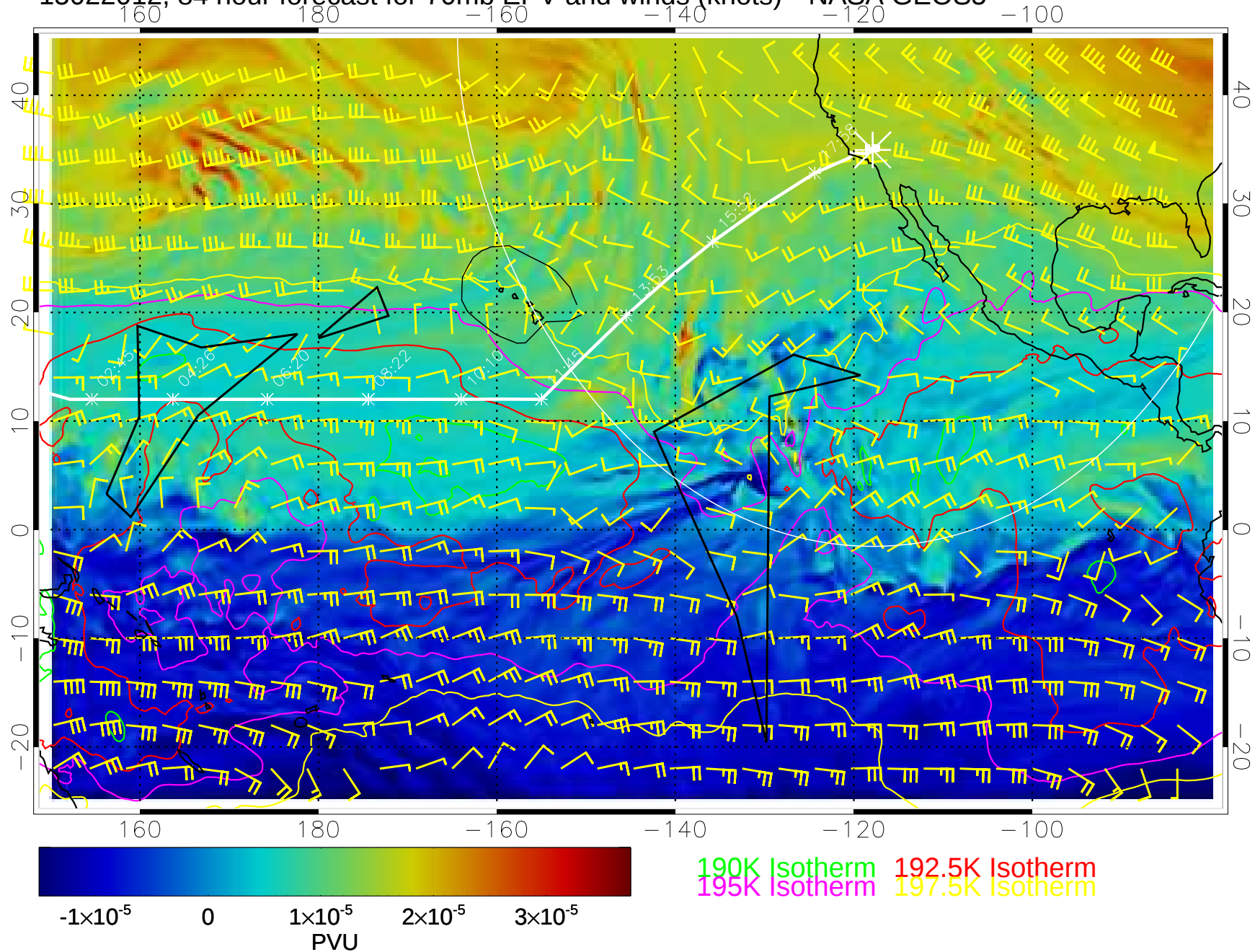
15022012, 84 hour forecast for 70mb EPV and winds (knots)-- NASA GEOS5
