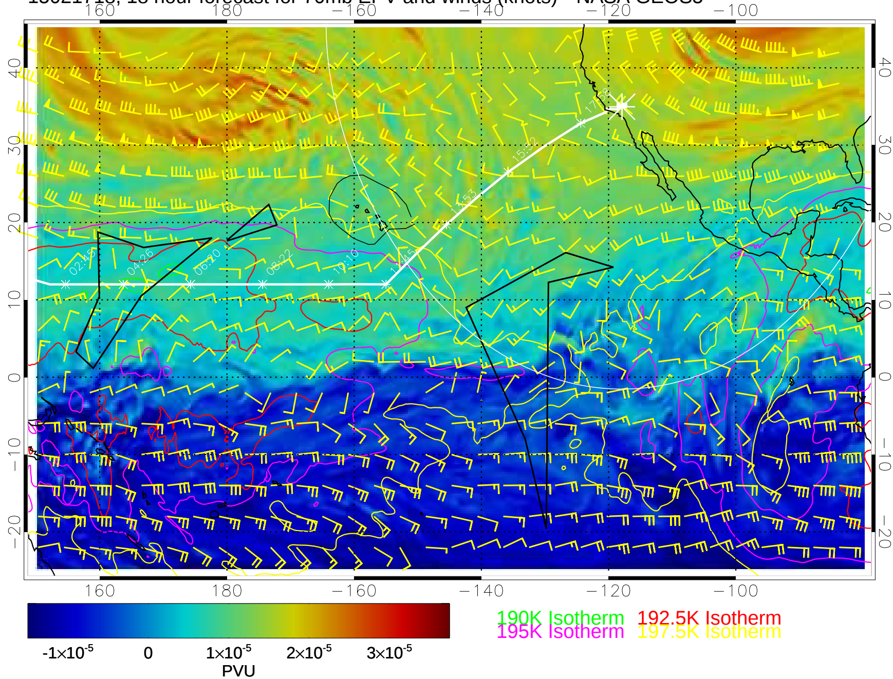
15021718, 18 hour forecast for 70mb EPV and winds (knots)-- NASA GEOS5
