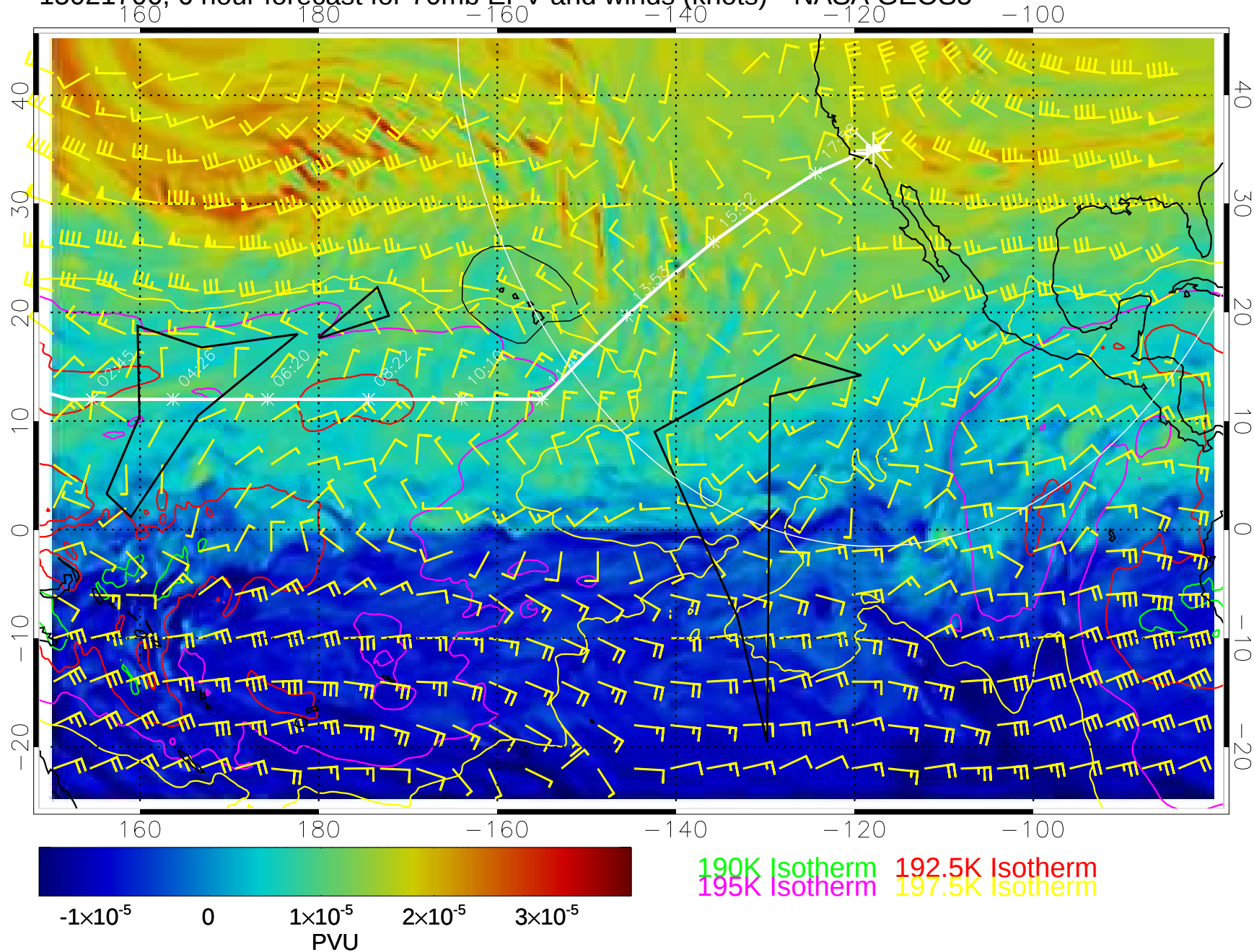
15021706, 6 hour forecast for 70mb EPV and winds (knots)-- NASA GEOS5
