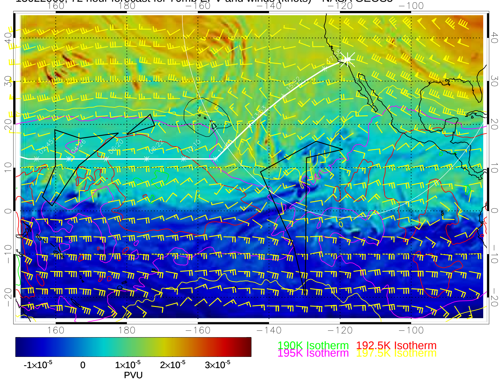
15022000, 72 hour forecast for 70mb EPV and winds (knots)-- NASA GEOS5
