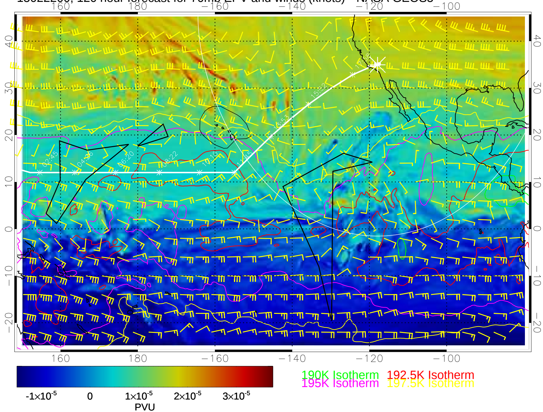
15022200, 120 hour forecast for 70mb EPV and winds (knots)-- NASA GEOS5
