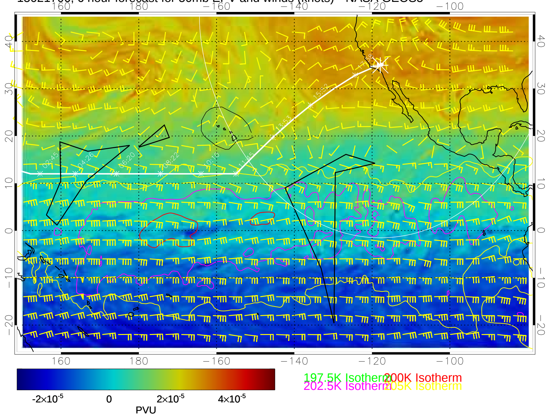
15021706, 6 hour forecast for 50mb EPV and winds (knots)-- NASA GEOS5
