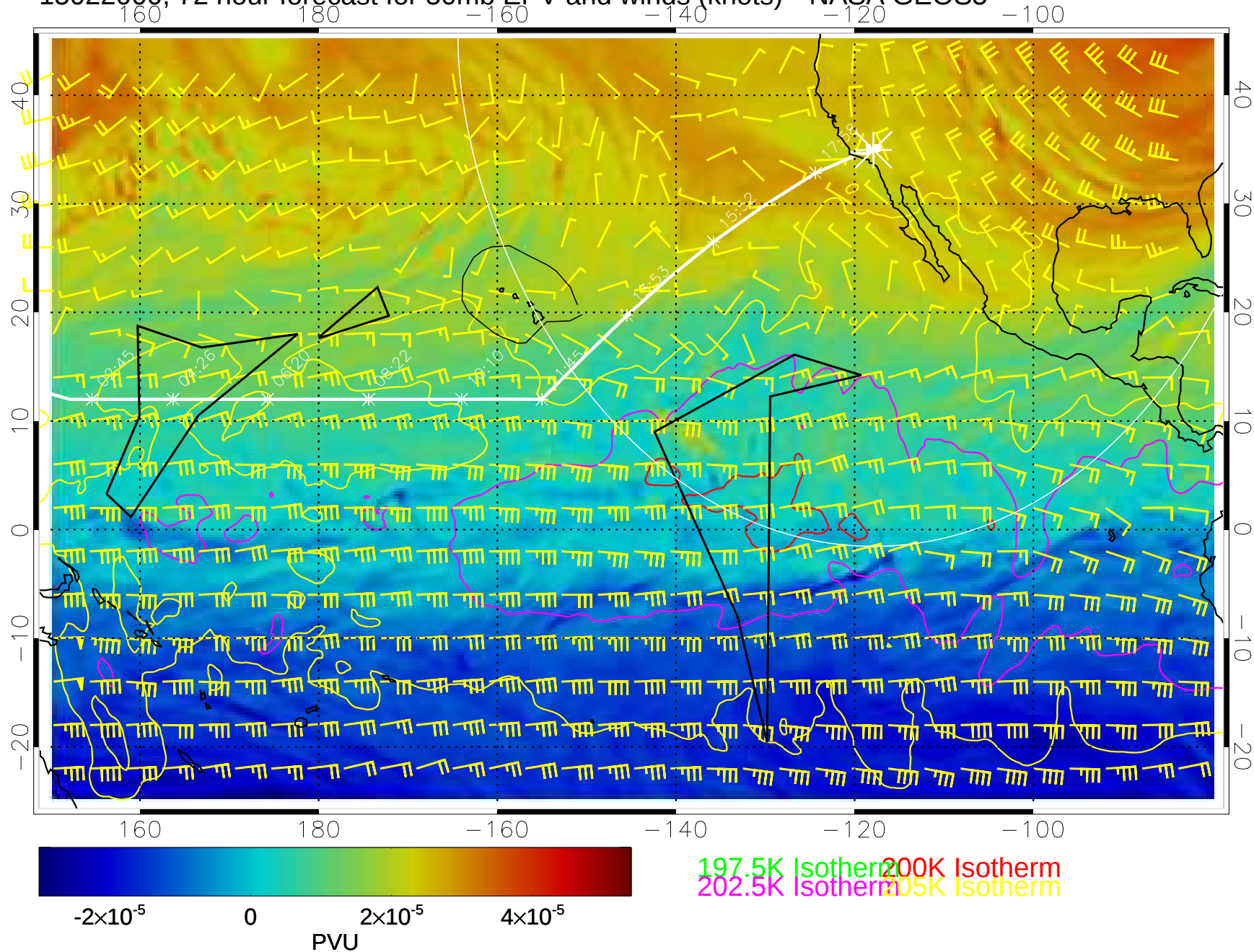
15022000, 72 hour forecast for 50mb EPV and winds (knots)-- NASA GEOS5
