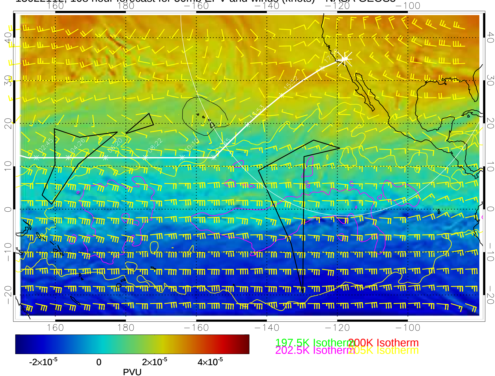
15022112, 108 hour forecast for 50mb EPV and winds (knots)-- NASA GEOS5
