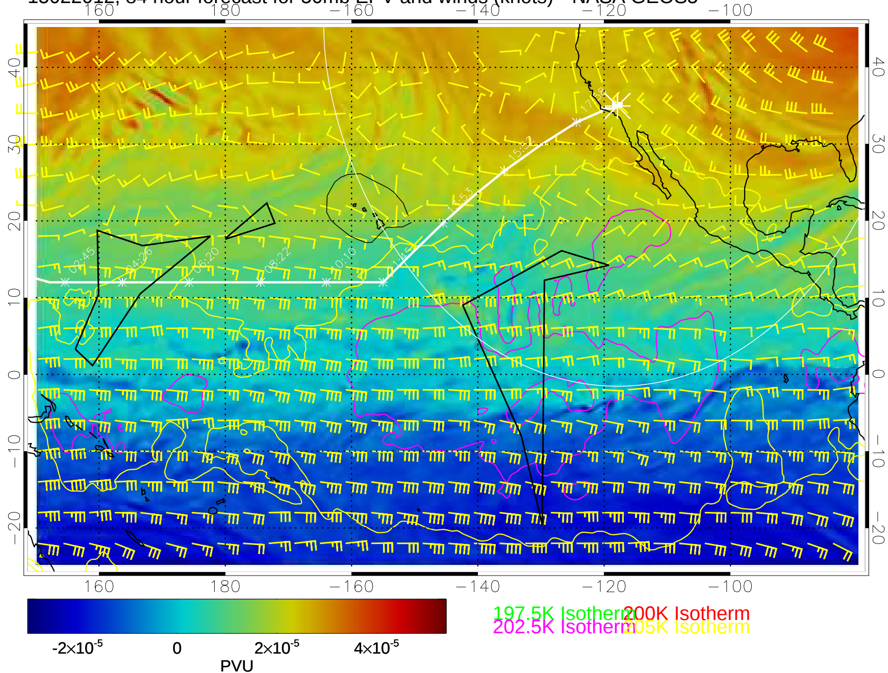
15022012, 84 hour forecast for 50mb EPV and winds (knots)-- NASA GEOS5
