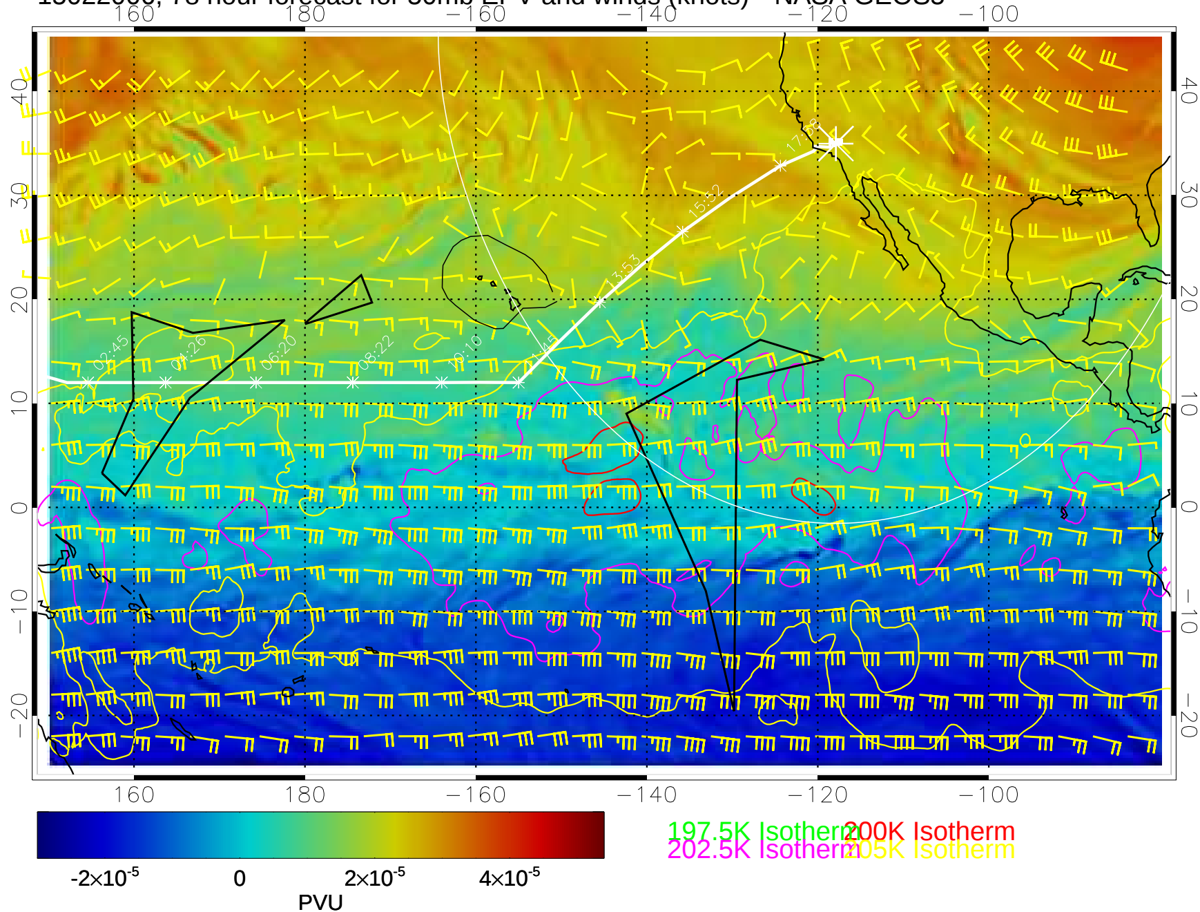
15022006, 78 hour forecast for 50mb EPV and winds (knots)-- NASA GEOS5
