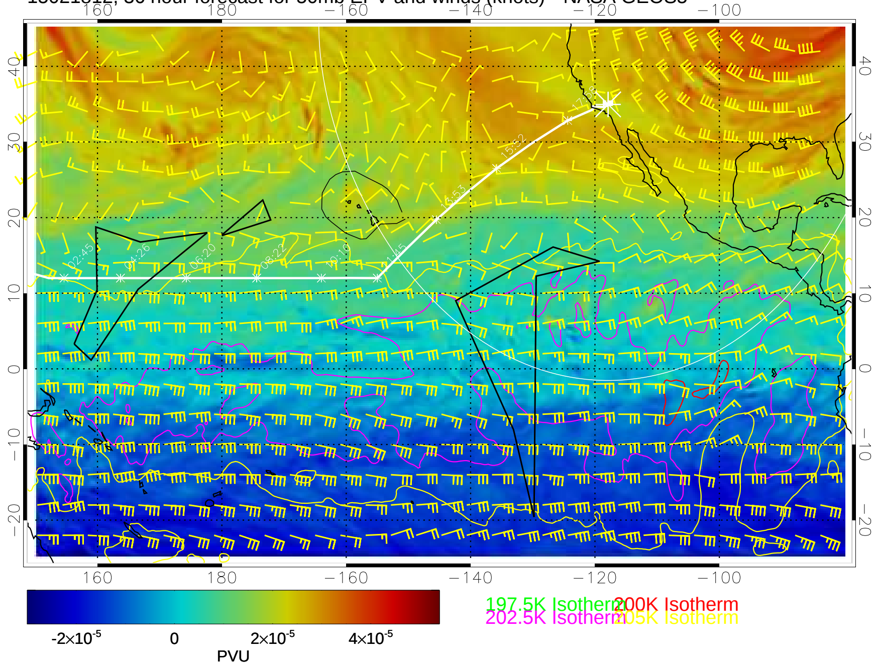
15021812, 36 hour forecast for 50mb EPV and winds (knots)-- NASA GEOS5
