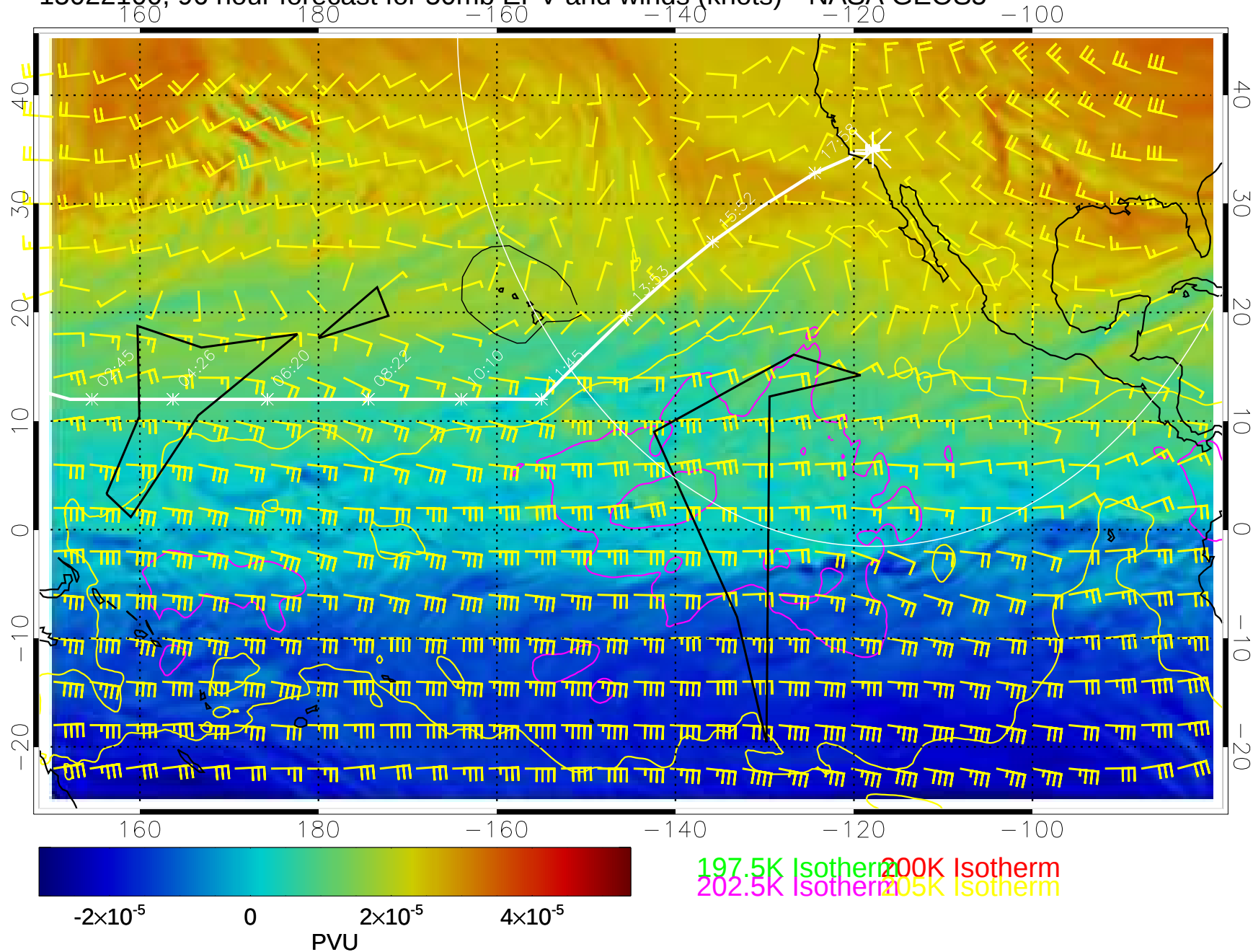
15022100, 96 hour forecast for 50mb EPV and winds (knots)-- NASA GEOS5
