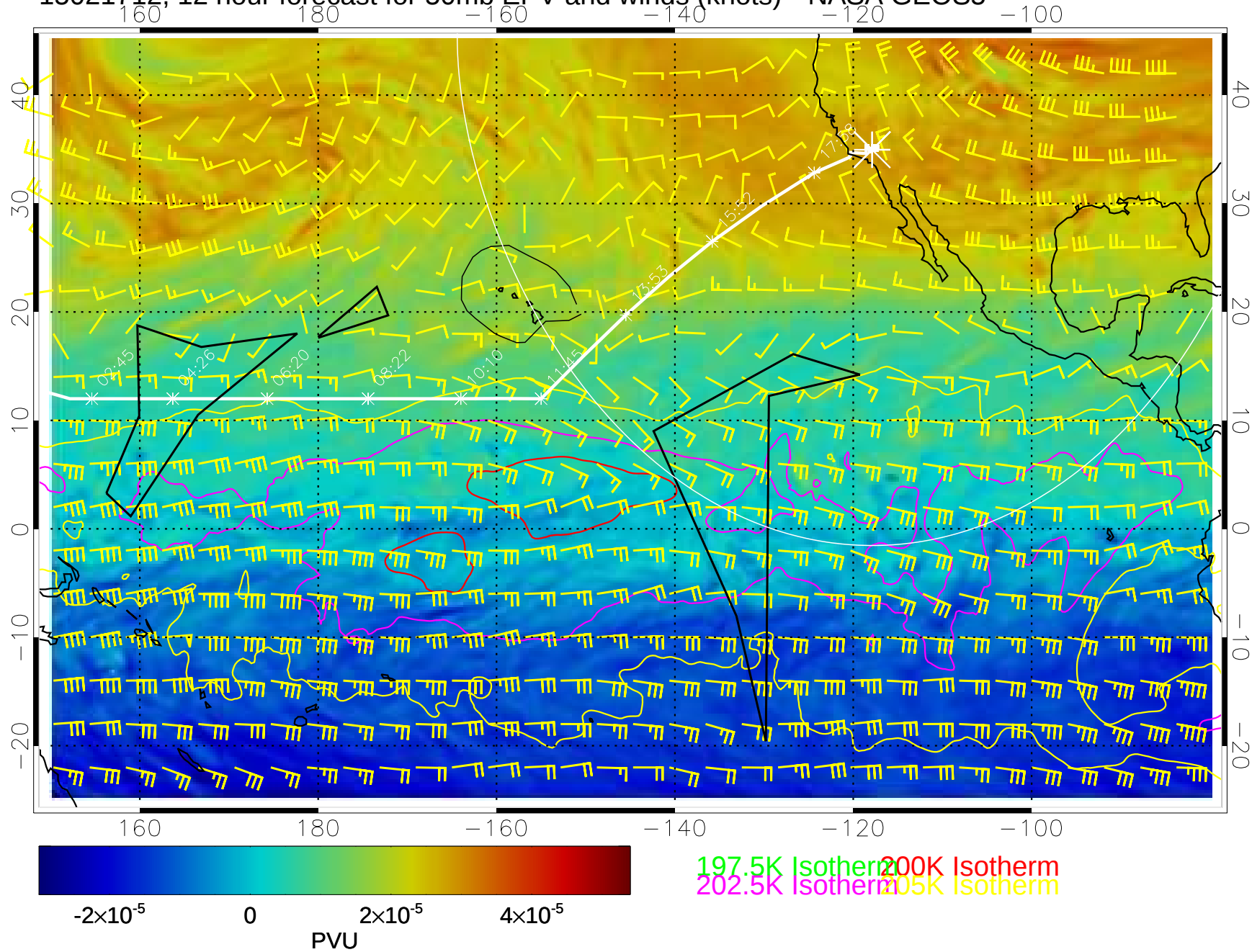
15021712, 12 hour forecast for 50mb EPV and winds (knots)-- NASA GEOS5
