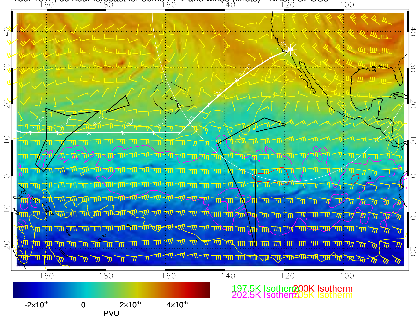
15021912, 60 hour forecast for 50mb EPV and winds (knots)-- NASA GEOS5
