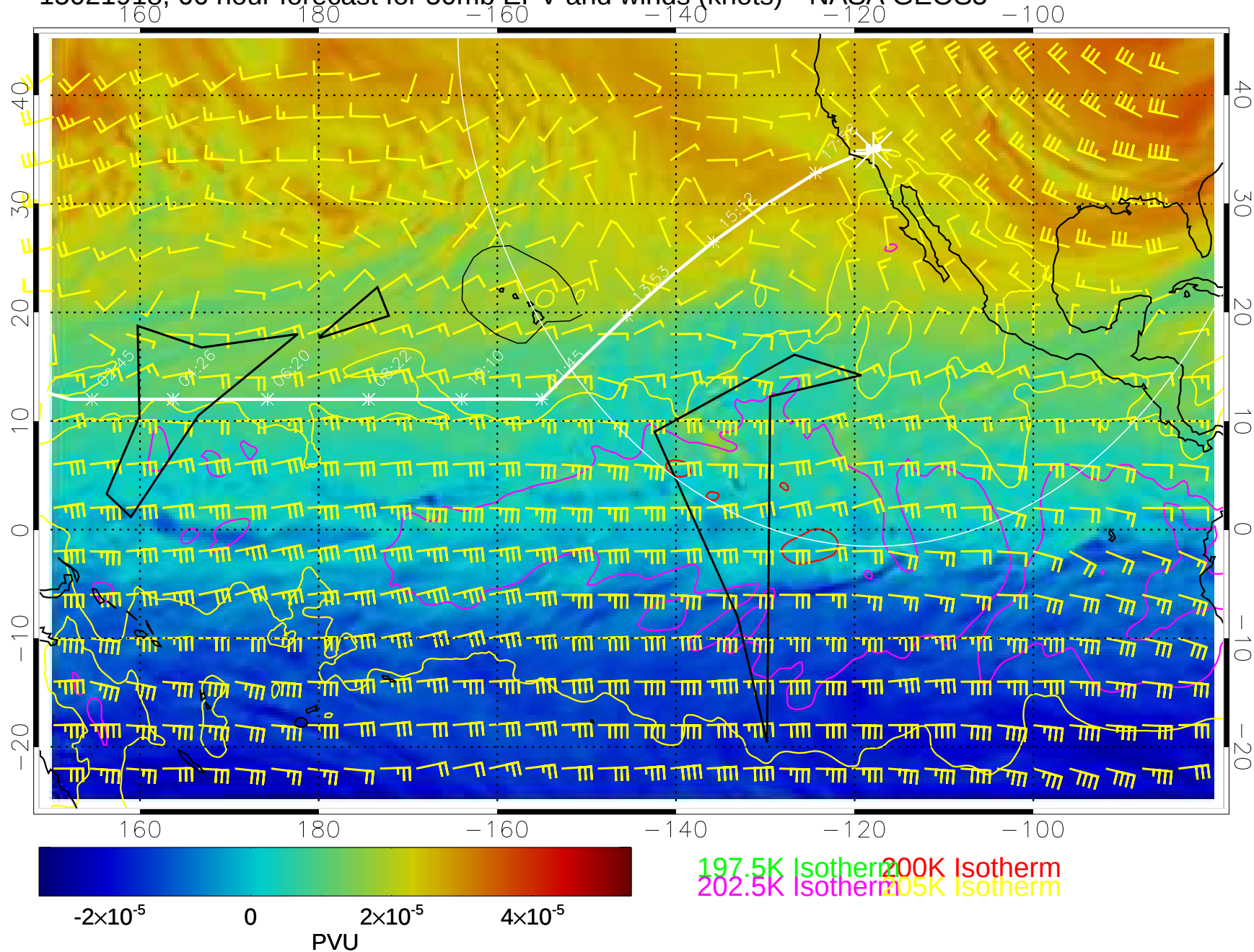
15021918, 66 hour forecast for 50mb EPV and winds (knots)-- NASA GEOS5
