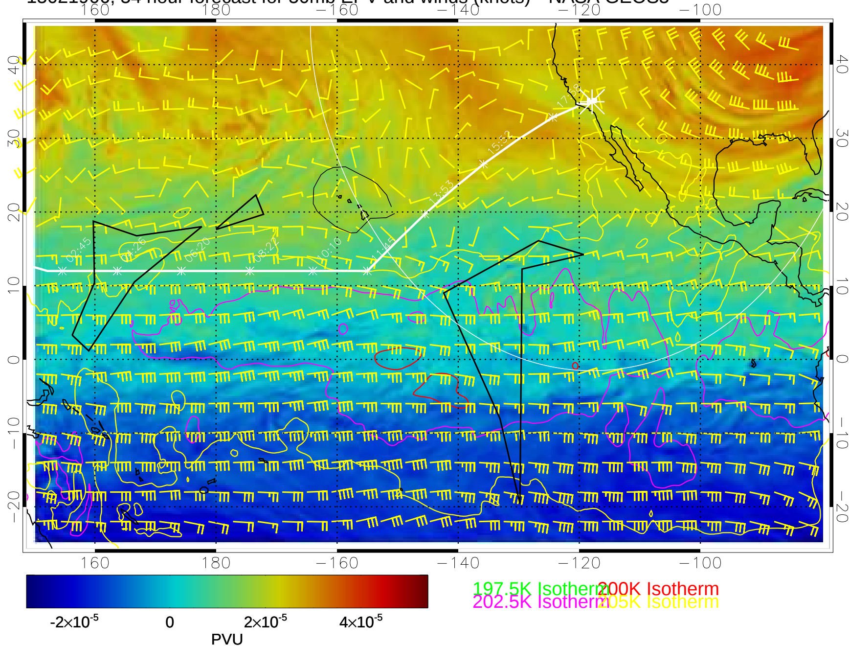
15021906, 54 hour forecast for 50mb EPV and winds (knots)-- NASA GEOS5
