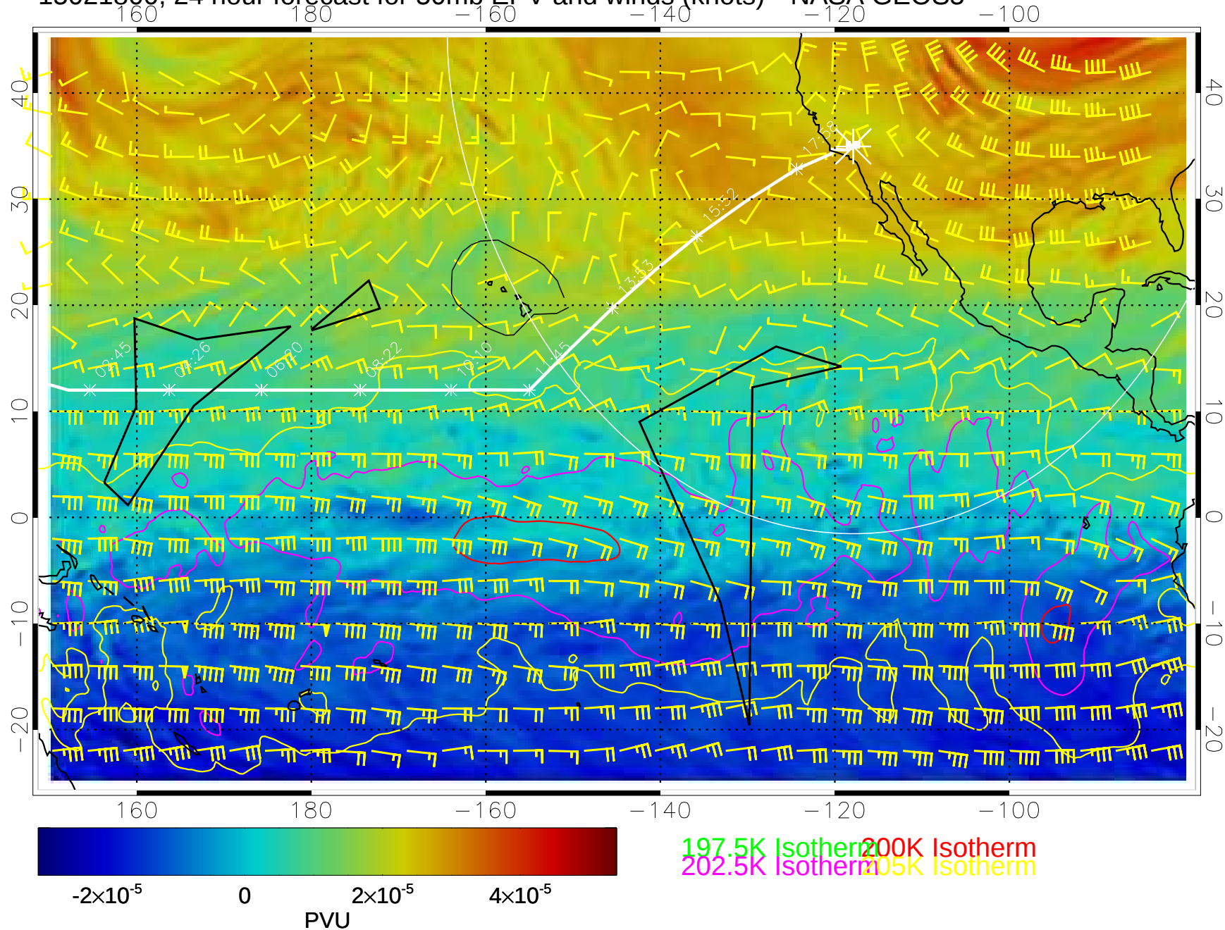
15021800, 24 hour forecast for 50mb EPV and winds (knots)-- NASA GEOS5
