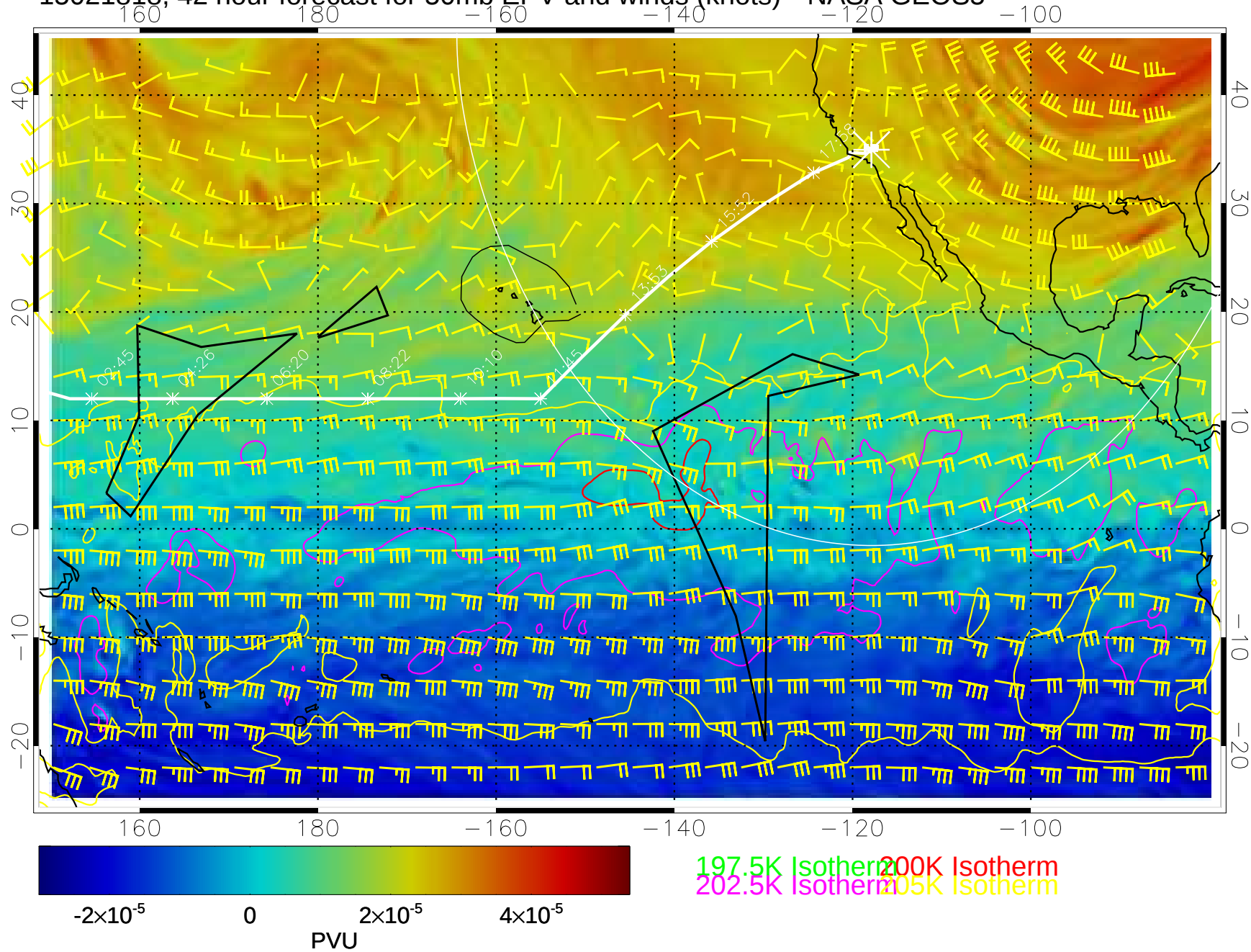
15021818, 42 hour forecast for 50mb EPV and winds (knots)-- NASA GEOS5
