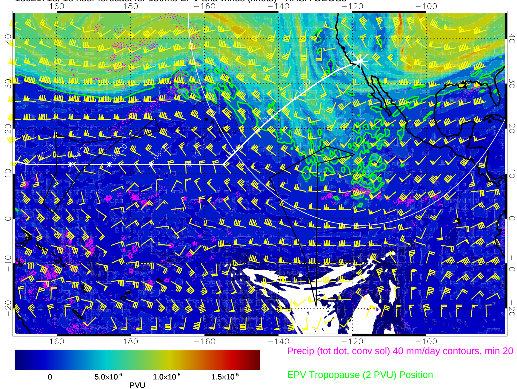
15021718, 18 hour forecast for 150mb EPV and winds (knots) - NASA GEOS5
