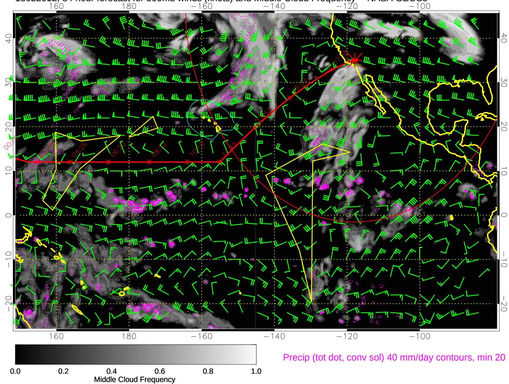
15022012, 84 hour forecast for 500mb winds (knots) and Middle Cloud Frequency -- NASA GEOS5
