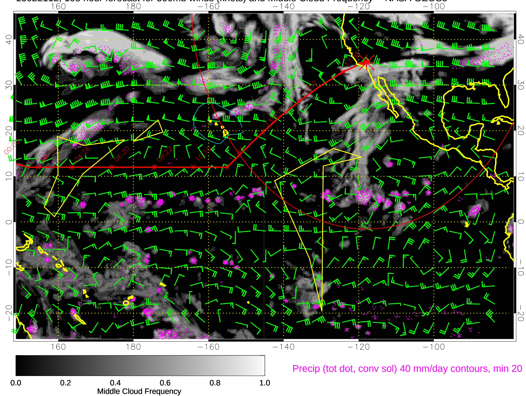
15022112, 108 hour forecast for 500mb winds (knots) and Middle Cloud Frequency -- NASA GEOS5
