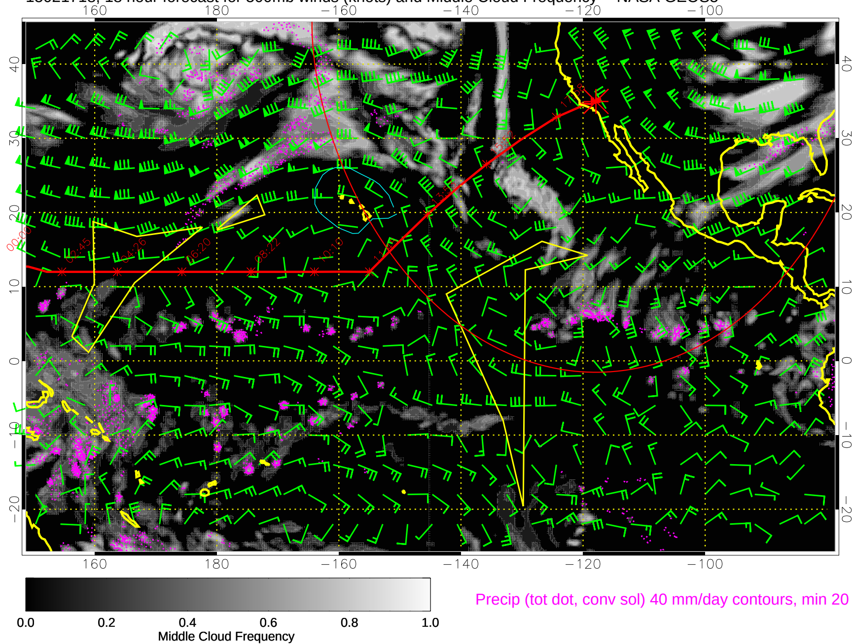
15021718, 18 hour forecast for 500mb winds (knots) and Middle Cloud Frequency -- NASA GEOS5
