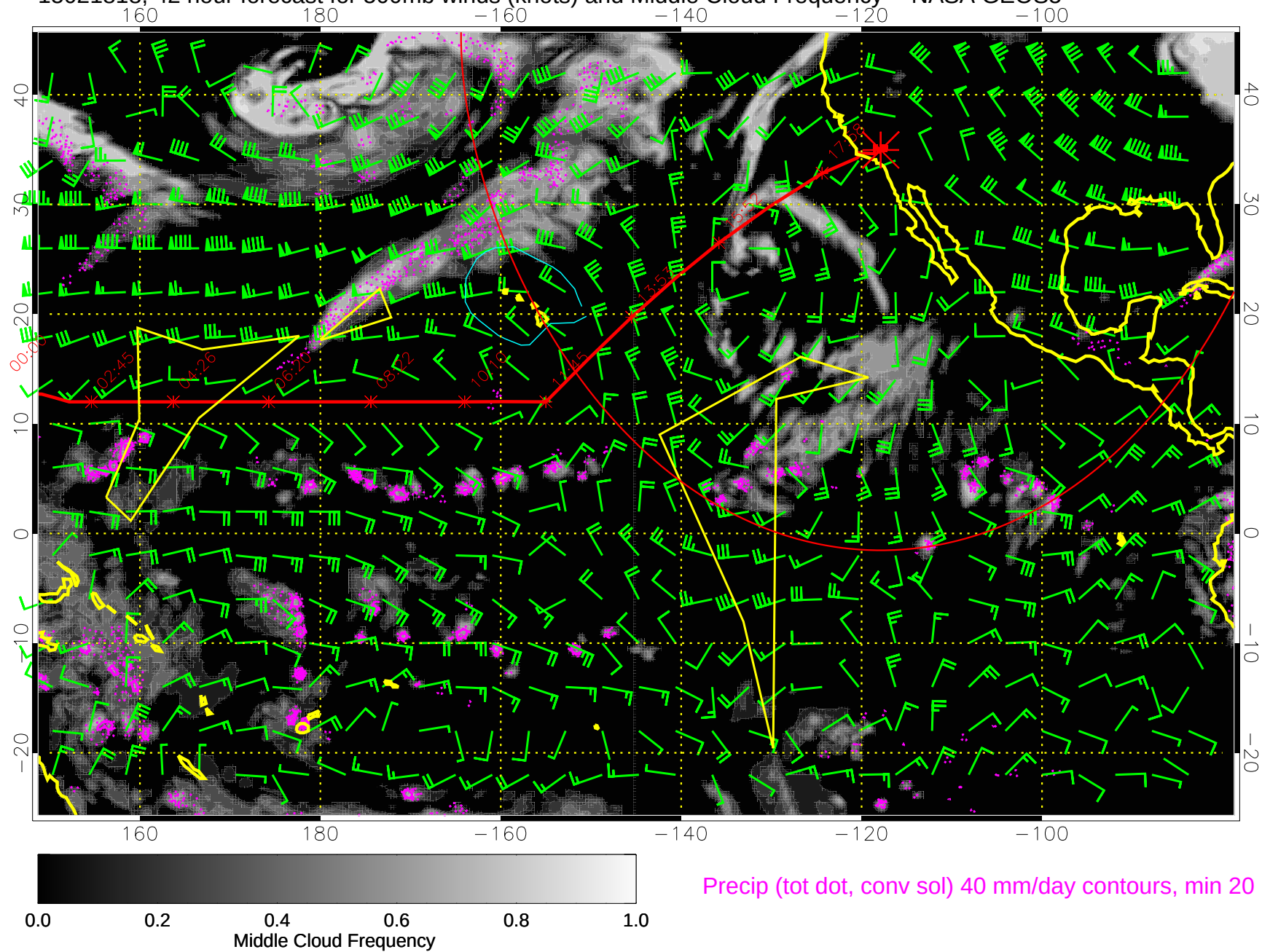
15021818, 42 hour forecast for 500mb winds (knots) and Middle Cloud Frequency -- NASA GEOS5
