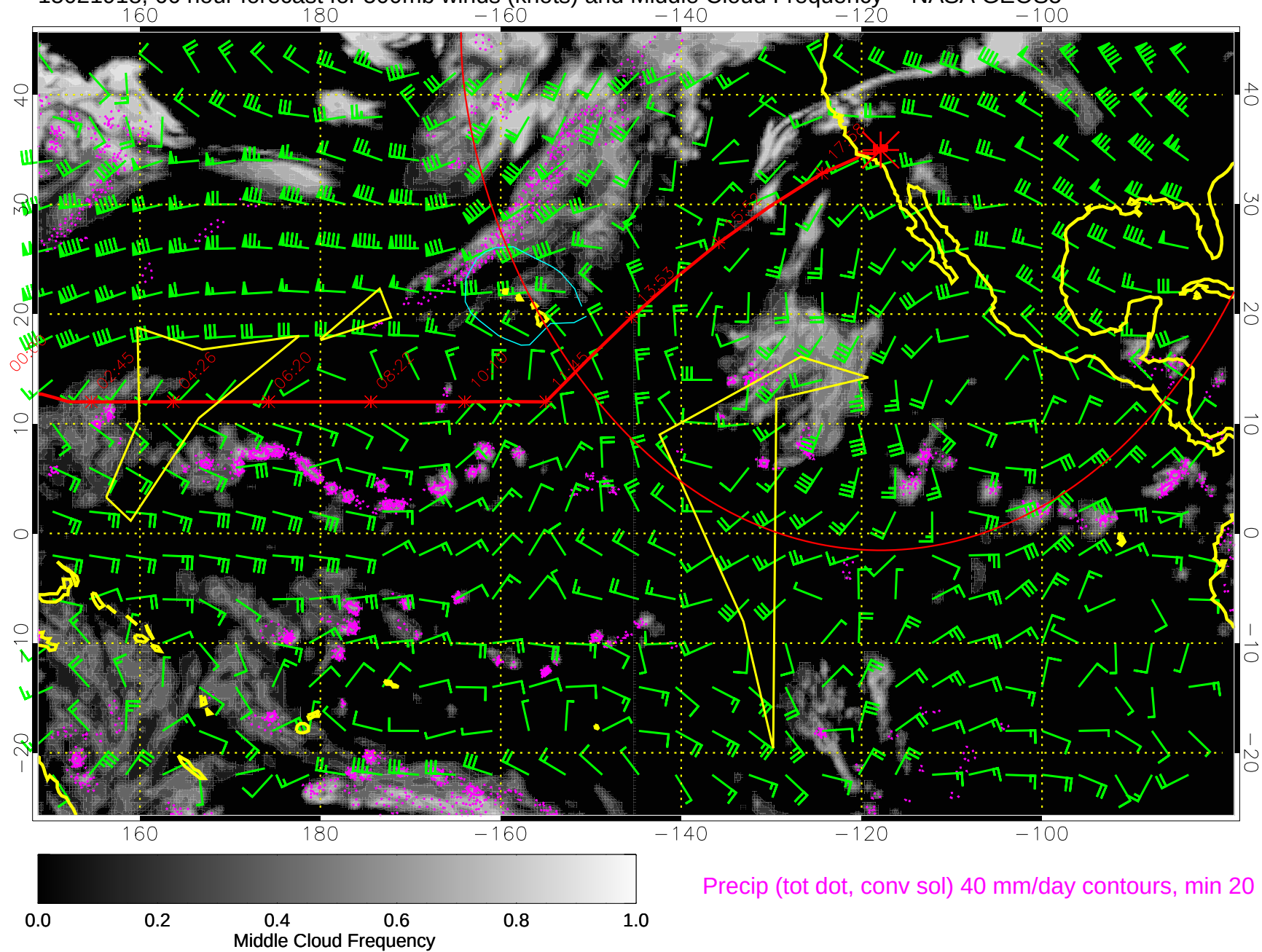
15021918, 66 hour forecast for 500mb winds (knots) and Middle Cloud Frequency -- NASA GEOS5
