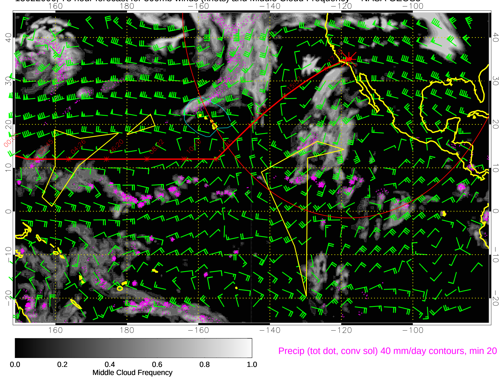
15022006, 78 hour forecast for 500mb winds (knots) and Middle Cloud Frequency -- NASA GEOS5
