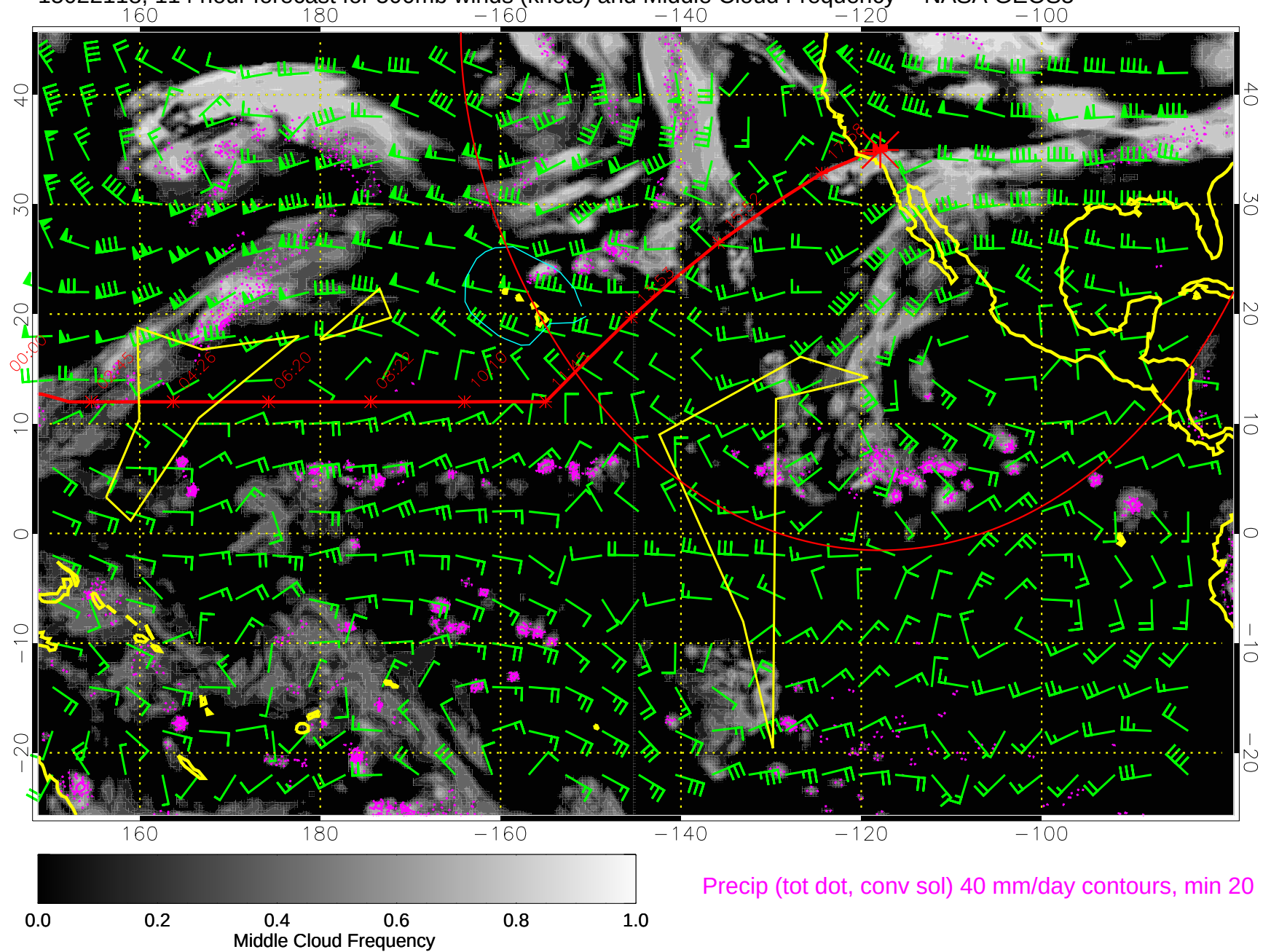
15022118, 114 hour forecast for 500mb winds (knots) and Middle Cloud Frequency -- NASA GEOS5
