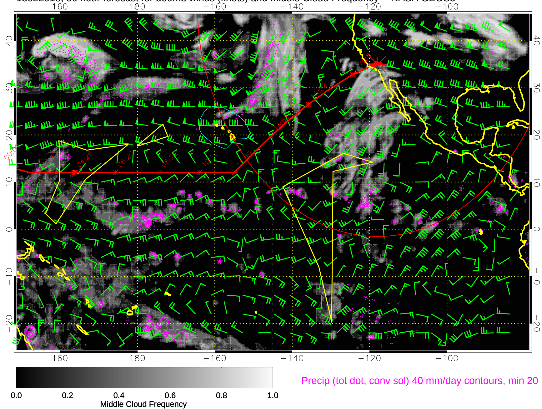
15022018, 90 hour forecast for 500mb winds (knots) and Middle Cloud Frequency -- NASA GEOS5
