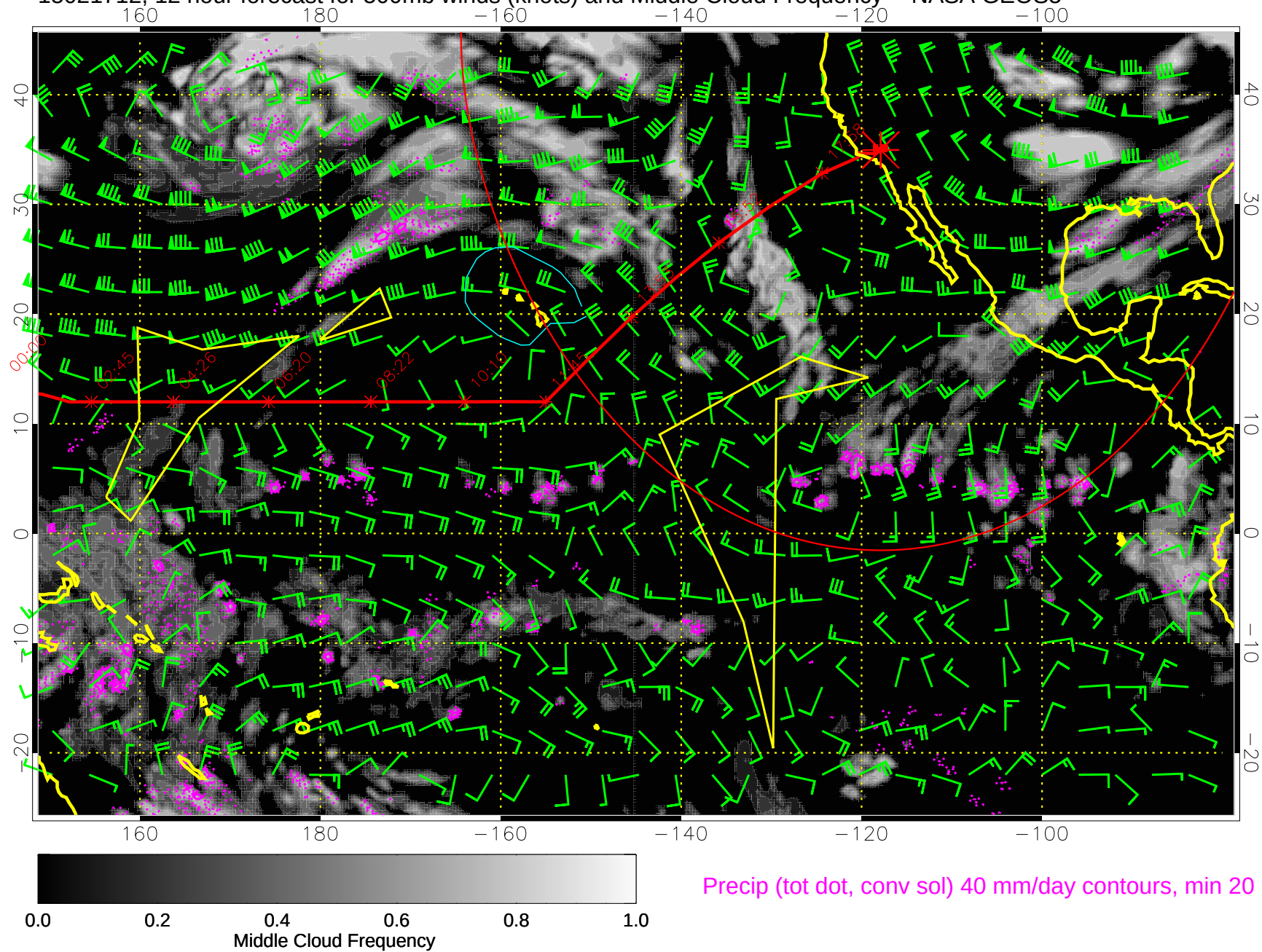
15021712, 12 hour forecast for 500mb winds (knots) and Middle Cloud Frequency -- NASA GEOS5
