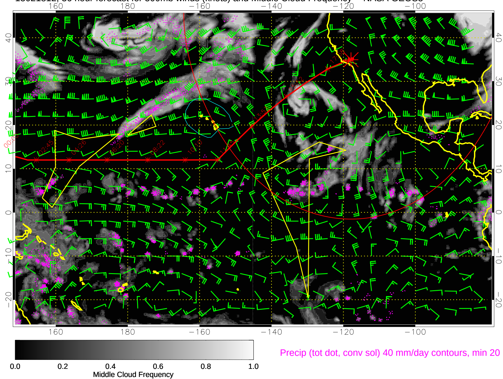
15021812, 36 hour forecast for 500mb winds (knots) and Middle Cloud Frequency -- NASA GEOS5
