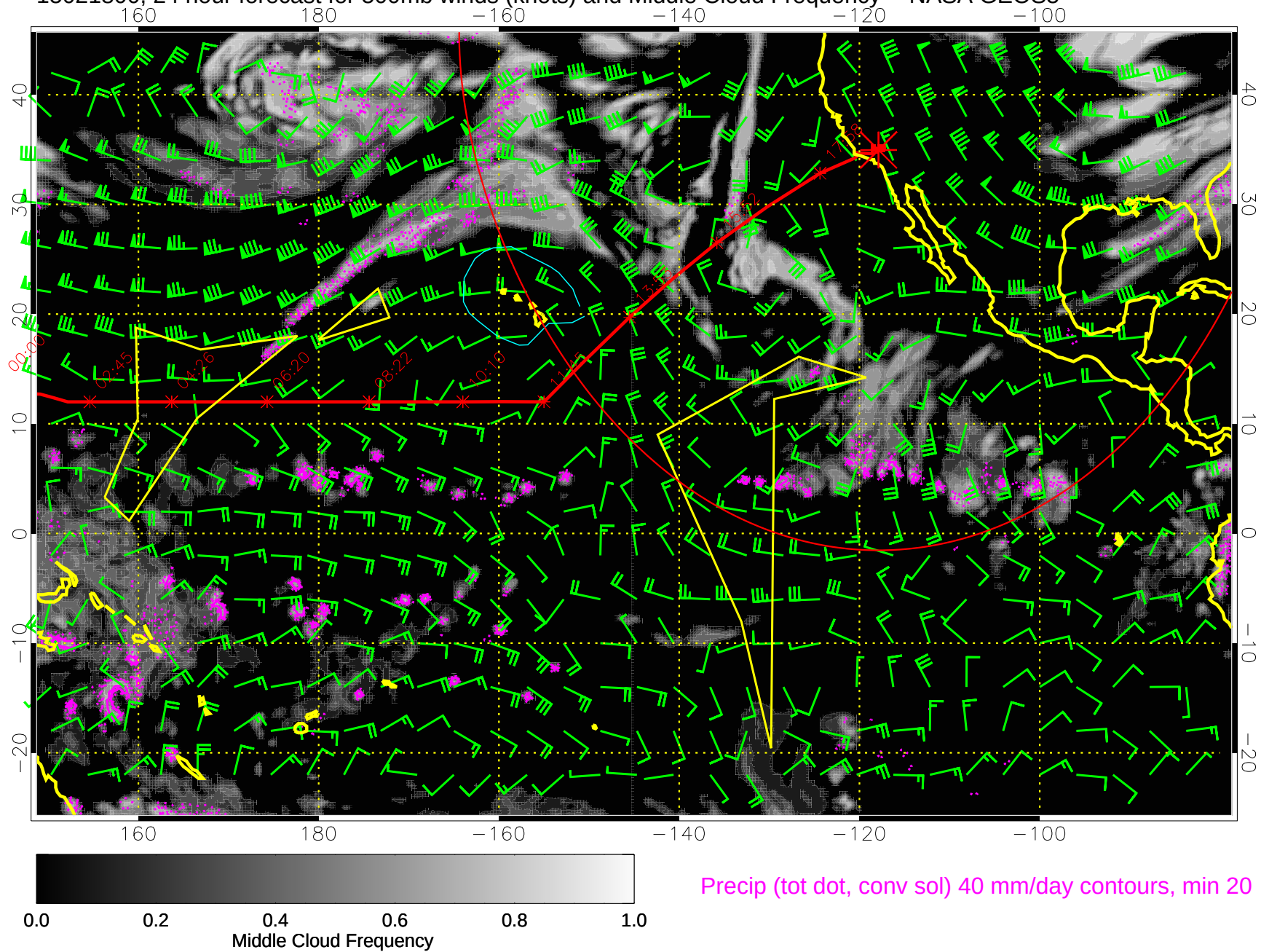
15021800, 24 hour forecast for 500mb winds (knots) and Middle Cloud Frequency -- NASA GEOS5
