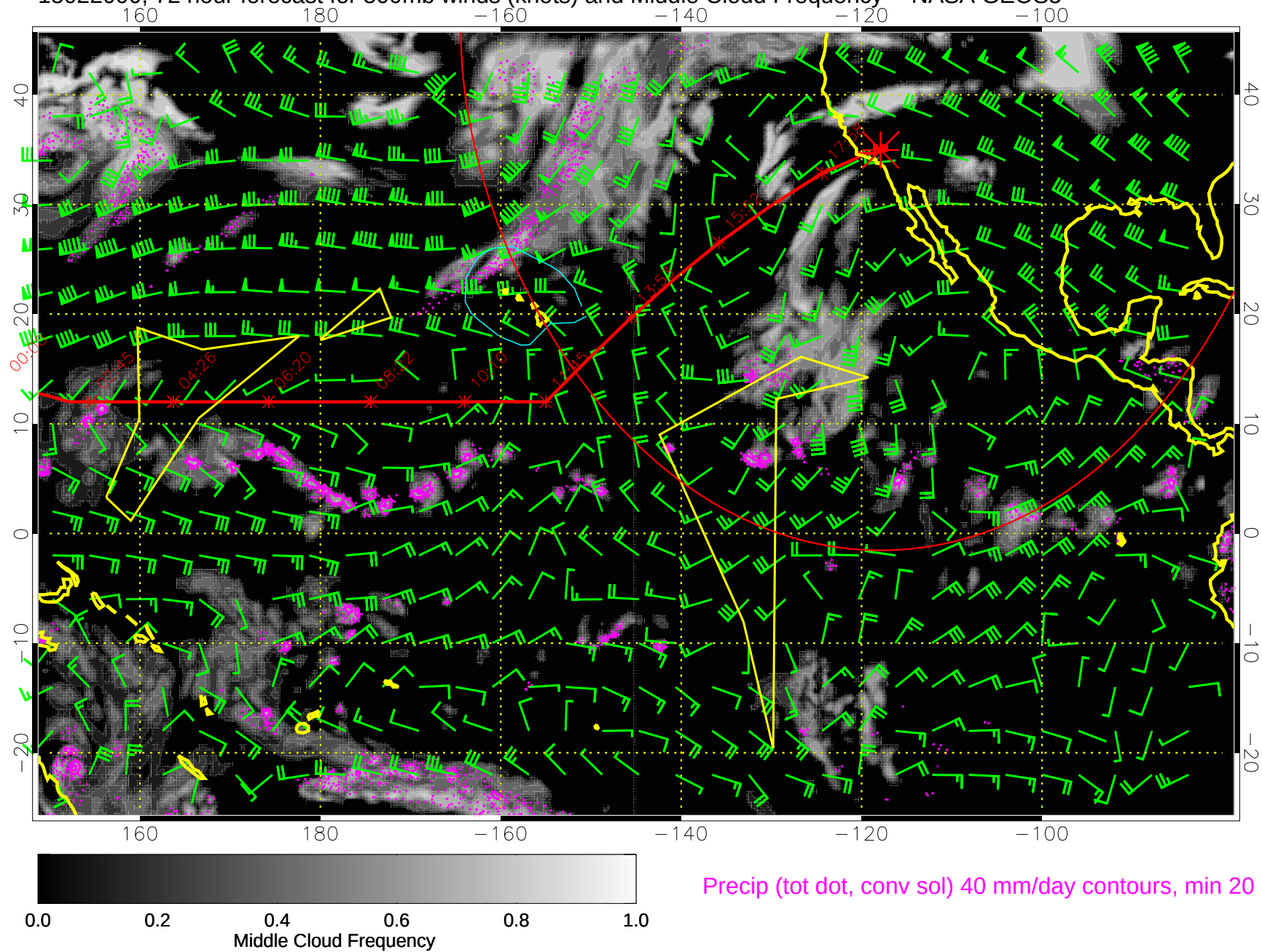
15022000, 72 hour forecast for 500mb winds (knots) and Middle Cloud Frequency -- NASA GEOS5
