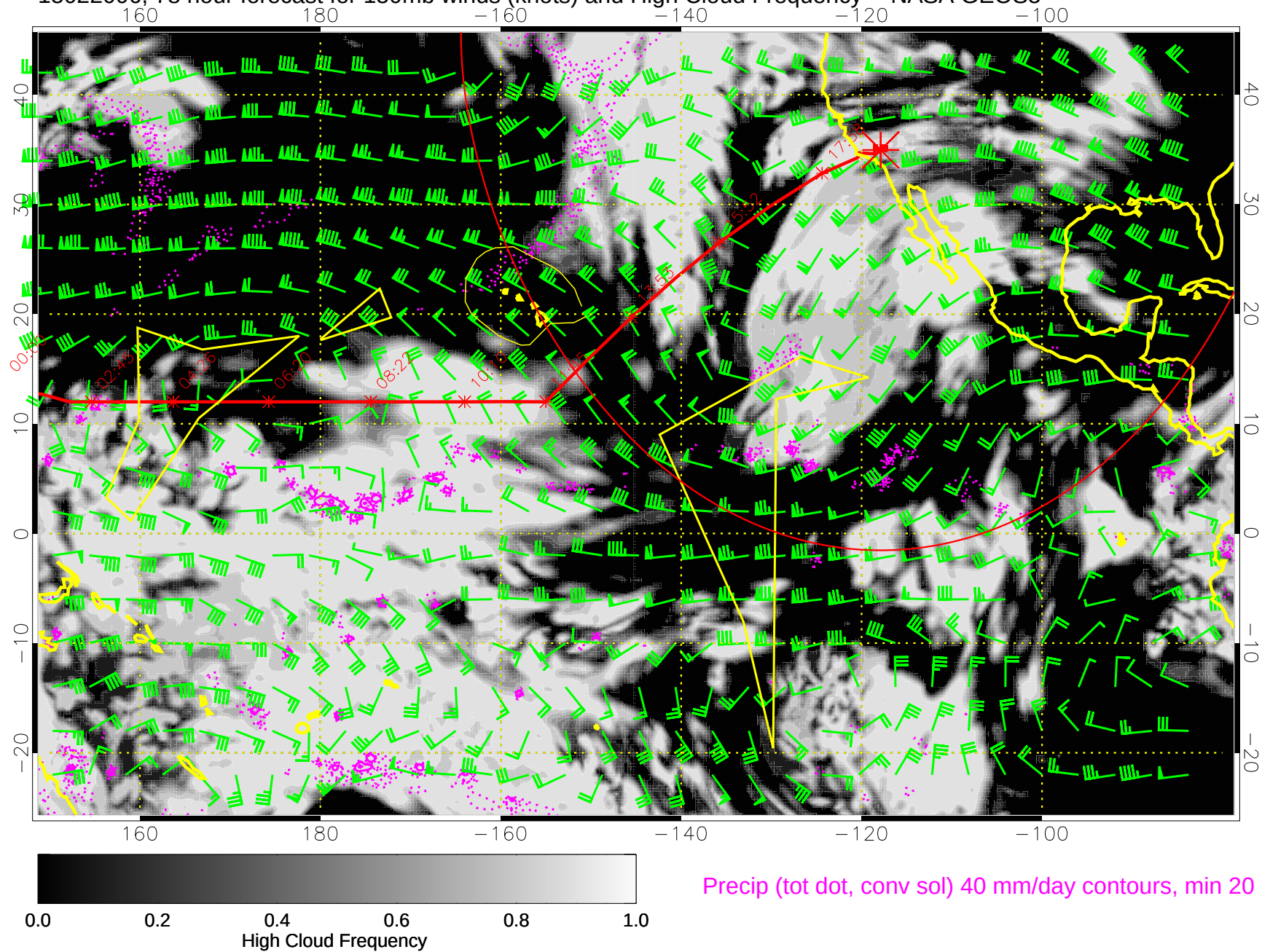
15022006, 78 hour forecast for 150mb winds (knots) and High Cloud Frequency -- NASA GEOS5
