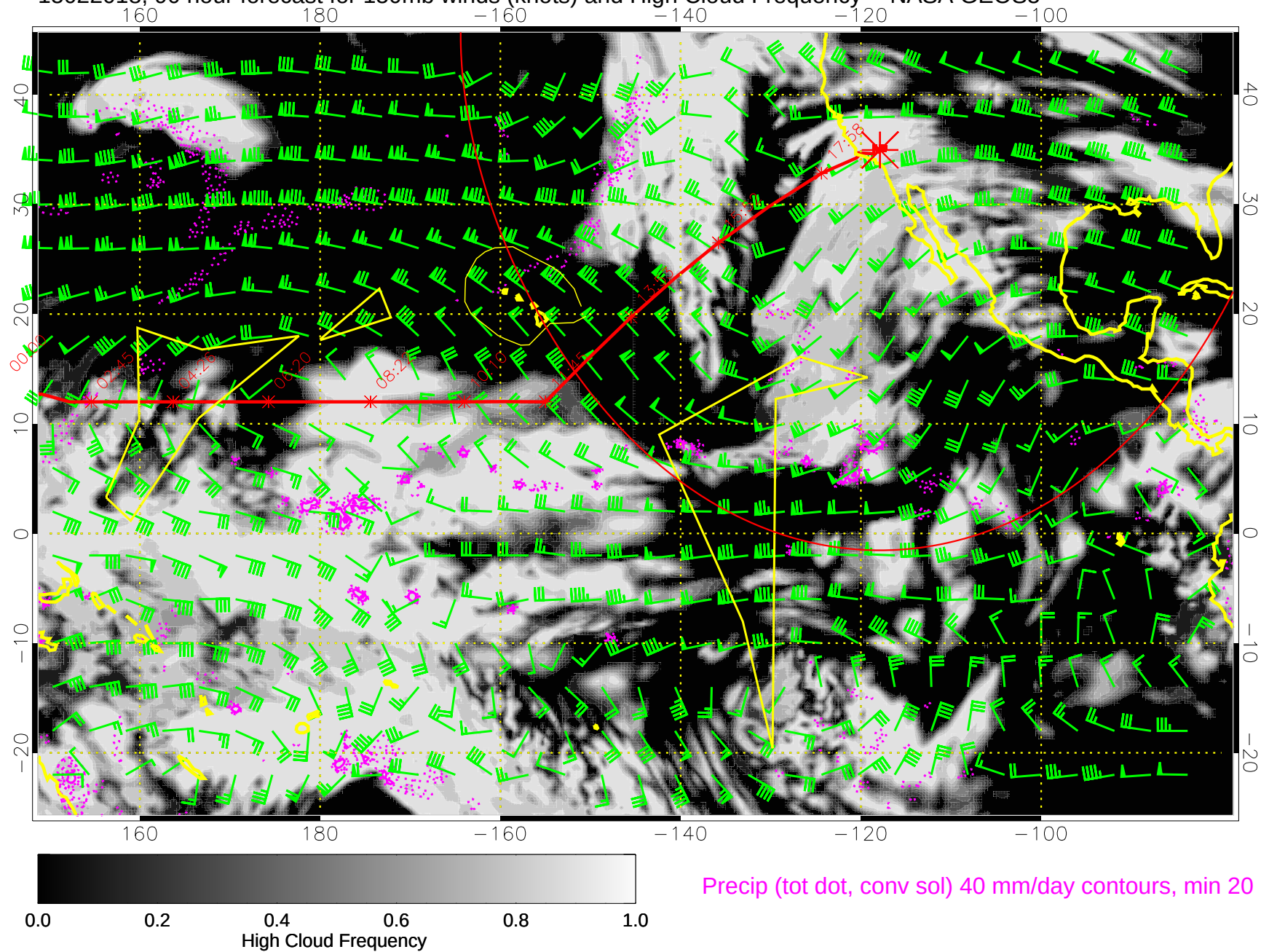
15022018, 90 hour forecast for 150mb winds (knots) and High Cloud Frequency -- NASA GEOS5
