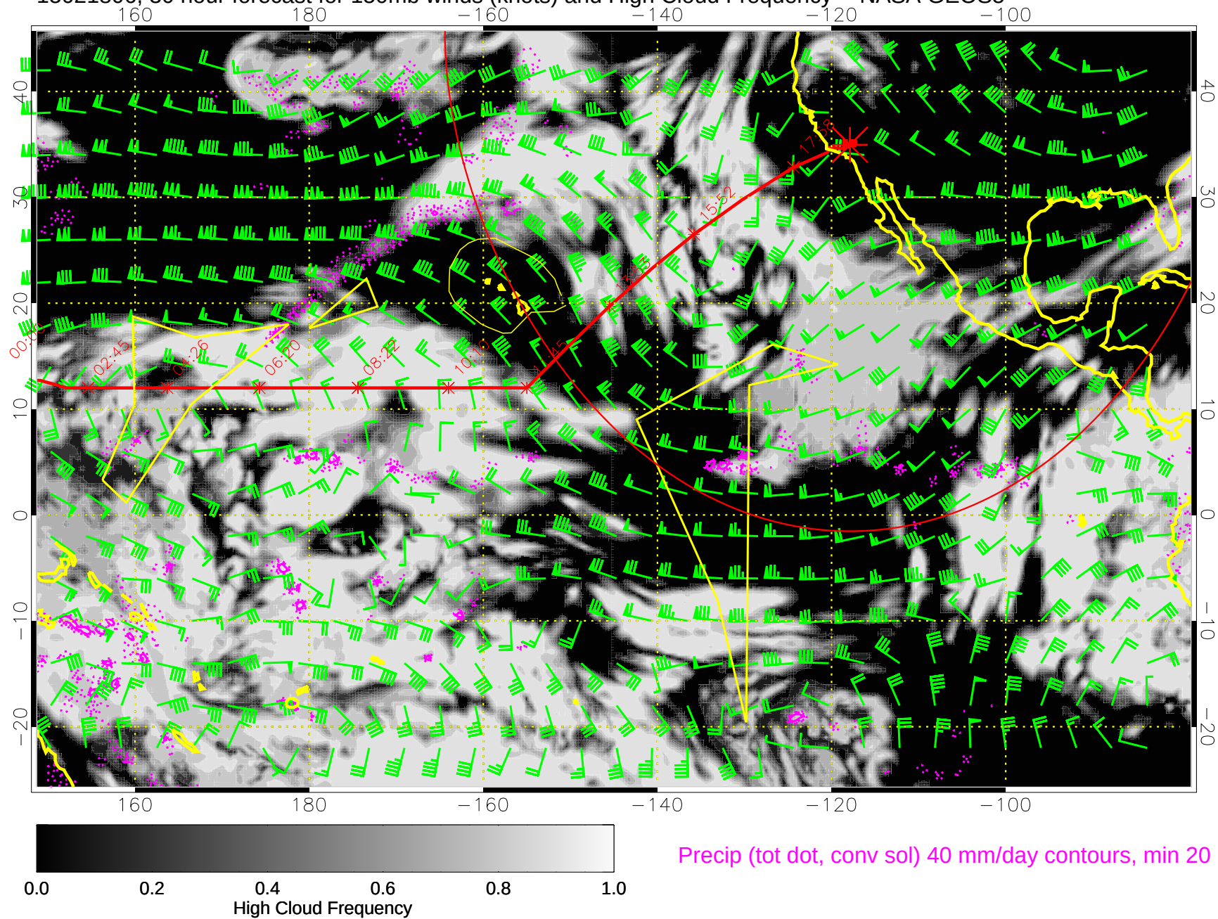
15021806, 30 hour forecast for 150mb winds (knots) and High Cloud Frequency -- NASA GEOS5
