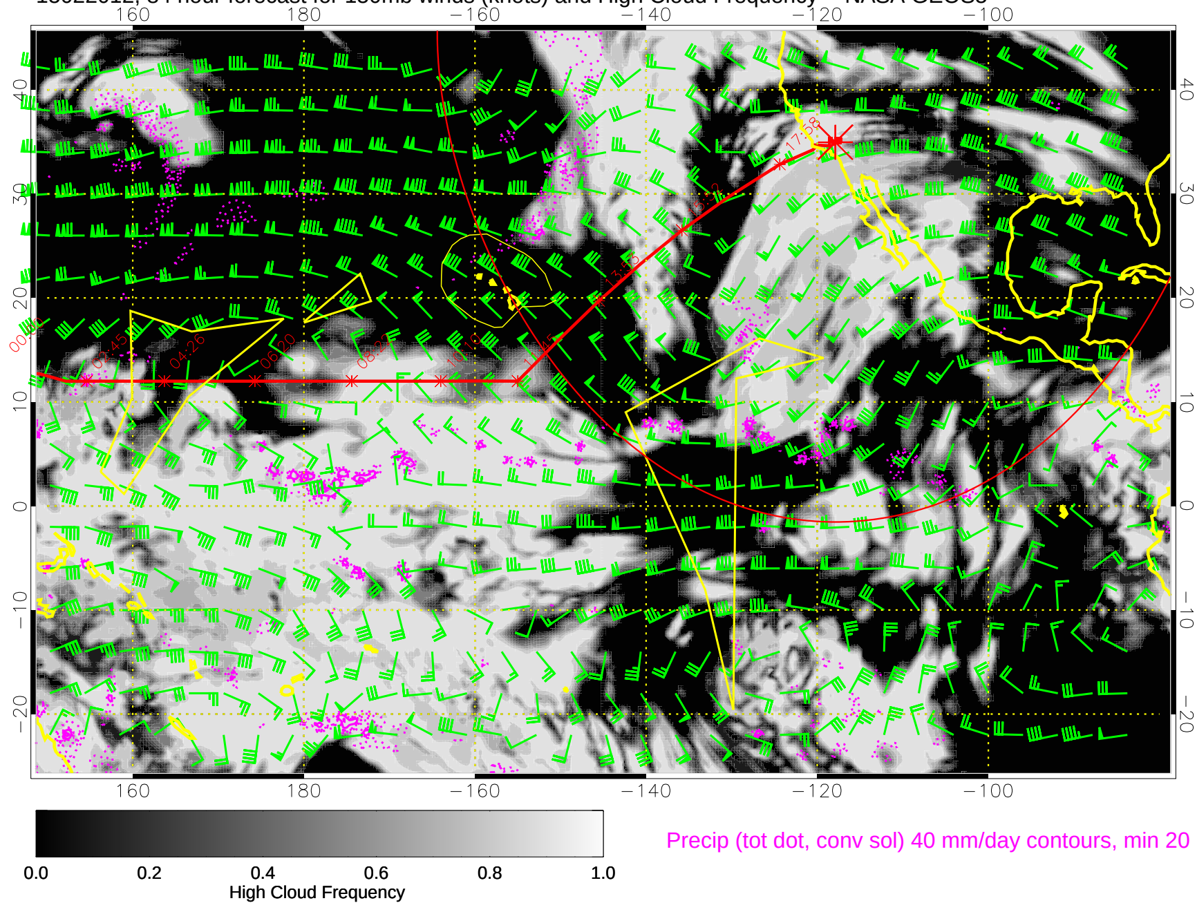
15022012, 84 hour forecast for 150mb winds (knots) and High Cloud Frequency -- NASA GEOS5
