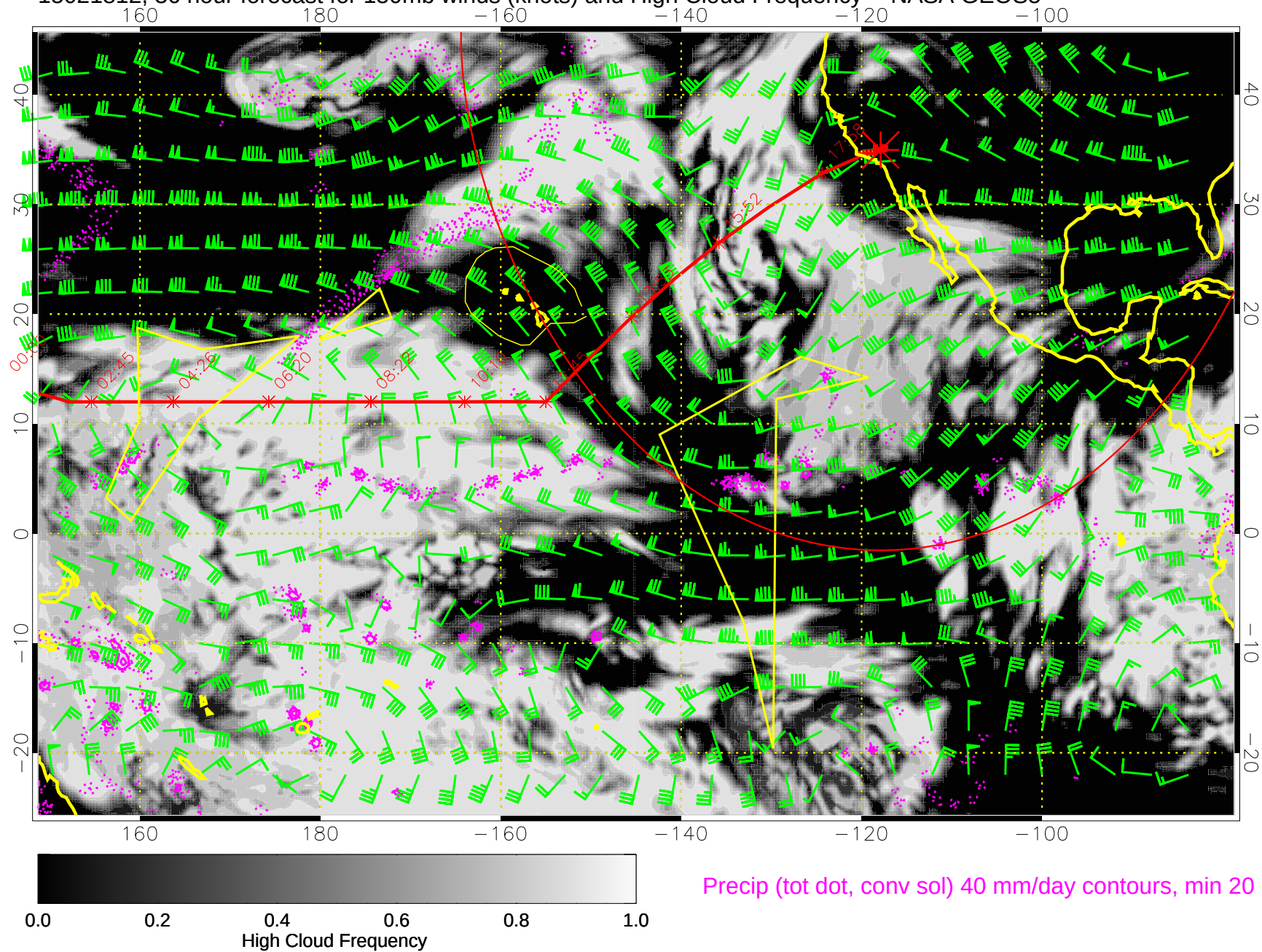
15021812, 36 hour forecast for 150mb winds (knots) and High Cloud Frequency -- NASA GEOS5
