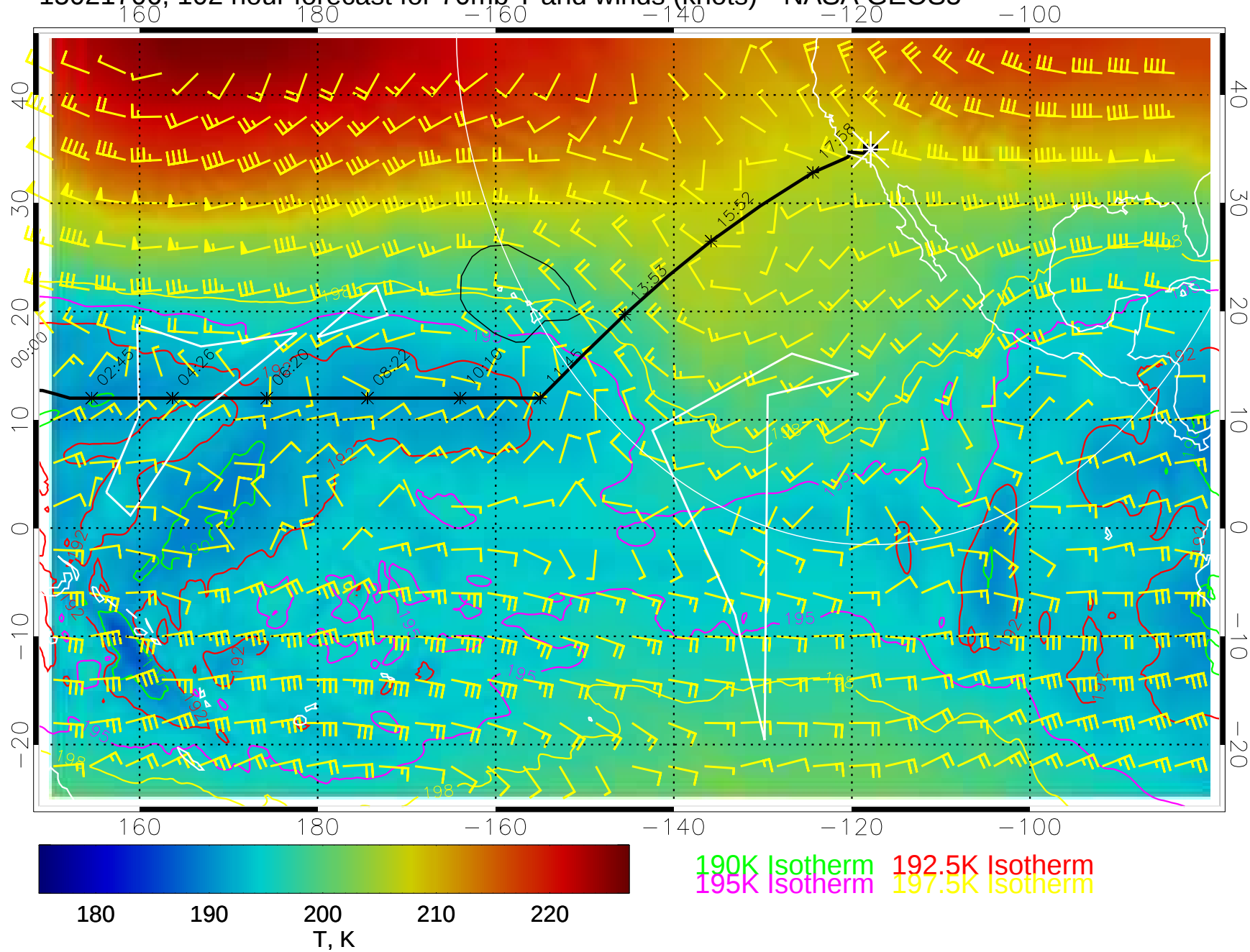
15021706, 102 hour forecast for 70mb T and winds (knots)-- NASA GEOS5
