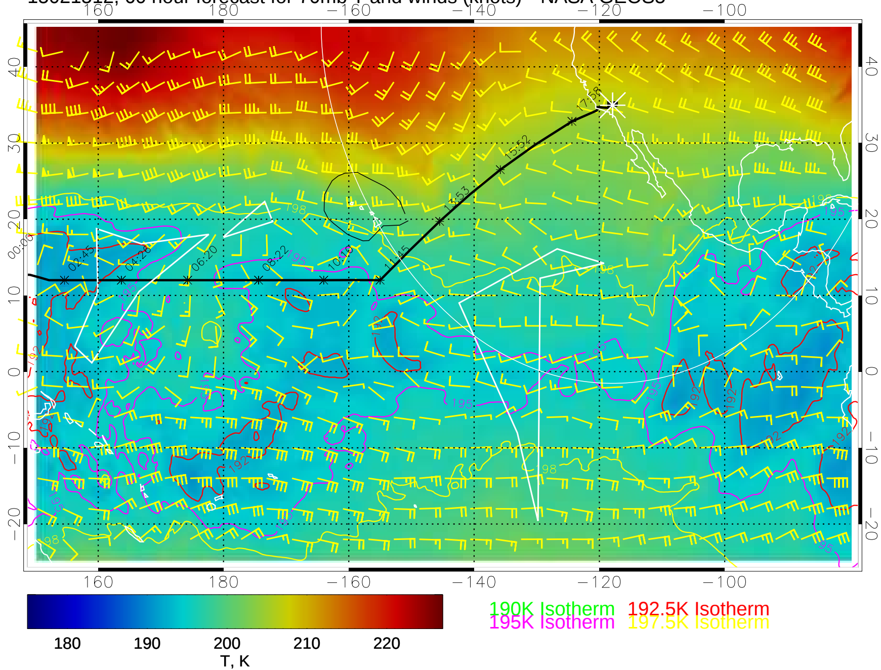
15021512, 60 hour forecast for 70mb T and winds (knots)-- NASA GEOS5
