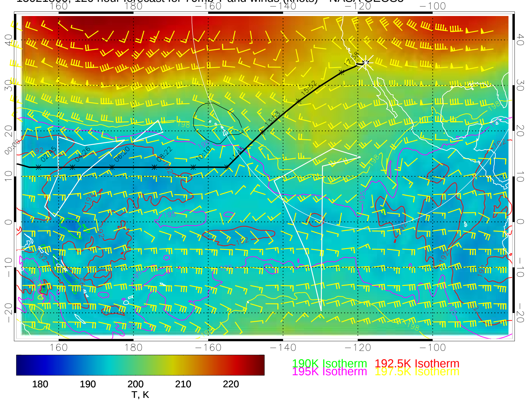
15021800, 120 hour forecast for 70mb T and winds (knots)-- NASA GEOS5
