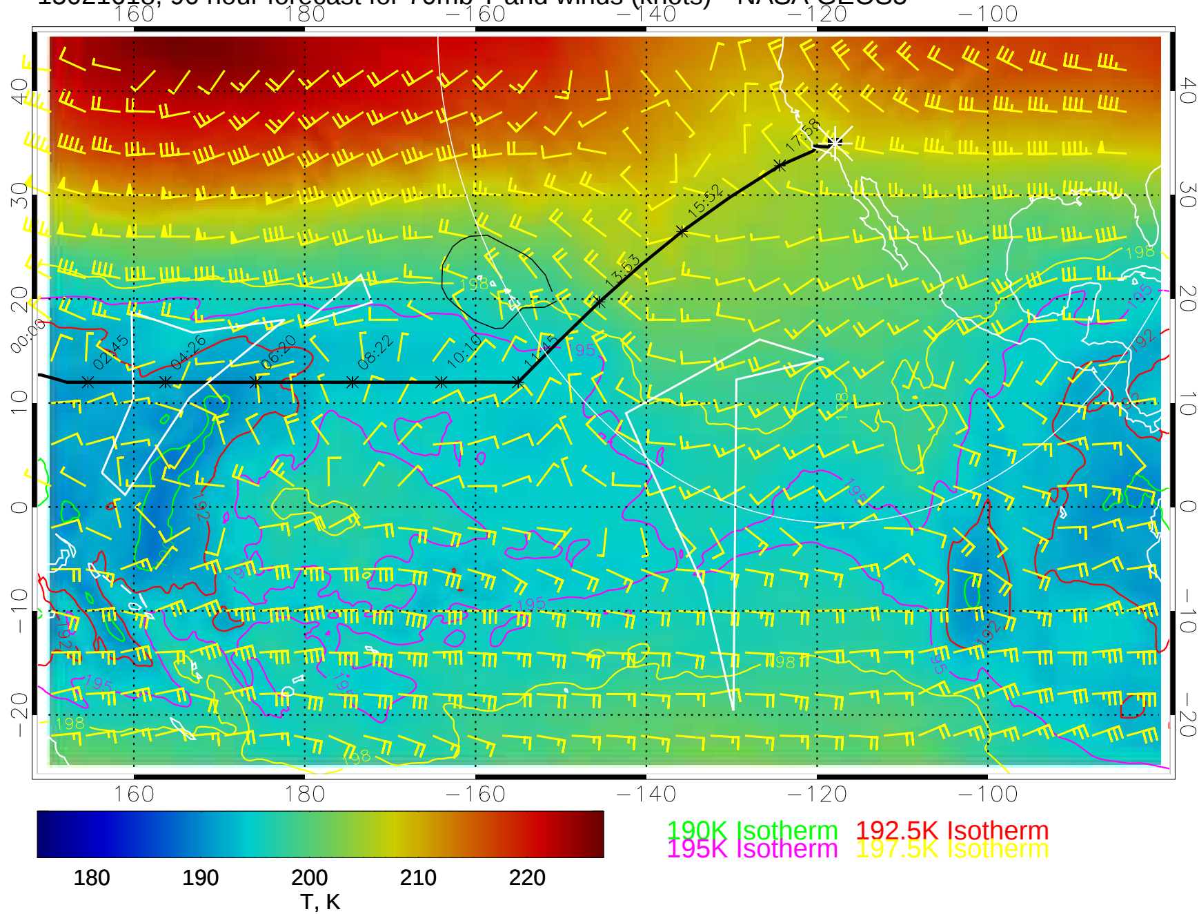
15021618, 90 hour forecast for 70mb T and winds (knots)-- NASA GEOS5
