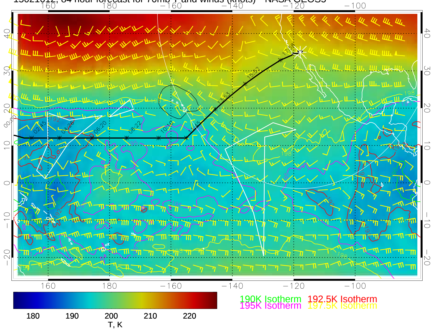
15021612, 84 hour forecast for 70mb T and winds (knots)-- NASA GEOS5
