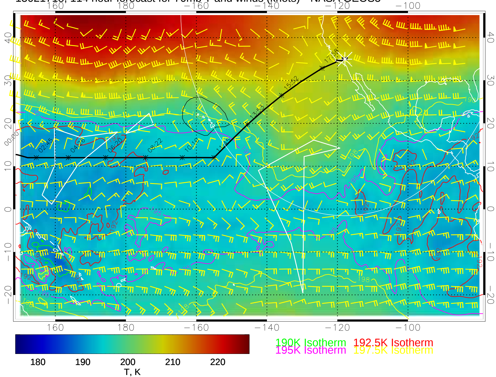
15021718, 114 hour forecast for 70mb T and winds (knots)-- NASA GEOS5
