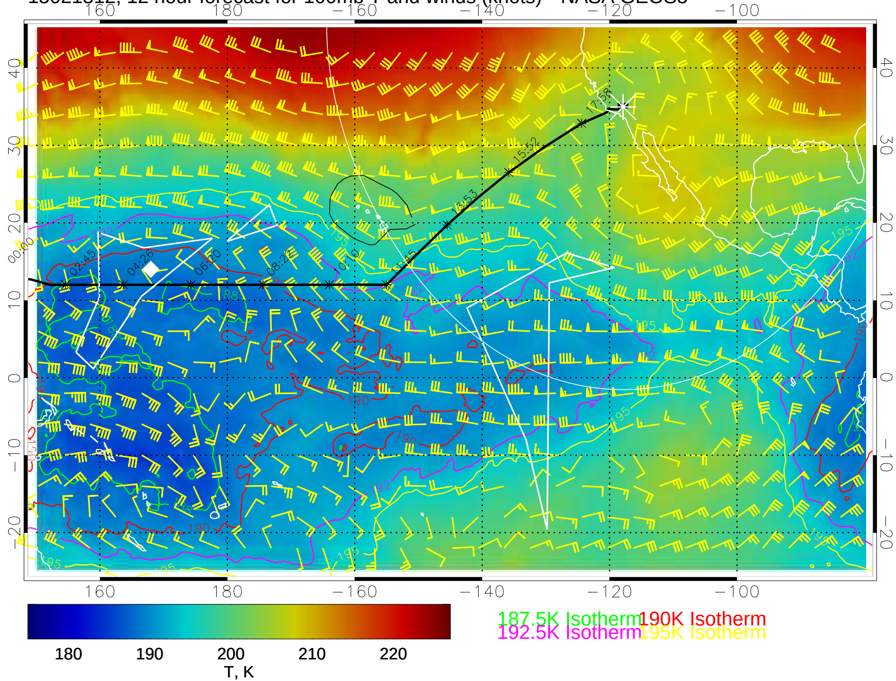
15021312, 12 hour forecast for 100mb T and winds (knots)-- NASA GEOS5
