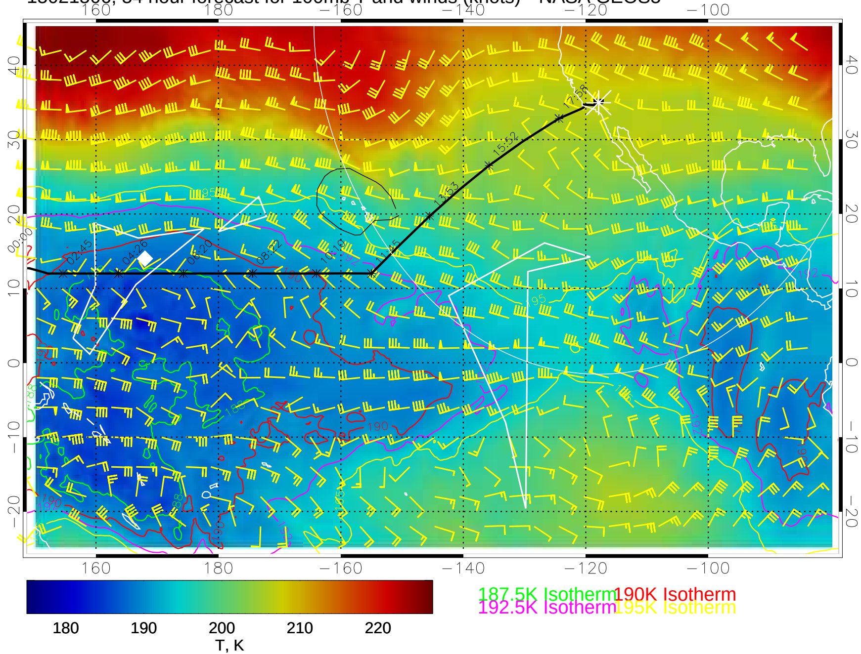
15021506, 54 hour forecast for 100mb T and winds (knots)-- NASA GEOS5
