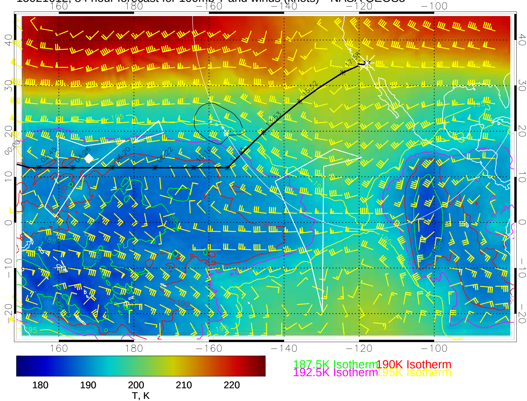
15021612, 84 hour forecast for 100mb T and winds (knots)-- NASA GEOS5
