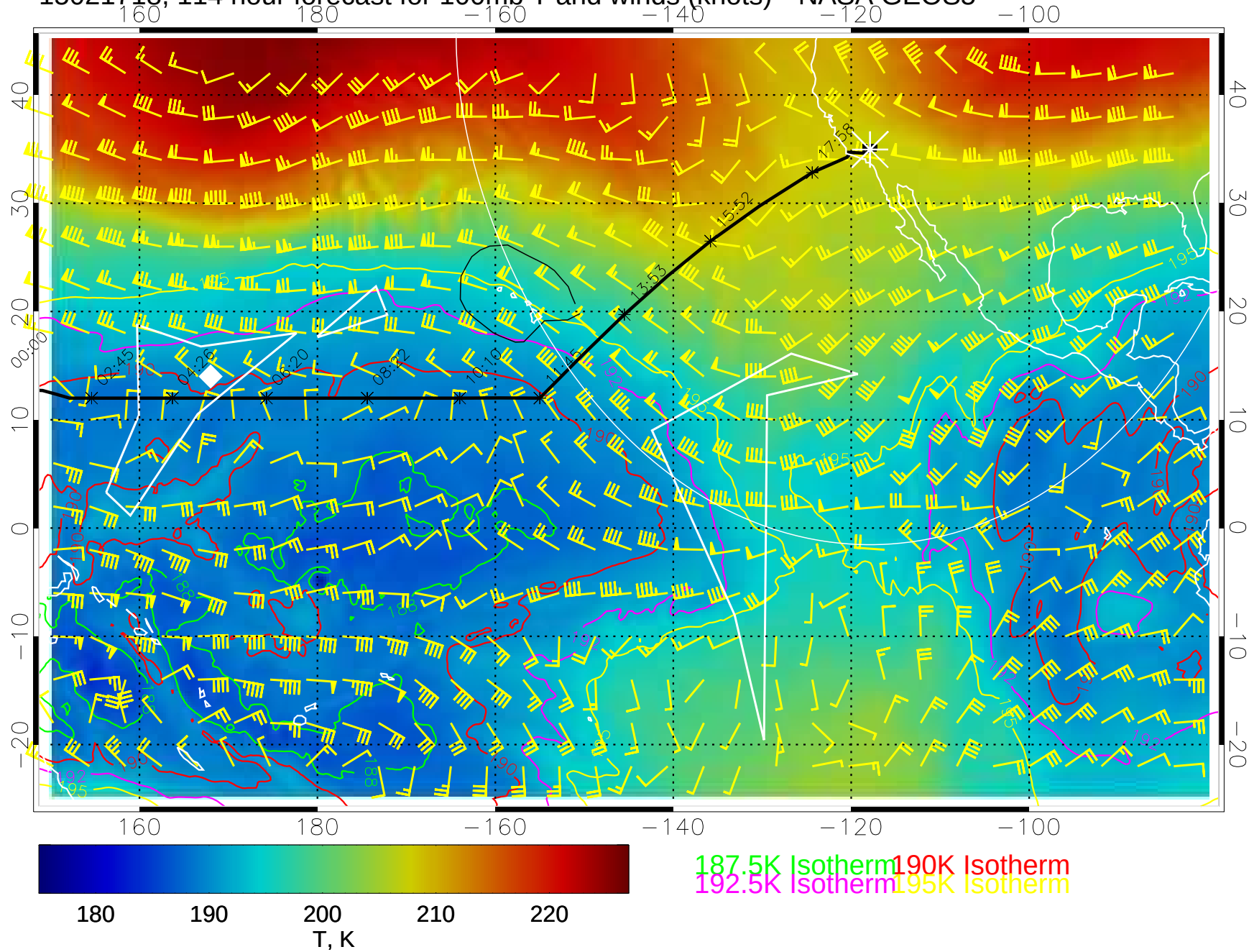
15021718, 114 hour forecast for 100mb T and winds (knots)-- NASA GEOS5
