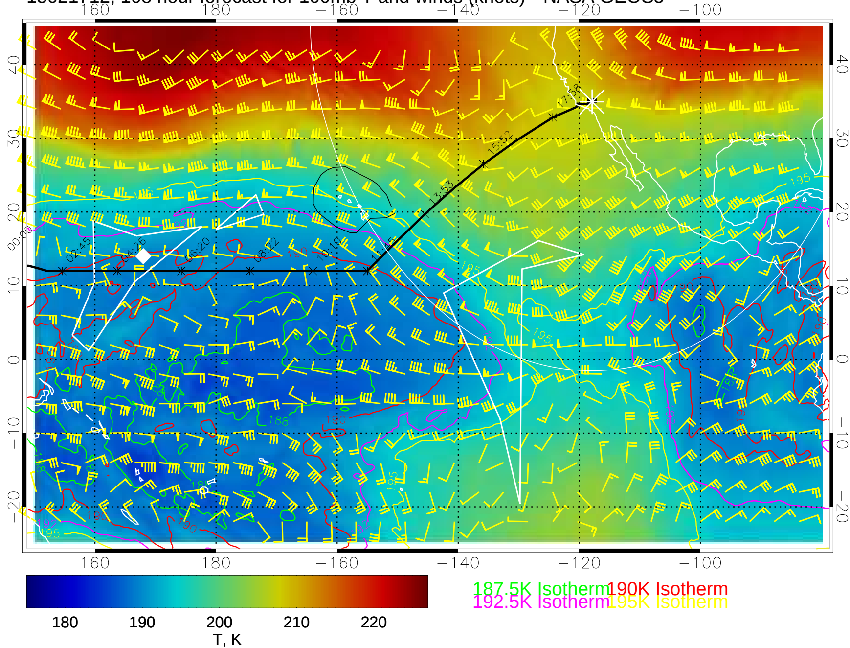
15021712, 108 hour forecast for 100mb T and winds (knots)-- NASA GEOS5
