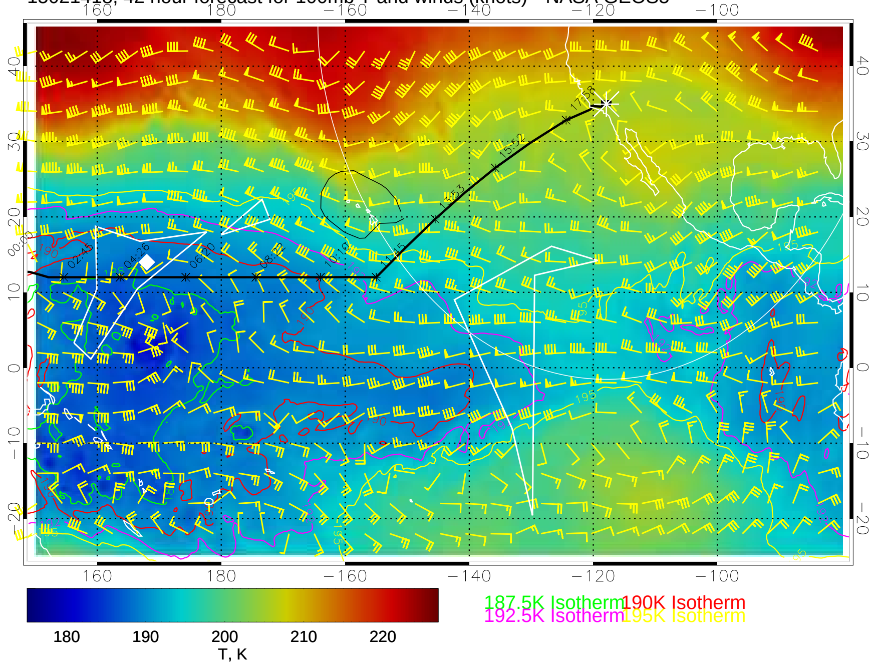
15021418, 42 hour forecast for 100mb T and winds (knots)-- NASA GEOS5
