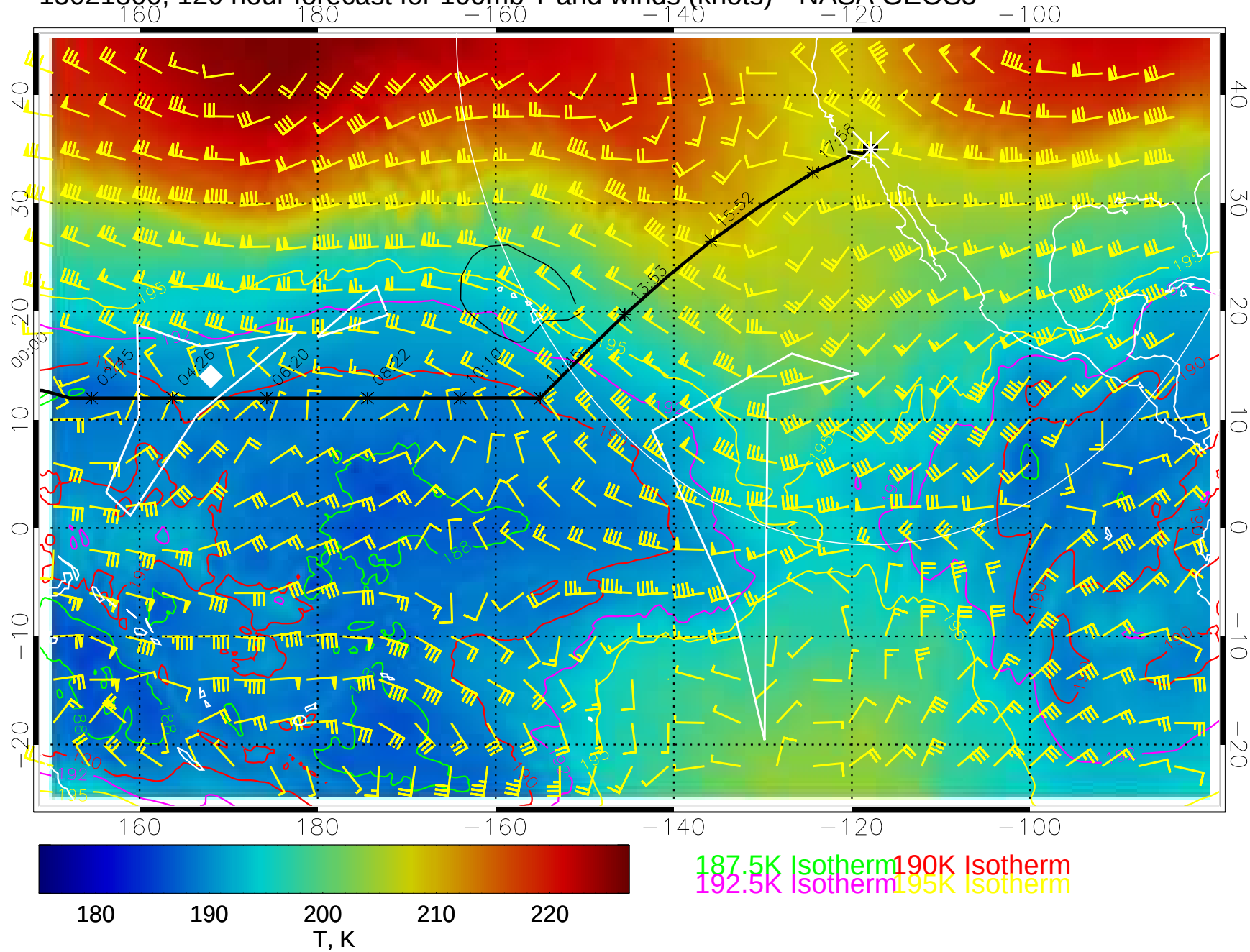
15021800, 120 hour forecast for 100mb T and winds (knots)-- NASA GEOS5
