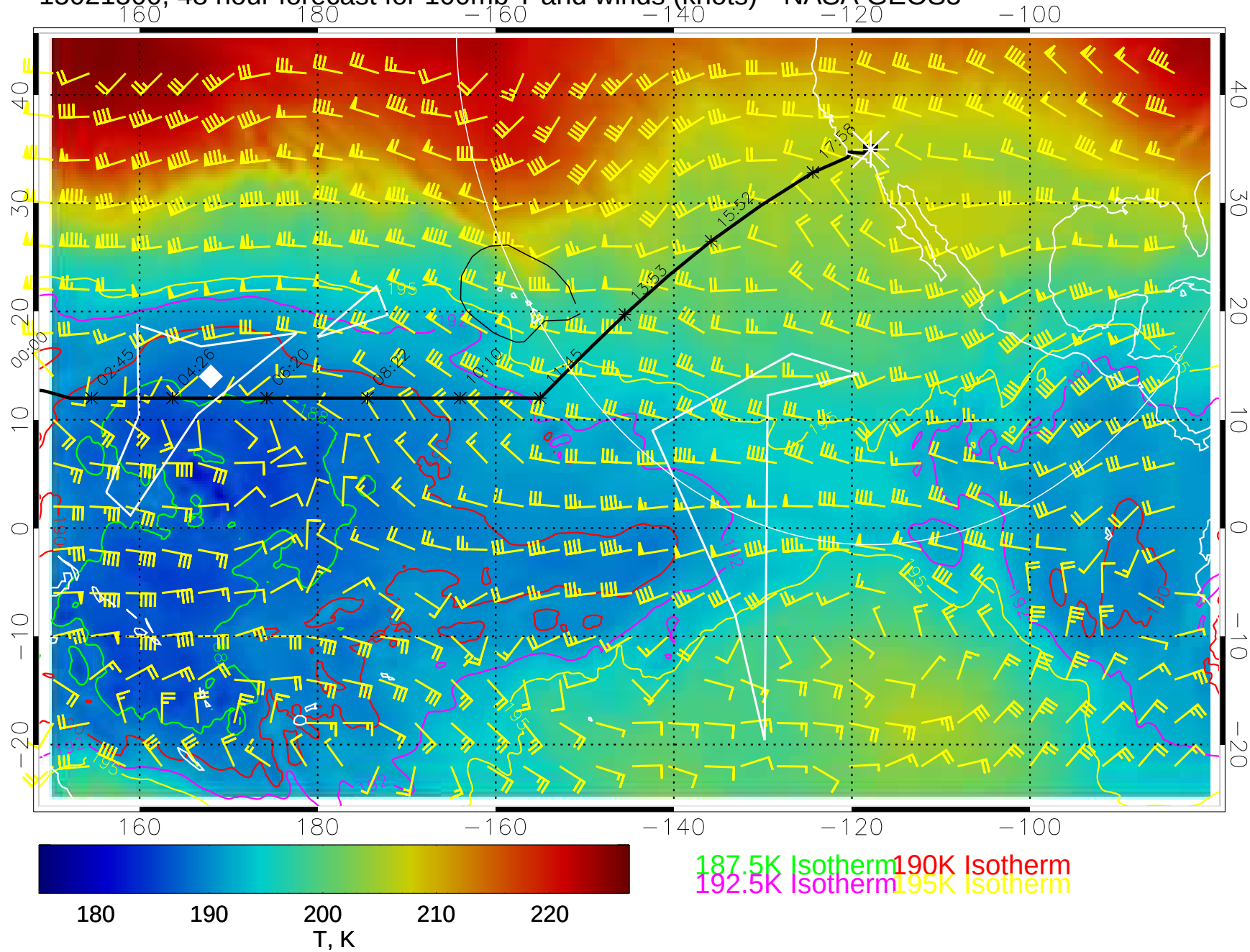
15021500, 48 hour forecast for 100mb T and winds (knots)-- NASA GEOS5
