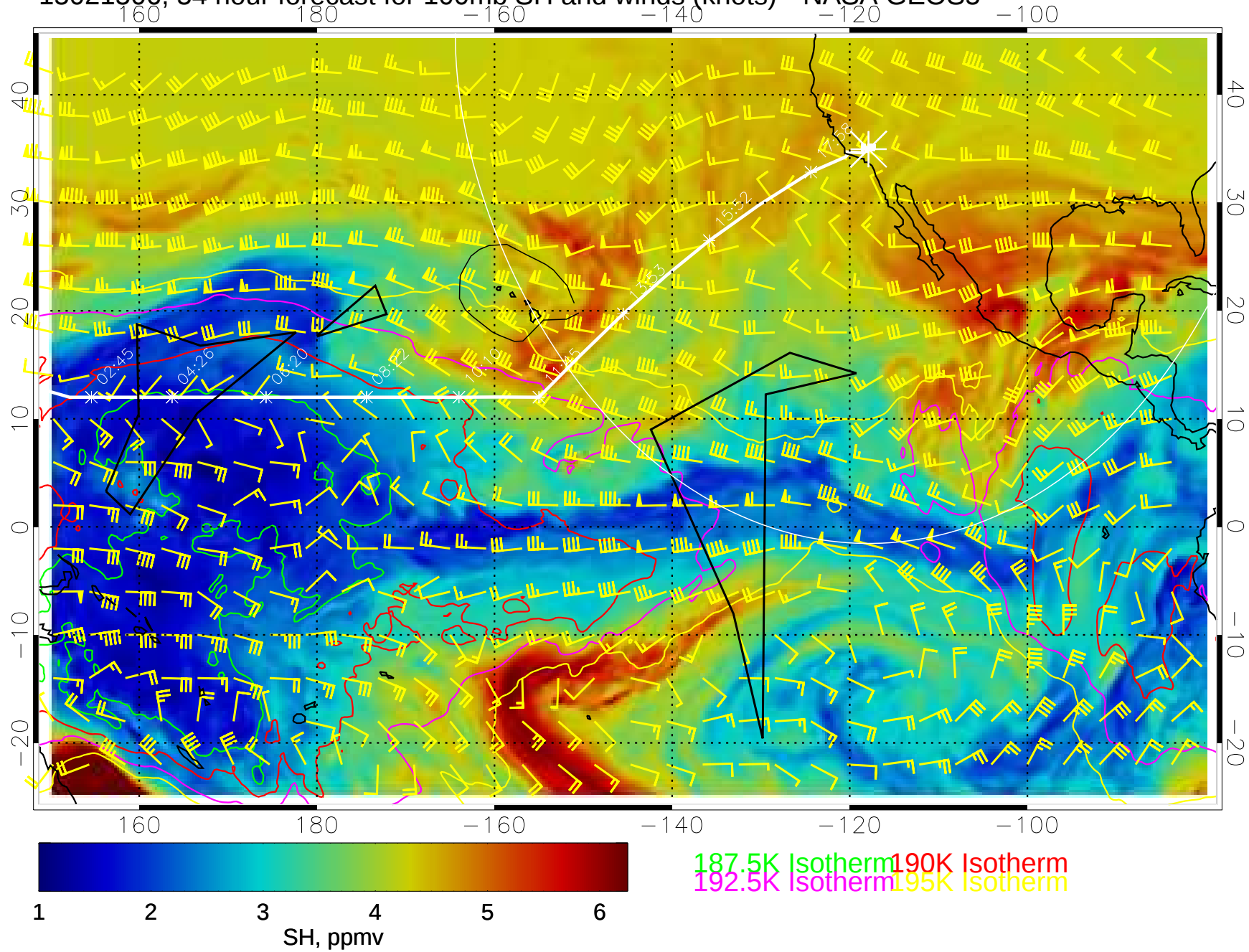
15021506, 54 hour forecast for 100mb SH and winds (knots)-- NASA GEOS5
