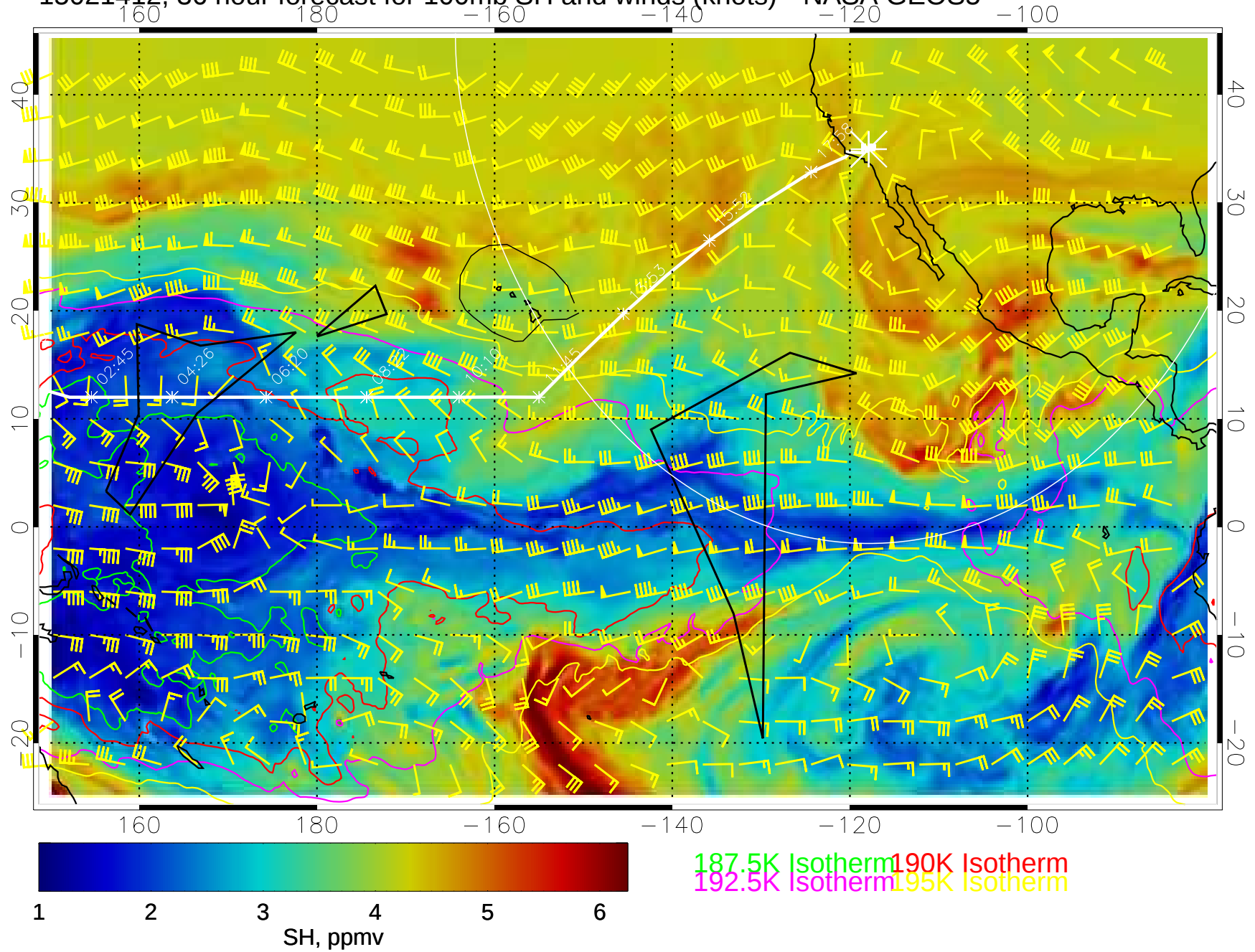
15021412, 36 hour forecast for 100mb SH and winds (knots)-- NASA GEOS5
