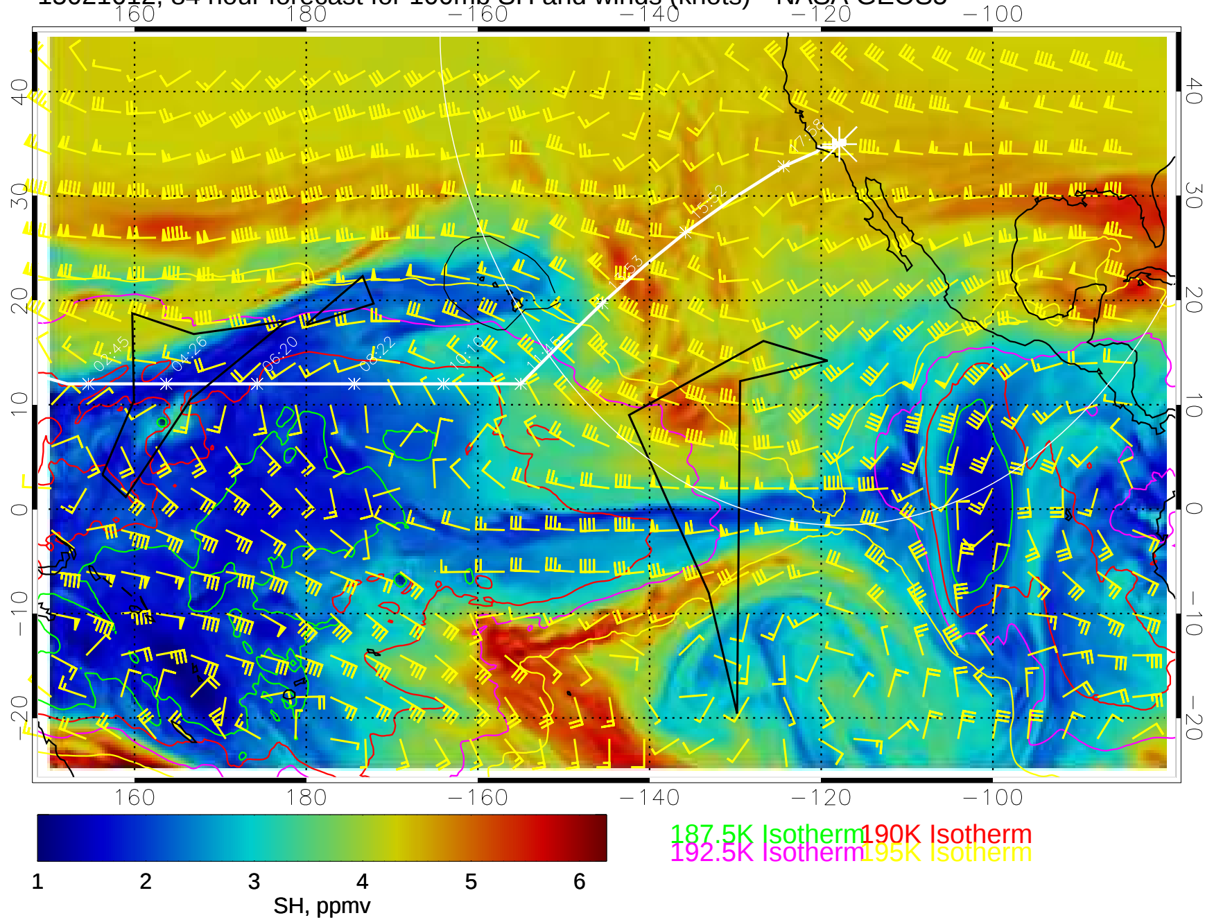
15021612, 84 hour forecast for 100mb SH and winds (knots)-- NASA GEOS5
