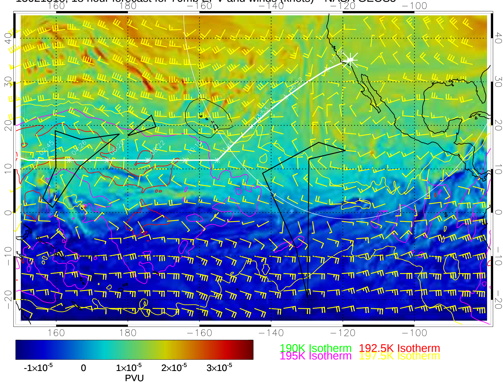
15021318, 18 hour forecast for 70mb EPV and winds (knots)-- NASA GEOS5
