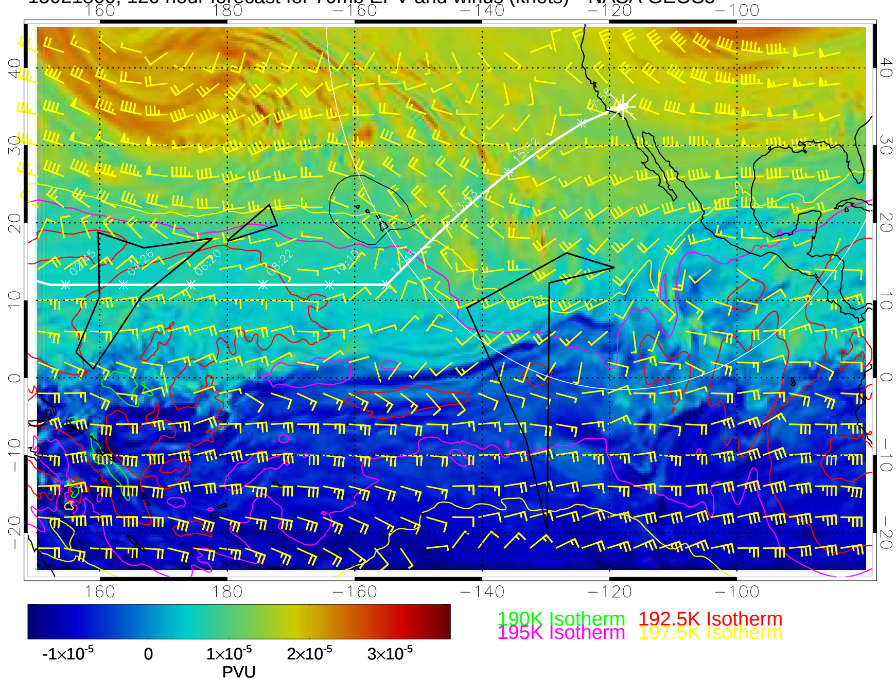
15021800, 120 hour forecast for 70mb EPV and winds (knots)-- NASA GEOS5
