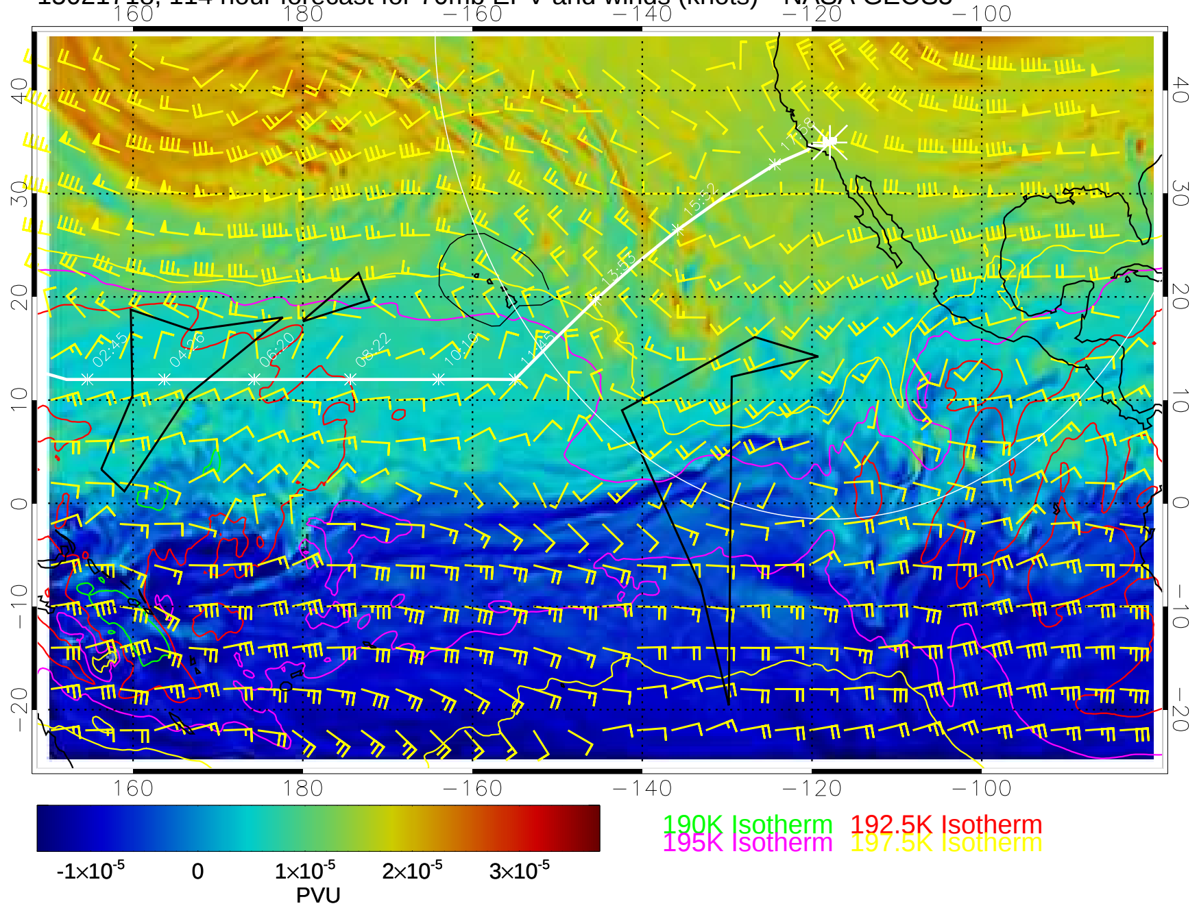
15021718, 114 hour forecast for 70mb EPV and winds (knots)-- NASA GEOS5
