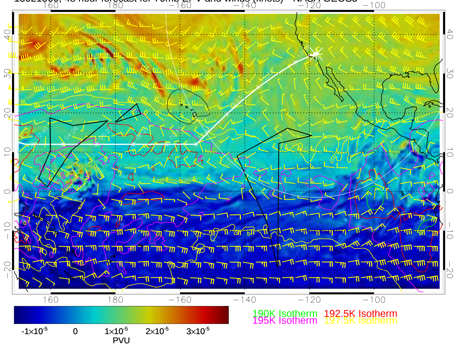
15021500, 48 hour forecast for 70mb EPV and winds (knots)-- NASA GEOS5
