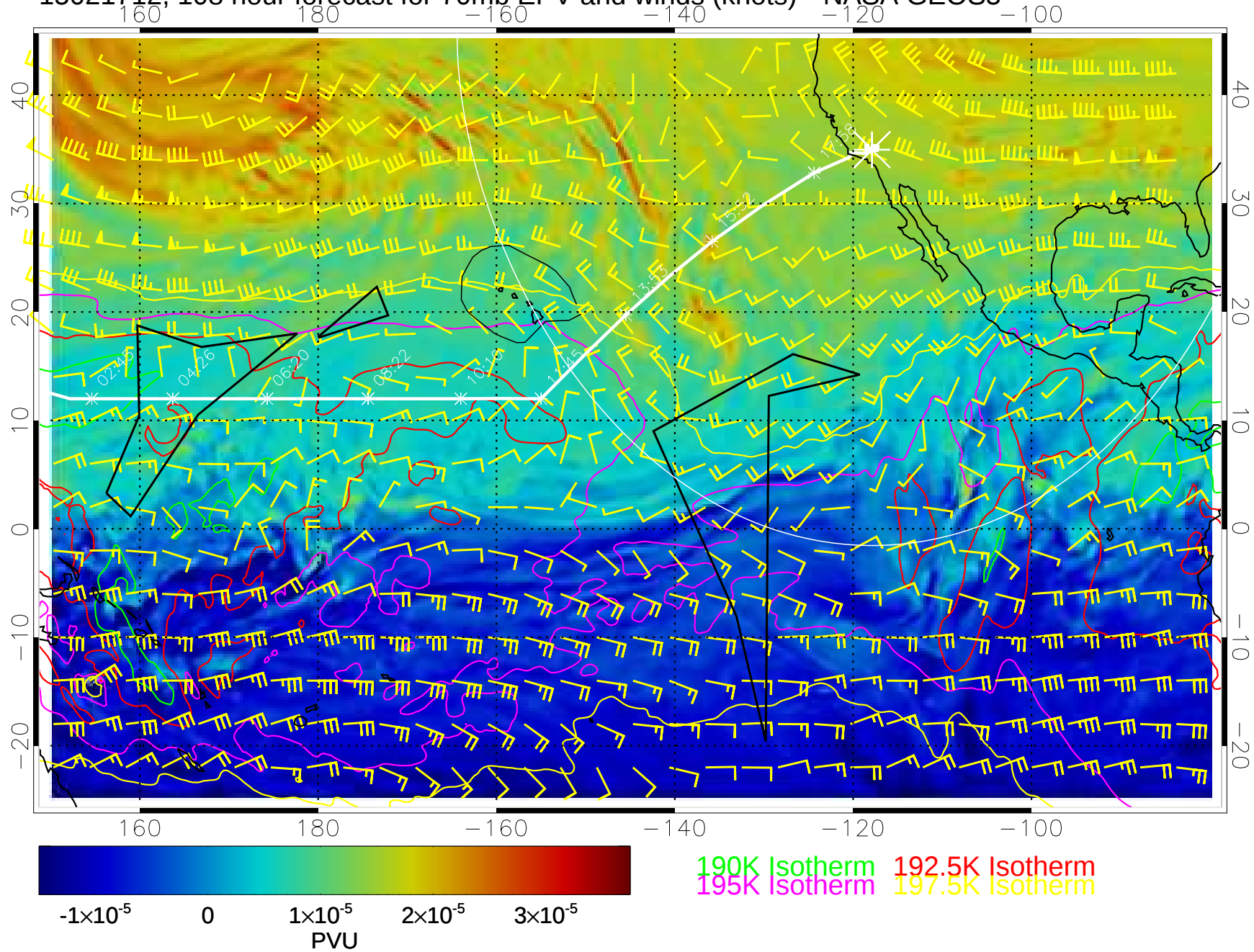
15021712, 108 hour forecast for 70mb EPV and winds (knots)-- NASA GEOS5
