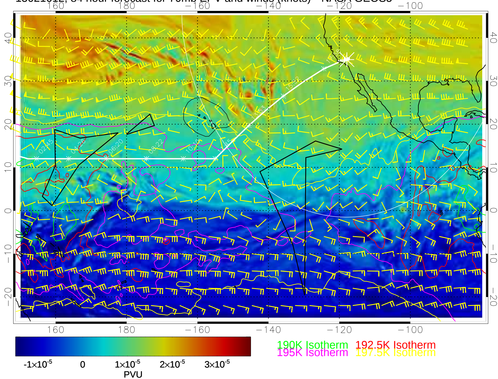
15021612, 84 hour forecast for 70mb EPV and winds (knots)-- NASA GEOS5
