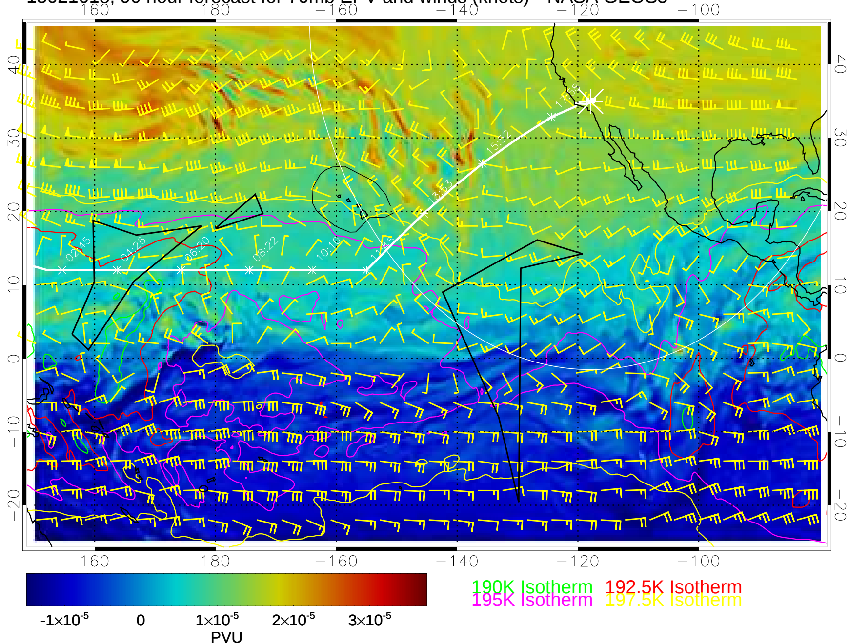
15021618, 90 hour forecast for 70mb EPV and winds (knots)-- NASA GEOS5
