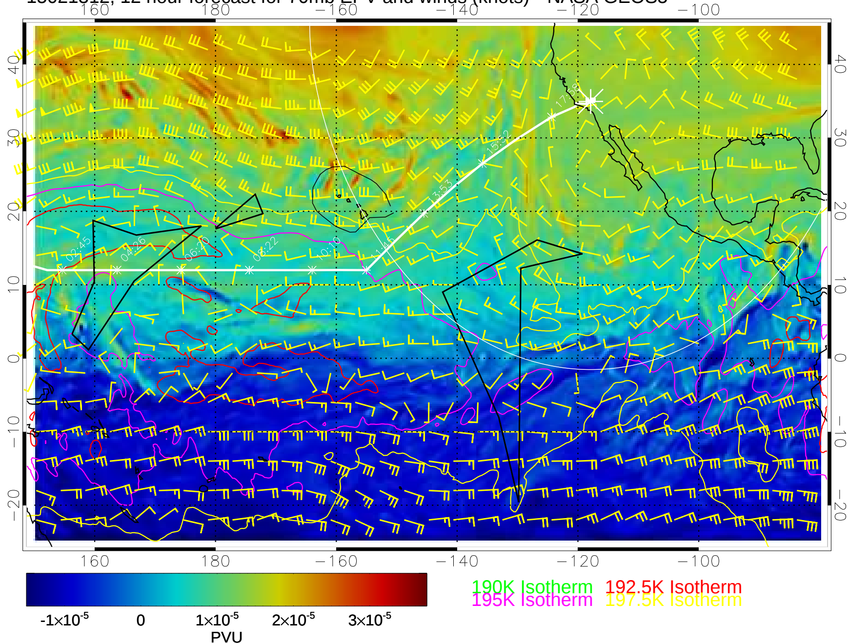
15021312, 12 hour forecast for 70mb EPV and winds (knots)-- NASA GEOS5
