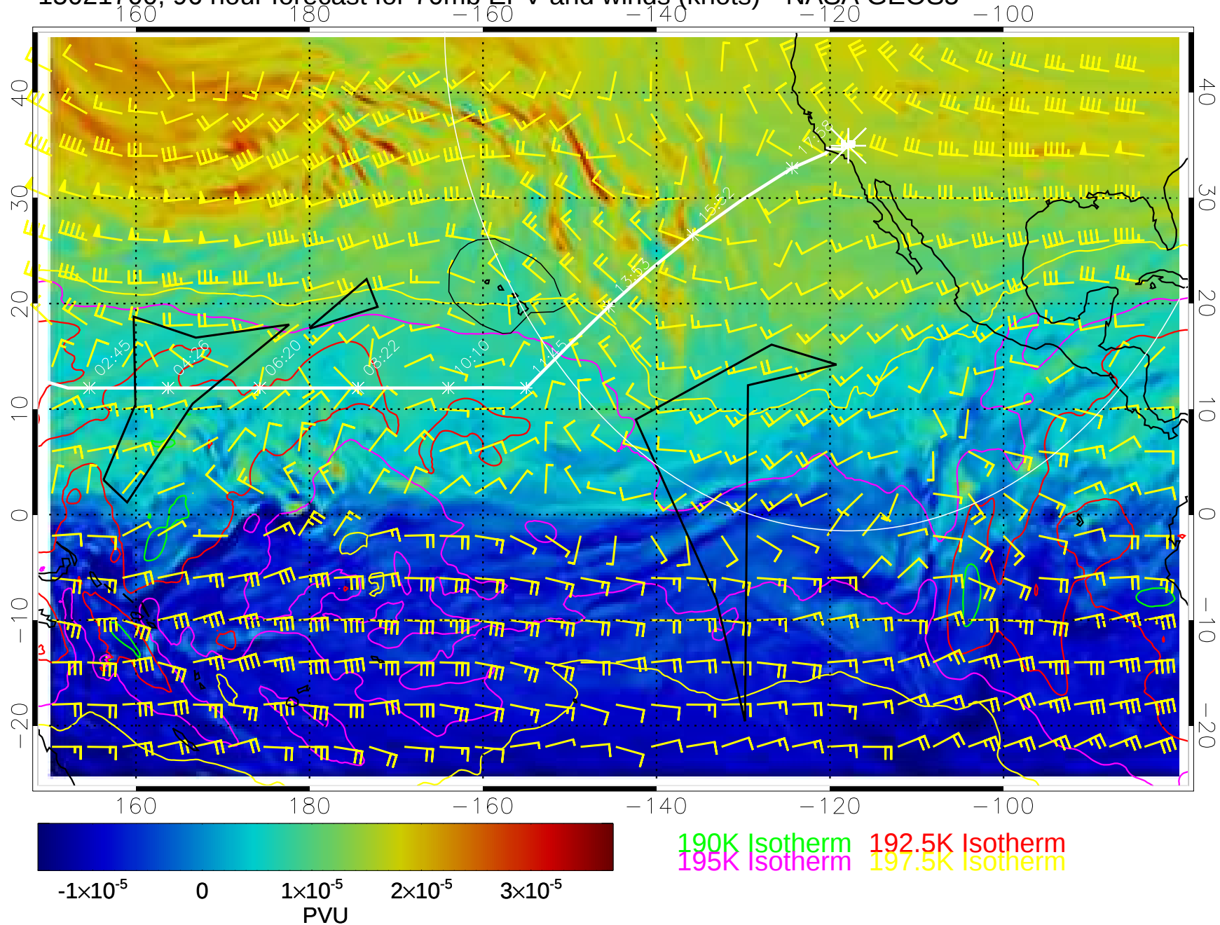
15021700, 96 hour forecast for 70mb EPV and winds (knots)-- NASA GEOS5
