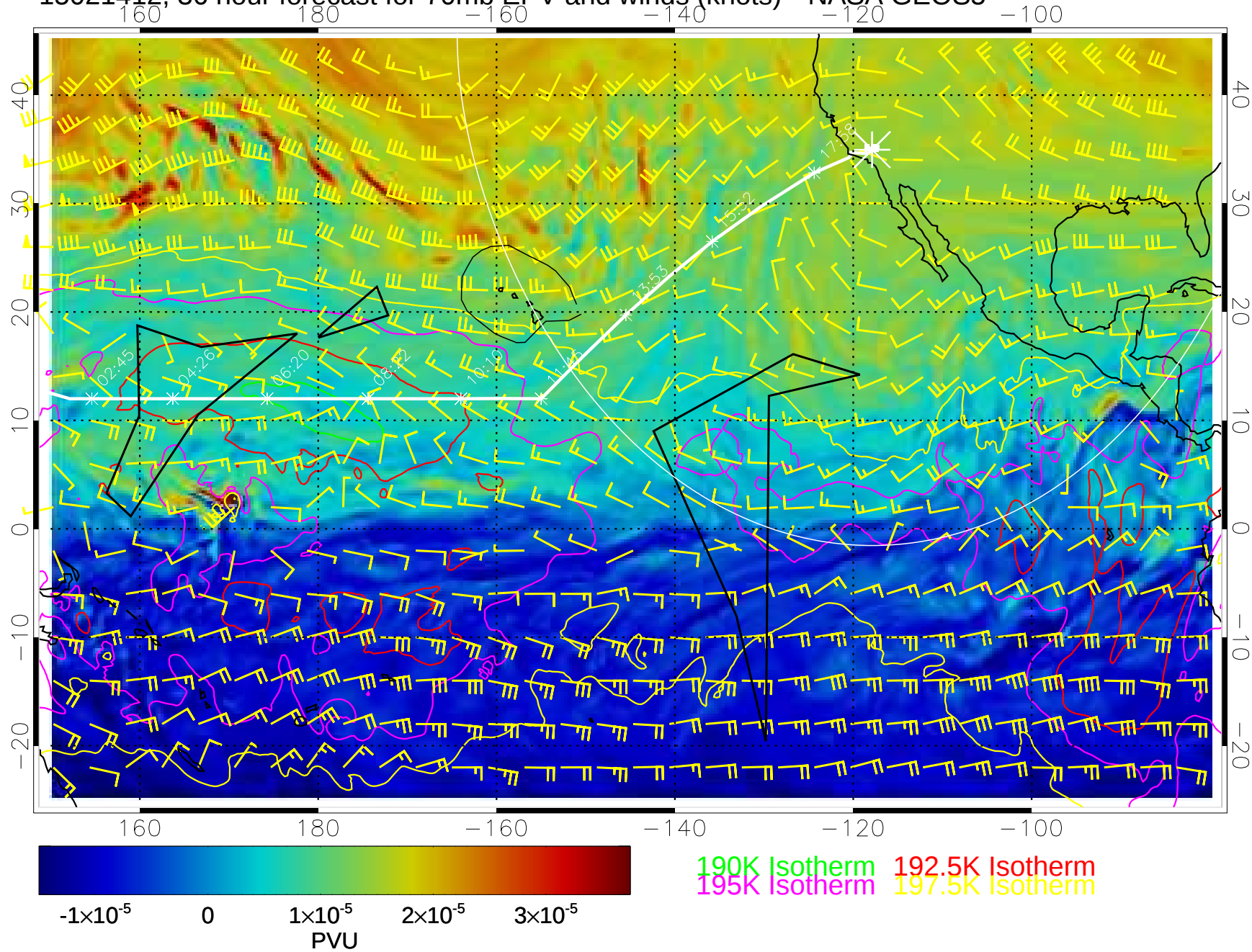
15021412, 36 hour forecast for 70mb EPV and winds (knots)-- NASA GEOS5
