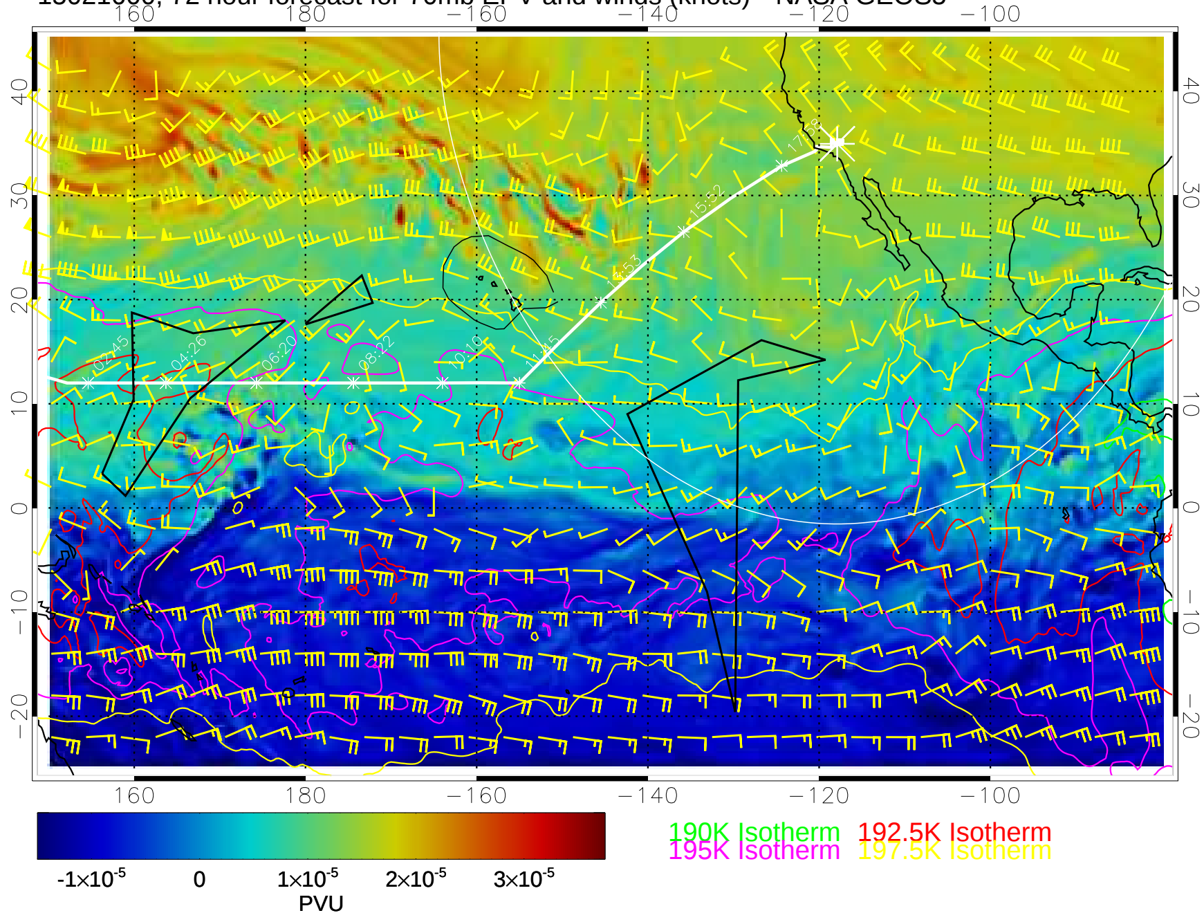
15021600, 72 hour forecast for 70mb EPV and winds (knots)-- NASA GEOS5
