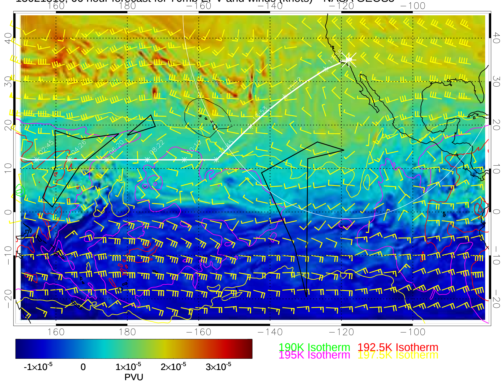
15021518, 66 hour forecast for 70mb EPV and winds (knots)-- NASA GEOS5
