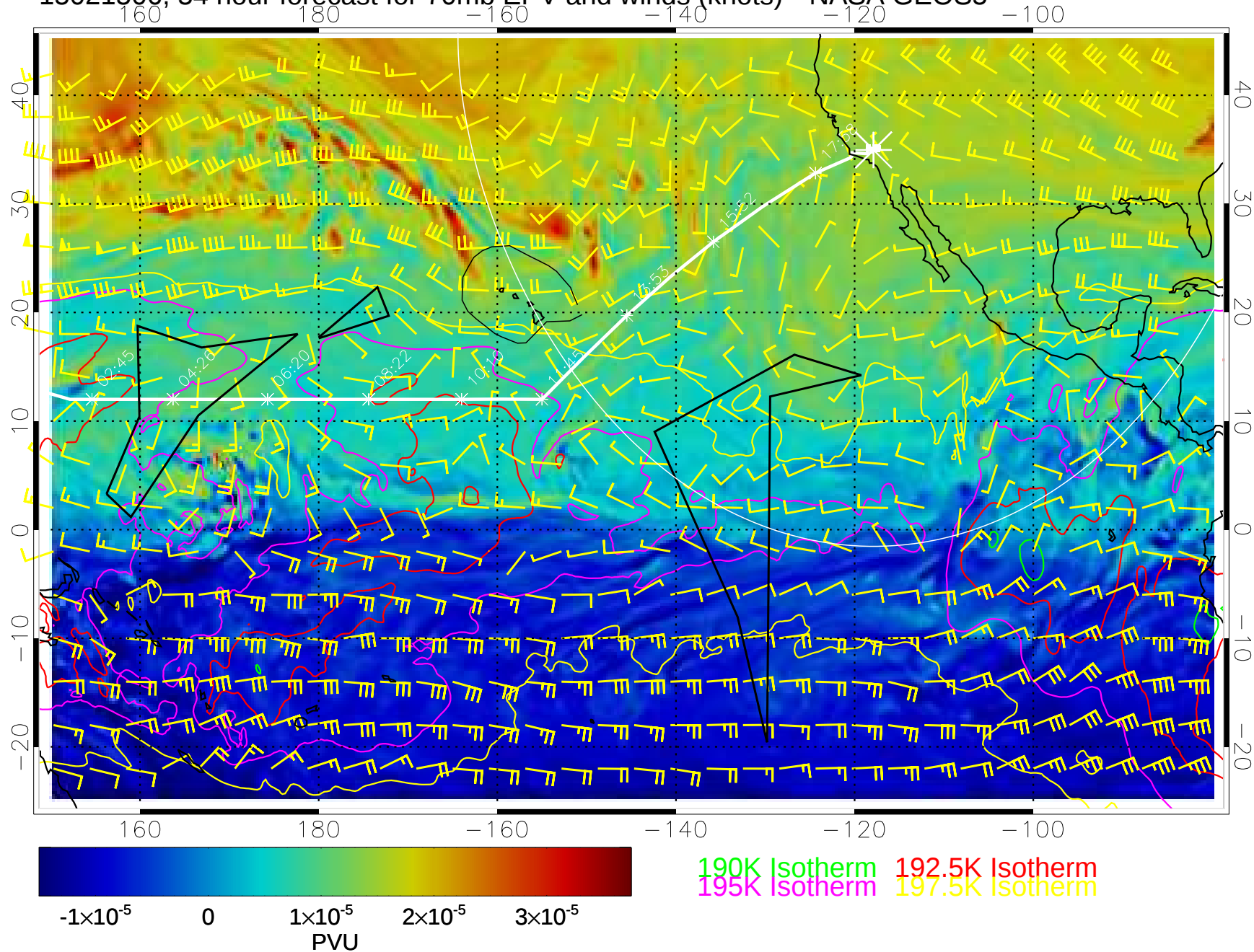
15021506, 54 hour forecast for 70mb EPV and winds (knots)-- NASA GEOS5
