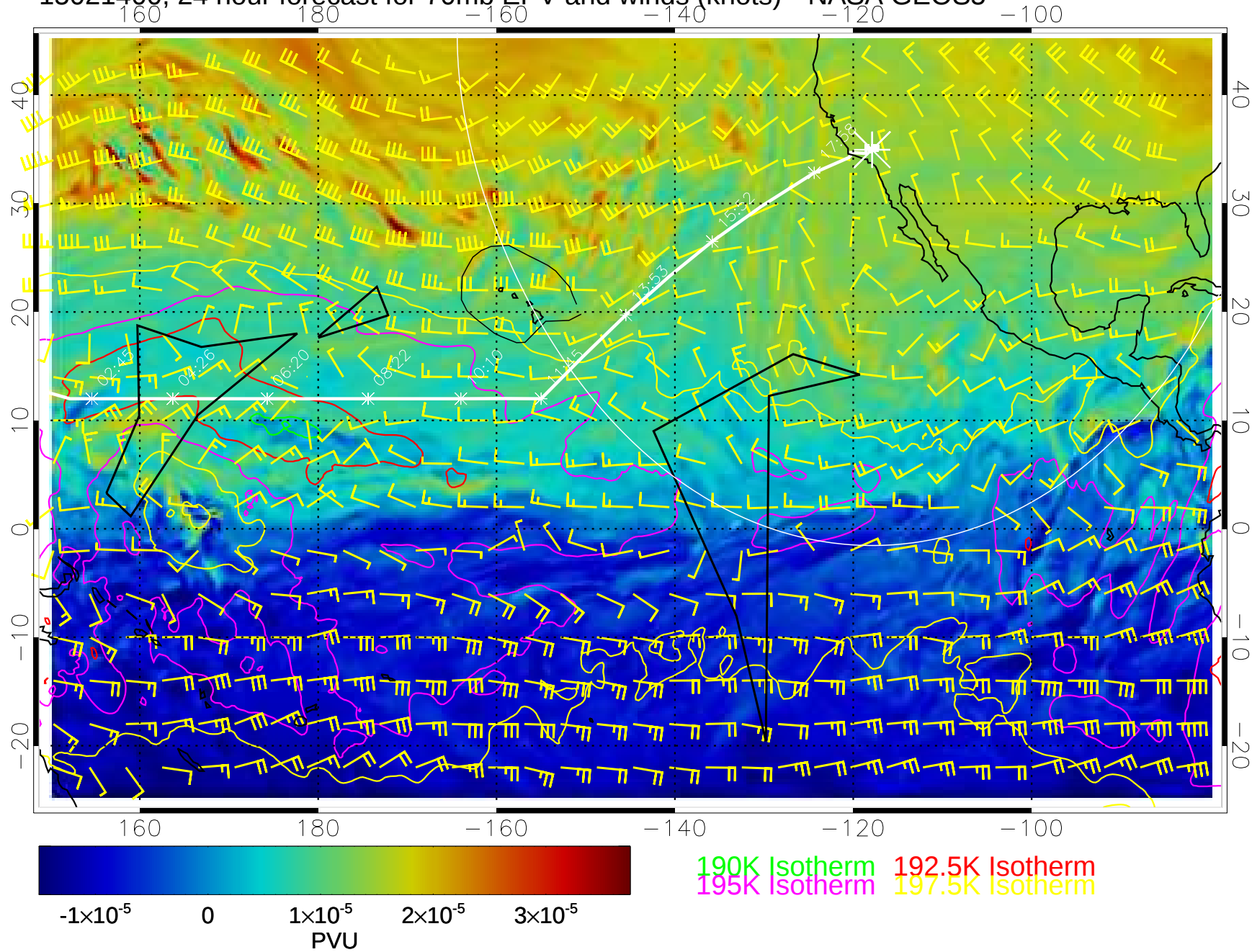
15021400, 24 hour forecast for 70mb EPV and winds (knots)-- NASA GEOS5
