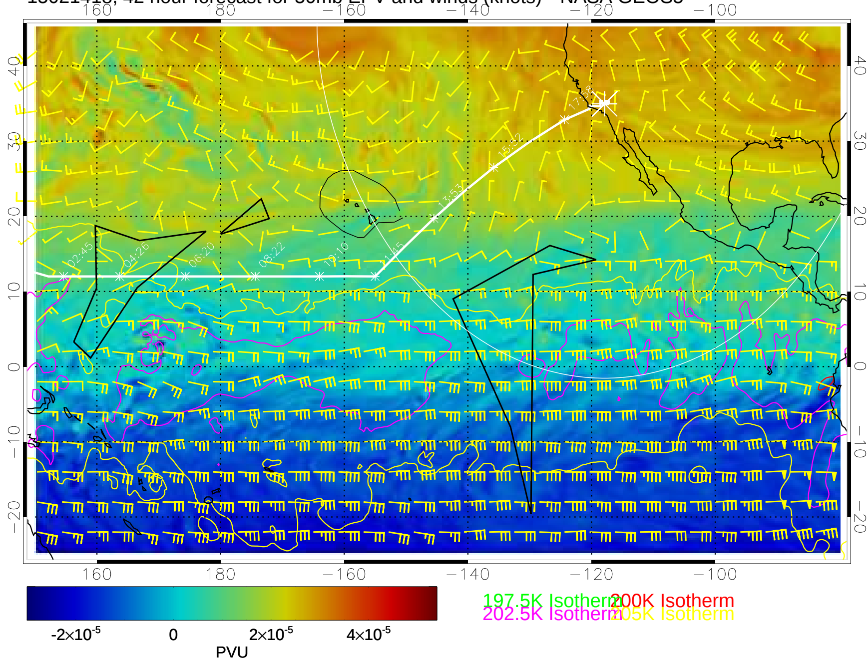
15021418, 42 hour forecast for 50mb EPV and winds (knots)-- NASA GEOS5
