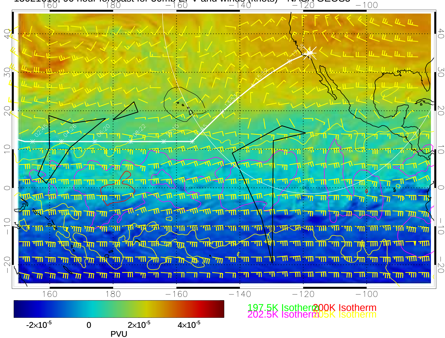
15021618, 90 hour forecast for 50mb EPV and winds (knots)-- NASA GEOS5
