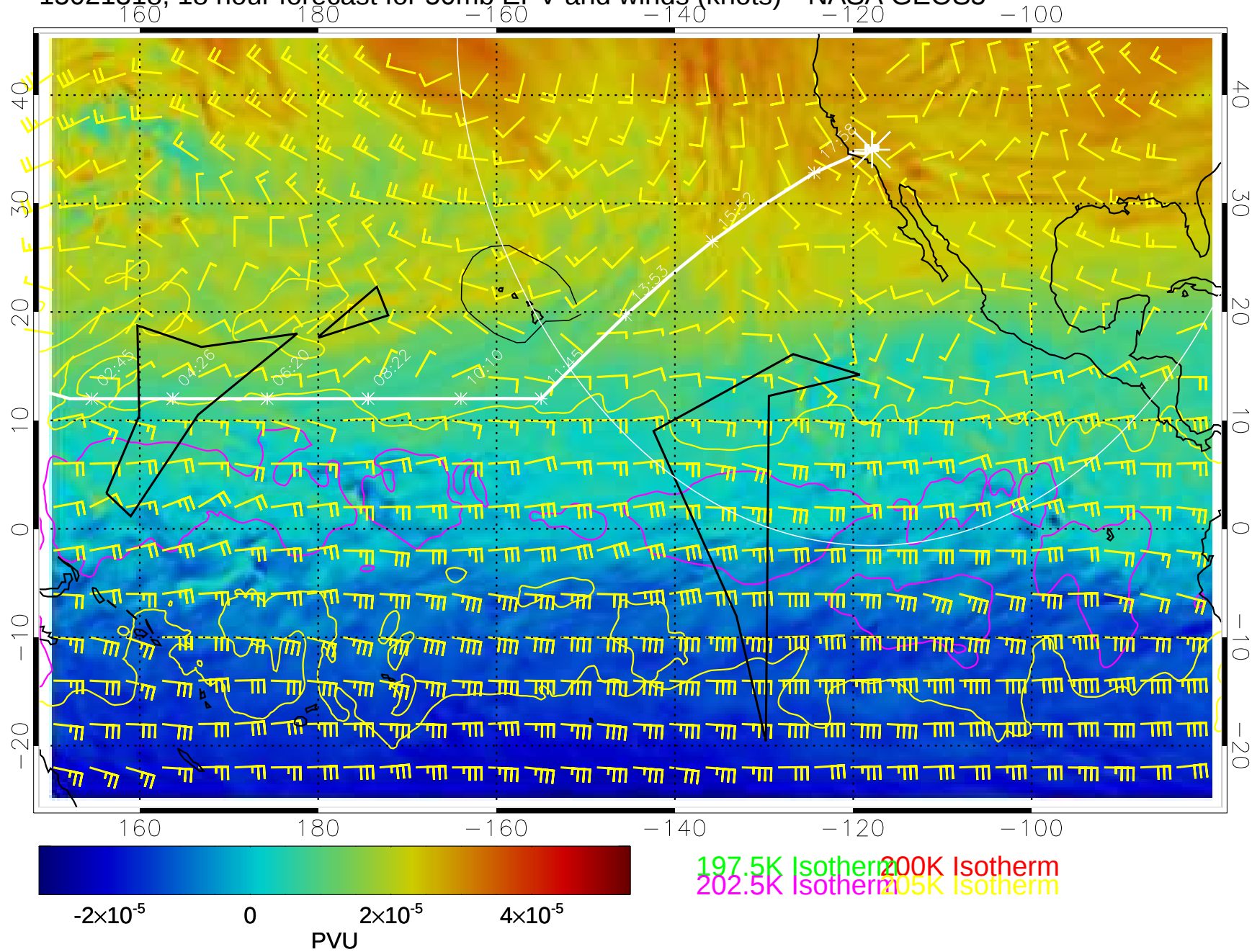
15021318, 18 hour forecast for 50mb EPV and winds (knots)-- NASA GEOS5
