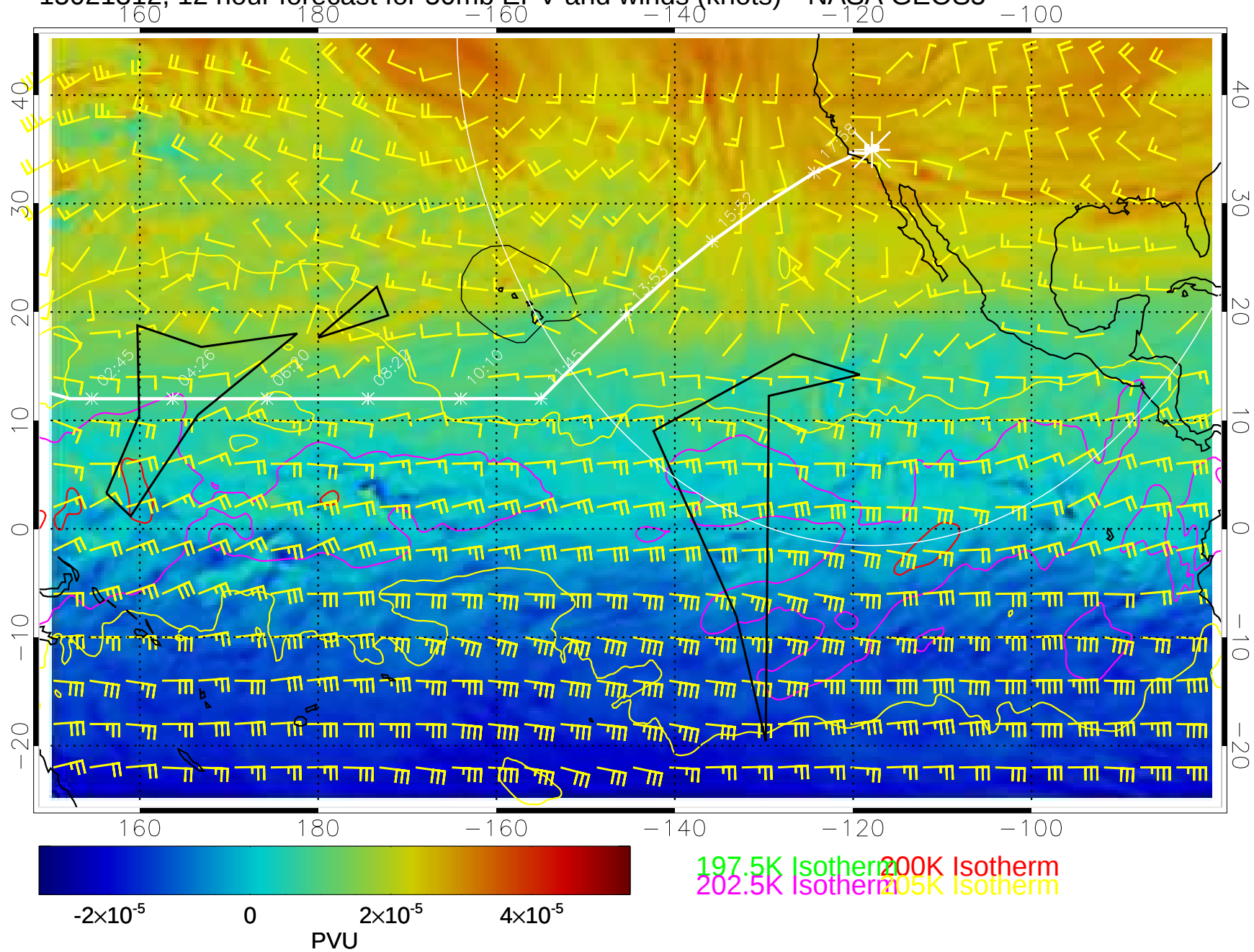
15021312, 12 hour forecast for 50mb EPV and winds (knots)-- NASA GEOS5
