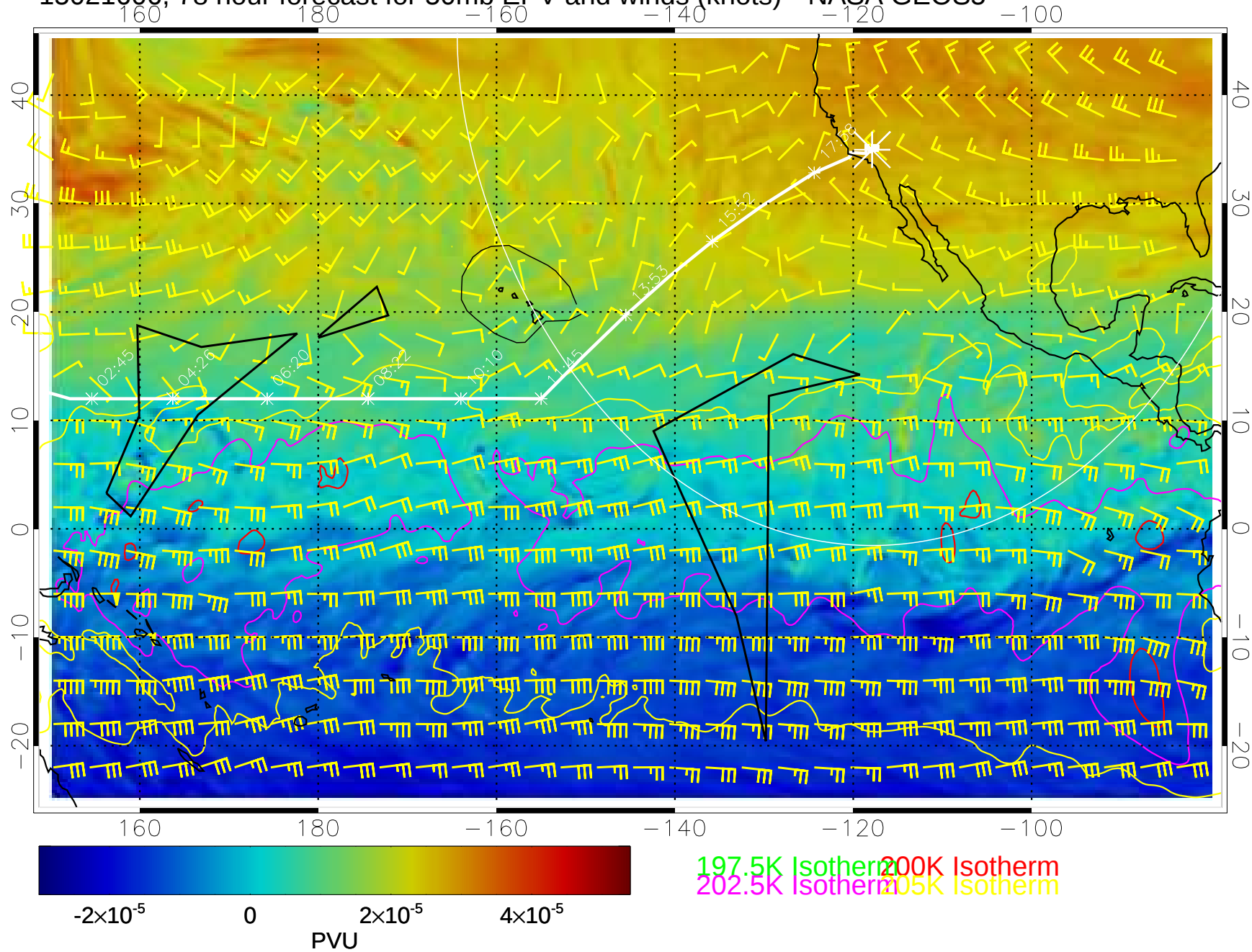
15021606, 78 hour forecast for 50mb EPV and winds (knots)-- NASA GEOS5
