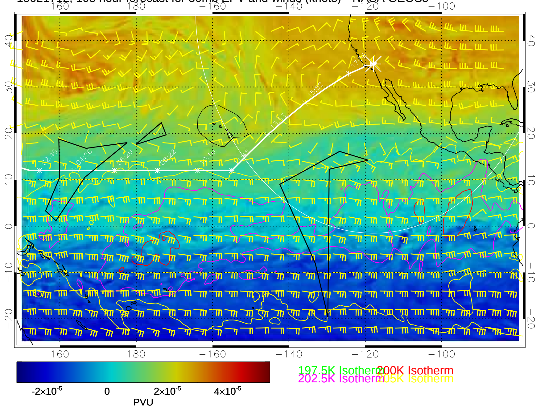
15021712, 108 hour forecast for 50mb EPV and winds (knots)-- NASA GEOS5
