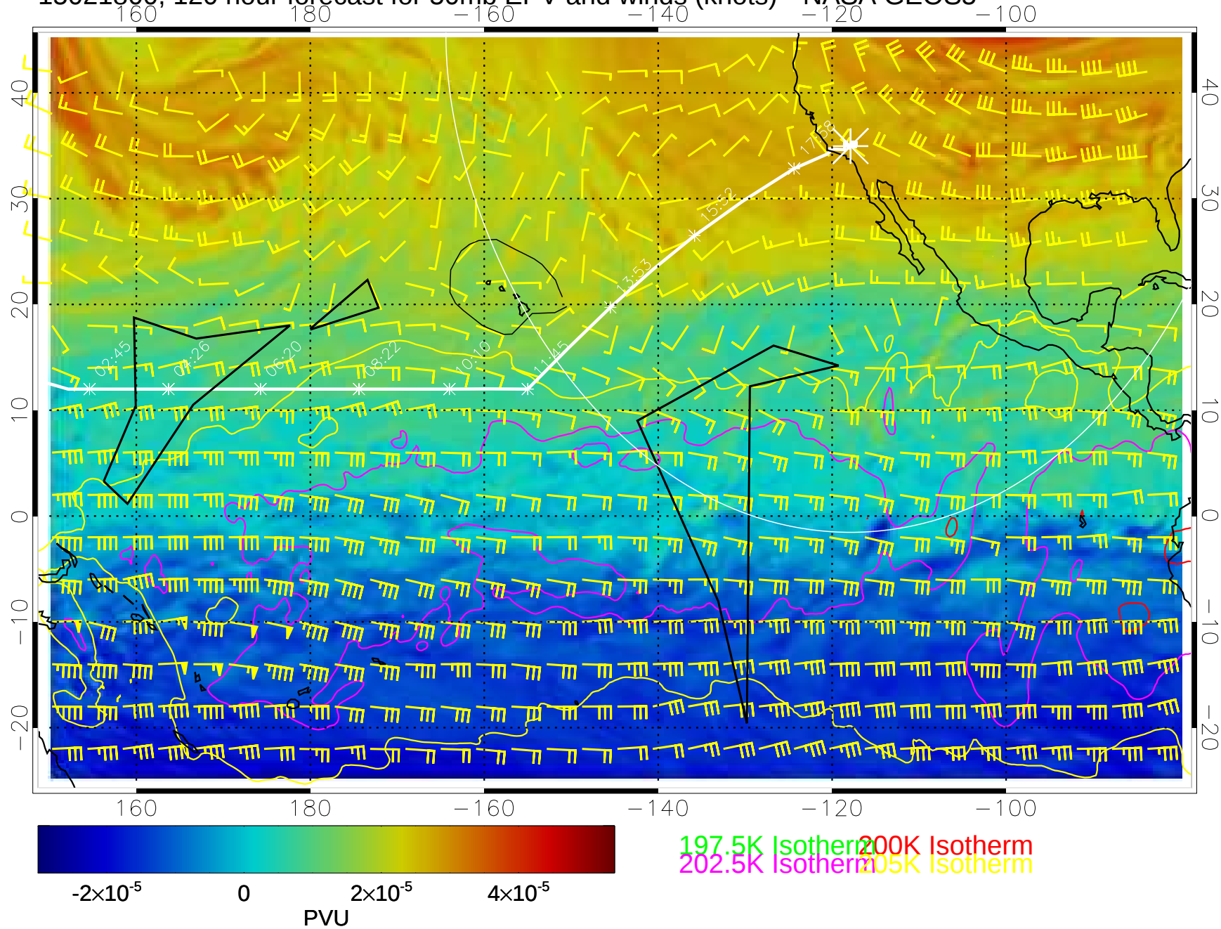
15021800, 120 hour forecast for 50mb EPV and winds (knots)-- NASA GEOS5
