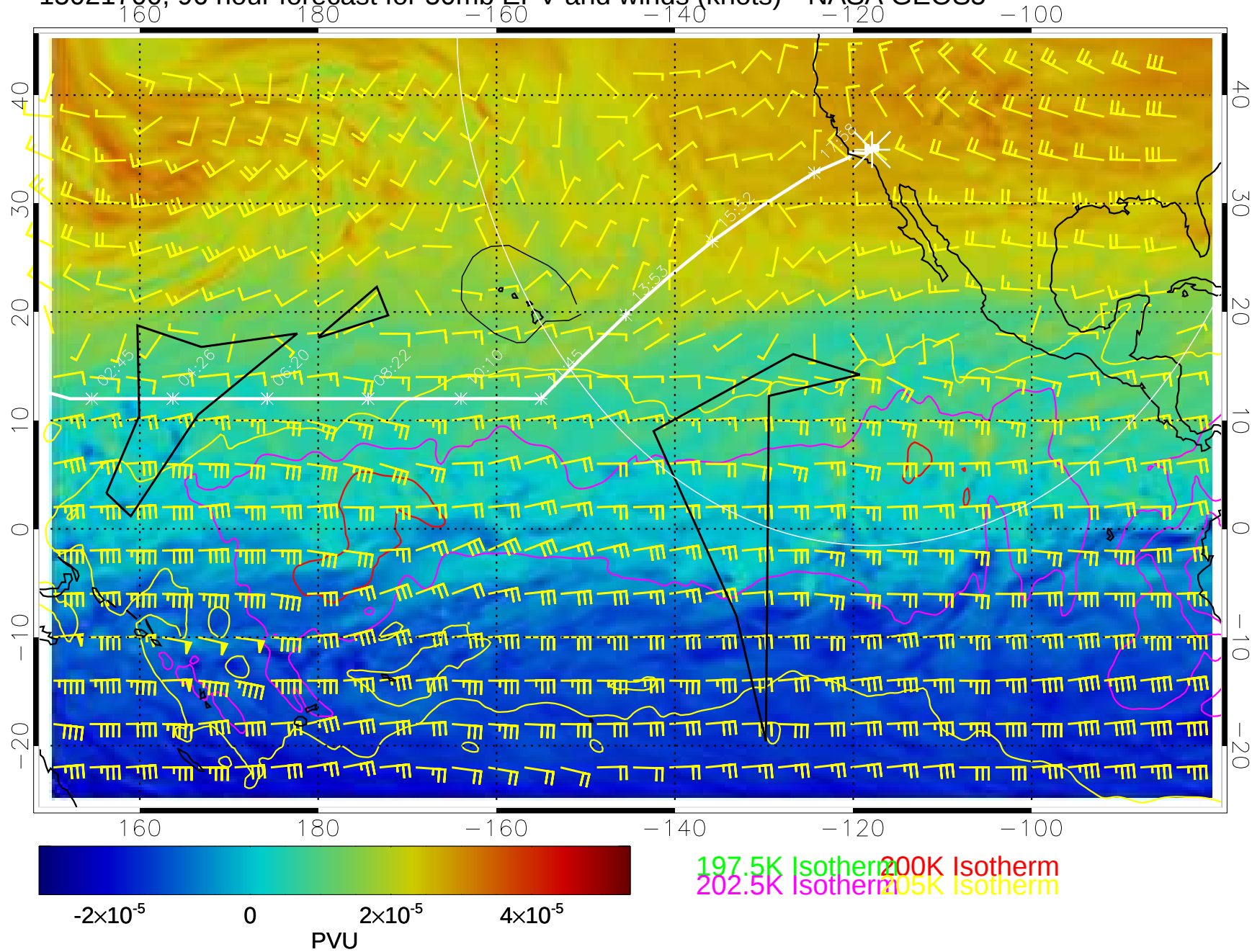
15021700, 96 hour forecast for 50mb EPV and winds (knots)-- NASA GEOS5
