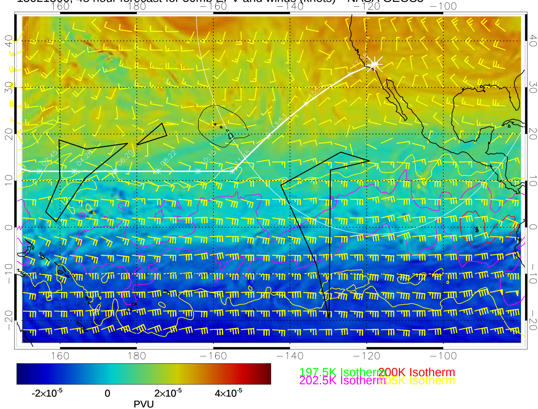
15021500, 48 hour forecast for 50mb EPV and winds (knots)-- NASA GEOS5
