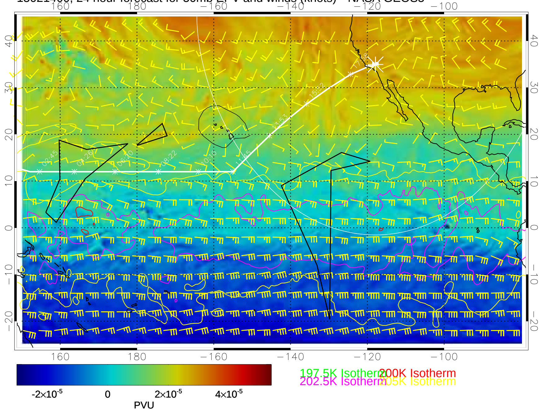
15021400, 24 hour forecast for 50mb EPV and winds (knots)-- NASA GEOS5
