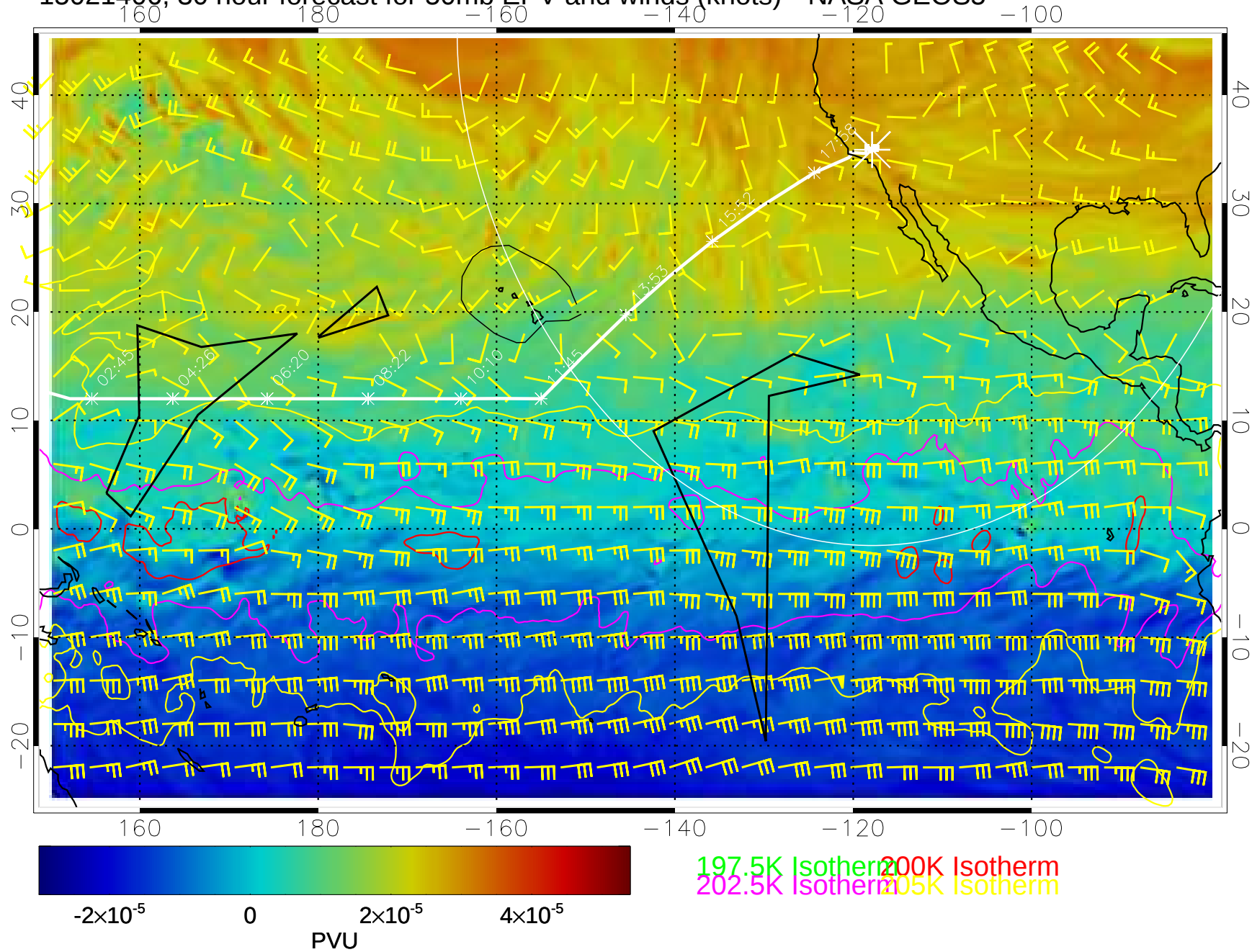
15021406, 30 hour forecast for 50mb EPV and winds (knots)-- NASA GEOS5
