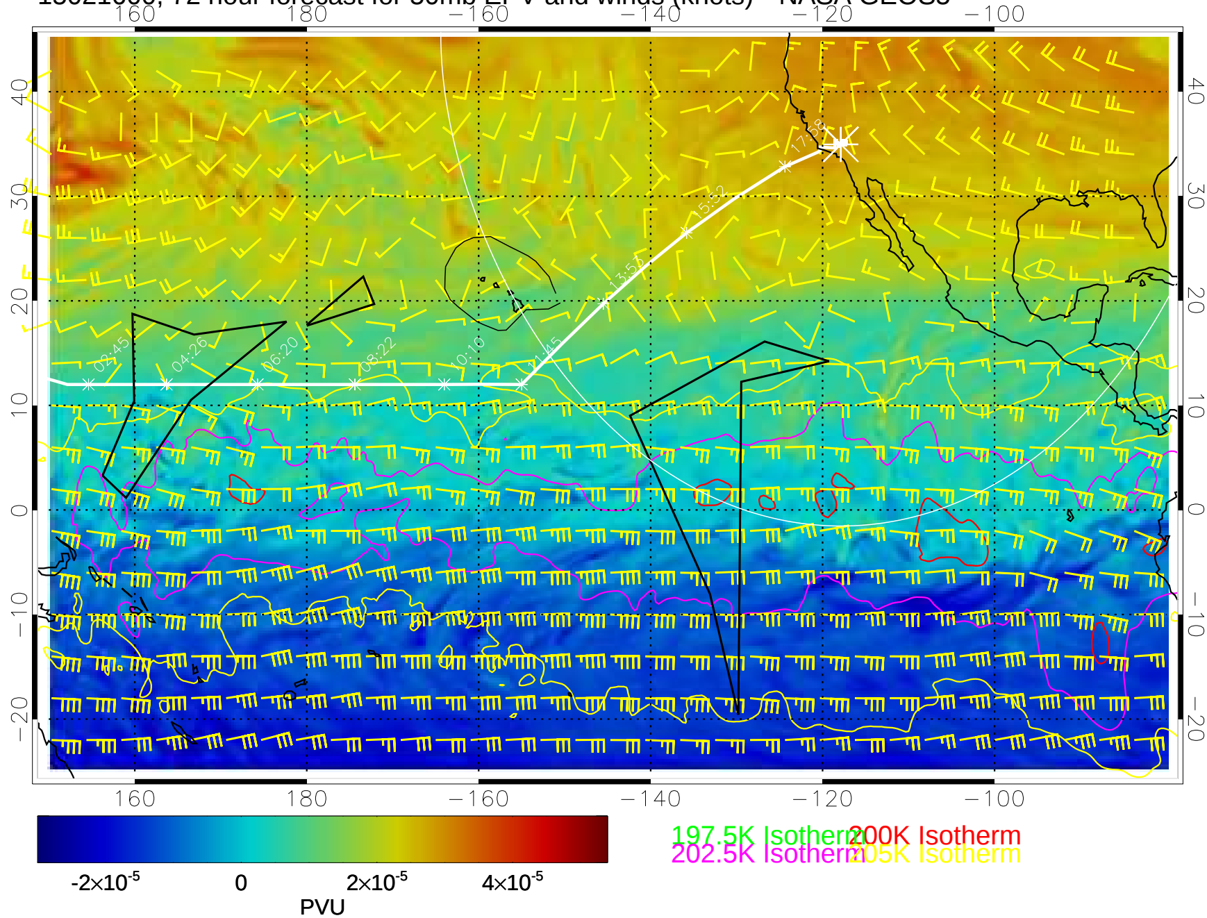
15021600, 72 hour forecast for 50mb EPV and winds (knots)-- NASA GEOS5
