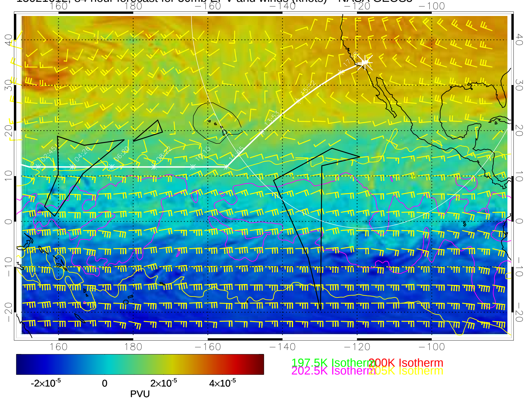
15021612, 84 hour forecast for 50mb EPV and winds (knots)-- NASA GEOS5
