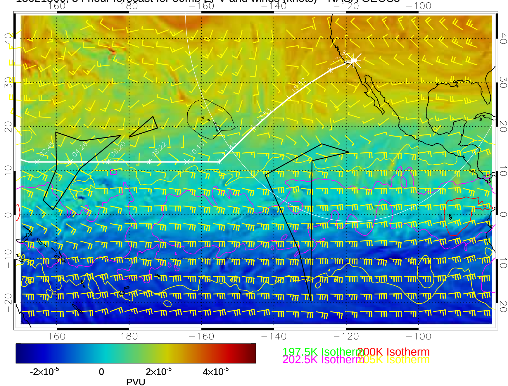
15021506, 54 hour forecast for 50mb EPV and winds (knots)-- NASA GEOS5
