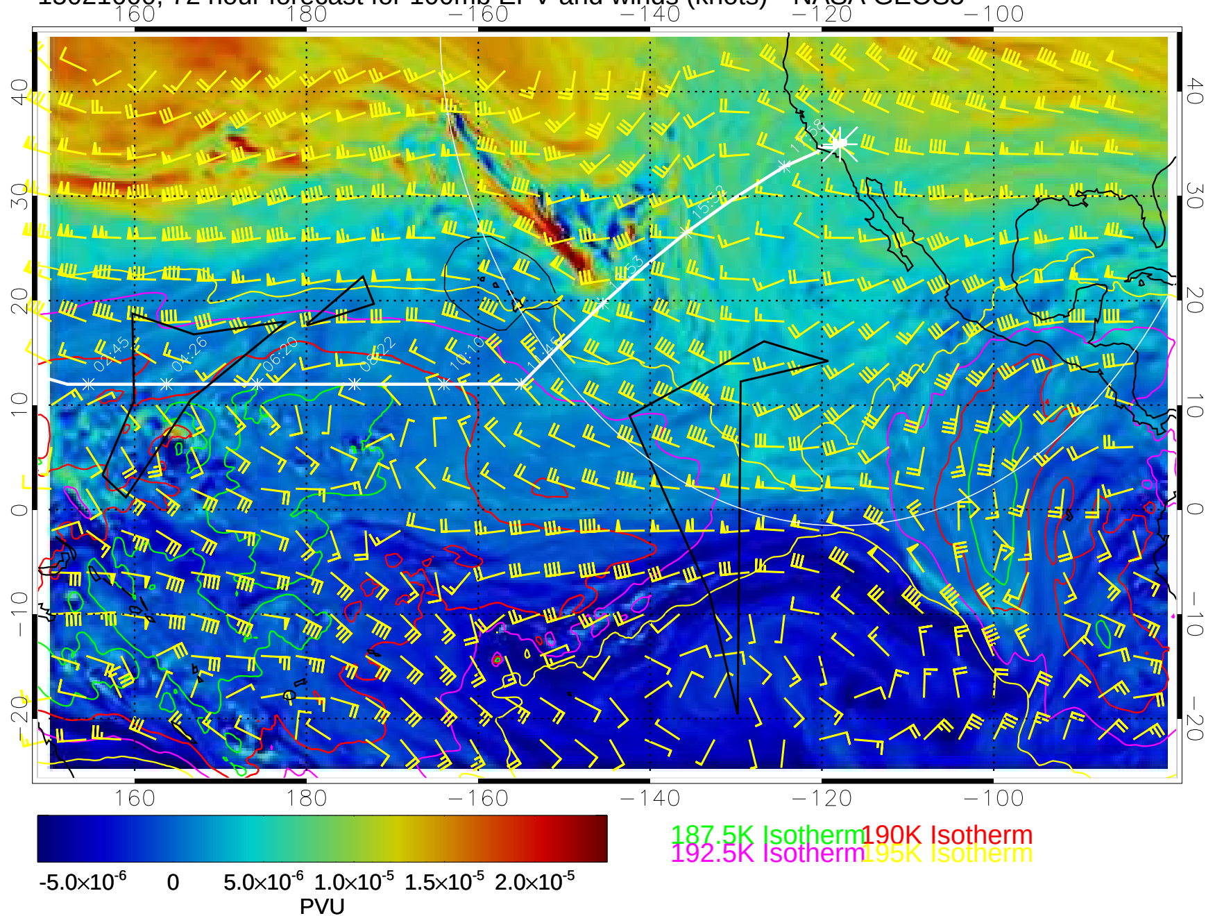
15021600, 72 hour forecast for 100mb EPV and winds (knots)-- NASA GEOS5
