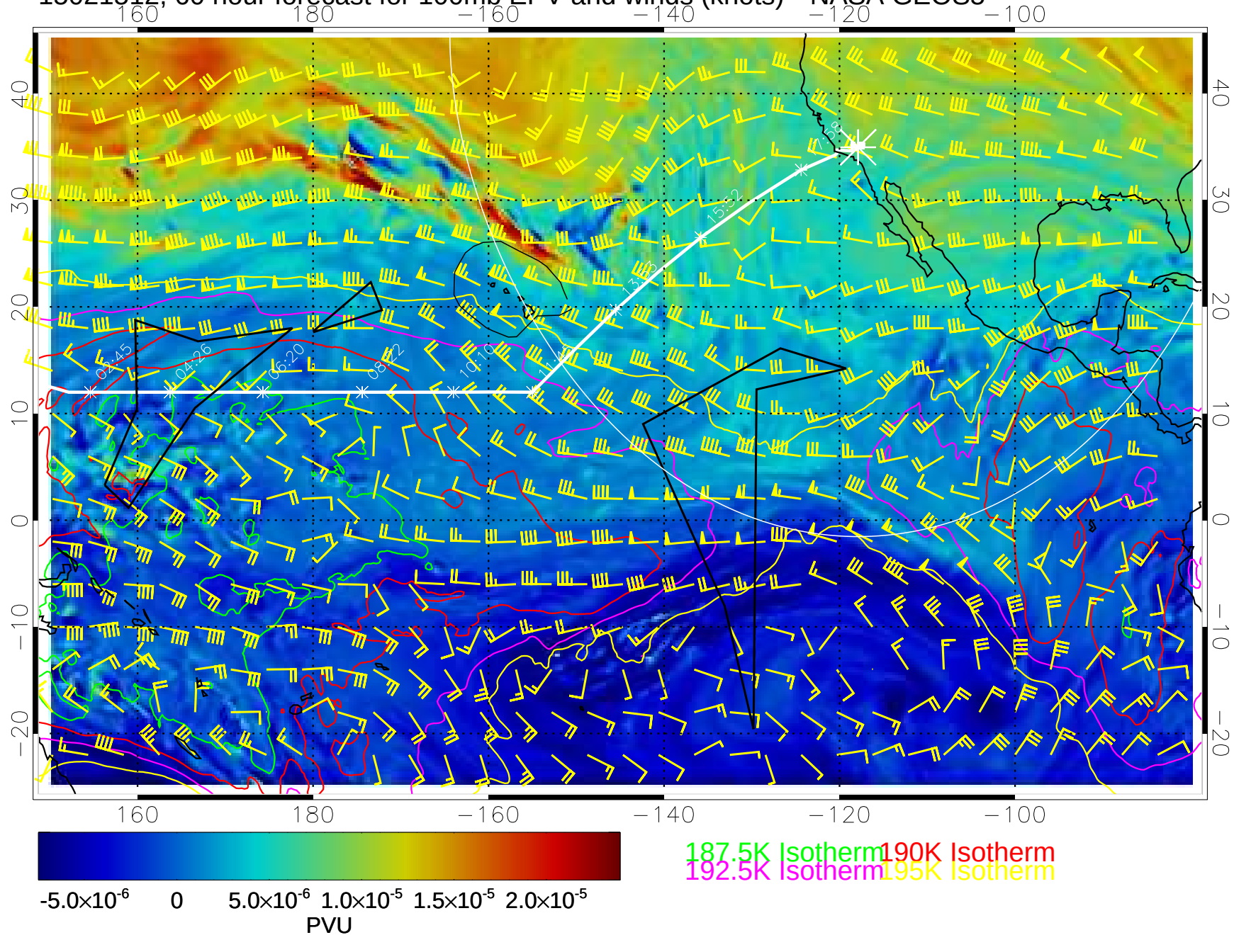
15021512, 60 hour forecast for 100mb EPV and winds (knots)-- NASA GEOS5
