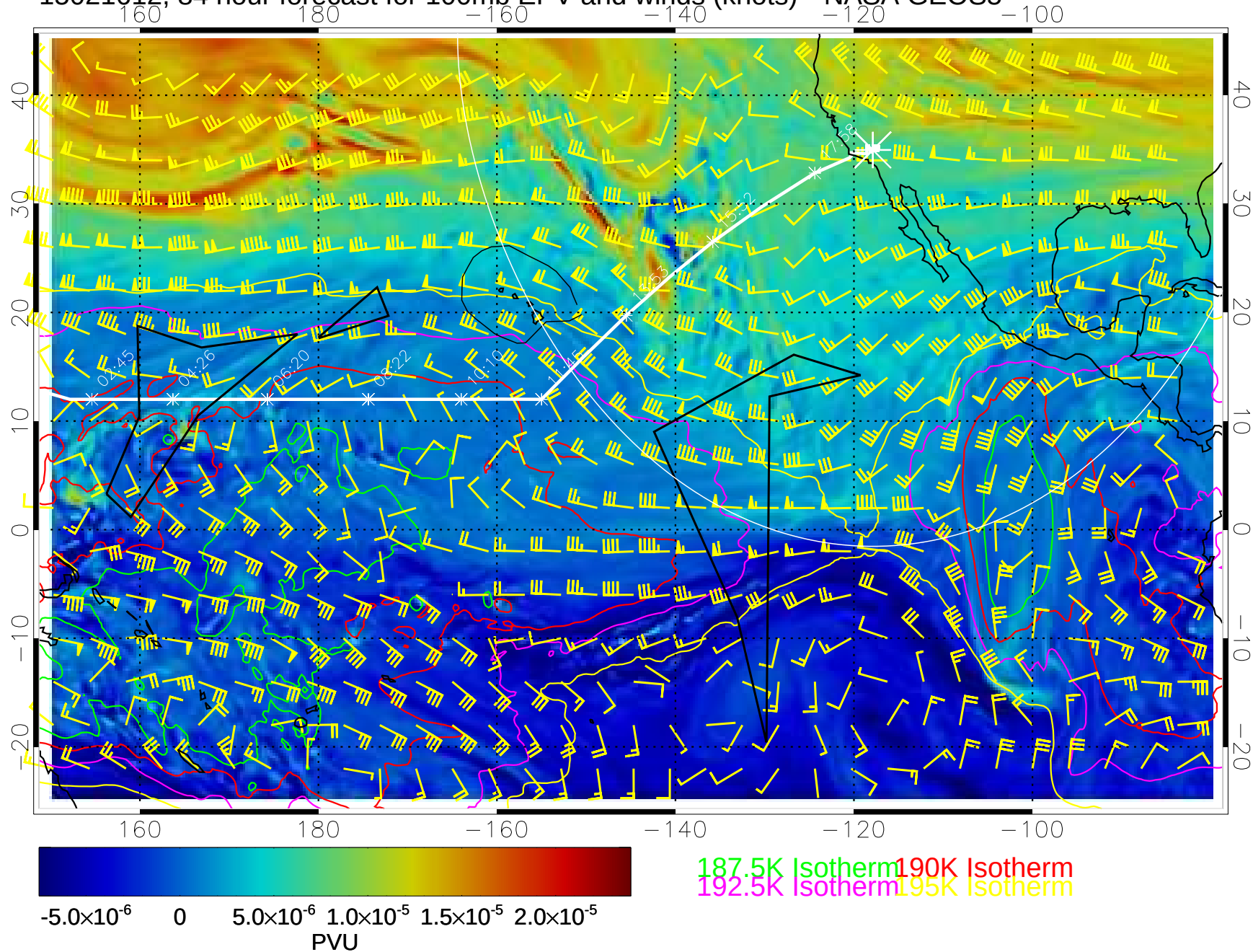
15021612, 84 hour forecast for 100mb EPV and winds (knots)-- NASA GEOS5
