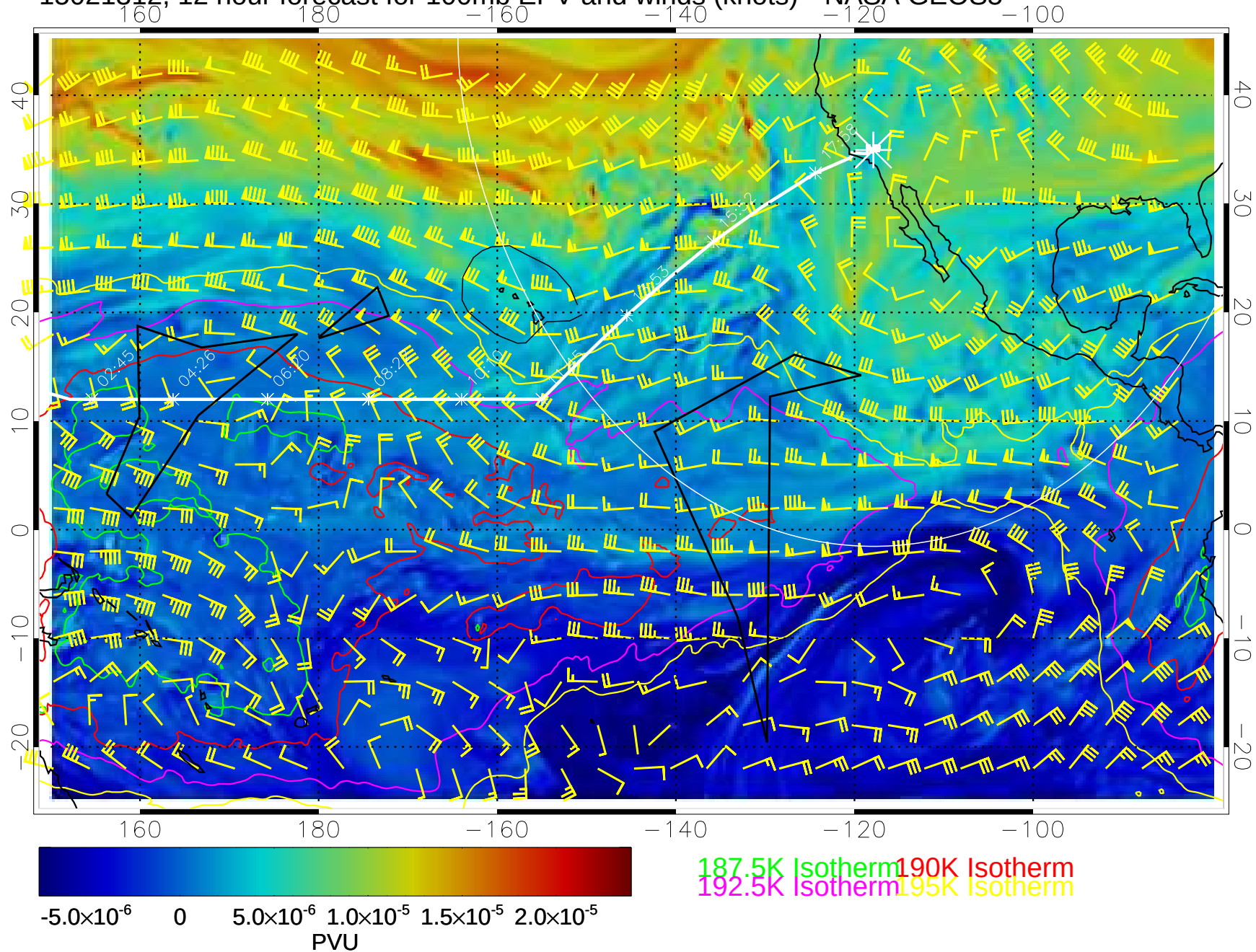
15021312, 12 hour forecast for 100mb EPV and winds (knots)-- NASA GEOS5
