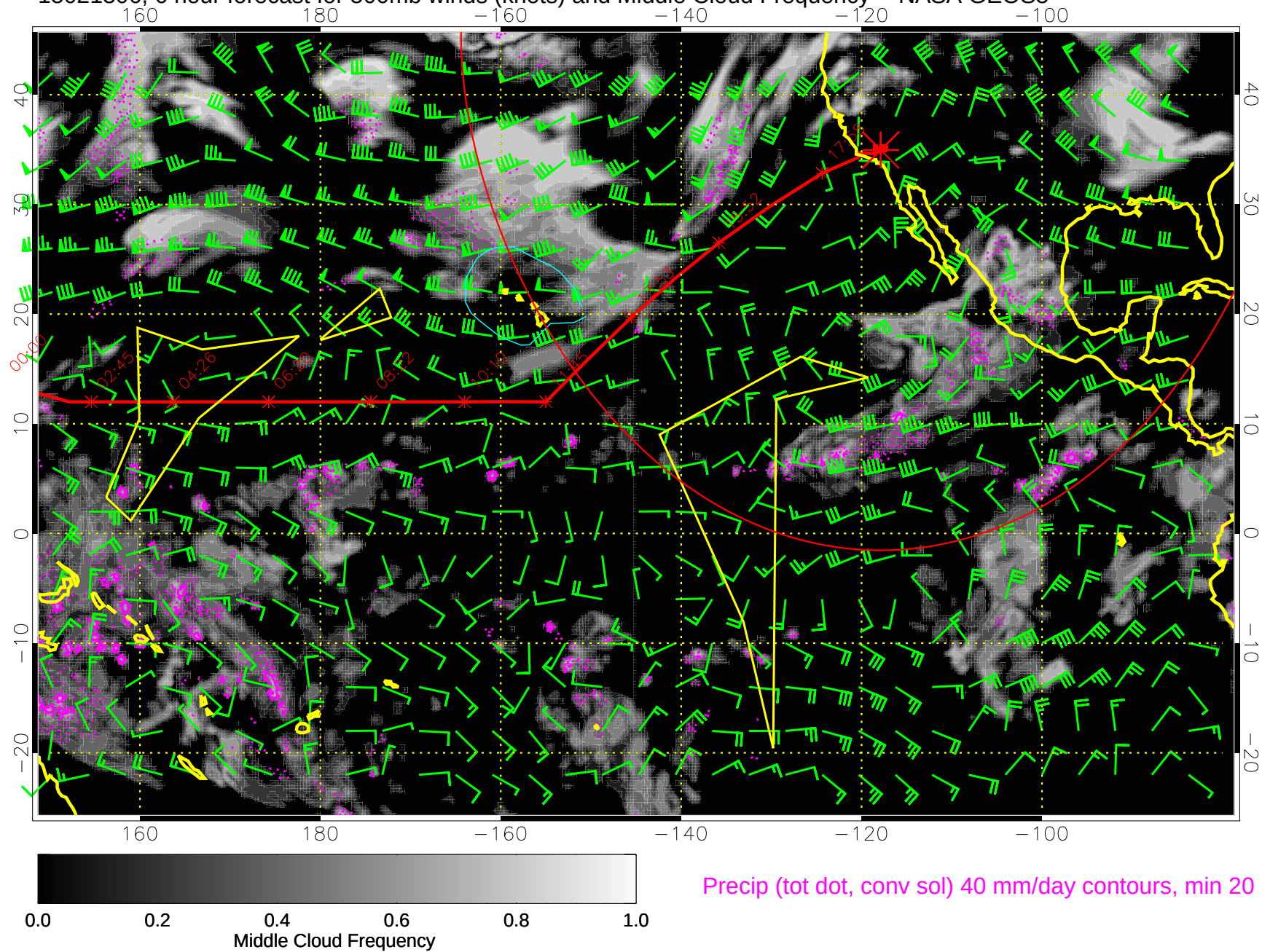
15021306, 6 hour forecast for 500mb winds (knots) and Middle Cloud Frequency -- NASA GEOS5
