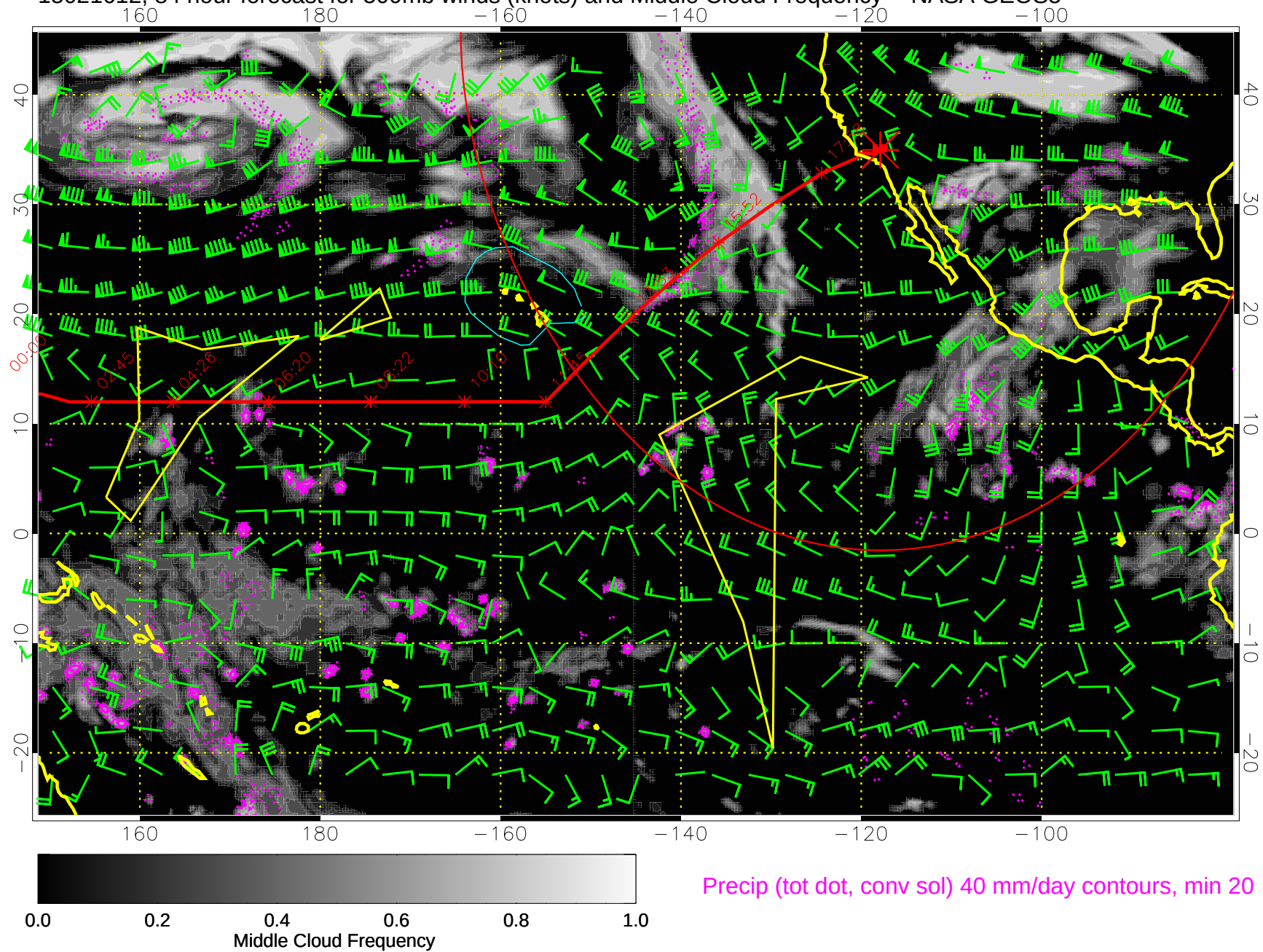
15021612, 84 hour forecast for 500mb winds (knots) and Middle Cloud Frequency -- NASA GEOS5
