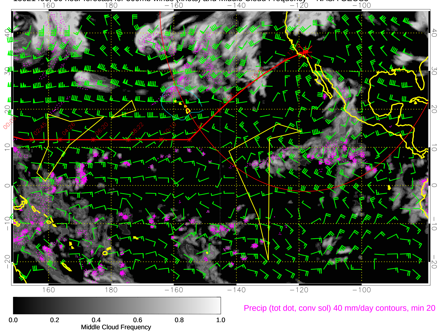
15021406, 30 hour forecast for 500mb winds (knots) and Middle Cloud Frequency -- NASA GEOS5
