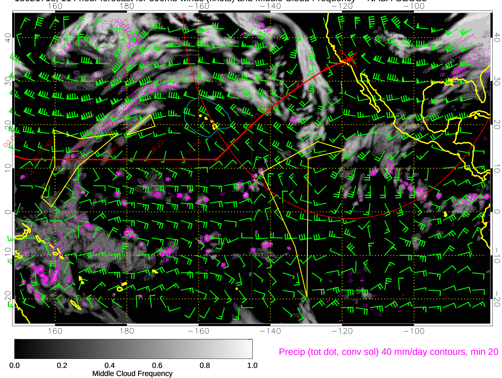
15021718, 114 hour forecast for 500mb winds (knots) and Middle Cloud Frequency -- NASA GEOS5
