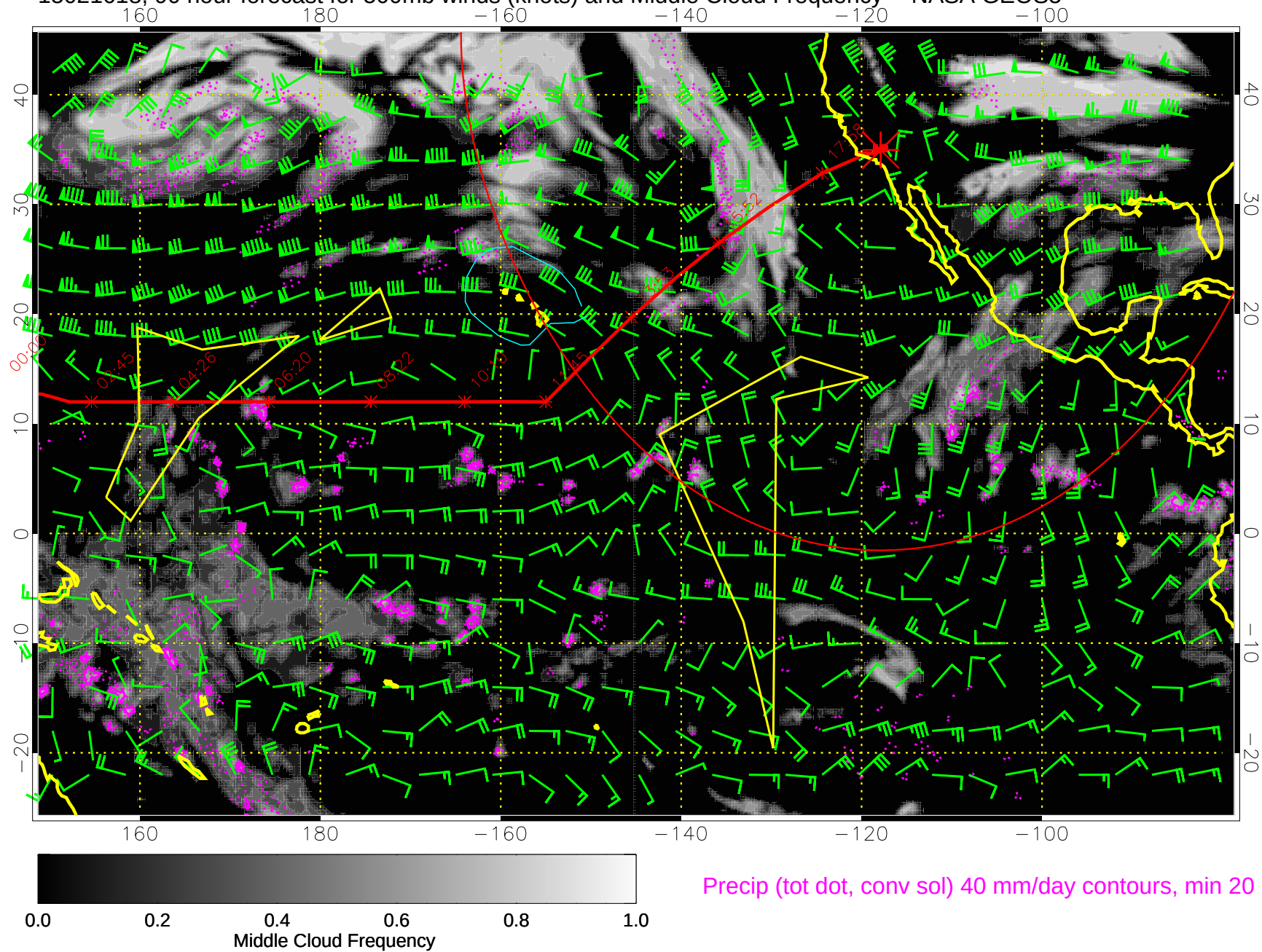
15021618, 90 hour forecast for 500mb winds (knots) and Middle Cloud Frequency -- NASA GEOS5
