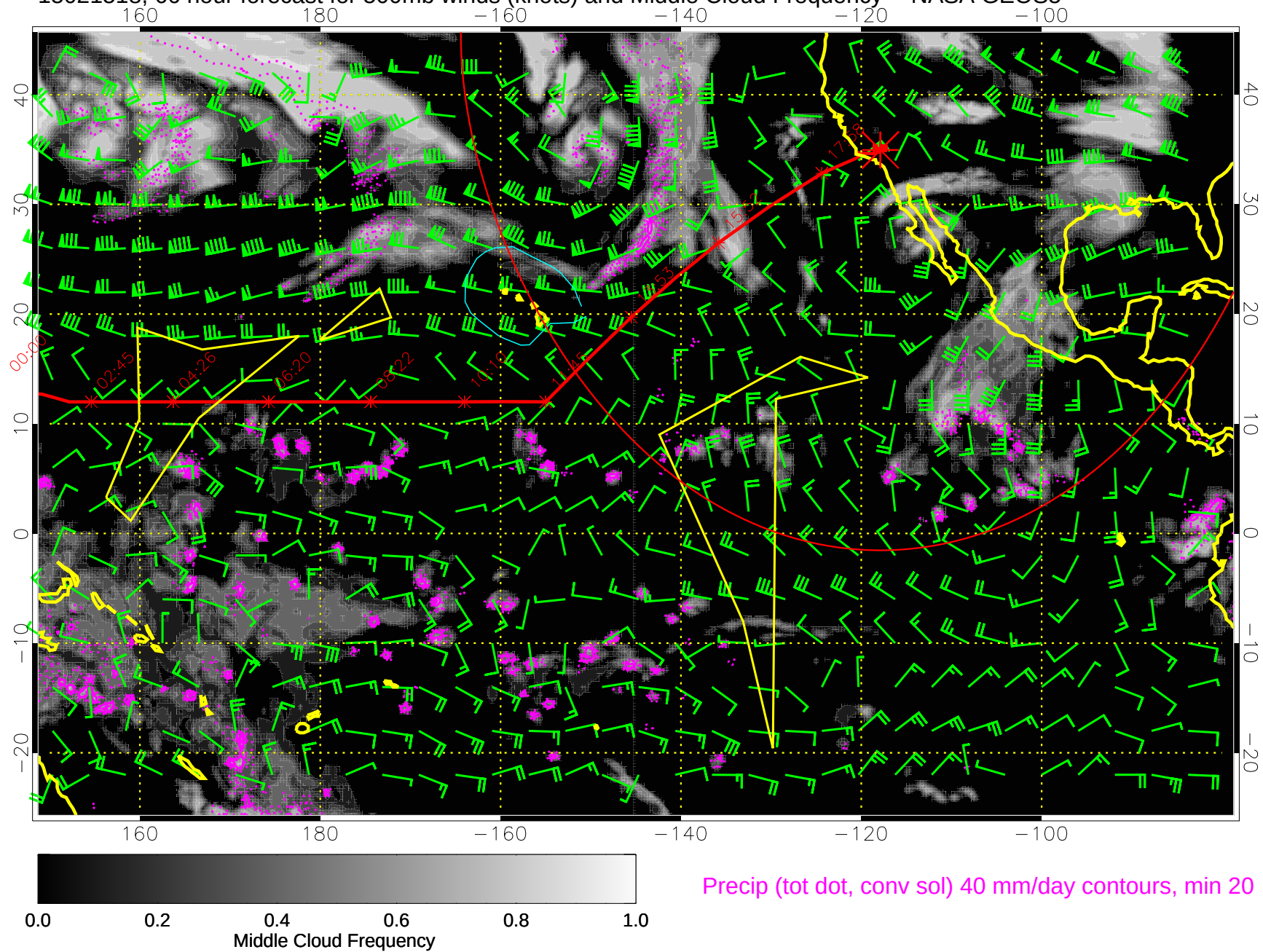
15021518, 66 hour forecast for 500mb winds (knots) and Middle Cloud Frequency -- NASA GEOS5
