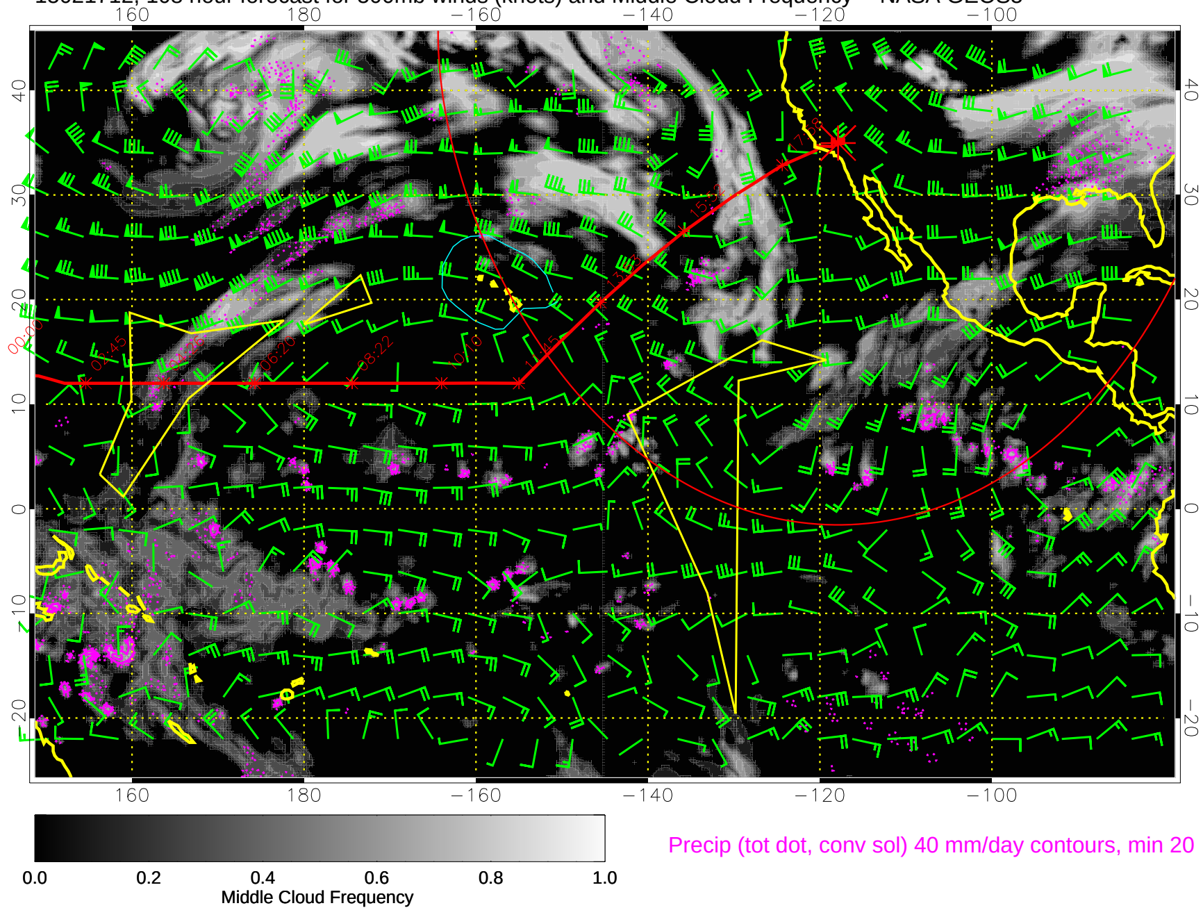
15021712, 108 hour forecast for 500mb winds (knots) and Middle Cloud Frequency -- NASA GEOS5
