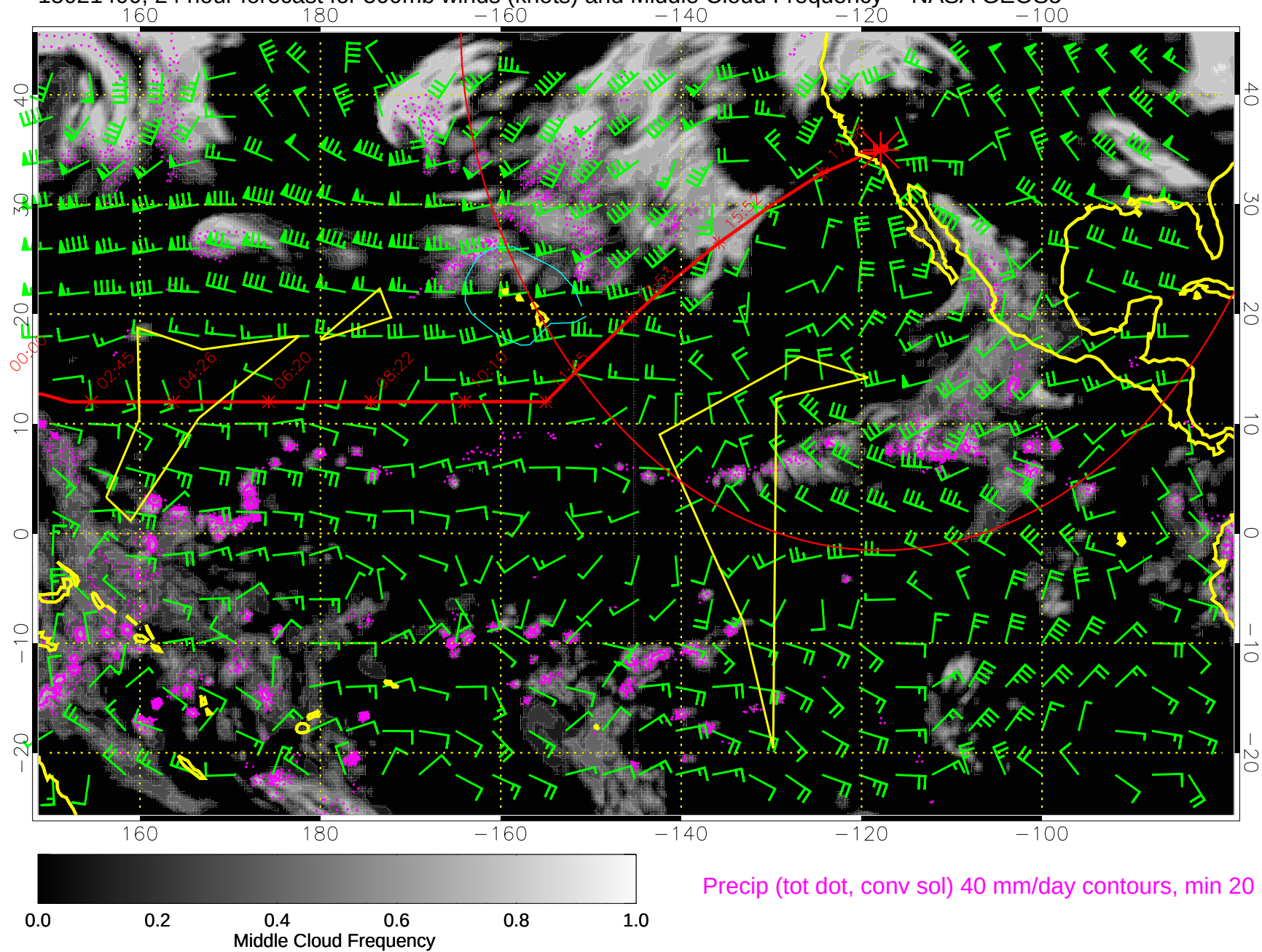
15021400, 24 hour forecast for 500mb winds (knots) and Middle Cloud Frequency -- NASA GEOS5
