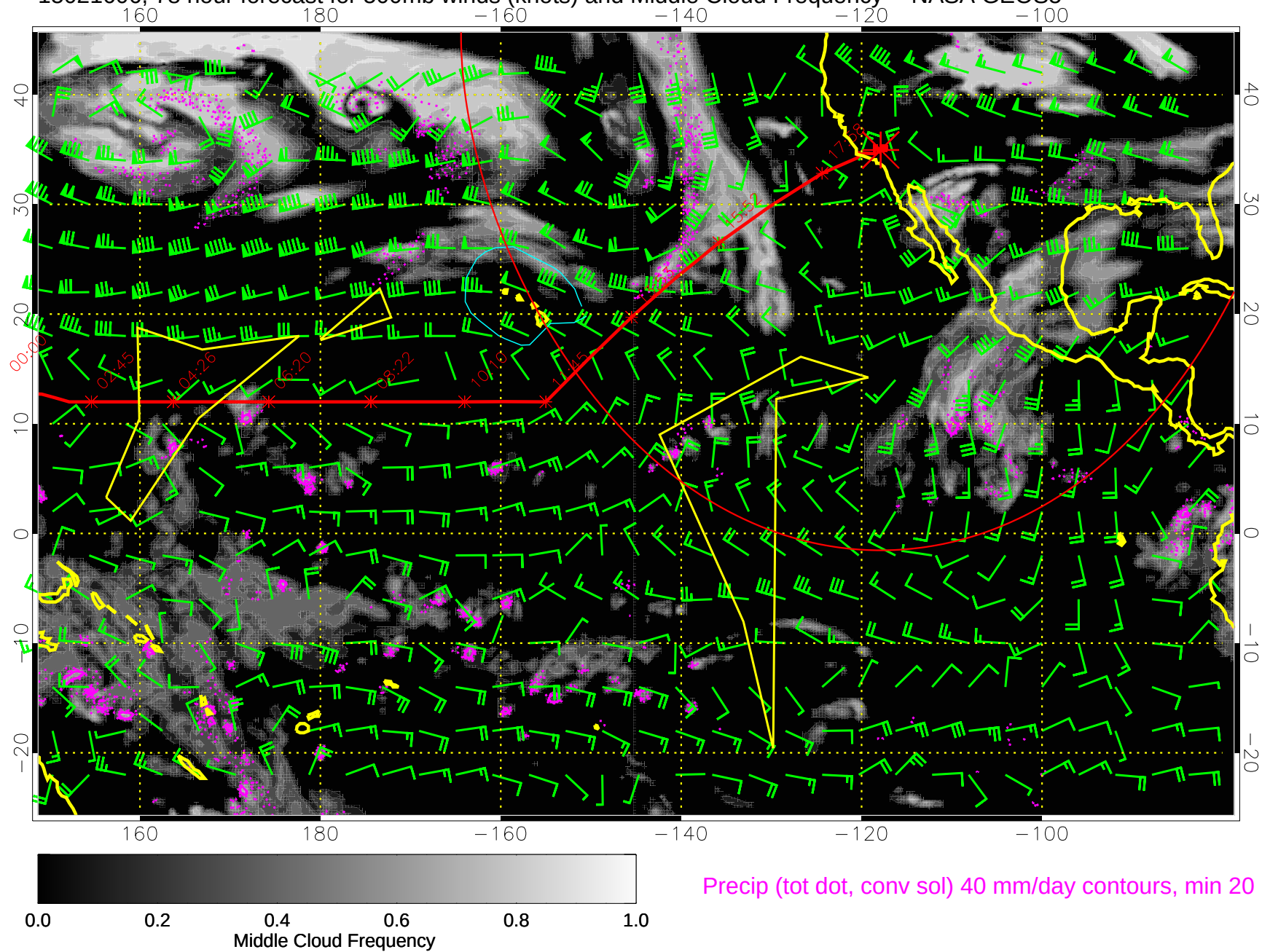
15021606, 78 hour forecast for 500mb winds (knots) and Middle Cloud Frequency -- NASA GEOS5
