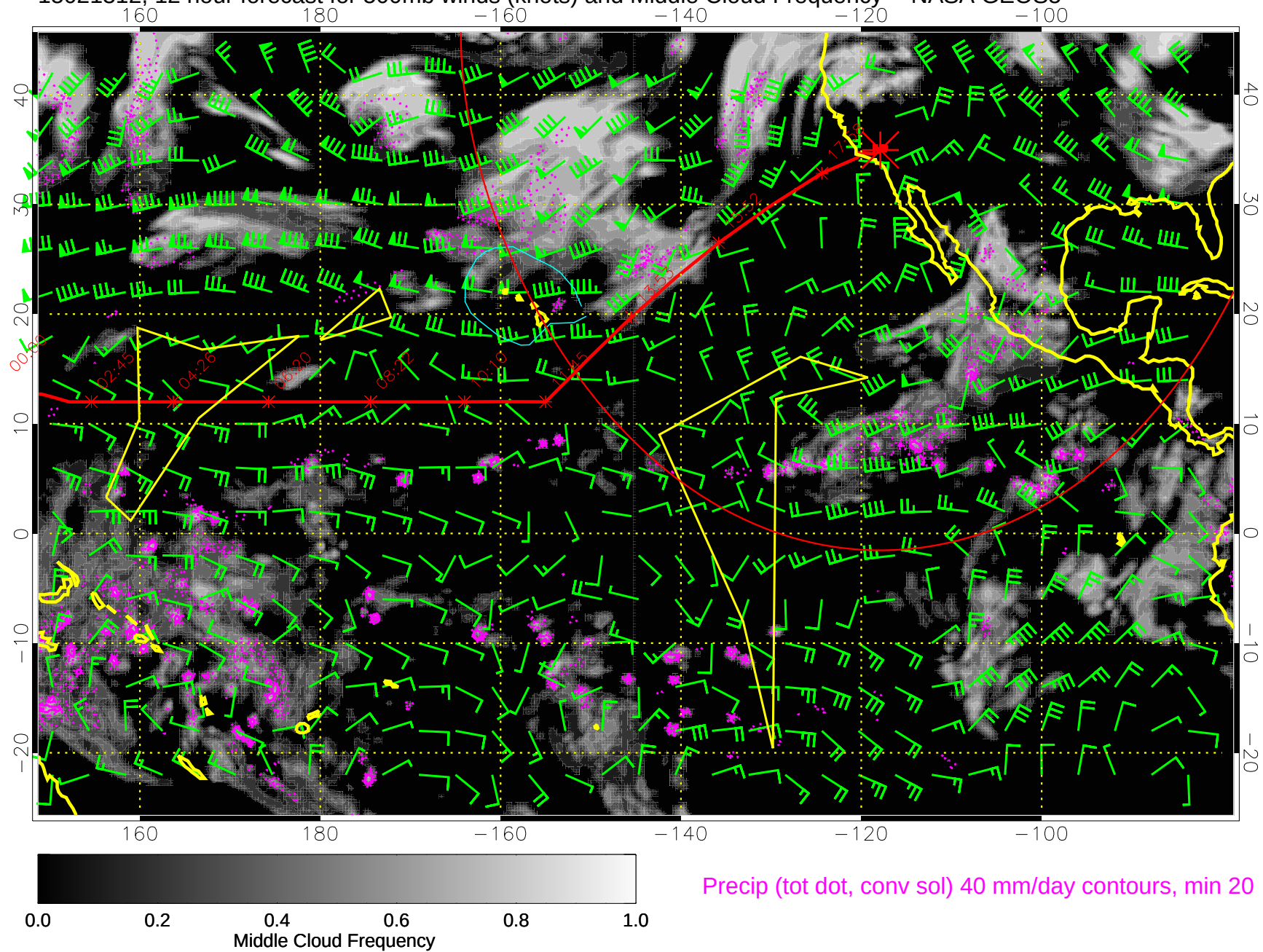
15021312, 12 hour forecast for 500mb winds (knots) and Middle Cloud Frequency -- NASA GEOS5
