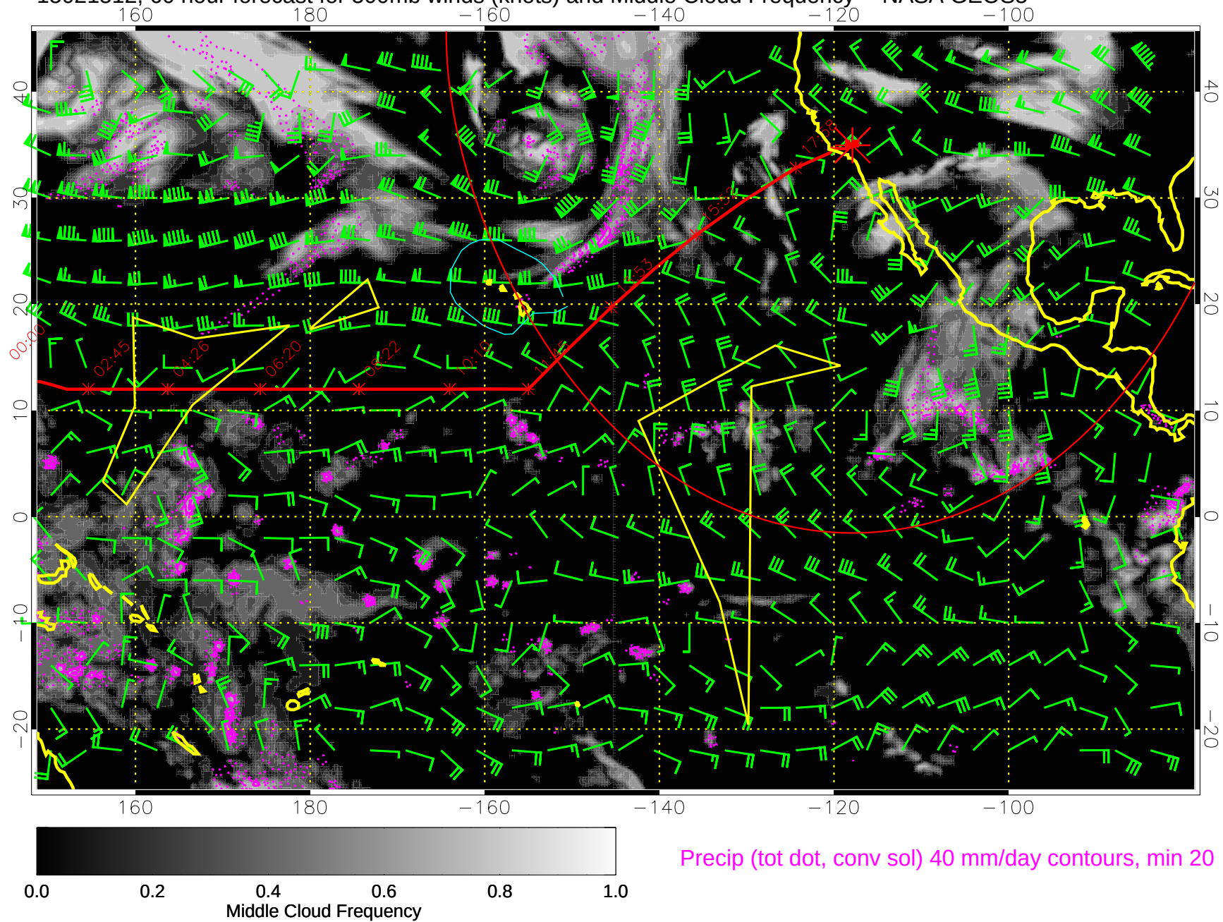
15021512, 60 hour forecast for 500mb winds (knots) and Middle Cloud Frequency -- NASA GEOS5
