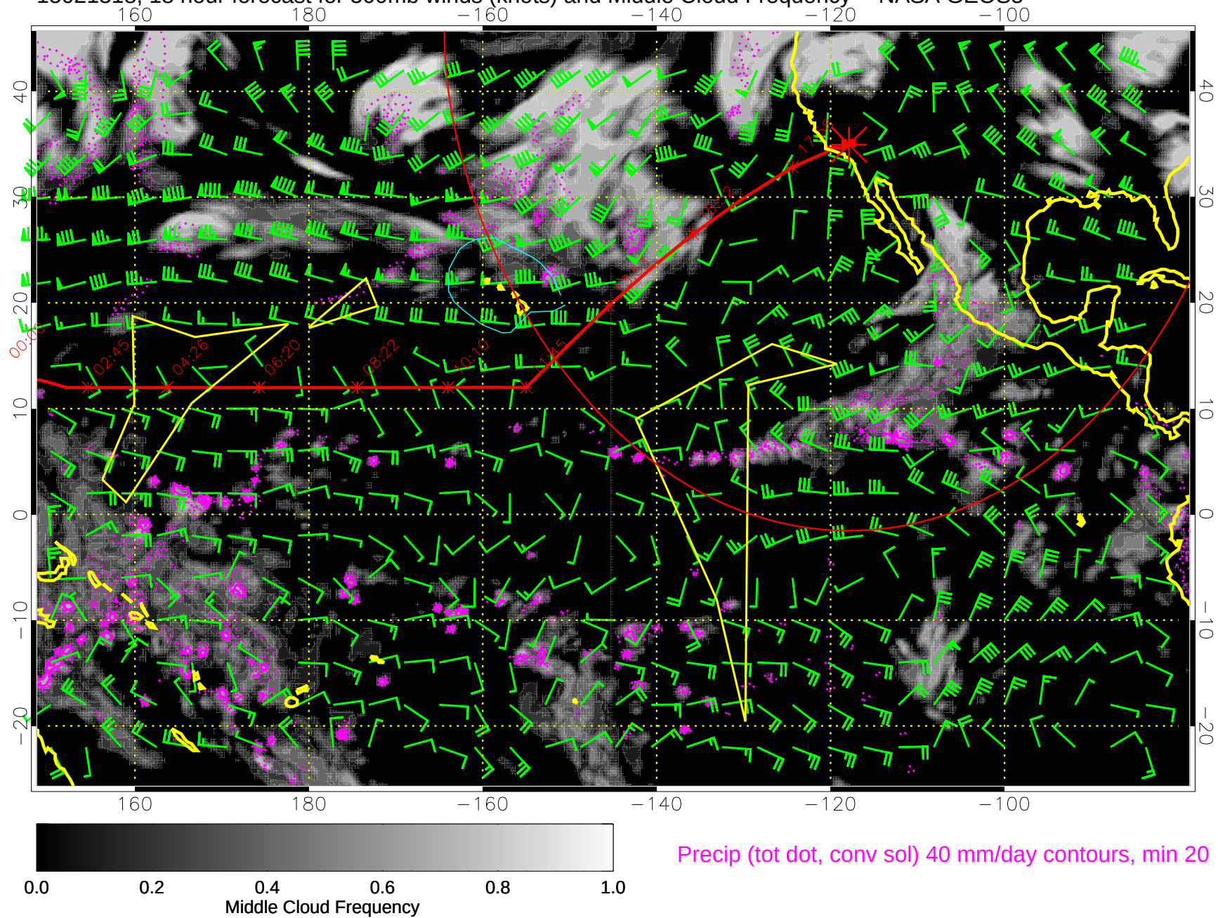
15021318, 18 hour forecast for 500mb winds (knots) and Middle Cloud Frequency -- NASA GEOS5
