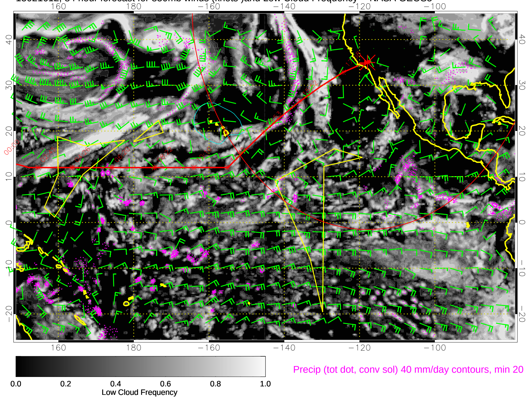
15021612, 84 hour forecast for 850mb winds (knots) and Low Cloud Frequency -- NASA GEOS5
