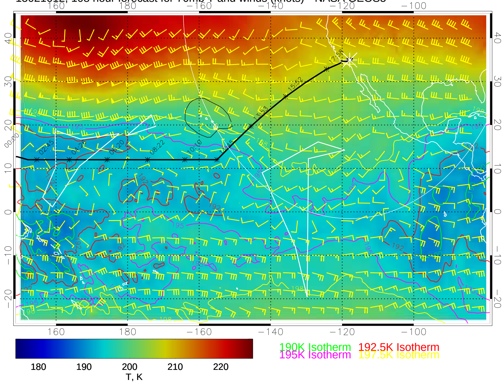
15021612, 108 hour forecast for 70mb T and winds (knots)-- NASA GEOS5
