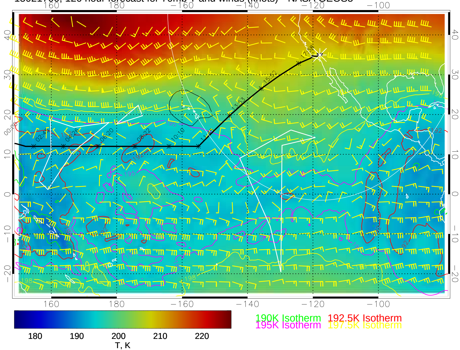
15021700, 120 hour forecast for 70mb T and winds (knots)-- NASA GEOS5
