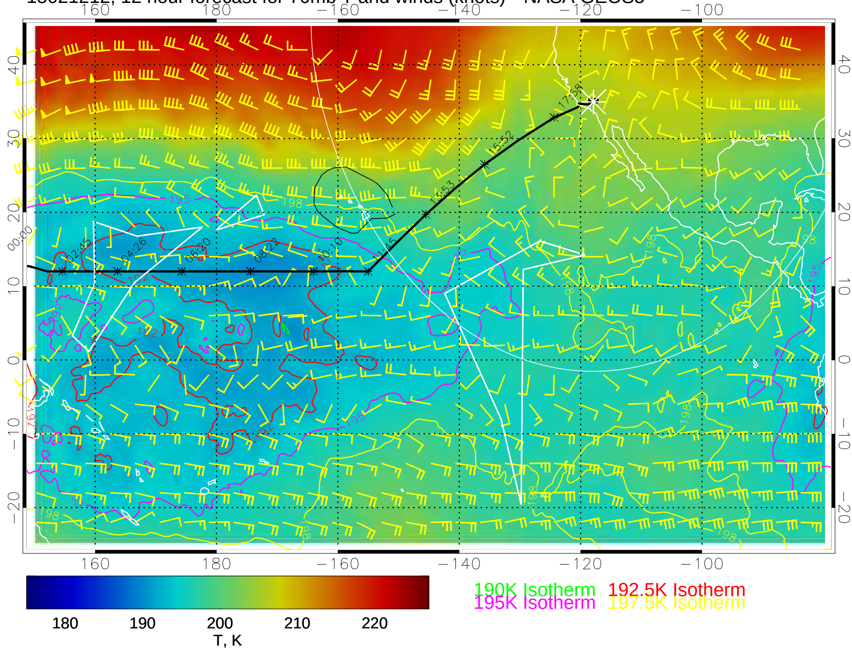
15021212, 12 hour forecast for 70mb T and winds (knots)-- NASA GEOS5
