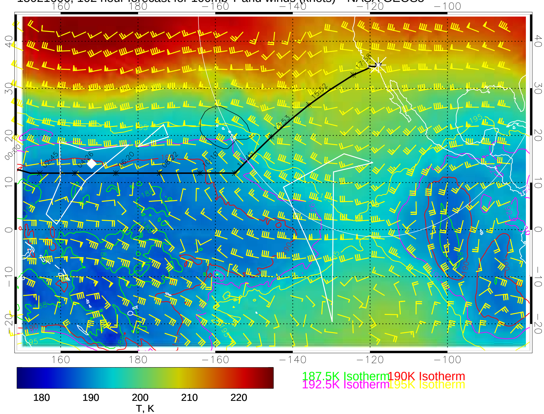
15021606, 102 hour forecast for 100mb T and winds (knots)-- NASA GEOS5
