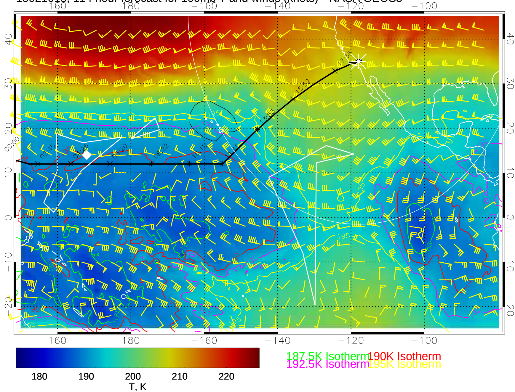
15021618, 114 hour forecast for 100mb T and winds (knots)-- NASA GEOS5
