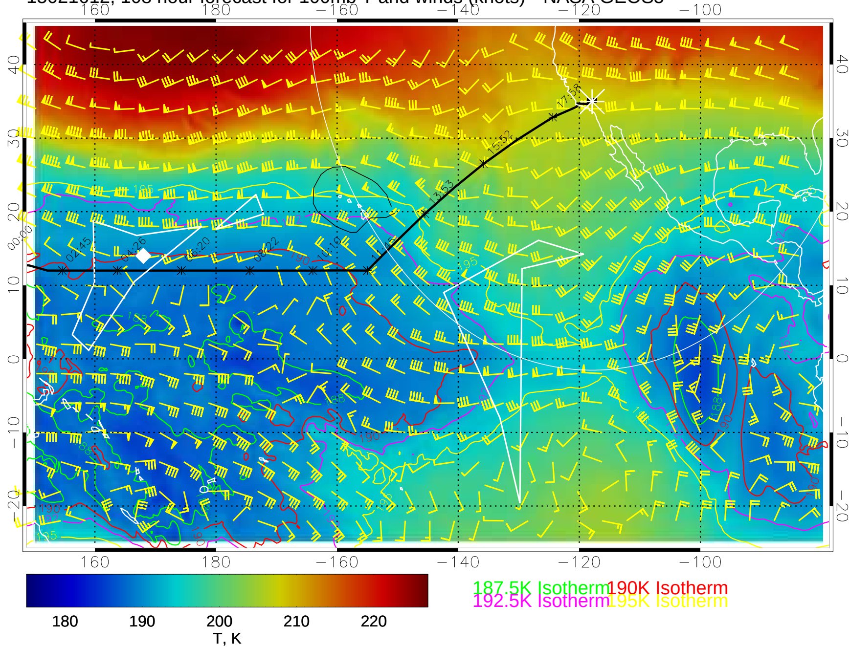
15021612, 108 hour forecast for 100mb T and winds (knots)-- NASA GEOS5
