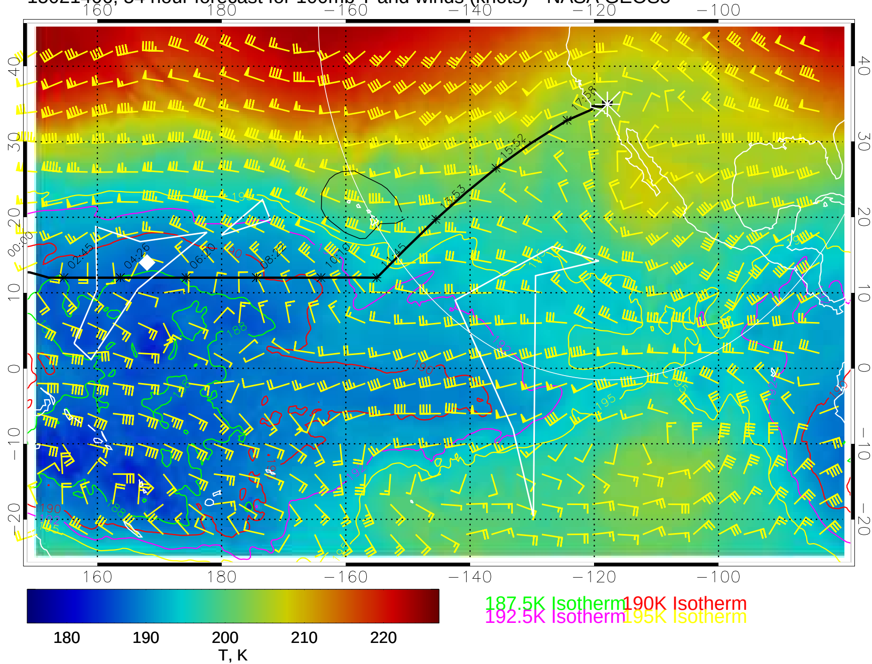
15021406, 54 hour forecast for 100mb T and winds (knots)-- NASA GEOS5
