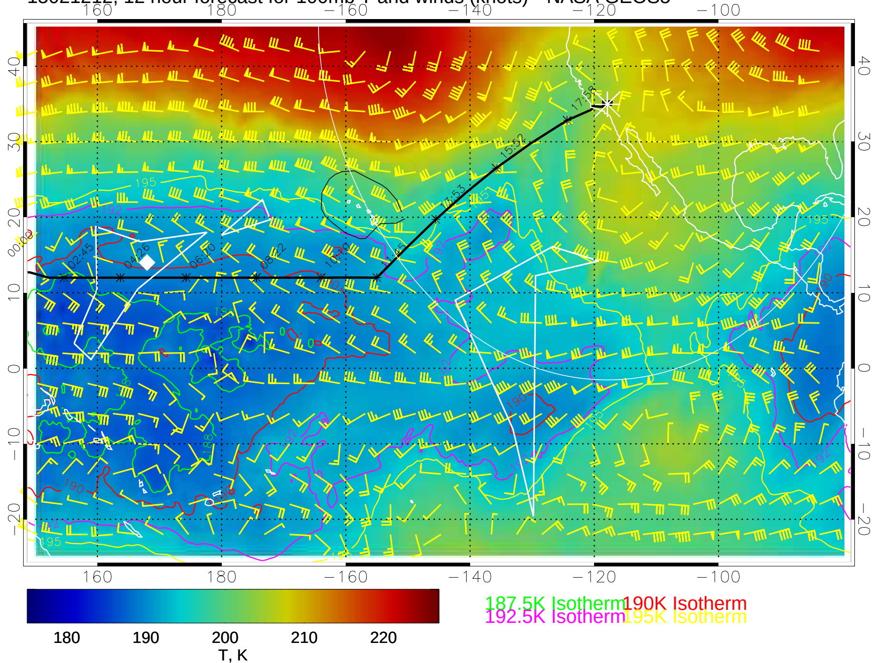
15021212, 12 hour forecast for 100mb T and winds (knots)-- NASA GEOS5
