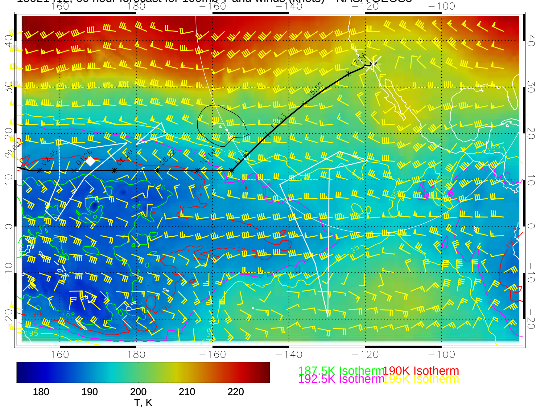
15021412, 60 hour forecast for 100mb T and winds (knots)-- NASA GEOS5
