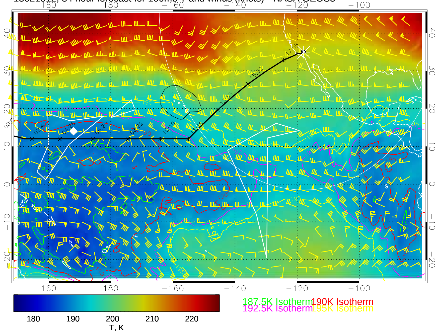
15021512, 84 hour forecast for 100mb T and winds (knots)-- NASA GEOS5
