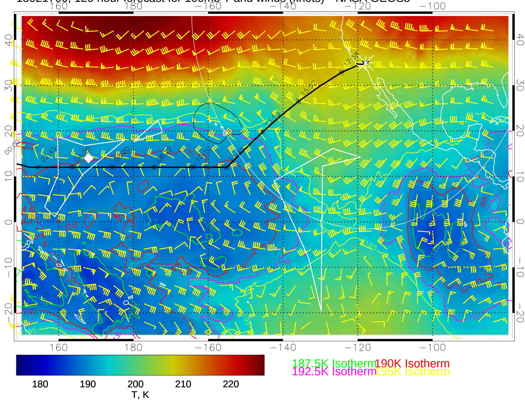
15021700, 120 hour forecast for 100mb T and winds (knots)-- NASA GEOS5
