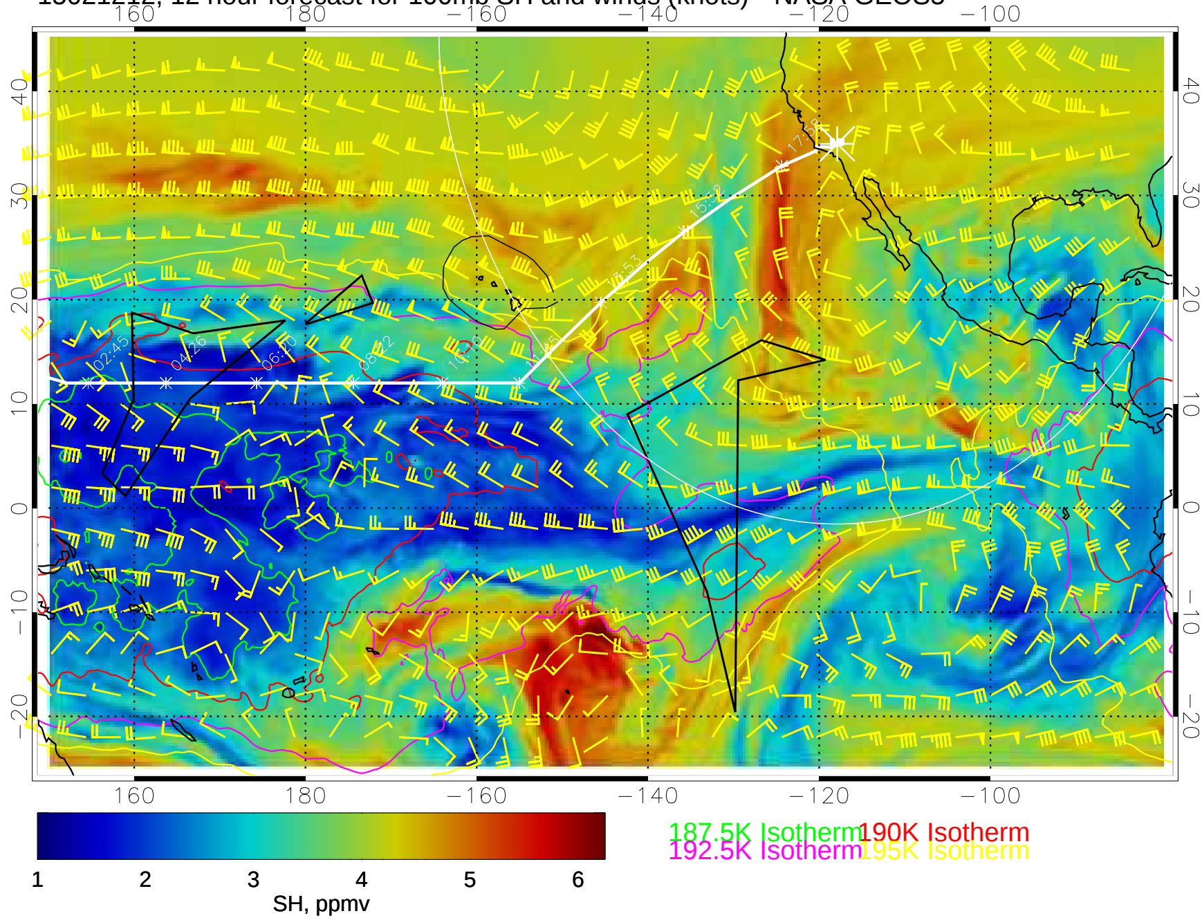
15021212, 12 hour forecast for 100mb SH and winds (knots)-- NASA GEOS5
