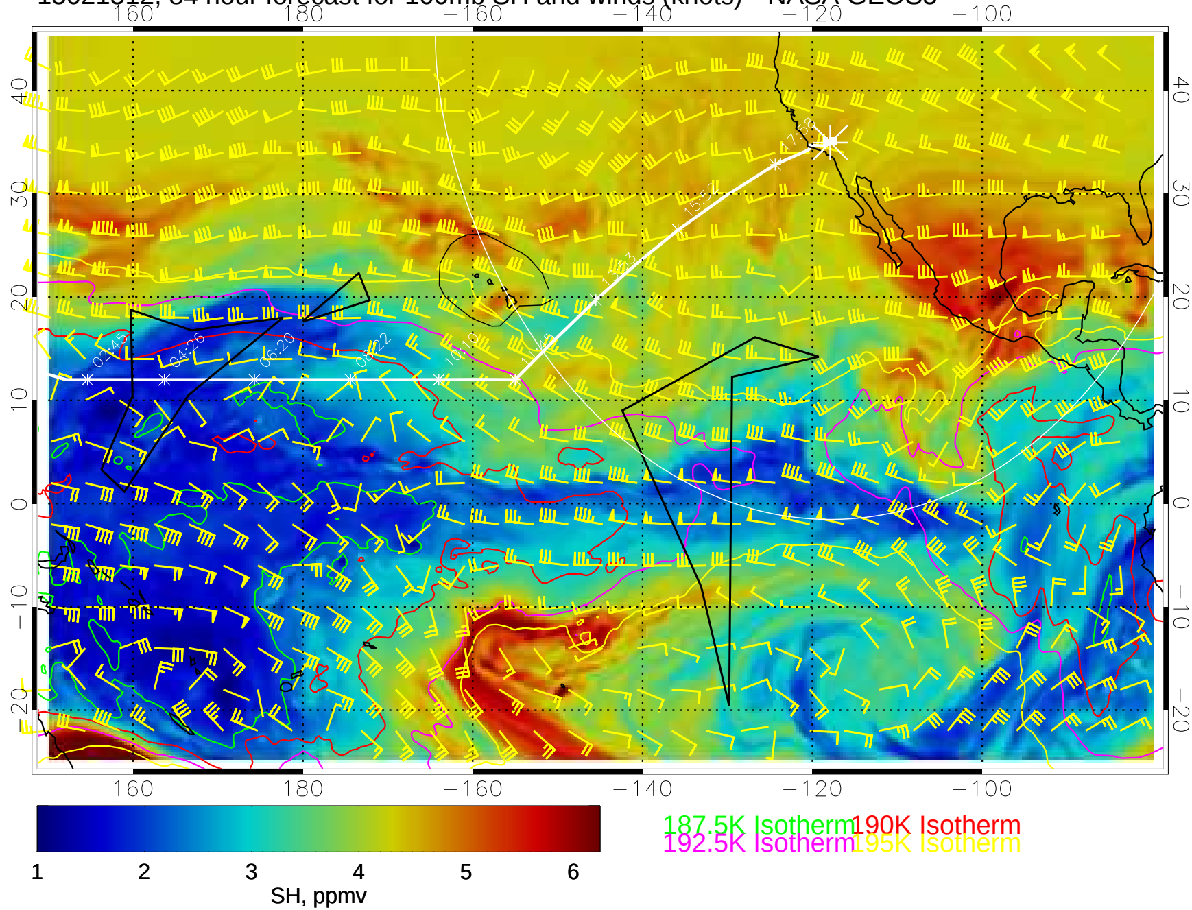
15021512, 84 hour forecast for 100mb SH and winds (knots)-- NASA GEOS5
