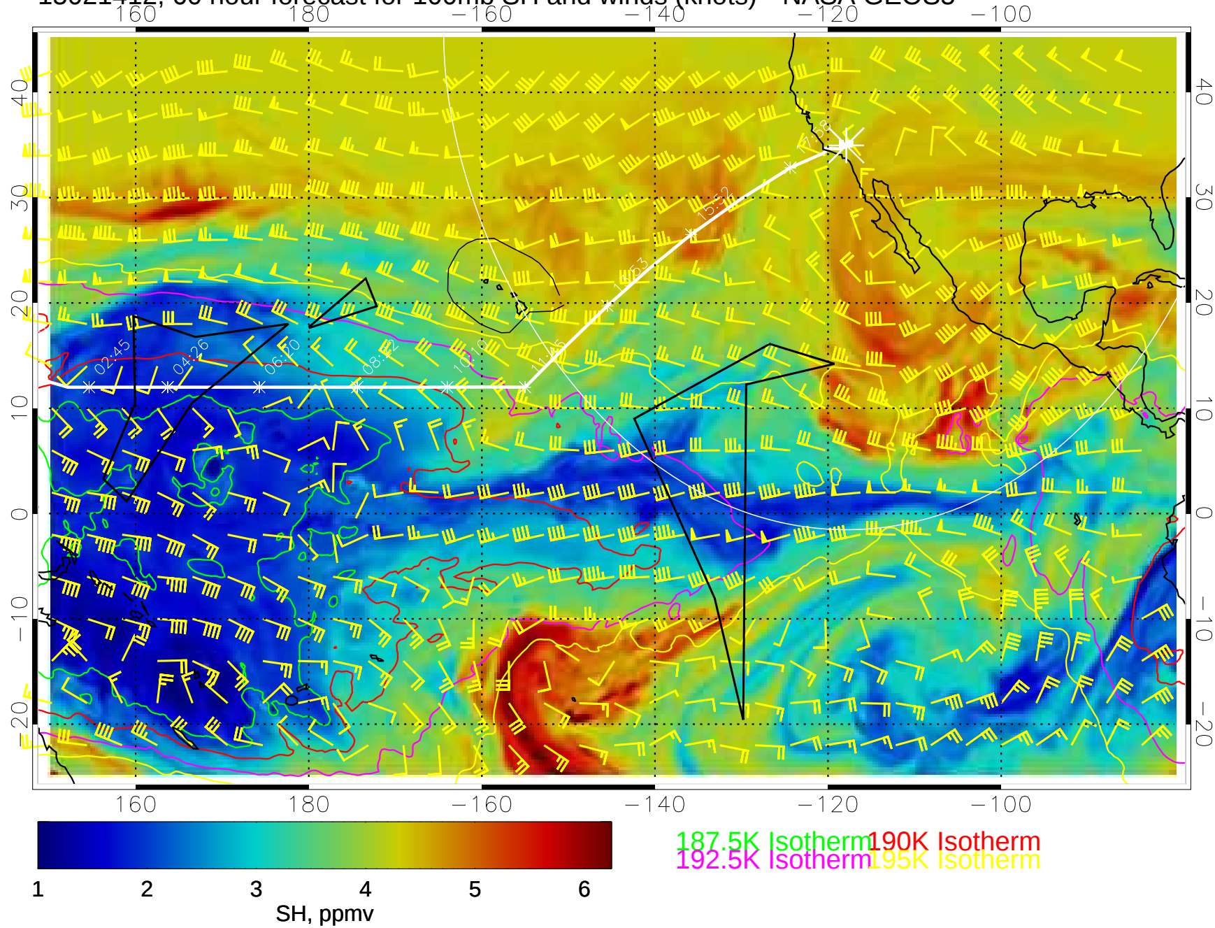
15021412, 60 hour forecast for 100mb SH and winds (knots)-- NASA GEOS5
